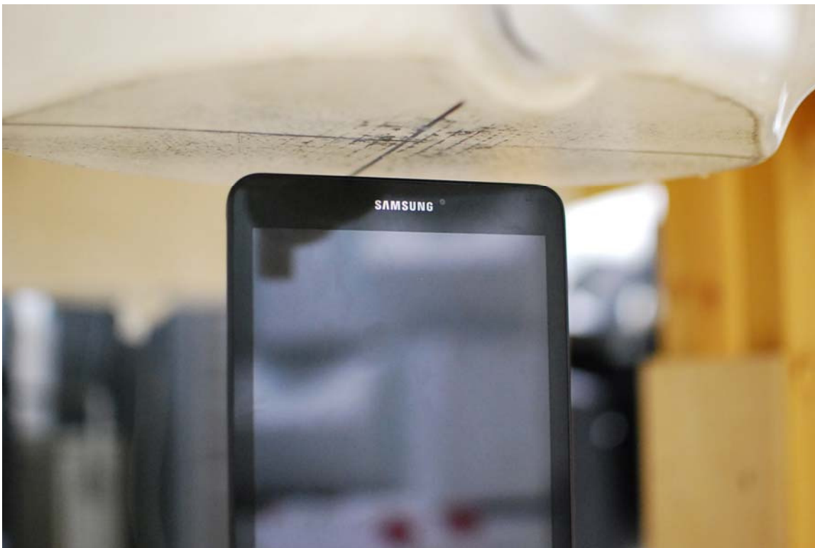
SAR Test Setup Photo 1: Top Edge at 13 mm
