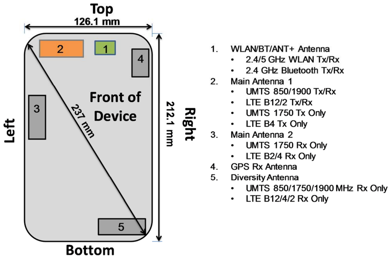
Figure F-1 DUT Antenna Locations
