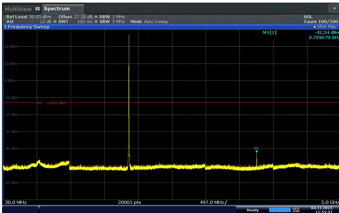
Plot 6-51. Conducted Spurious Plot (Band 2–10.0MHz–QPSK–RB Size 1–RB Offset 24–Ch.18900)
