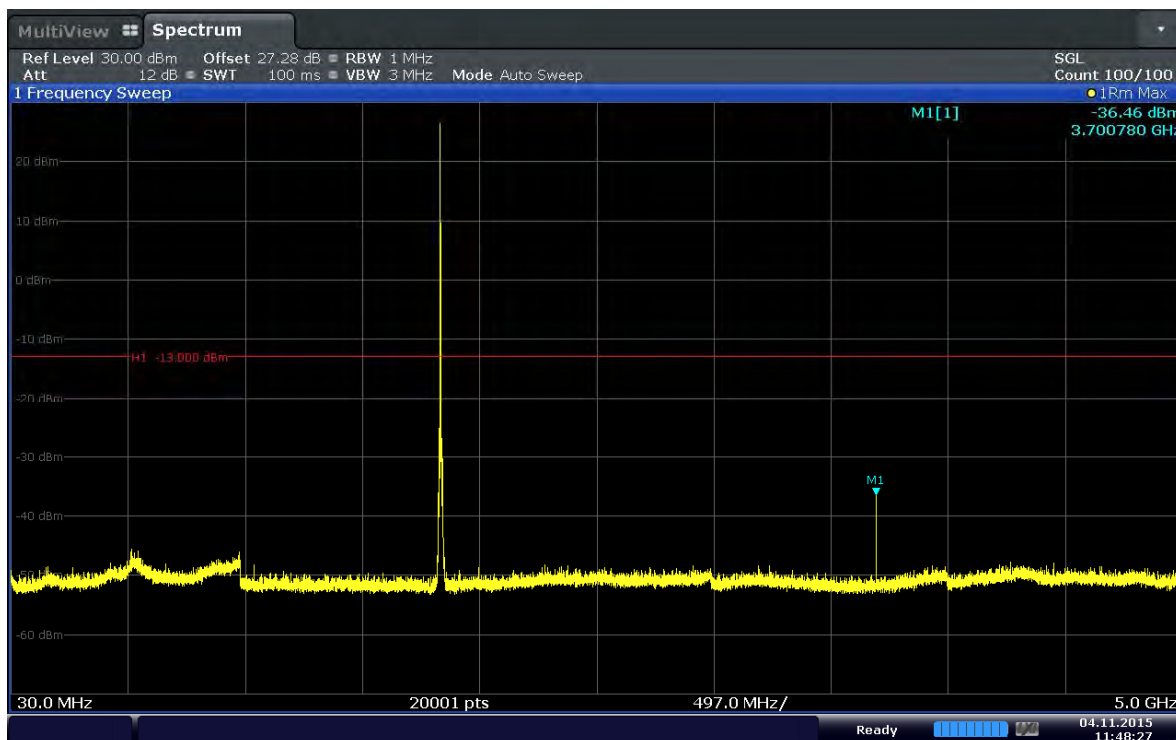
Plot 6-39. Conducted Spurious Plot (Band 2–5.0MHz–QPSK–RB Size 1–RB Offset 0–Ch.18625)
