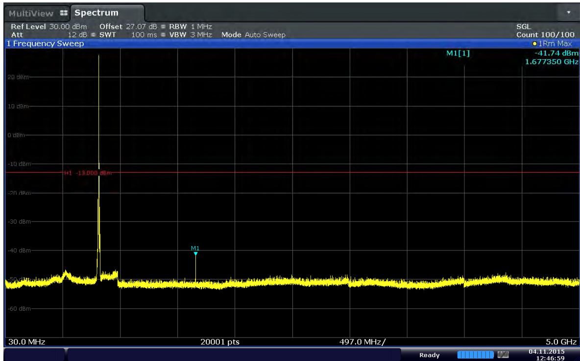
Plot 6-89. Conducted Spurious Plot (Band 5–5.0MHz–QPSK–RB Size 1–RB Offset 24–Ch.20525)
