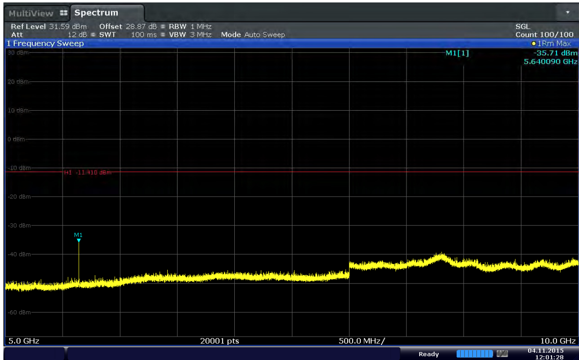
Plot 6-61. Conducted Spurious Plot (Band 2–15.0MHz–QPSK–RB Size 1–RB Offset 37–Ch.18900)
