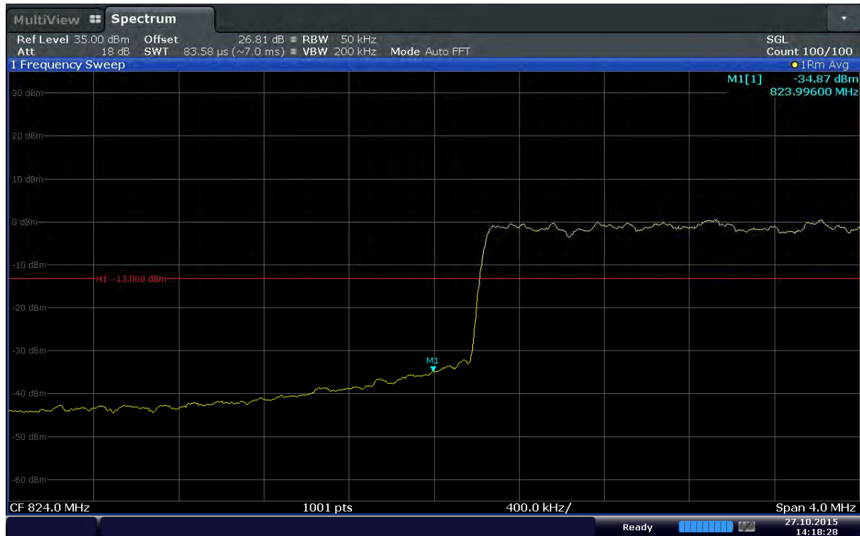
Plot 6-135. Lower Band Edge Plot (Band 5 – 5.0MHz – QPSK – RB Size 25)
