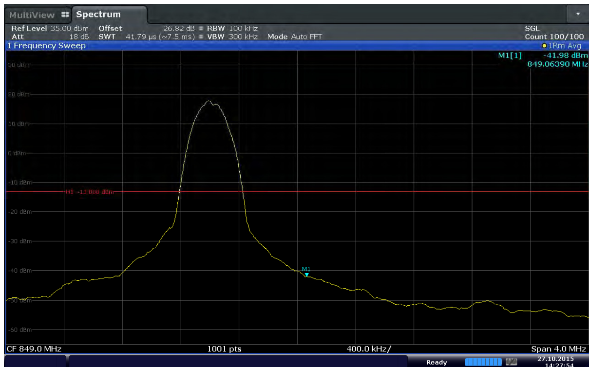
Plot 6-142. Upper Band Edge Plot (Band 5 – 10.0MHz – QPSK – RB Size 1 – RB Offset 49)
