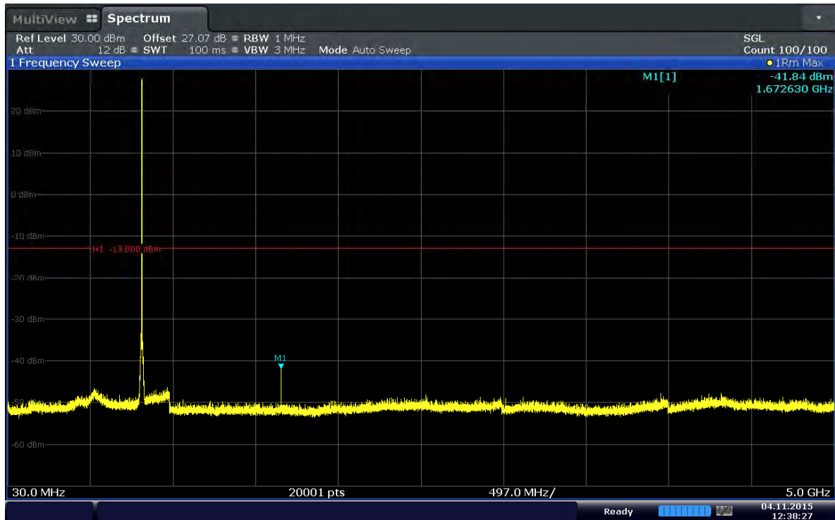
Plot 6-77. Conducted Spurious Plot (Band 5–1.4MHz–QPSK–RB Size 1–RB Offset 2–Ch.20525)
