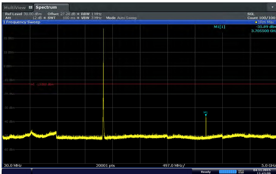
Plot 6-30. Conducted Spurious Plot (Band 2–3.0MHz–QPSK–RB Size 1–RB Offset 14–Ch.18615)
