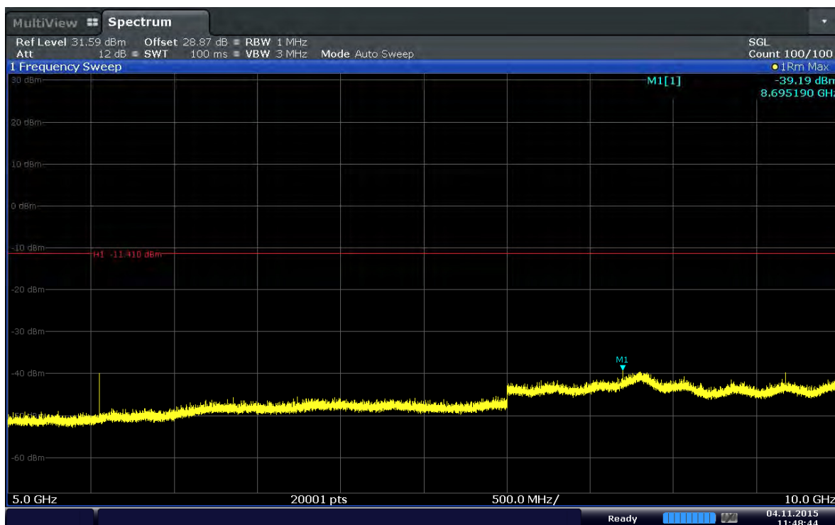
Plot 6-40. Conducted Spurious Plot (Band 2–5.0MHz–QPSK–RB Size 1–RB Offset 0–Ch.18625)
