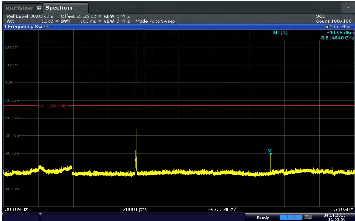
Plot 6-45. Conducted Spurious Plot (Band 2–5.0MHz–QPSK–RB Size 1–RB Offset 12–Ch.19175)
