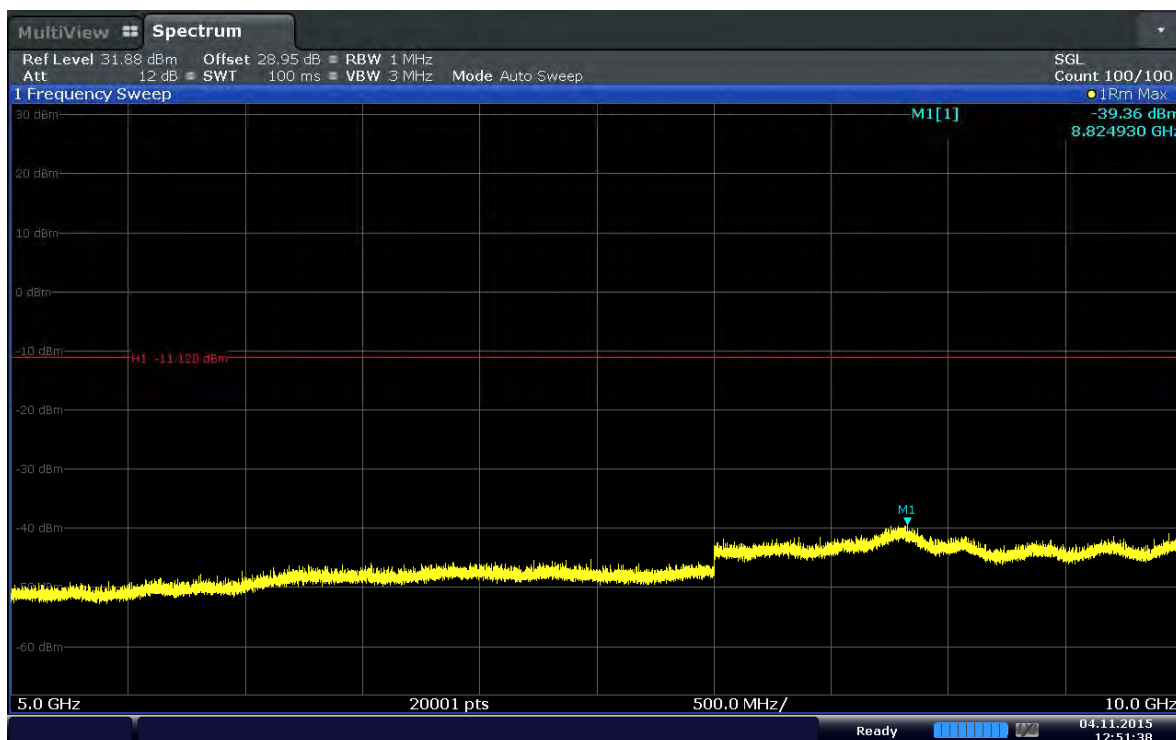
Plot 6-96. Conducted Spurious Plot (Band 5–10.0MHz–QPSK–RB Size 1–RB Offset 0–Ch.20525)
