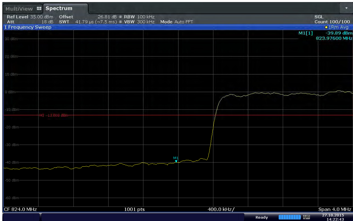
Plot 6-139. Lower Band Edge Plot (Band 5 – 10.0MHz – QPSK – RB Size 50)
