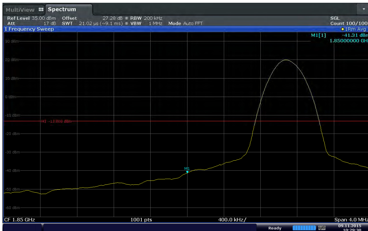
Plot 6-123. Lower Band Edge Plot (Band2 – 20.0MHz – QPSK – RB Size 1 – RB Offset 0)
