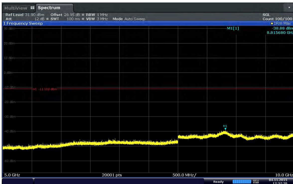
Plot 6-76. Conducted Spurious Plot (Band 5–1.4MHz–QPSK–RB Size 1–RB Offset 5–Ch.20407)
