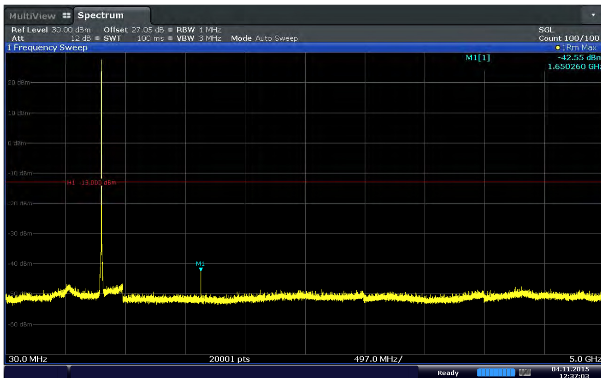
Plot 6-75. Conducted Spurious Plot (Band 5–1.4MHz–QPSK–RB Size 1–RB Offset 5–Ch.20407)
