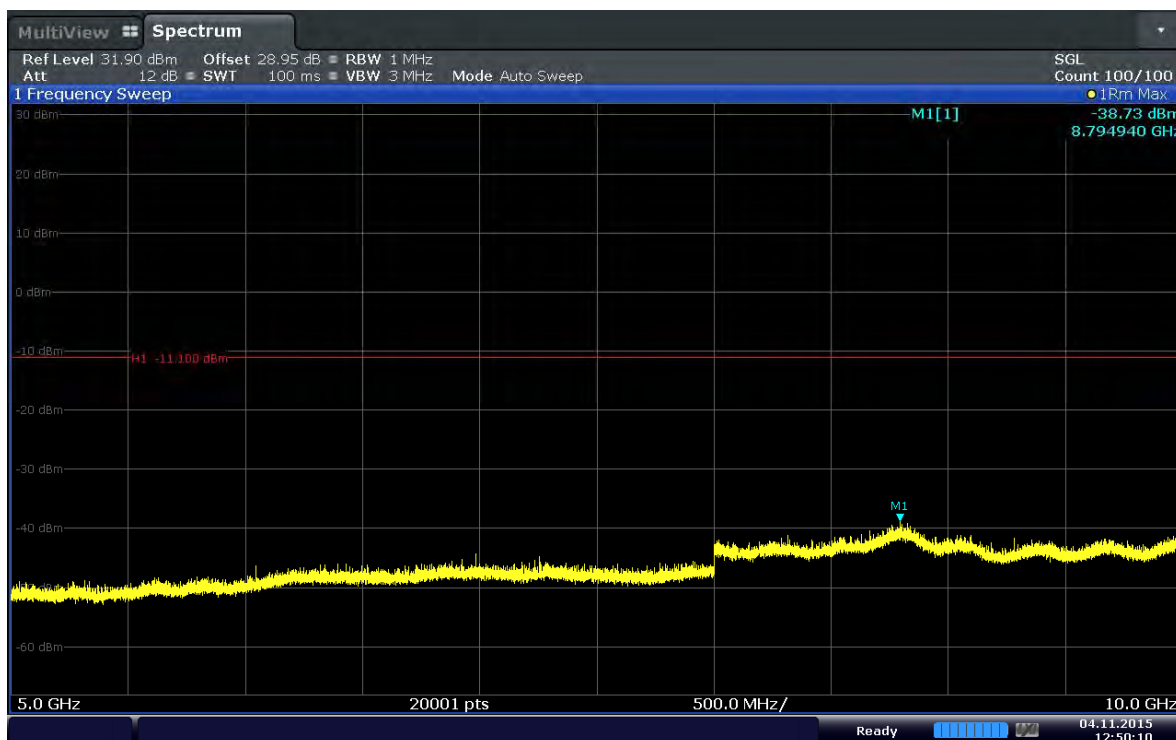
Plot 6-94. Conducted Spurious Plot (Band 5–10.0MHz–QPSK–RB Size 1–RB Offset 0–Ch.20450)
