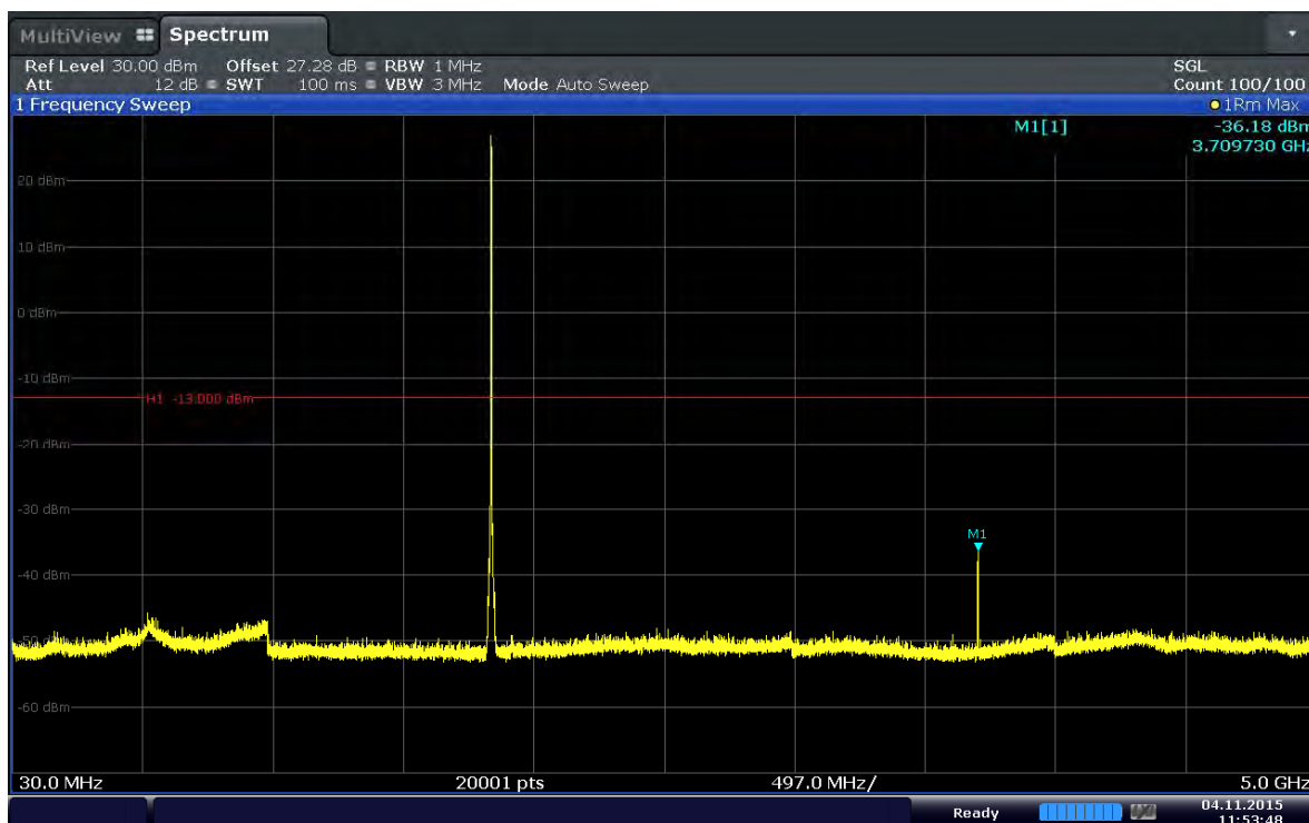
Plot 6-48. Conducted Spurious Plot (Band 2–10.0MHz–QPSK–RB Size 1–RB Offset 24–Ch.18650)
