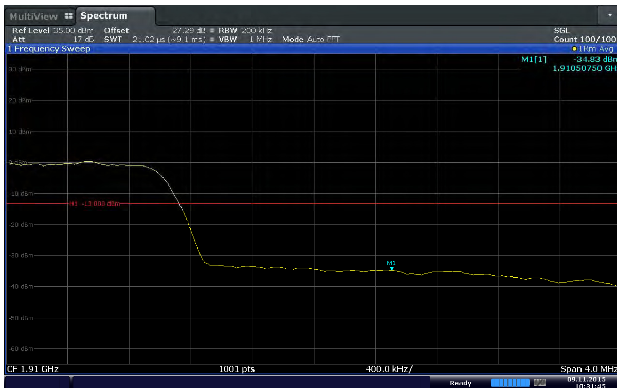
Plot 6-121. Upper Band Edge Plot (Band2 – 20.0MHz – QPSK – RB Size 100)
