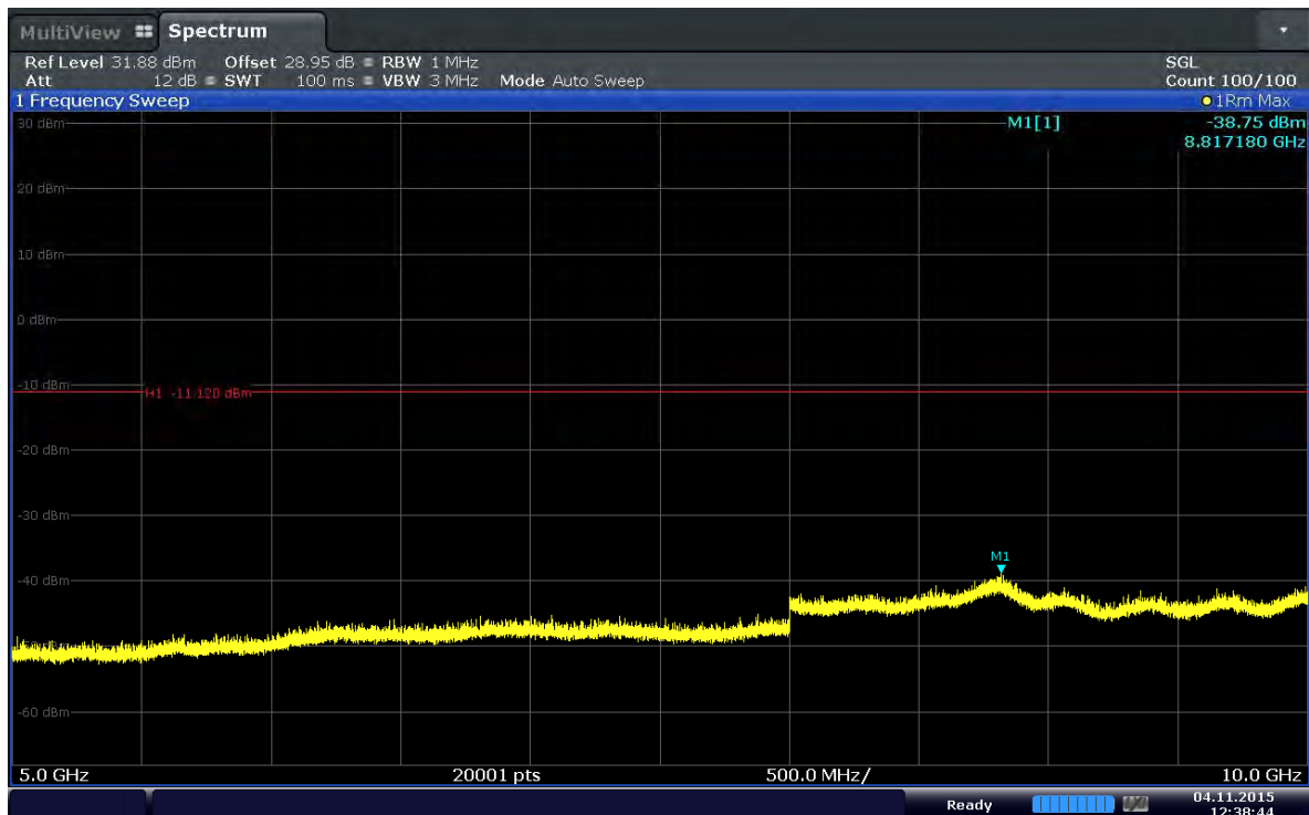
Plot 6-78. Conducted Spurious Plot (Band 5–1.4MHz–QPSK–RB Size 1–RB Offset 2–Ch.20525)
