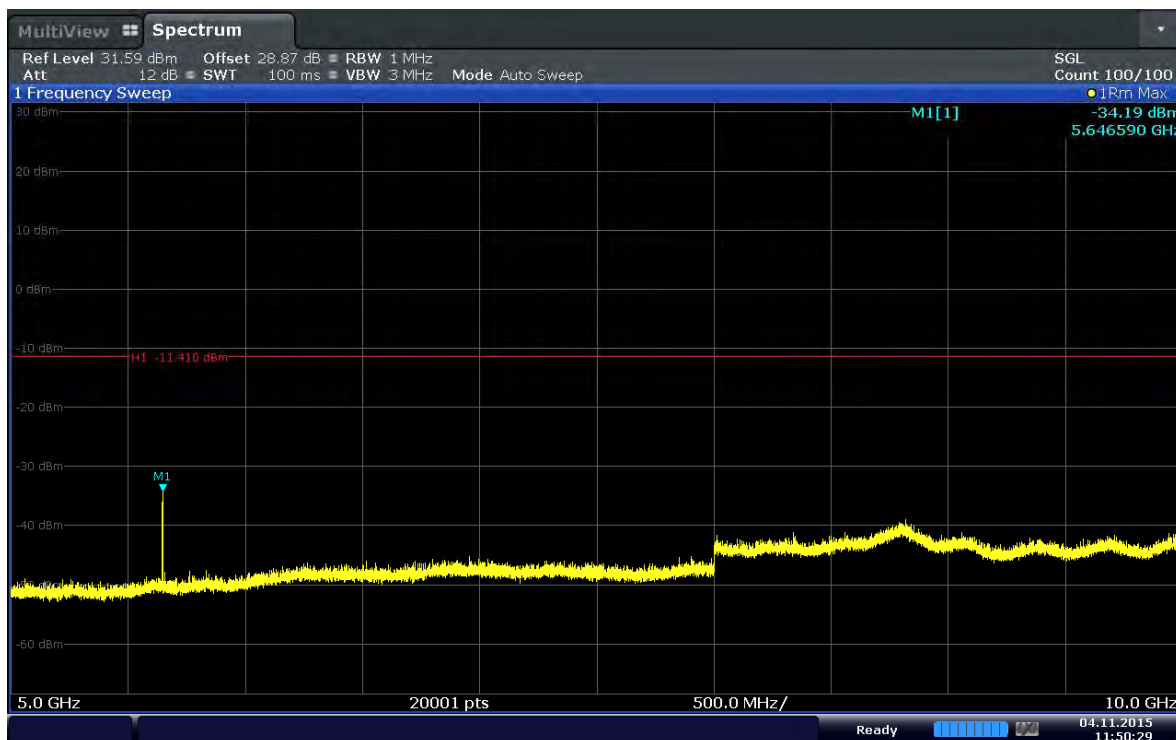
Plot 6-43. Conducted Spurious Plot (Band 2–5.0MHz–QPSK–RB Size 1–RB Offset 24–Ch.18900)
