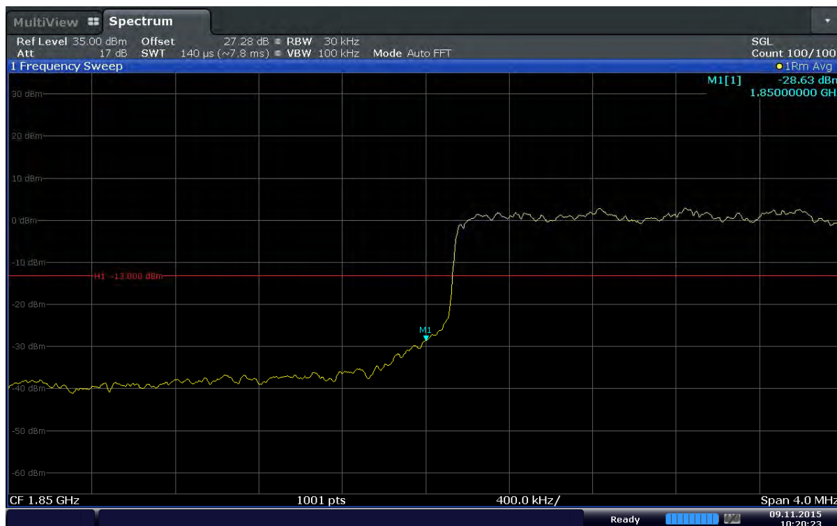
Plot 6-103. Lower Band Edge Plot (Band2 – 3.0MHz – QPSK – RB Size 15)
