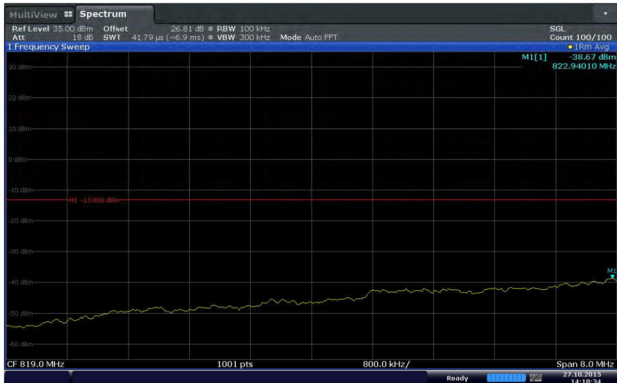
Plot 6-136. Extended Lower Band Edge Plot (Band 5 – 5.0MHz – QPSK – RB Size 25)
