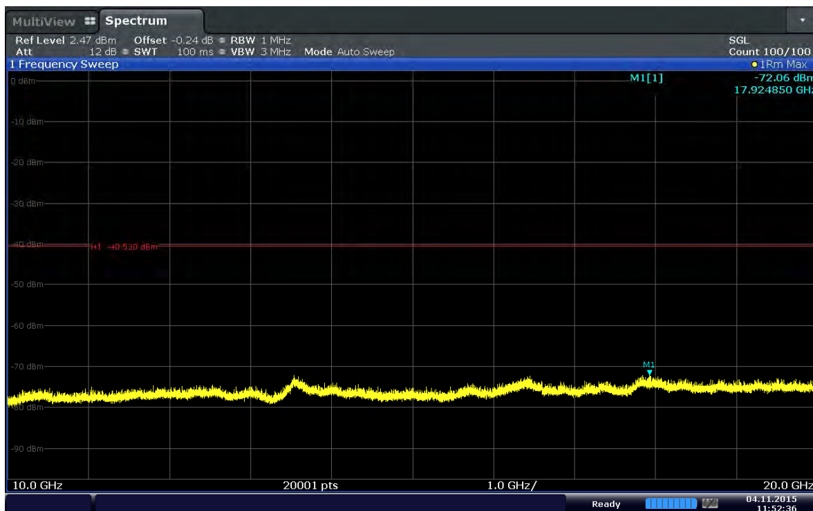
Plot 6-47. Conducted Spurious Plot (Band 2–5.0MHz–QPSK–RB Size 1–RB Offset 12–Ch.19175)
