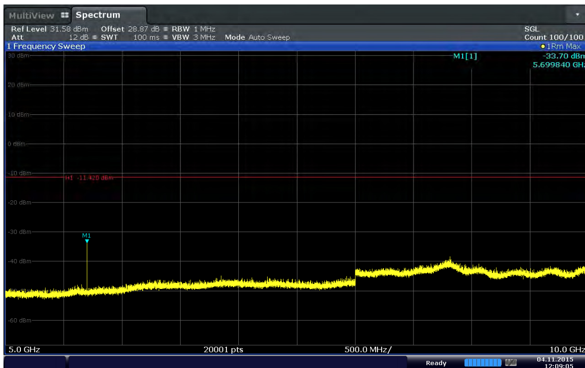
Plot 6-73. Conducted Spurious Plot (Band 2–20.0MHz–QPSK–RB Size 1–RB Offset 49–Ch.19100)
