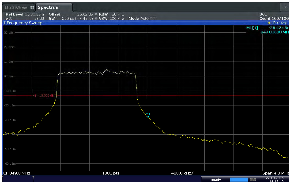
Plot 6-129. Upper Band Edge Plot (Band 5 – 1.4MHz – QPSK – RB Size 6)
