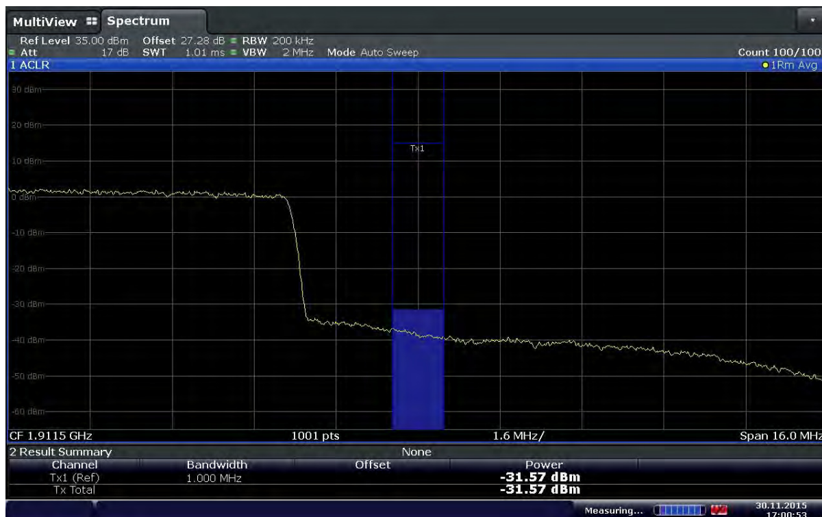
Plot 6-122. Extended Upper Band Edge Plot (Band2 – 20.0MHz – QPSK – RB Size 100)
