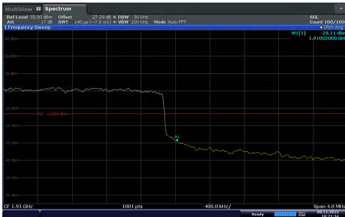
Plot 6-105. Upper Band Edge Plot (Band2 – 3.0MHz – QPSK – RB Size 15)
