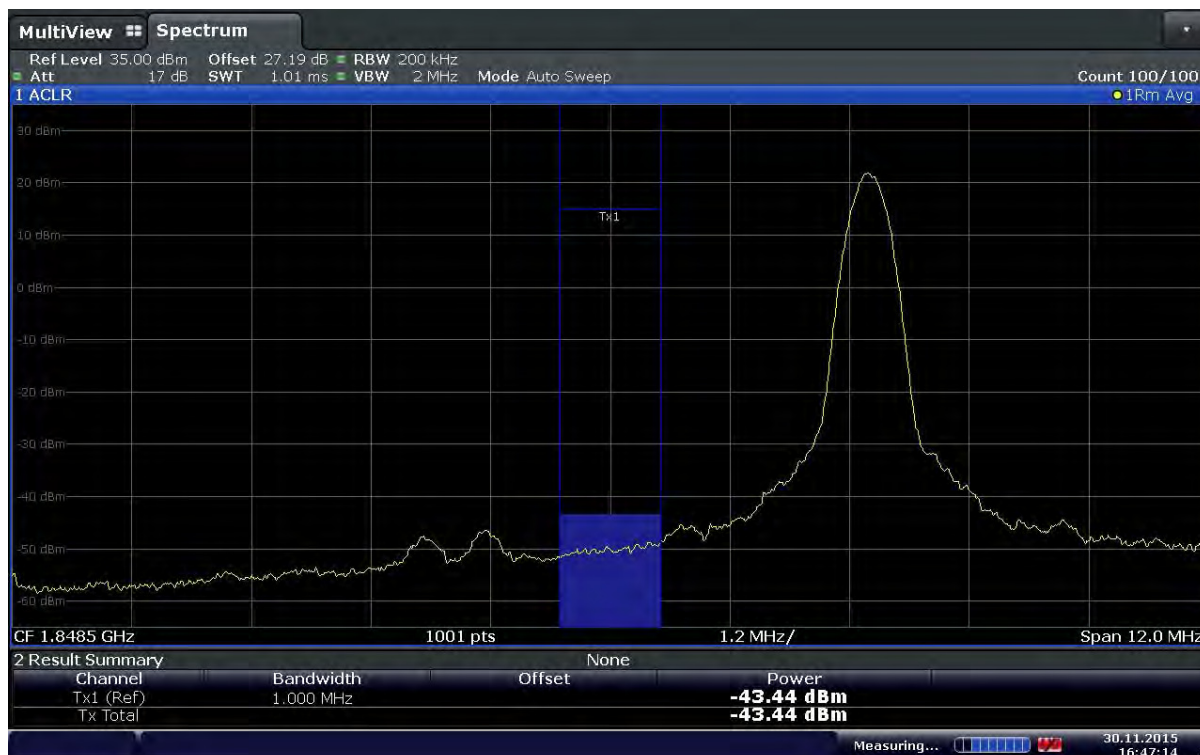
Plot 6-124. Extended Lower Band Edge Plot (Band2 – 20.0MHz – QPSK – RB Size 1 – RB Offset 0)
