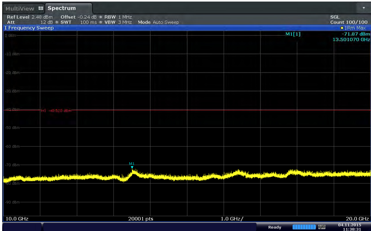
Plot 6-23. Conducted Spurious Plot (Band 2–1.4MHz–QPSK–RB Size 1–RB Offset 0–Ch.18607)
