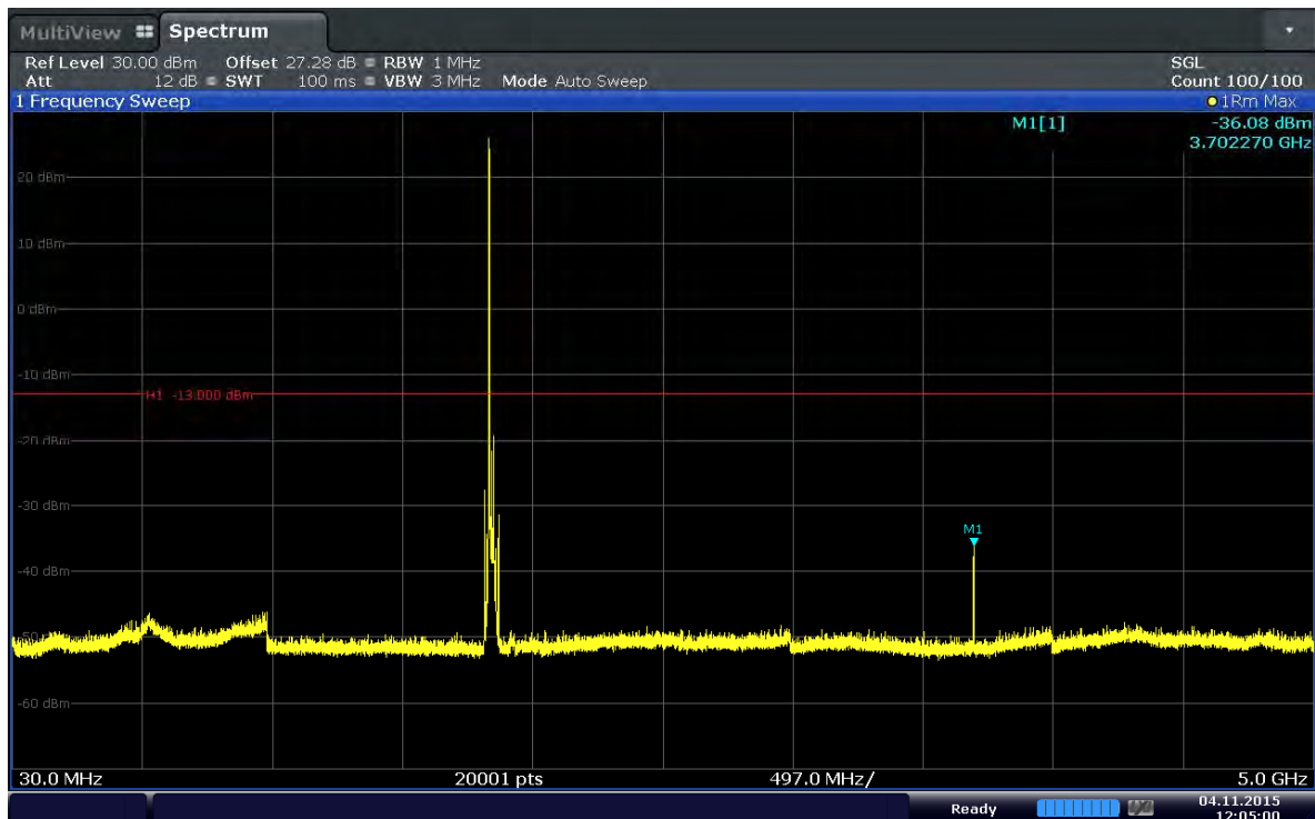
Plot 6-66. Conducted Spurious Plot (Band 2–20.0MHz–QPSK–RB Size 1–RB Offset 0–Ch.18700)
