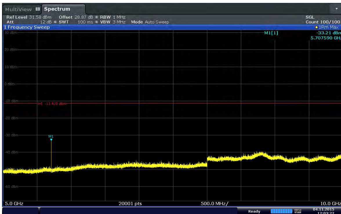
Plot 6-64. Conducted Spurious Plot (Band 2–15.0MHz–QPSK–RB Size 1–RB Offset 37–Ch.19125)
