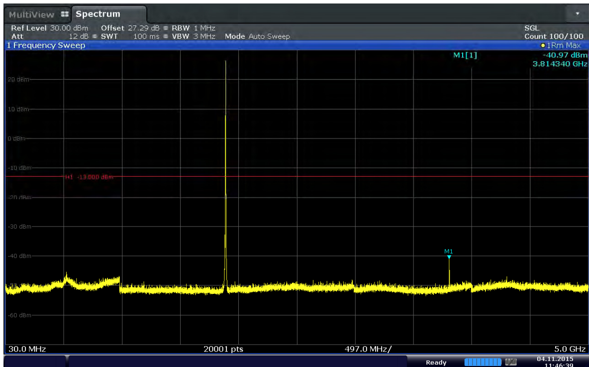
Plot 6-36. Conducted Spurious Plot (Band 2–3.0MHz–QPSK–RB Size 1–RB Offset 0–Ch.19185)
