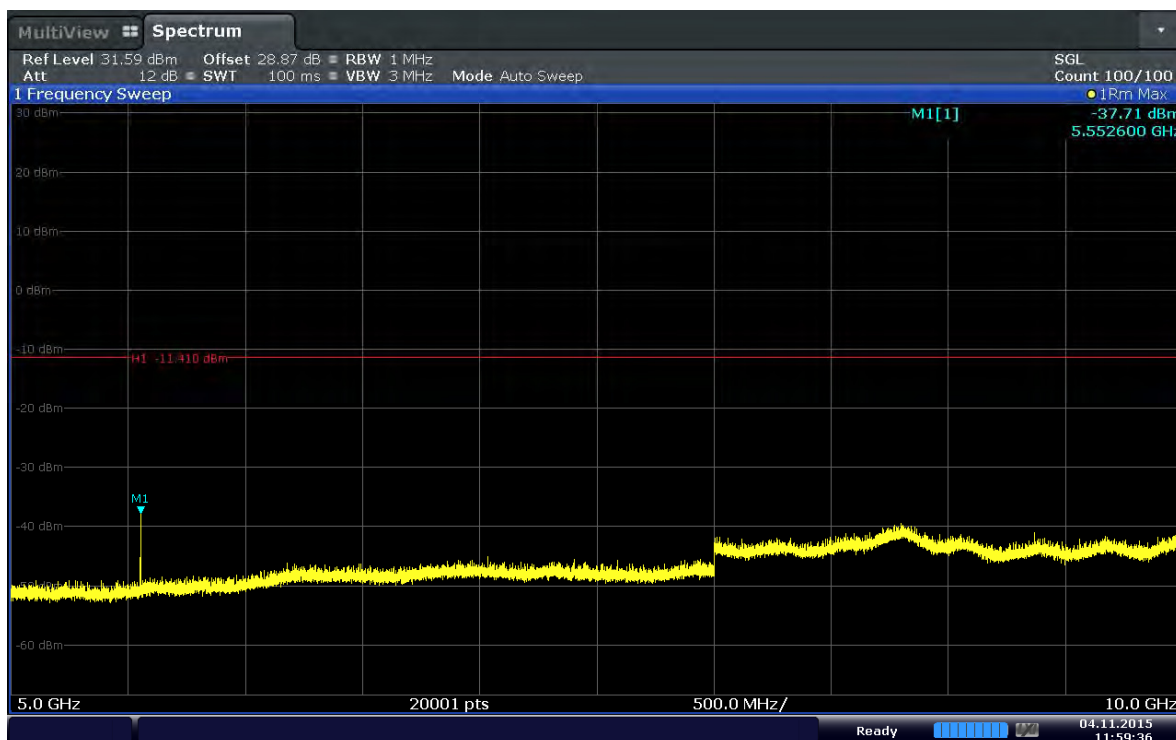
Plot 6-58. Conducted Spurious Plot (Band 2–15.0MHz–QPSK–RB Size 1–RB Offset 0–Ch.18675)
