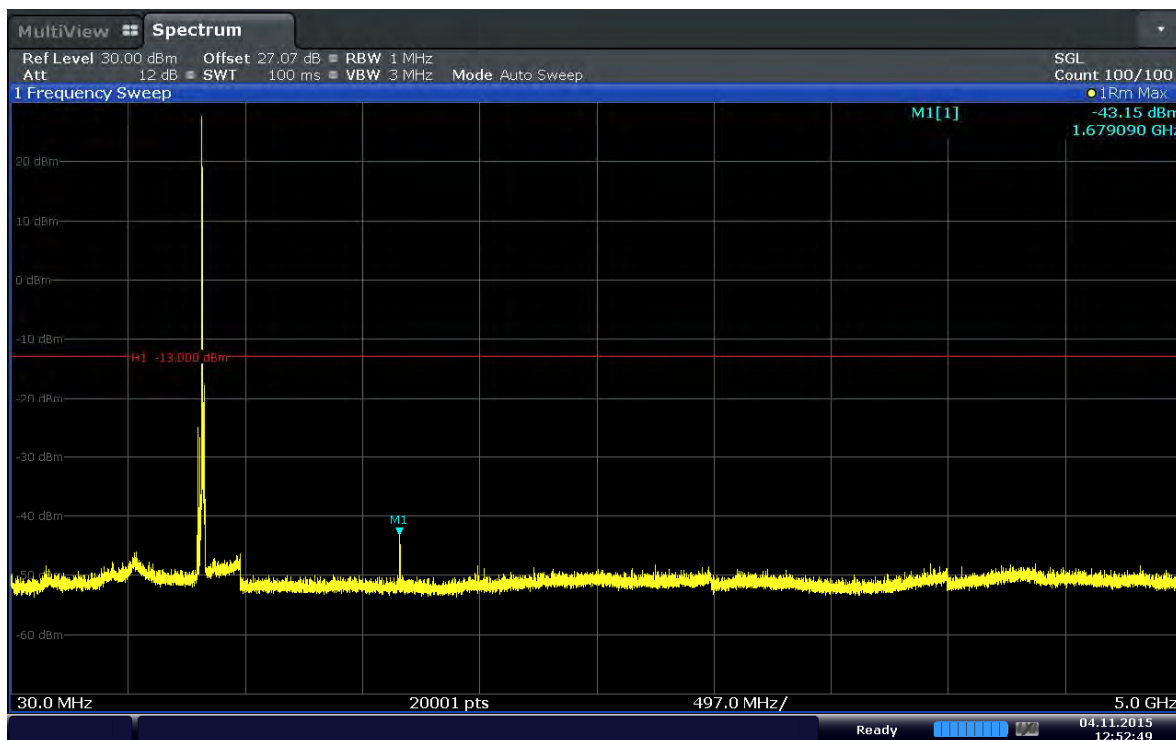
Plot 6-97. Conducted Spurious Plot (Band 5–10.0MHz–QPSK–RB Size 1–RB Offset 0–Ch.20600)
