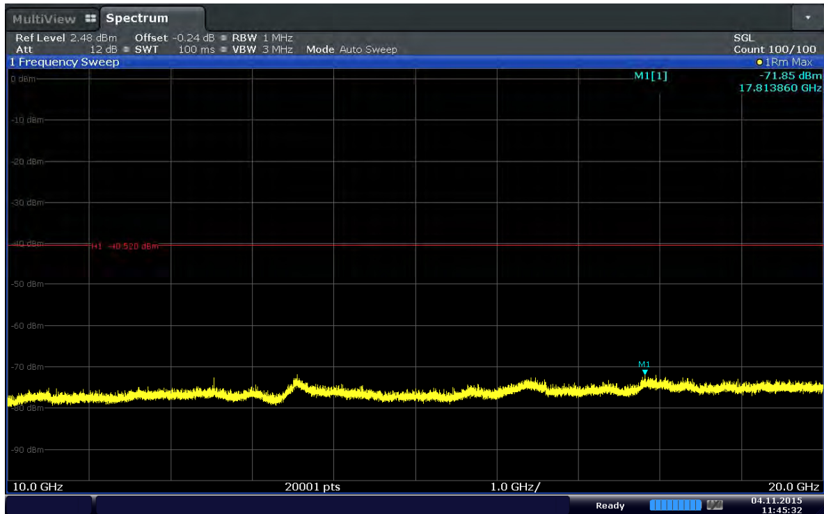
Plot 6-35. Conducted Spurious Plot (Band 2–3.0MHz–QPSK–RB Size 1–RB Offset 0–Ch.18900)
