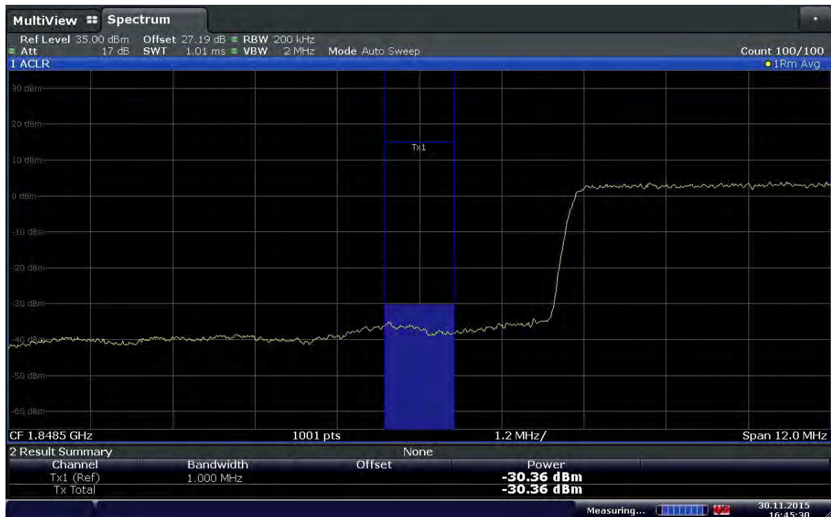
Plot 6-116. Extended Lower Band Edge Plot (Band2 – 15.0MHz – QPSK – RB Size 75)
