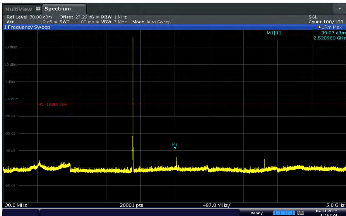
Plot 6-27. Conducted Spurious Plot (Band 2–1.4MHz–QPSK–RB Size 1–RB Offset 5–Ch.19193)
