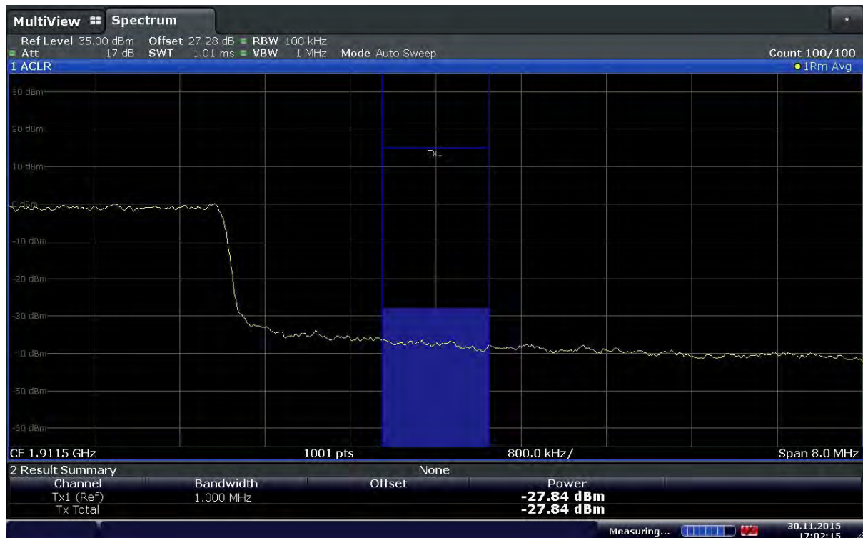
Plot 6-114. Extended Upper Band Edge Plot (Band2 – 10.0MHz – QPSK – RB Size 50)
