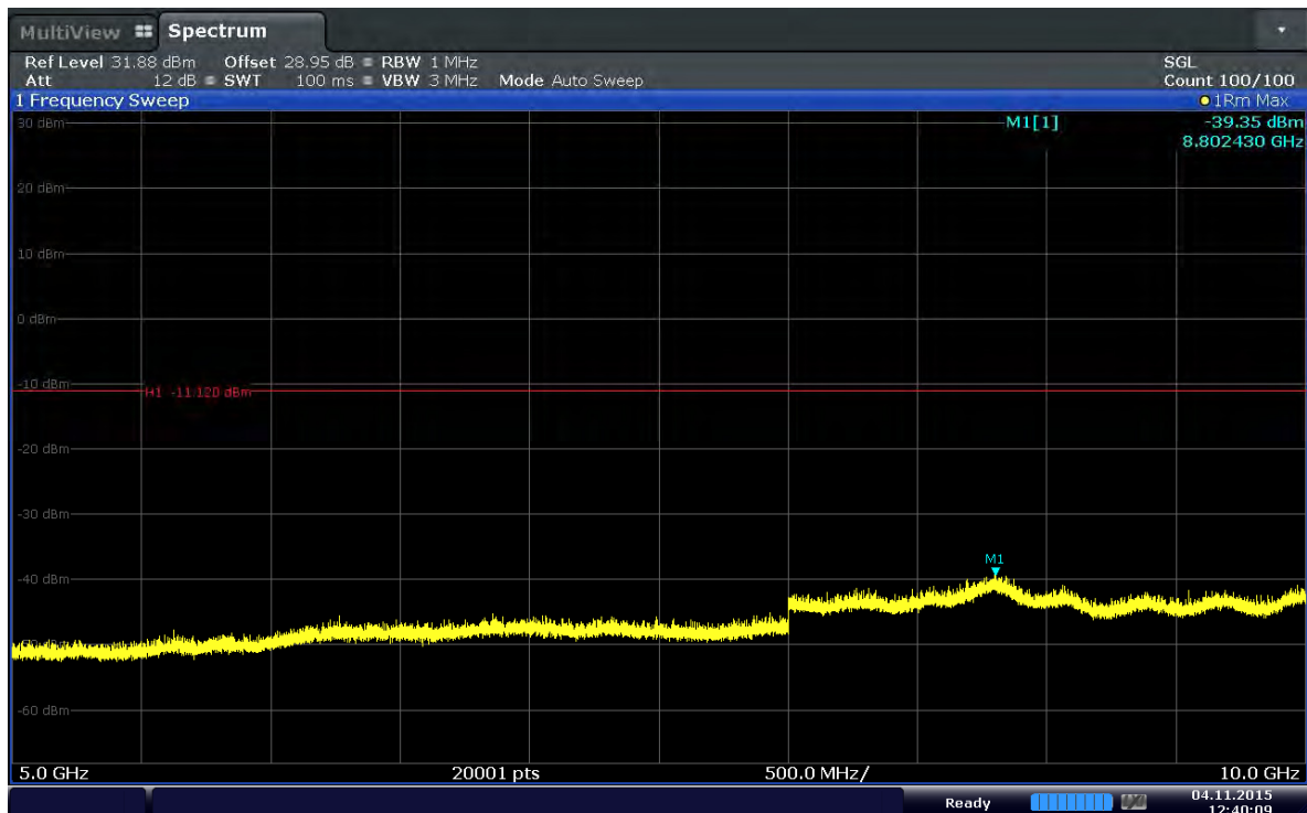
Plot 6-80. Conducted Spurious Plot (Band 5–1.4MHz–QPSK–RB Size 1–RB Offset 2–Ch.20643)
