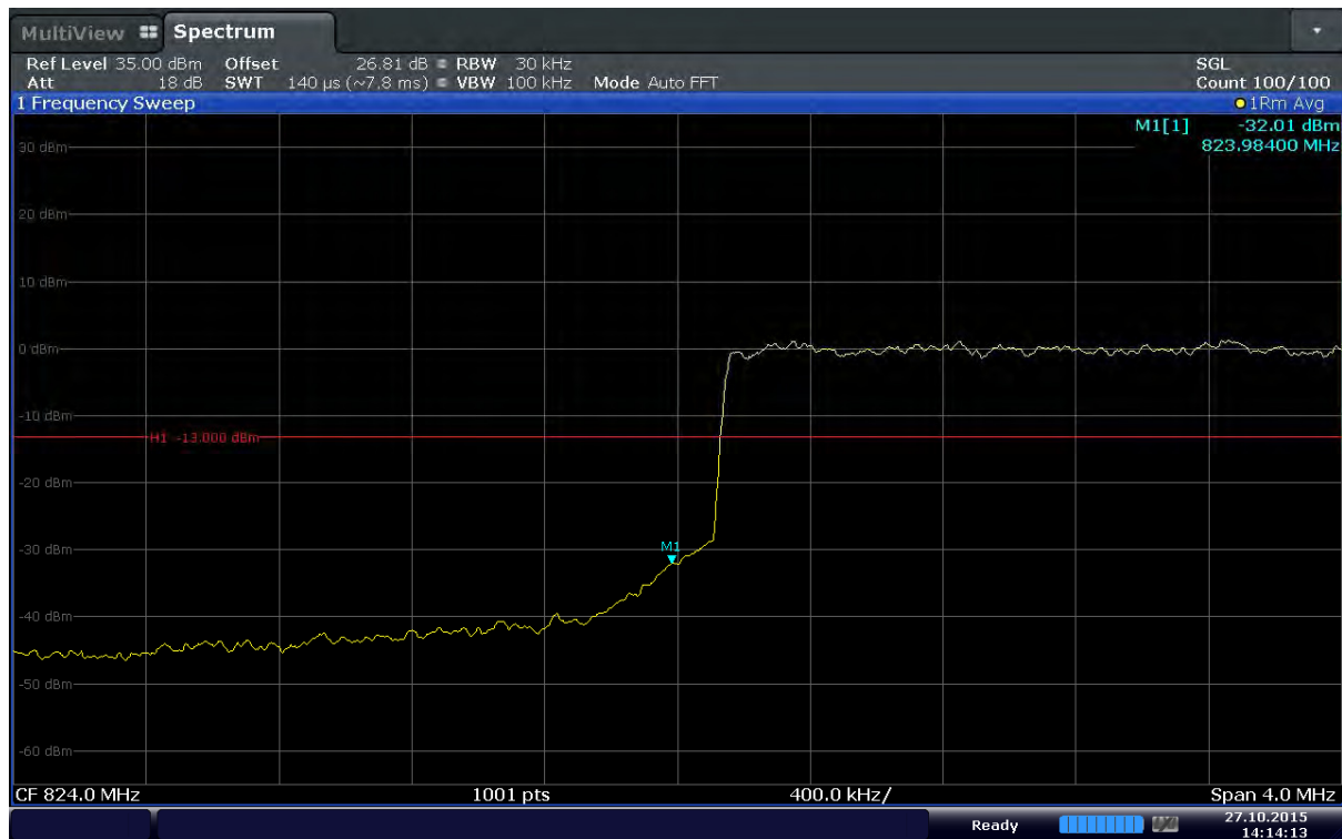
Plot 6-131. Lower Band Edge Plot (Band 5 – 3.0MHz – QPSK – RB Size 15)
