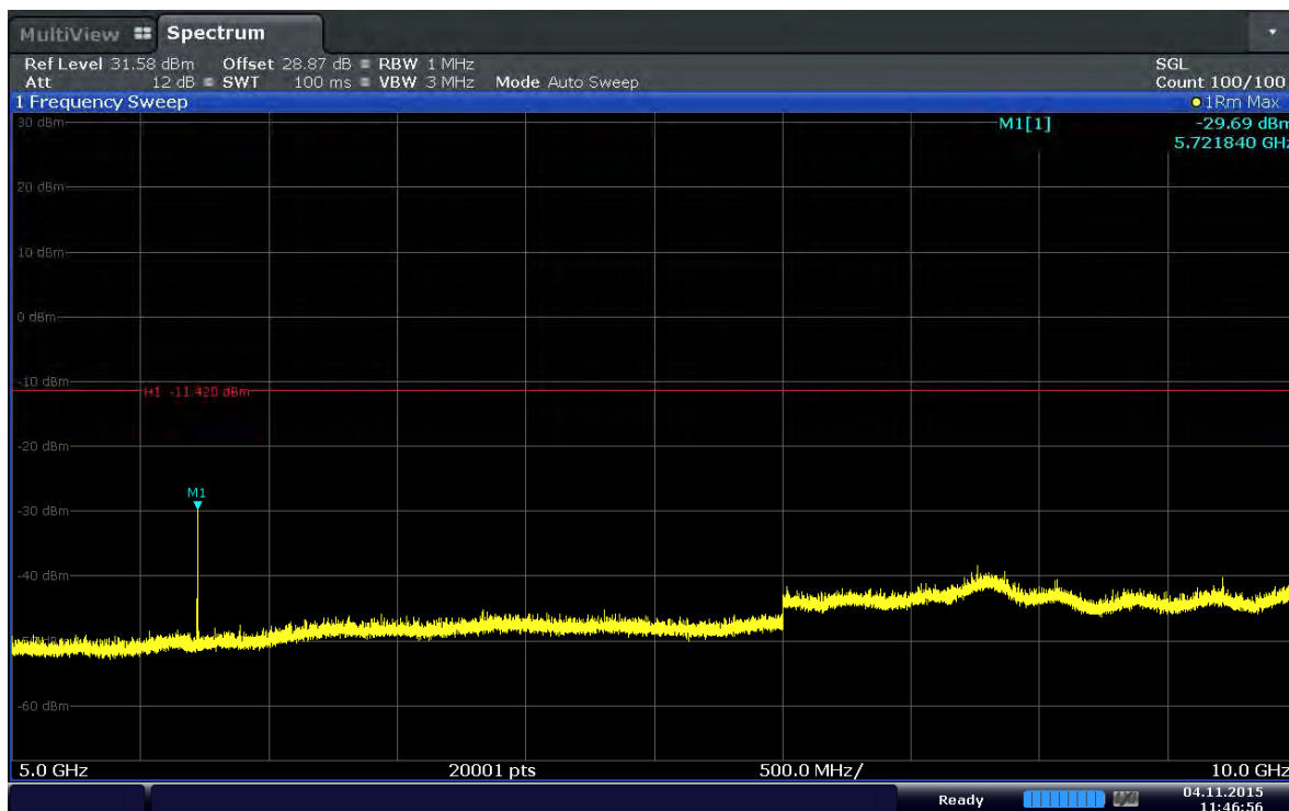
Plot 6-37. Conducted Spurious Plot (Band 2–3.0MHz–QPSK–RB Size 1–RB Offset 0–Ch.19185)
