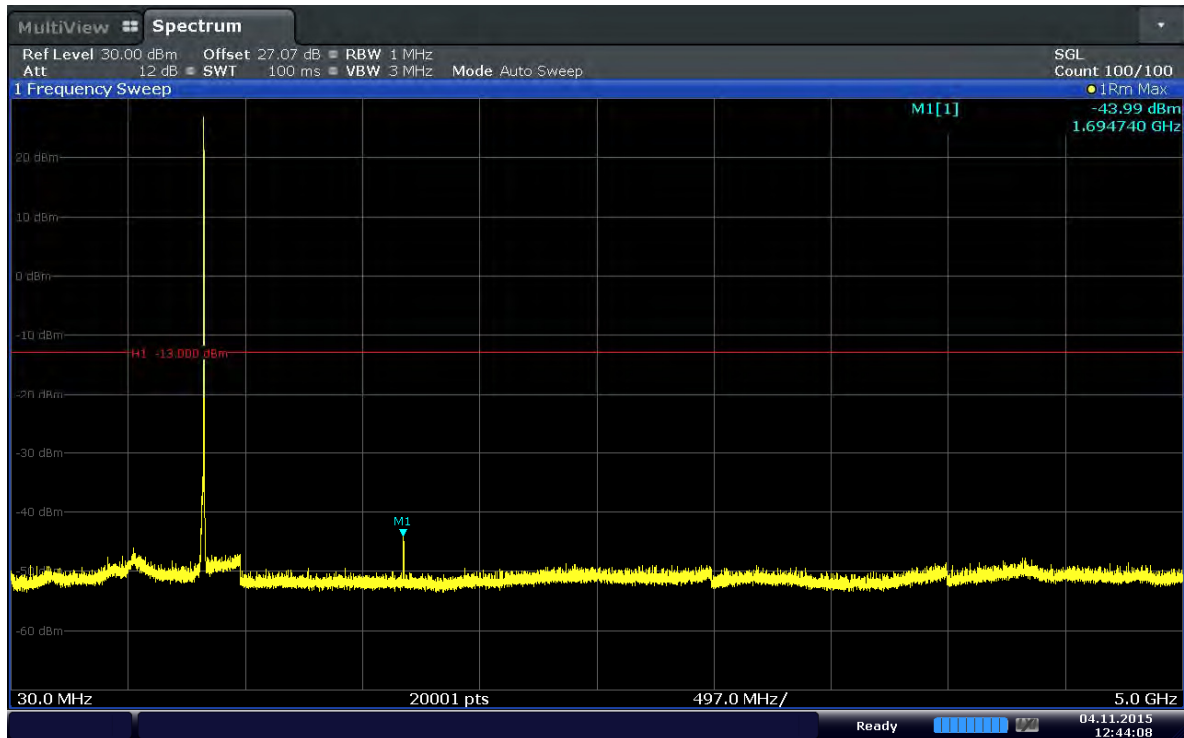
Plot 6-85. Conducted Spurious Plot (Band 5–3.0MHz–QPSK–RB Size 1–RB Offset 7–Ch.20635)
