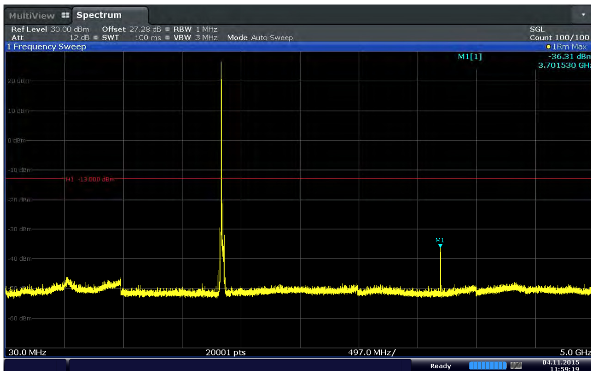
Plot 6-57. Conducted Spurious Plot (Band 2–15.0MHz–QPSK–RB Size 1–RB Offset 0–Ch.18675)
