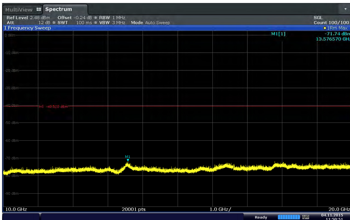
Plot 6-44. Conducted Spurious Plot (Band 2–5.0MHz–QPSK–RB Size 1–RB Offset 24–Ch.18900)
