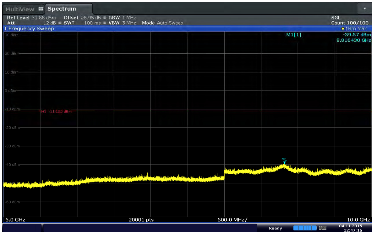
Plot 6-90. Conducted Spurious Plot (Band 5–5.0MHz–QPSK–RB Size 1–RB Offset 24–Ch.20525)
