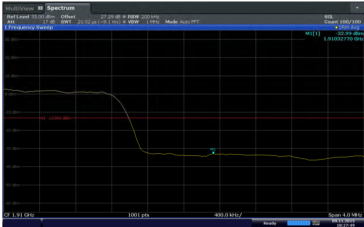
Plot 6-117. Upper Band Edge Plot (Band2 – 15.0MHz – QPSK – RB Size 75)
