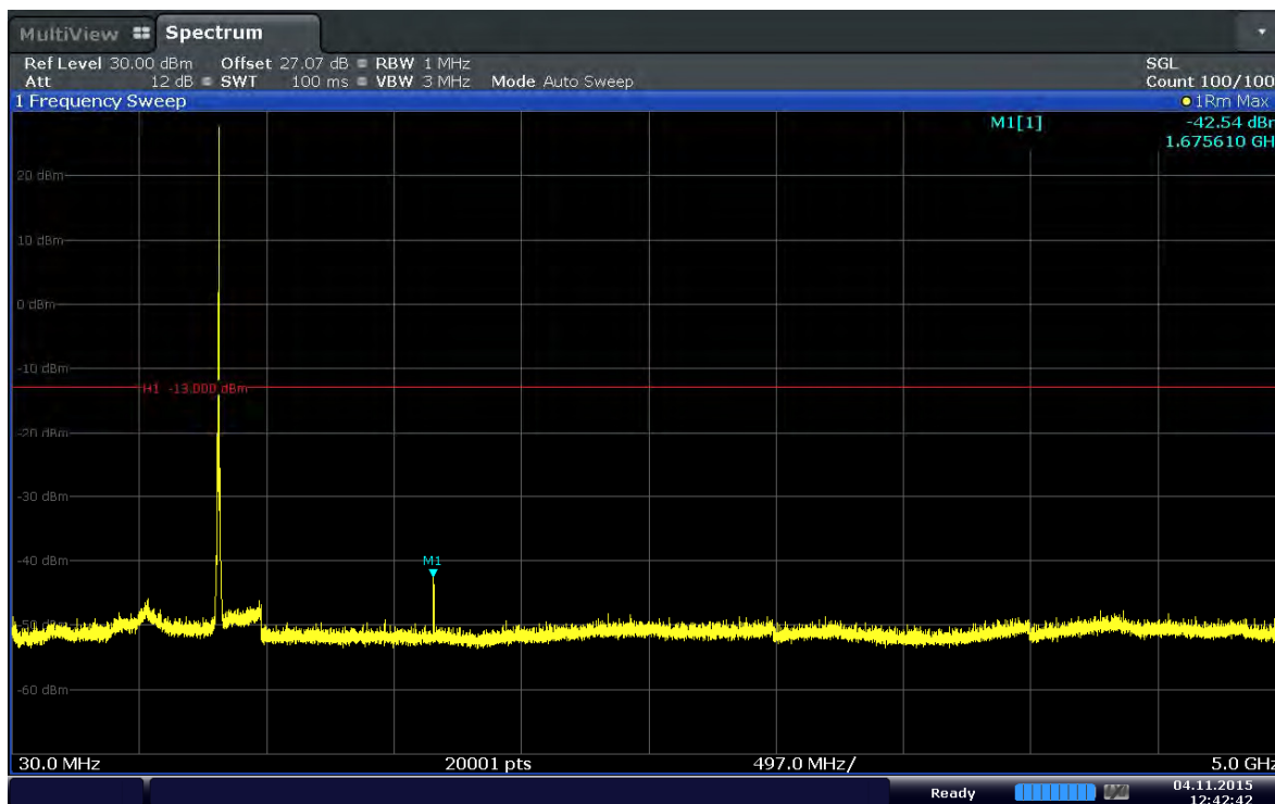
Plot 6-83. Conducted Spurious Plot (Band 5–3.0MHz–QPSK–RB Size 1–RB Offset 14–Ch.20525)
