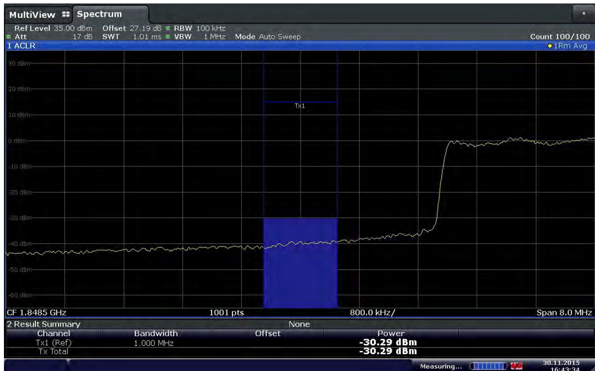
Plot 6-112. Extended Lower Band Edge Plot (Band2 – 10.0MHz – QPSK – RB Size 50)
