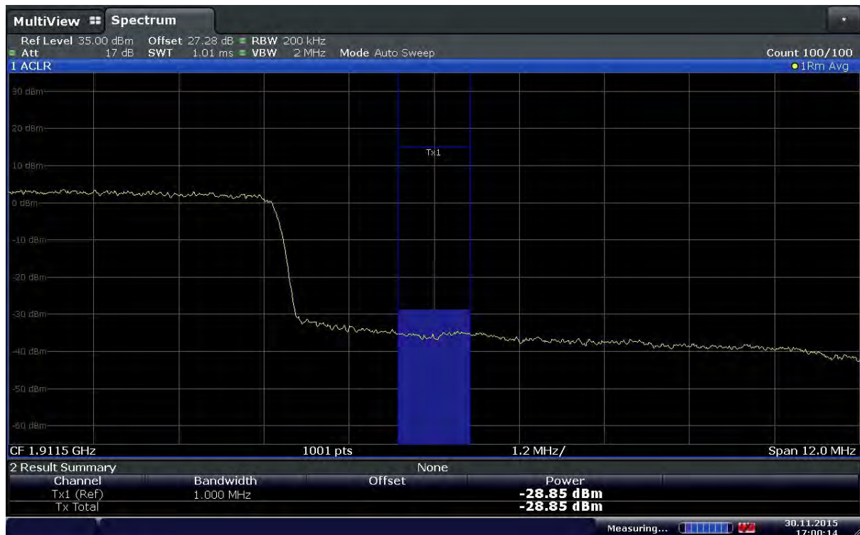
Plot 6-118. Extended Upper Band Edge Plot (Band2 – 15.0MHz – QPSK – RB Size 75)
