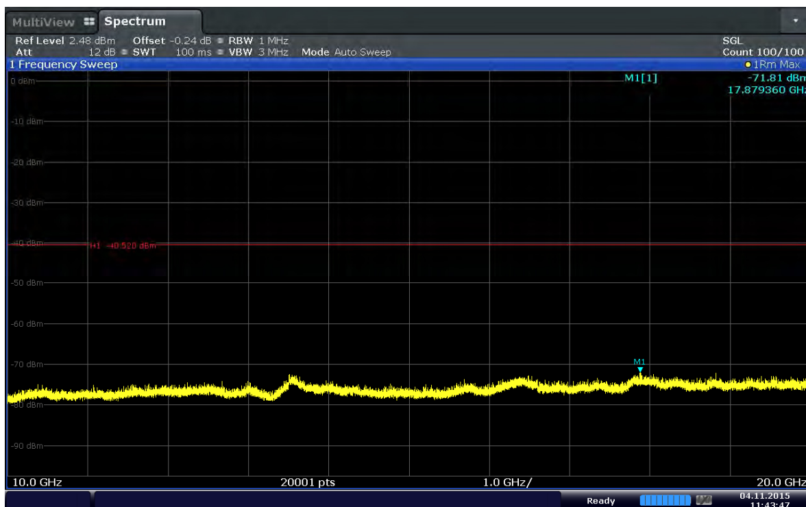
Plot 6-32. Conducted Spurious Plot (Band 2–3.0MHz–QPSK–RB Size 1–RB Offset 14–Ch.18615)
