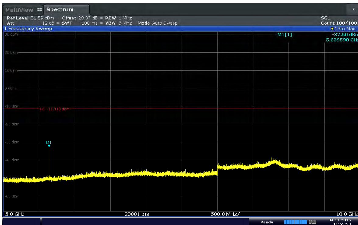
Plot 6-52. Conducted Spurious Plot (Band 2–10.0MHz–QPSK–RB Size 1–RB Offset 24–Ch.18900)
