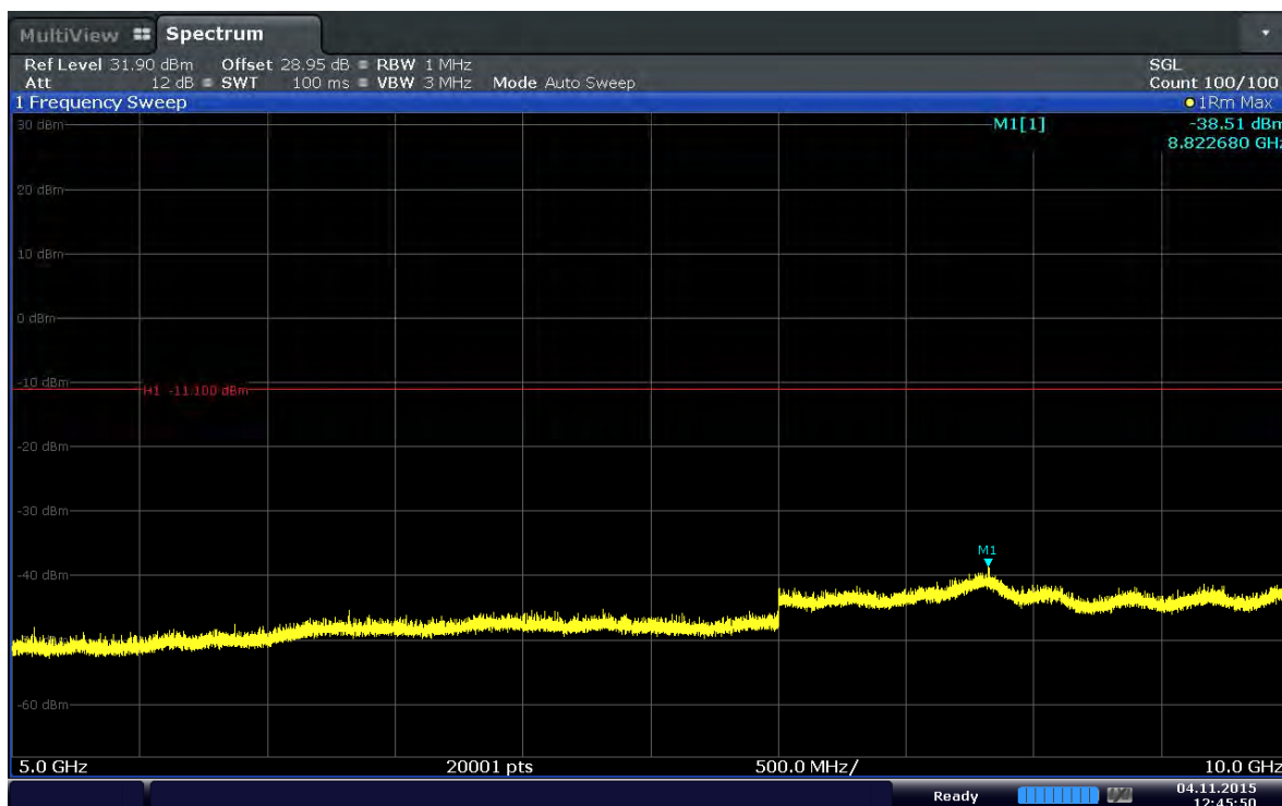
Plot 6-88. Conducted Spurious Plot (Band 5–5.0MHz–QPSK–RB Size 1–RB Offset 0–Ch.20425)
