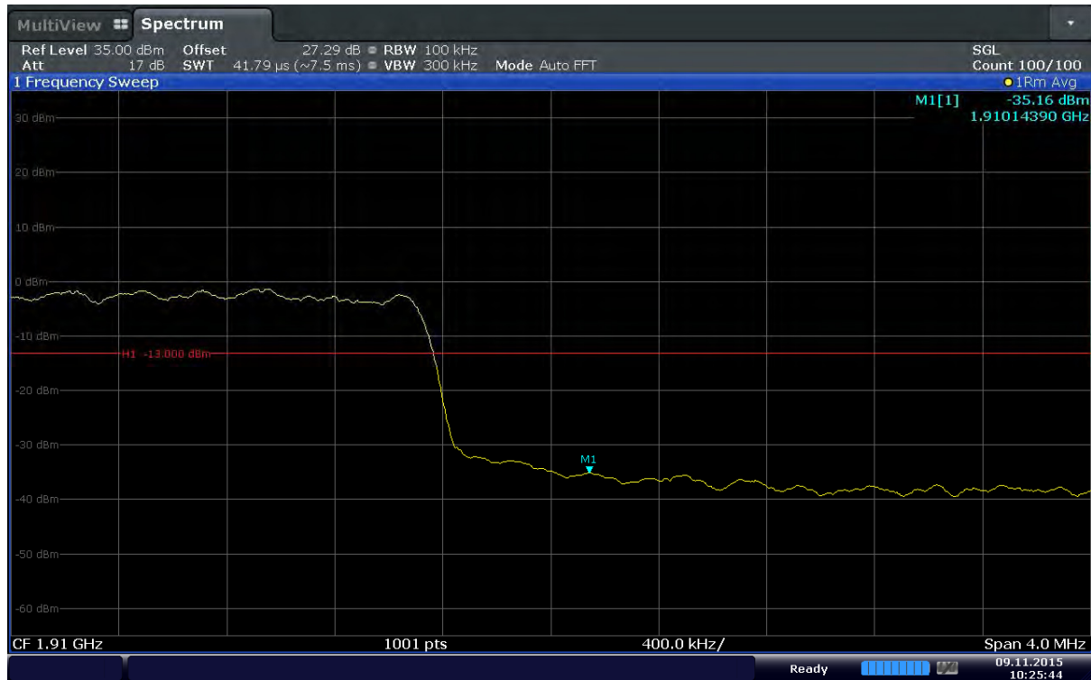
Plot 6-113. Upper Band Edge Plot (Band2 – 10.0MHz – QPSK – RB Size 50)
