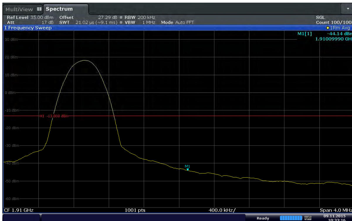
Plot 6-125. Upper Band Edge Plot (Band2 – 20.0MHz – QPSK – RB Size 1 – RB Offset 99)
