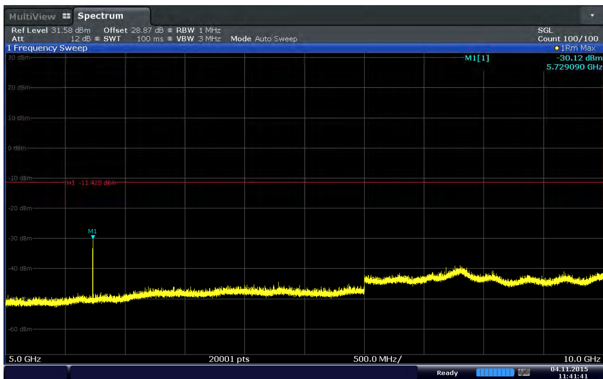
Plot 6-28. Conducted Spurious Plot (Band 2–1.4MHz–QPSK–RB Size 1–RB Offset 5–Ch.19193)
