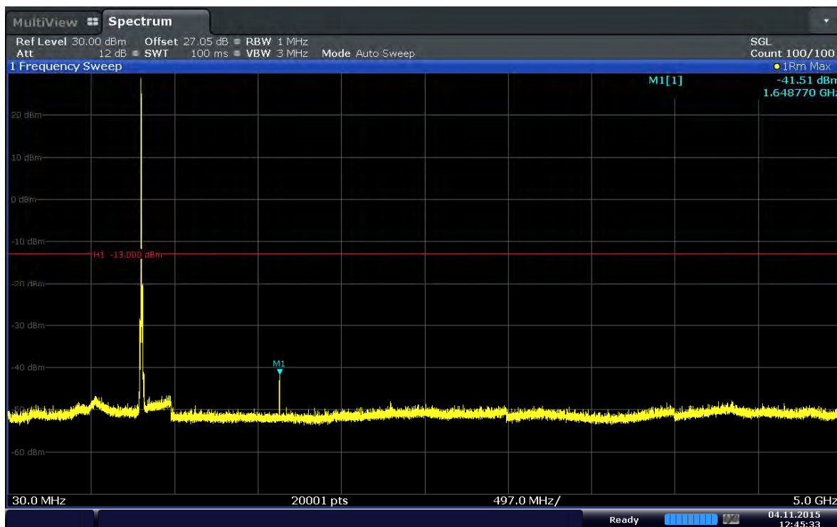
Plot 6-87. Conducted Spurious Plot (Band 5–5.0MHz–QPSK–RB Size 1–RB Offset 0–Ch.20425)
