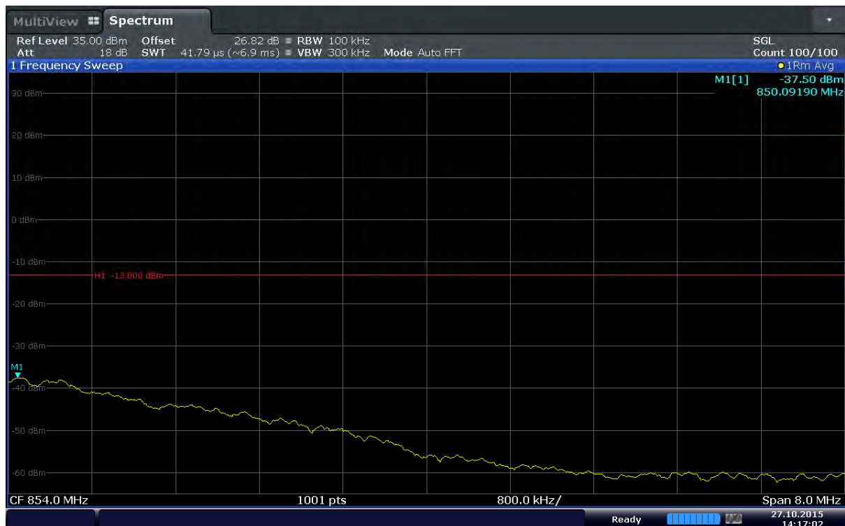
Plot 6-134. Extended Upper Band Edge Plot (Band 5 – 3.0MHz – QPSK – RB Size 15)
