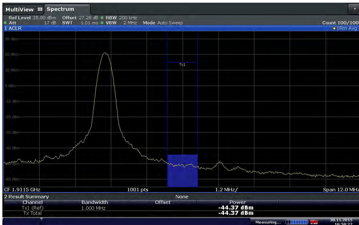
Plot 6-126. Extended Upper Band Edge Plot (Band2 – 20.0MHz – QPSK – RB Size 1 – RB Offset 99)
