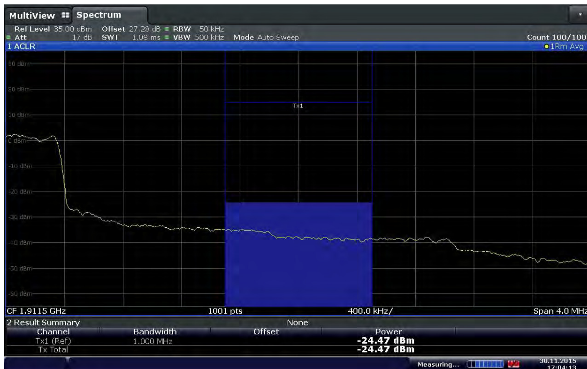
Plot 6-106. Extended Upper Band Edge Plot (Band2 – 3.0MHz – QPSK – RB Size 15)
