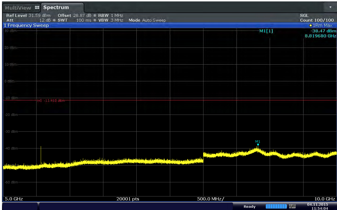
Plot 6-49. Conducted Spurious Plot (Band 2–10.0MHz–QPSK–RB Size 1–RB Offset 24–Ch.18650)
