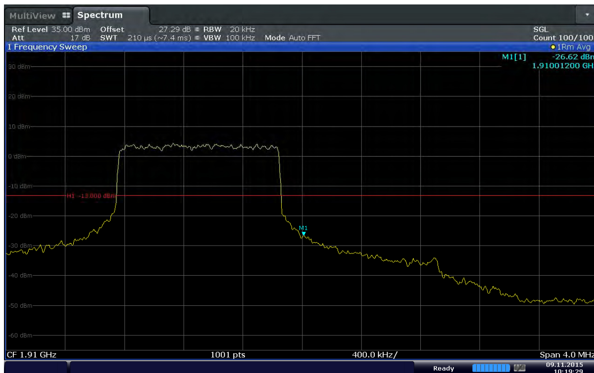
Plot 6-101. Upper Band Edge Plot (Band2 – 1.4MHz – QPSK – RB Size 6)
