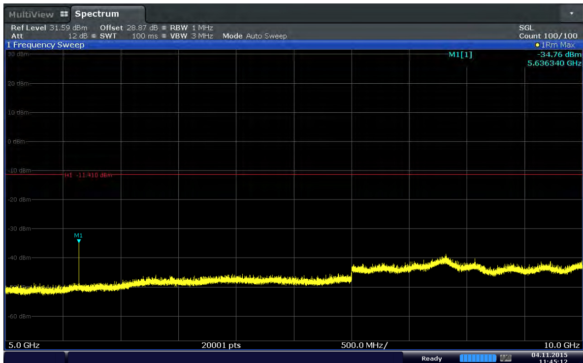
Plot 6-34. Conducted Spurious Plot (Band 2–3.0MHz–QPSK–RB Size 1–RB Offset 0–Ch.18900)
