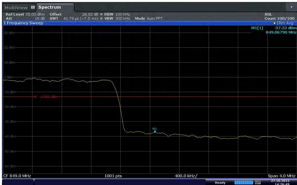
Plot 6-140. Upper Band Edge Plot (Band 5 – 10.0MHz – QPSK – RB Size 50)
