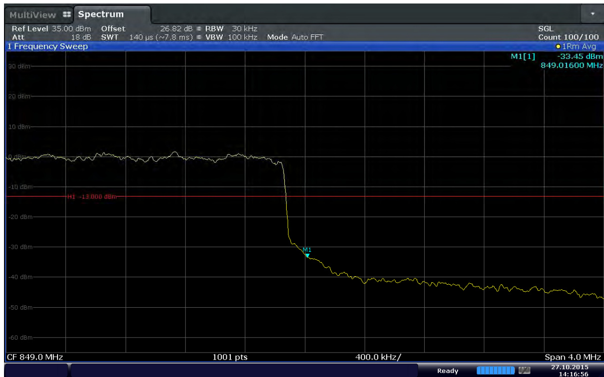
Plot 6-133. Upper Band Edge Plot (Band 5 – 3.0MHz – QPSK – RB Size 15)
