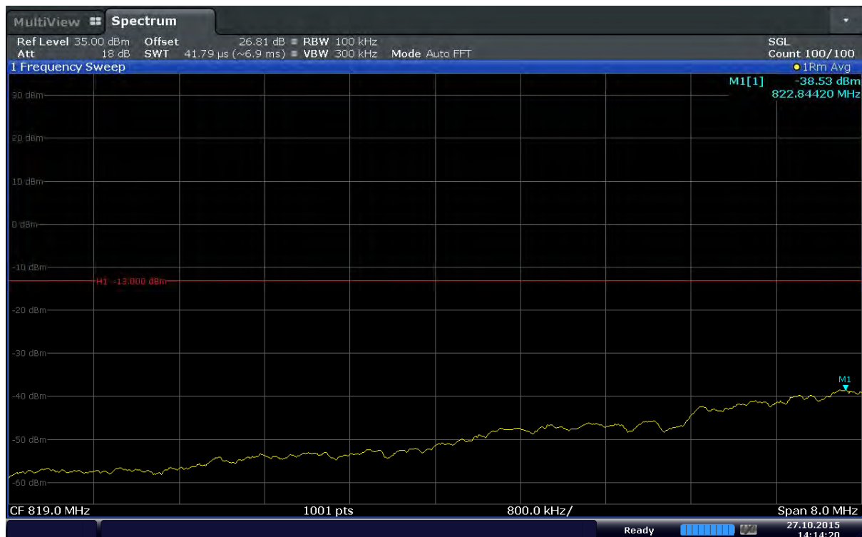
Plot 6-132. Extended Lower Band Edge Plot (Band 5 – 3.0MHz – QPSK – RB Size 15)
