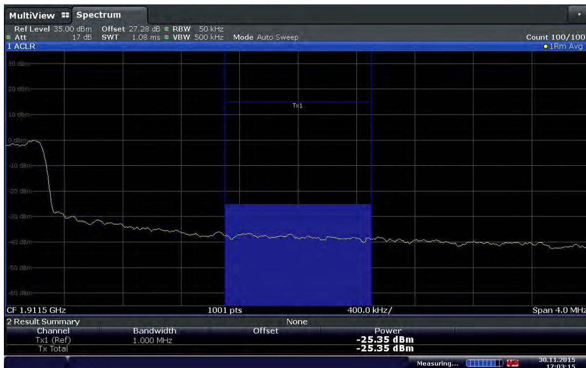
Plot 6-110. Extended Upper Band Edge Plot (Band2 – 5.0MHz – QPSK – RB Size 25)
