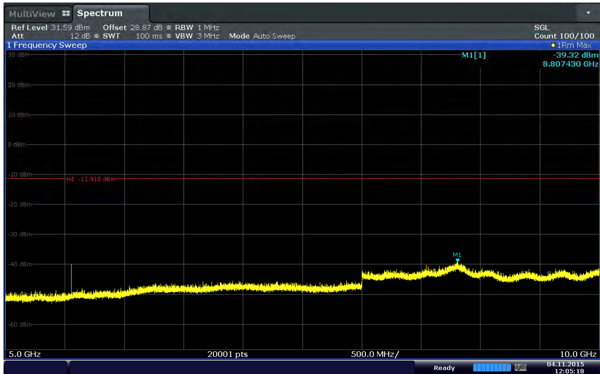
Plot 6-67. Conducted Spurious Plot (Band 2–20.0MHz–QPSK–RB Size 1–RB Offset 0–Ch.18700)
