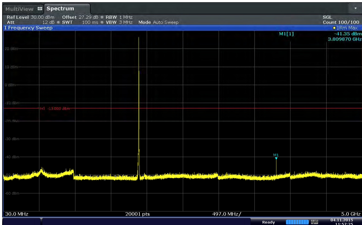
Plot 6-54. Conducted Spurious Plot (Band 2–10.0MHz–QPSK–RB Size 1–RB Offset 24–Ch.19150)
