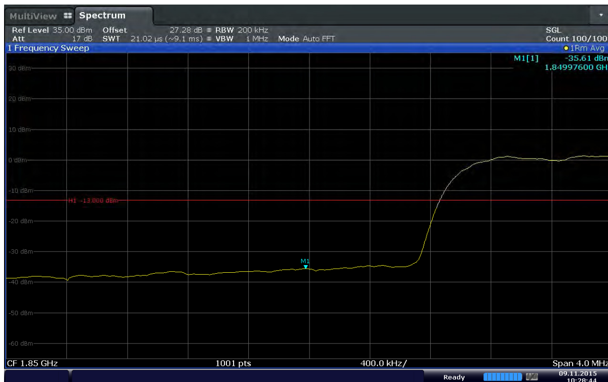
Plot 6-119. Lower Band Edge Plot (Band2 – 20.0MHz – QPSK – RB Size 100)
