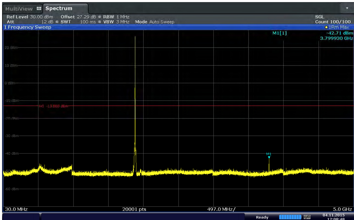
Plot 6-72. Conducted Spurious Plot (Band 2–20.0MHz–QPSK–RB Size 1–RB Offset 49–Ch.19100)
