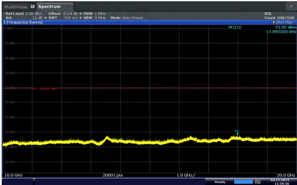
Plot 6-59. Conducted Spurious Plot (Band 2–15.0MHz–QPSK–RB Size 1–RB Offset 0–Ch.18675)
