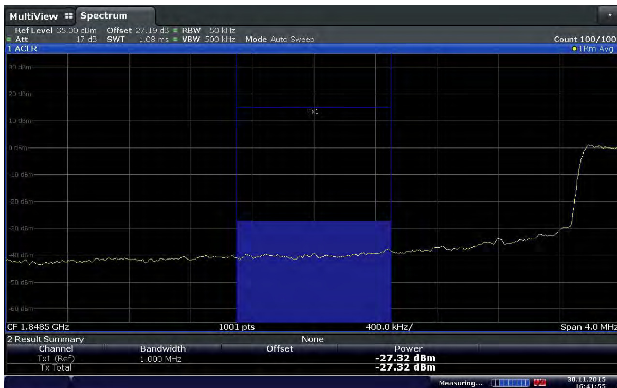
Plot 6-108. Extended Lower Band Edge Plot (Band2 – 5.0MHz – QPSK – RB Size 25)
