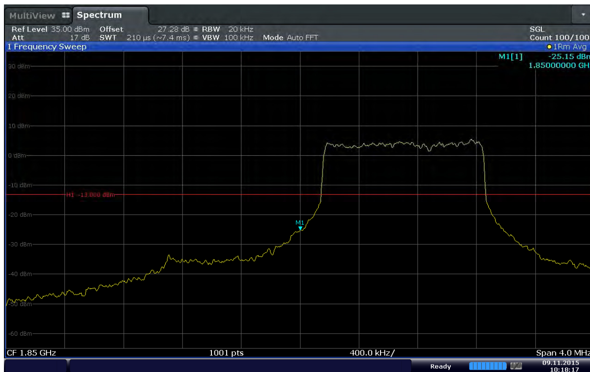
Plot 6-99. Lower Band Edge Plot (Band2 – 1.4MHz – QPSK – RB Size 6)
