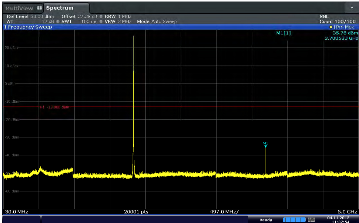
Plot 6-21. Conducted Spurious Plot (Band 2-1.4MHz-QPSK-RB Size 1-RB Offset 0-Ch.18607)
