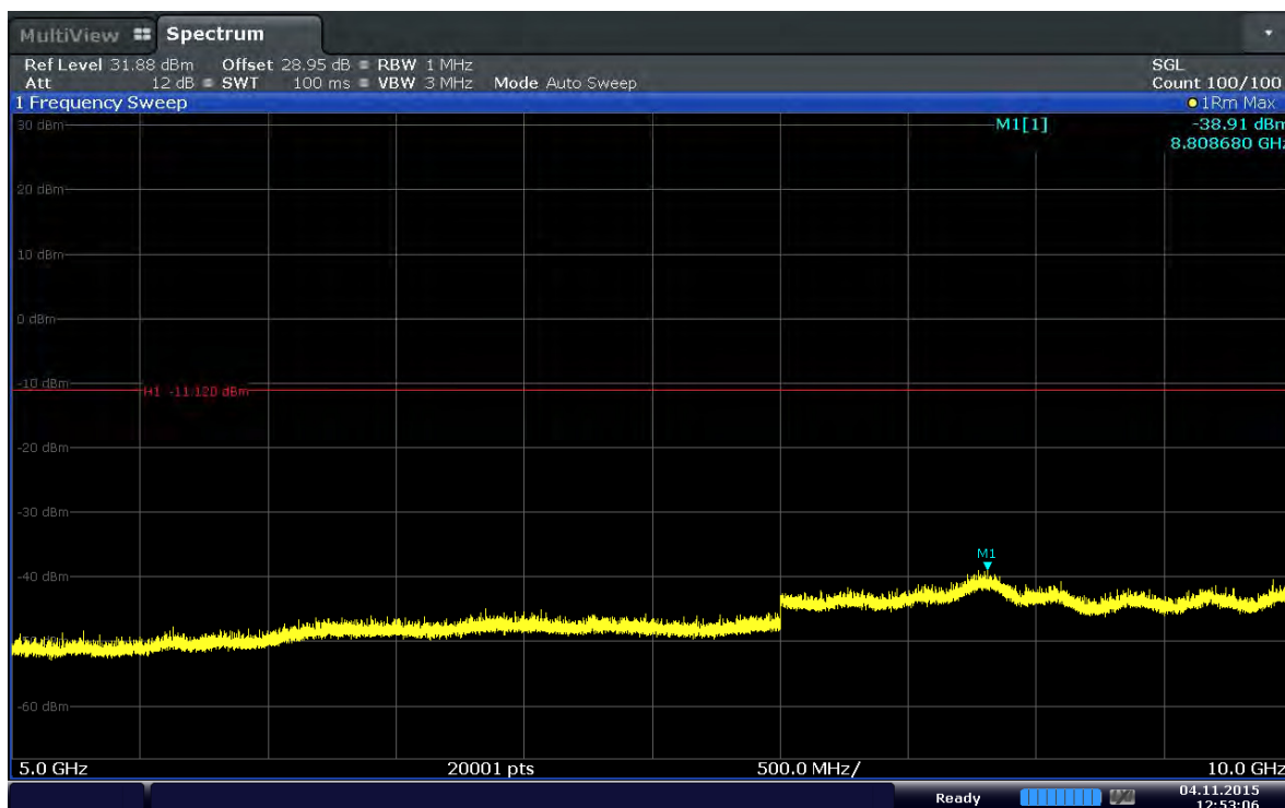
Plot 6-98. Conducted Spurious Plot (Band 5–10.0MHz–QPSK–RB Size 1–RB Offset 0–Ch.20600)
