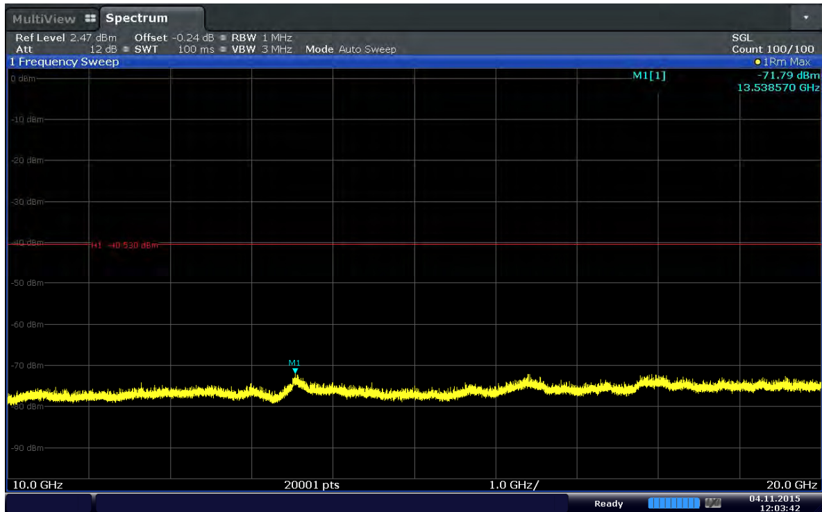
Plot 6-65. Conducted Spurious Plot (Band 2–15.0MHz–QPSK–RB Size 1–RB Offset 37–Ch.19125)
