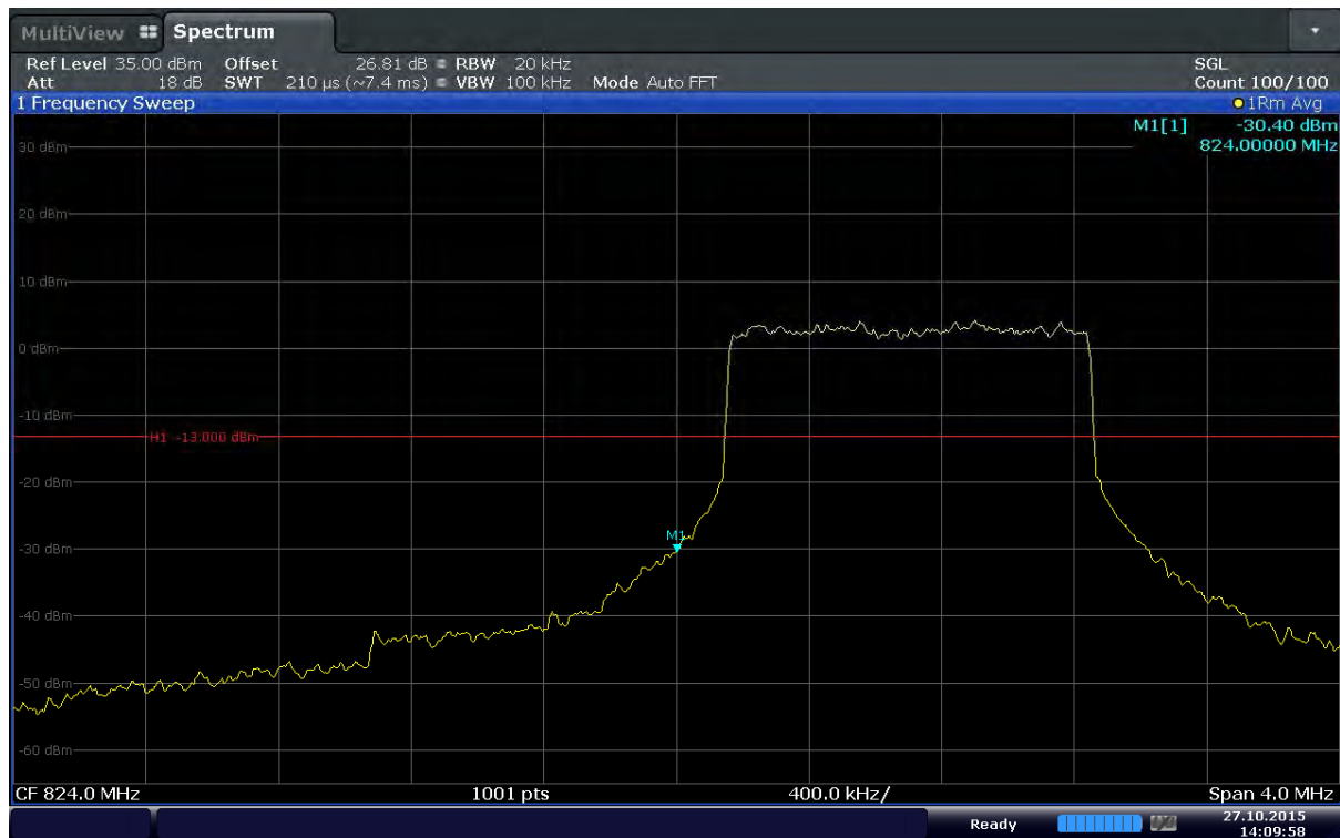
Plot 6-127. Lower Band Edge Plot (Band 5 – 1.4MHz – QPSK – RB Size 6)
