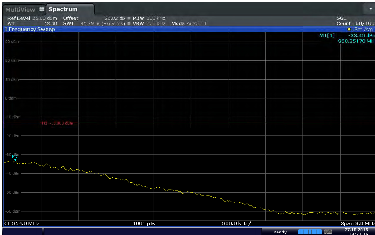
Plot 6-138. Extended Upper Band Edge Plot (Band 5 – 5.0MHz – QPSK – RB Size 25)
