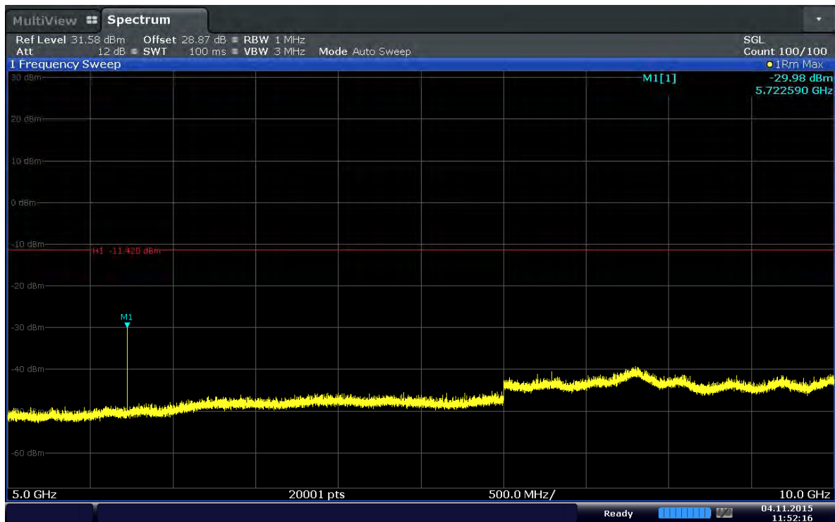
Plot 6-46. Conducted Spurious Plot (Band 2–5.0MHz–QPSK–RB Size 1–RB Offset 12–Ch.19175)
