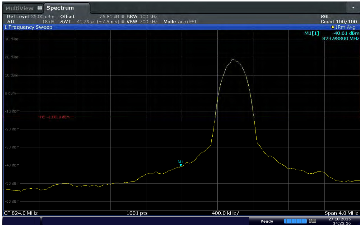
Plot 6-141. Lower Band Edge Plot (Band 5 – 10.0MHz – QPSK – RB Size 1 – RB Offset 0)
