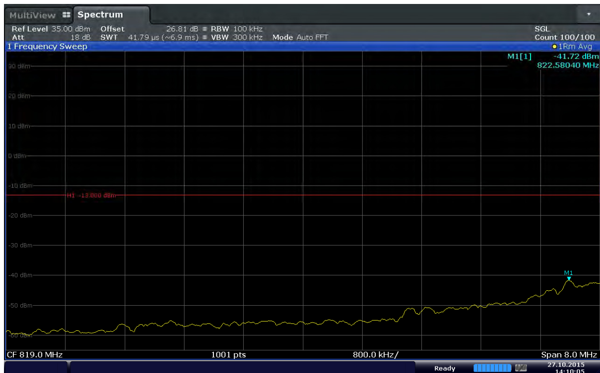
Plot 6-128. Extended Lower Band Edge Plot (Band 5 – 1.4MHz – QPSK – RB Size 6)
