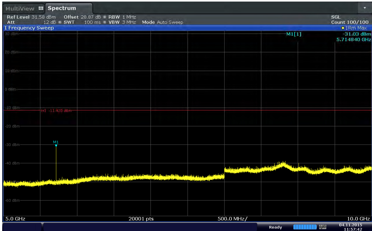
Plot 6-55. Conducted Spurious Plot (Band 2–10.0MHz–QPSK–RB Size 1–RB Offset 24–Ch.19150)
