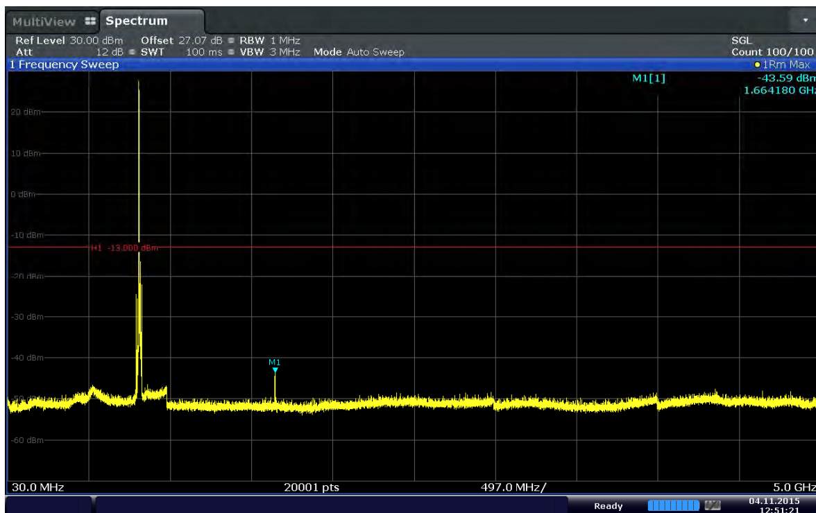
Plot 6-95. Conducted Spurious Plot (Band 5–10.0MHz–QPSK–RB Size 1–RB Offset 0–Ch.20525)
