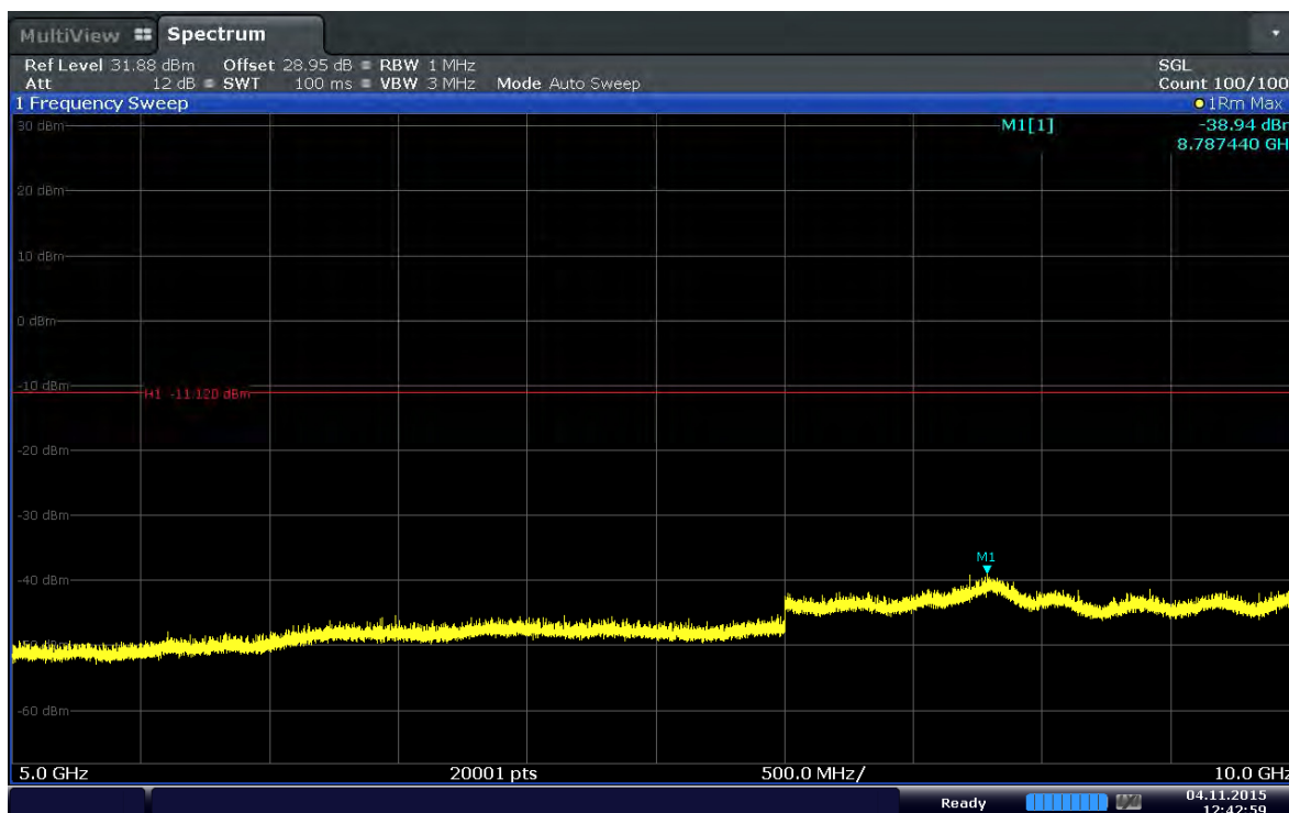
Plot 6-84. Conducted Spurious Plot (Band 5–3.0MHz–QPSK–RB Size 1–RB Offset 14–Ch.20525)
