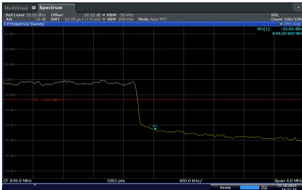
Plot 6-137. Upper Band Edge Plot (Band 5 – 5.0MHz – QPSK – RB Size 25)
