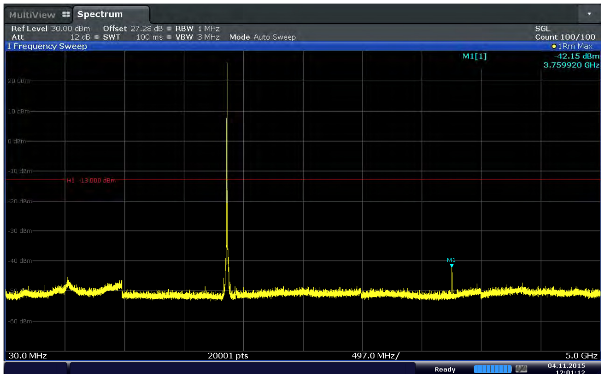
Plot 6-60. Conducted Spurious Plot (Band 2–15.0MHz–QPSK–RB Size 1–RB Offset 37–Ch.18900)
