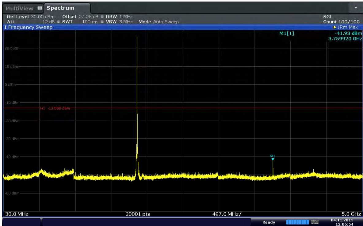
Plot 6-69. Conducted Spurious Plot (Band 2–20.0MHz–QPSK–RB Size 1–RB Offset 49–Ch.18900)
