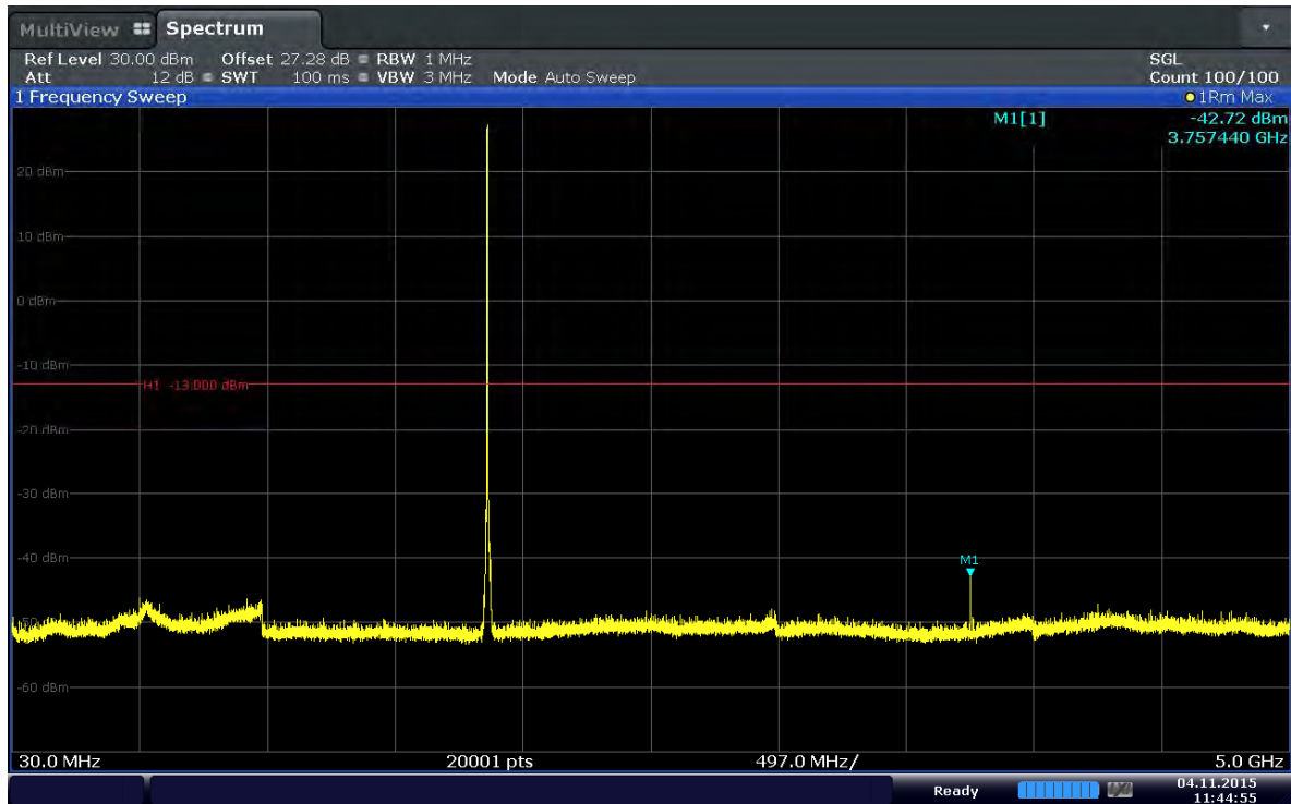
Plot 6-33. Conducted Spurious Plot (Band 2–3.0MHz–QPSK–RB Size 1–RB Offset 0–Ch.18900)
