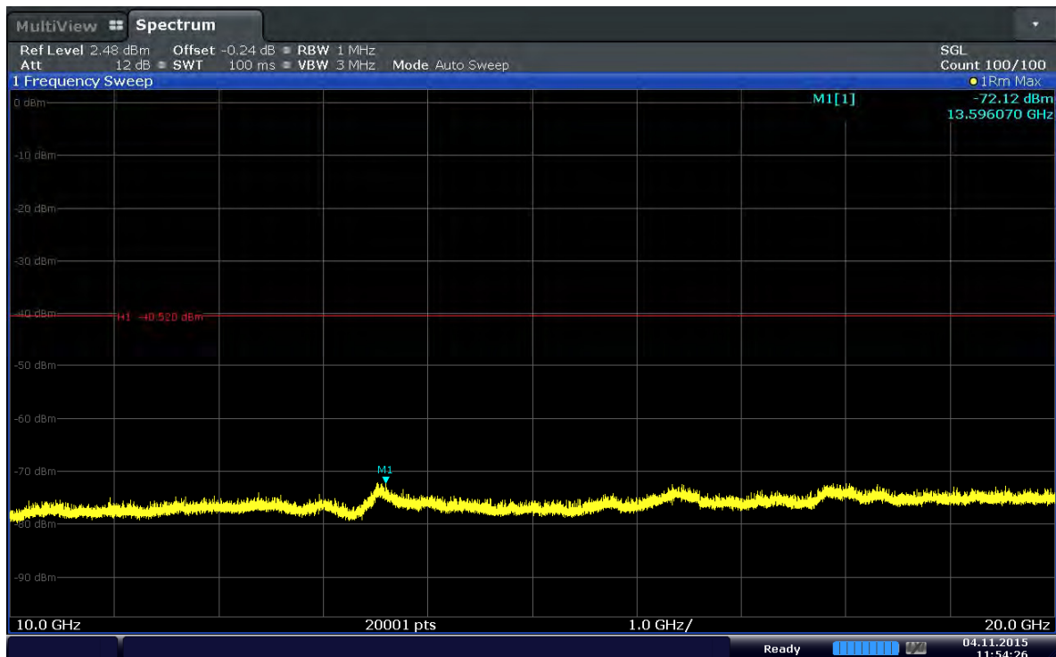
Plot 6-50. Conducted Spurious Plot (Band 2–10.0MHz–QPSK–RB Size 1–RB Offset 24–Ch.18650)
