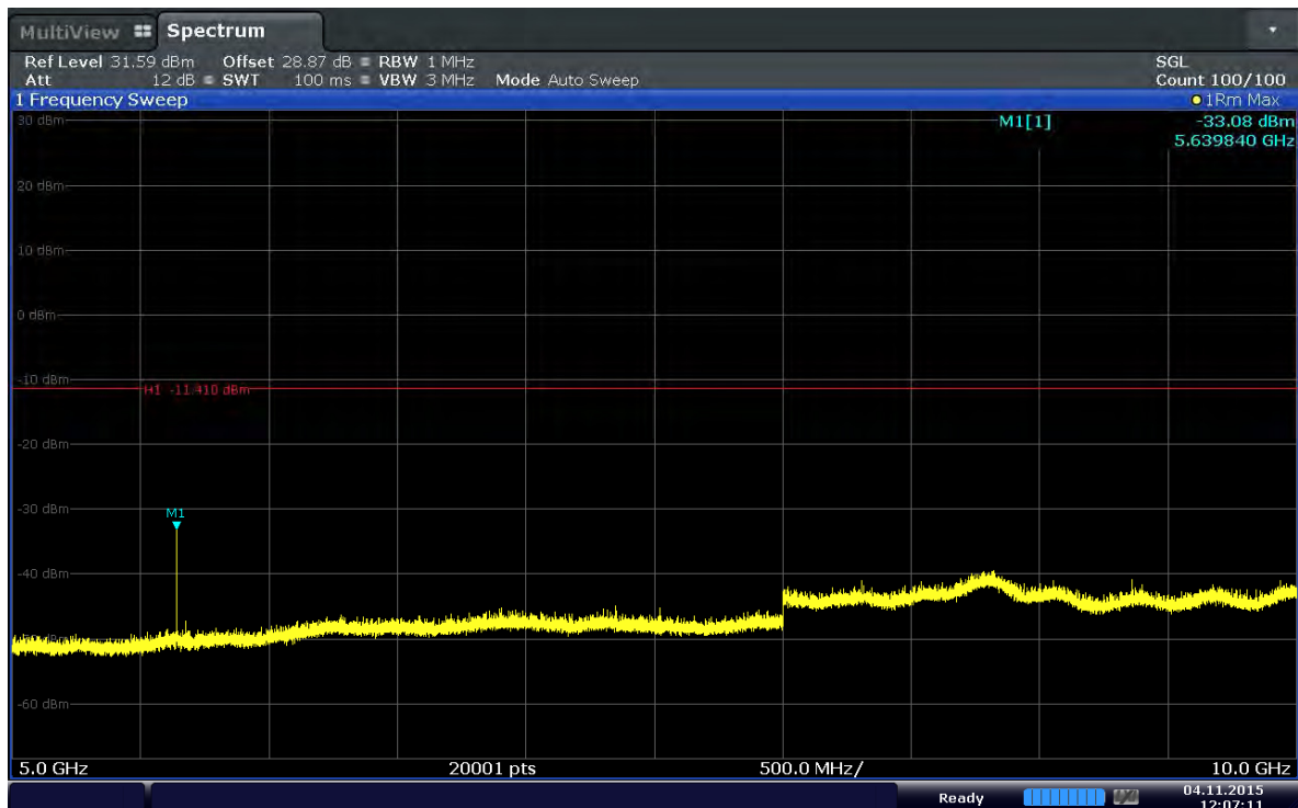
Plot 6-70. Conducted Spurious Plot (Band 2–20.0MHz–QPSK–RB Size 1–RB Offset 49–Ch.18900)
