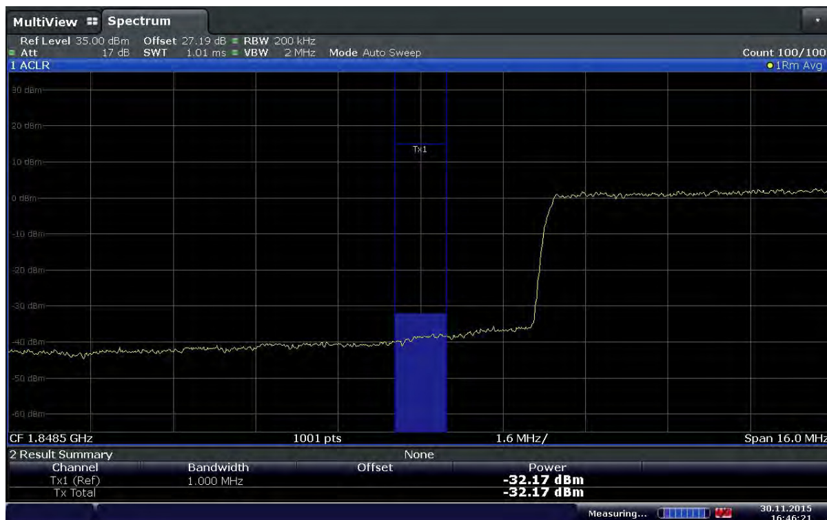
Plot 6-120. Extended Lower Band Edge Plot (Band2 – 20.0MHz – QPSK – RB Size 100)
