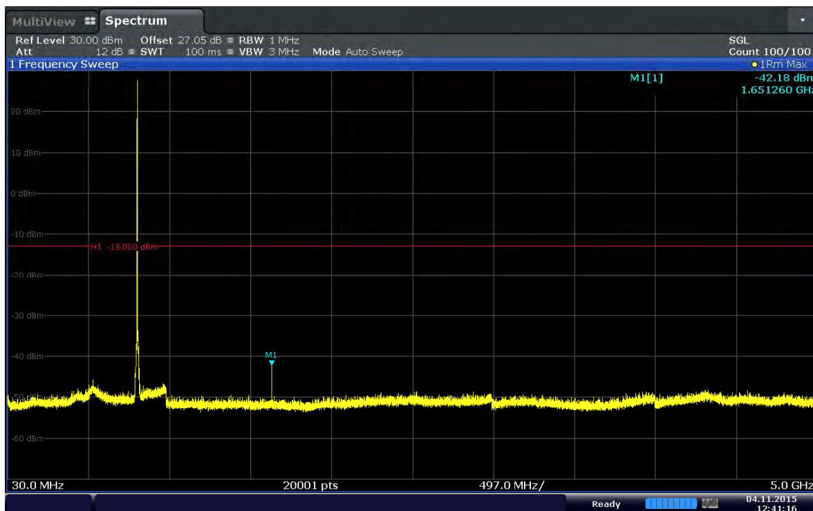
Plot 6-81. Conducted Spurious Plot (Band 5–3.0MHz–QPSK–RB Size 1–RB Offset 7–Ch.20415)
