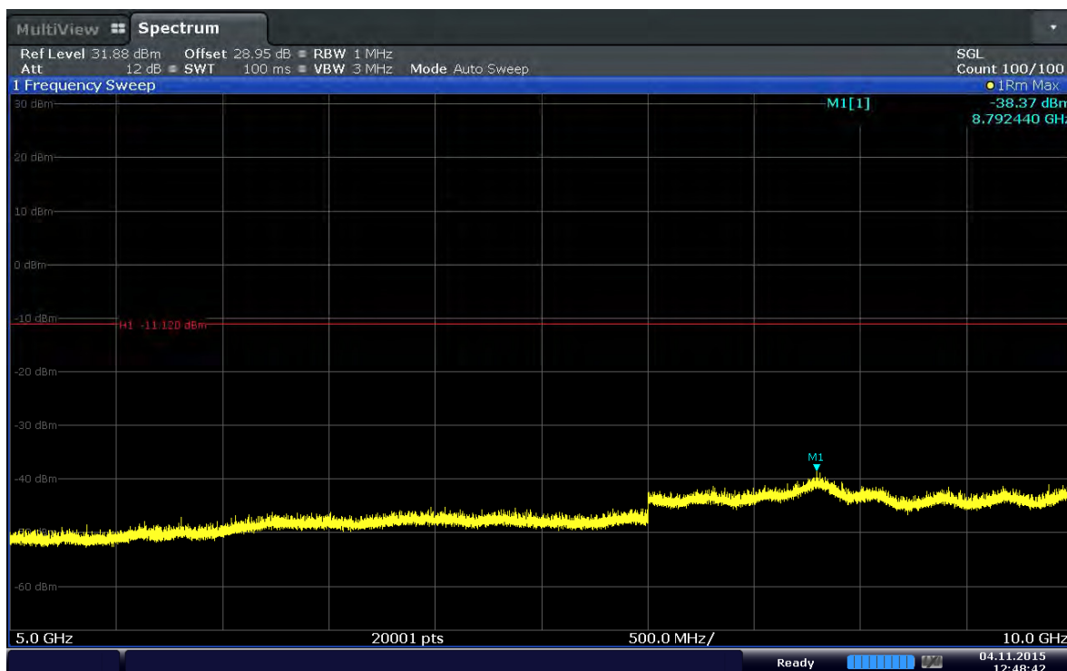
Plot 6-92. Conducted Spurious Plot (Band 5–5.0MHz–QPSK–RB Size 1–RB Offset 24–Ch.20625)
