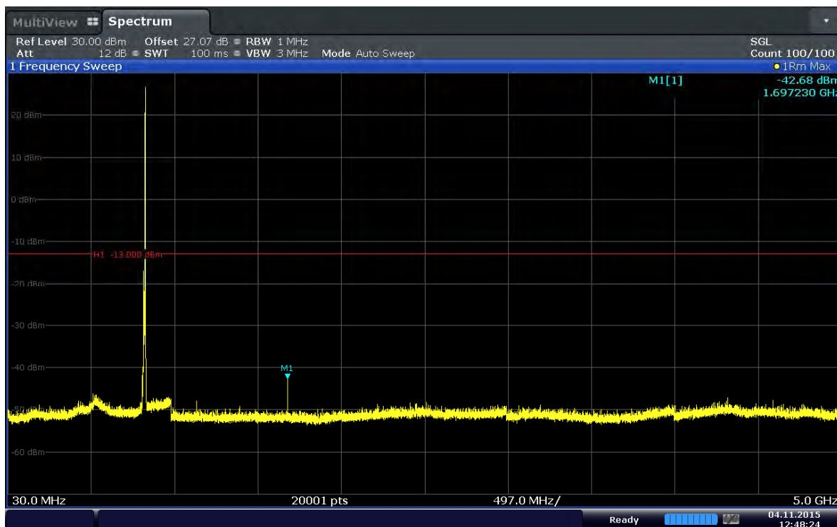
Plot 6-91. Conducted Spurious Plot (Band 5–5.0MHz–QPSK–RB Size 1–RB Offset 24–Ch.20625)
