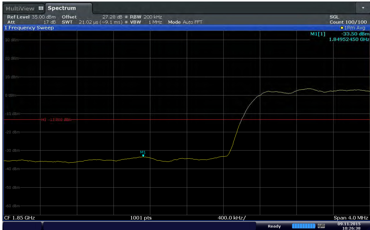
Plot 6-115. Lower Band Edge Plot (Band2 – 15.0MHz – QPSK – RB Size 75)
