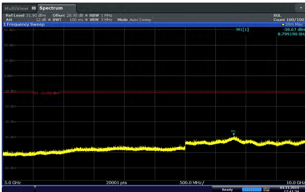
Plot 6-82. Conducted Spurious Plot (Band 5–3.0MHz–QPSK–RB Size 1–RB Offset 7–Ch.20415)
