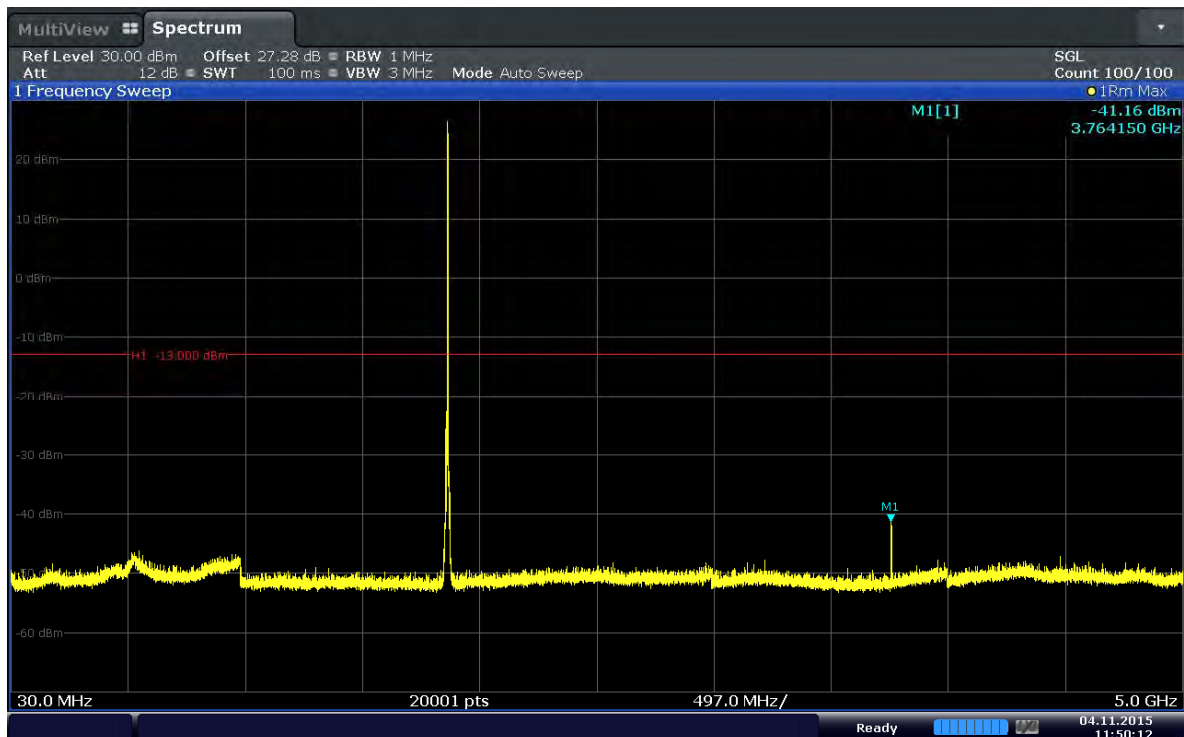
Plot 6-42. Conducted Spurious Plot (Band 2–5.0MHz–QPSK–RB Size 1–RB Offset 24–Ch.18900)
