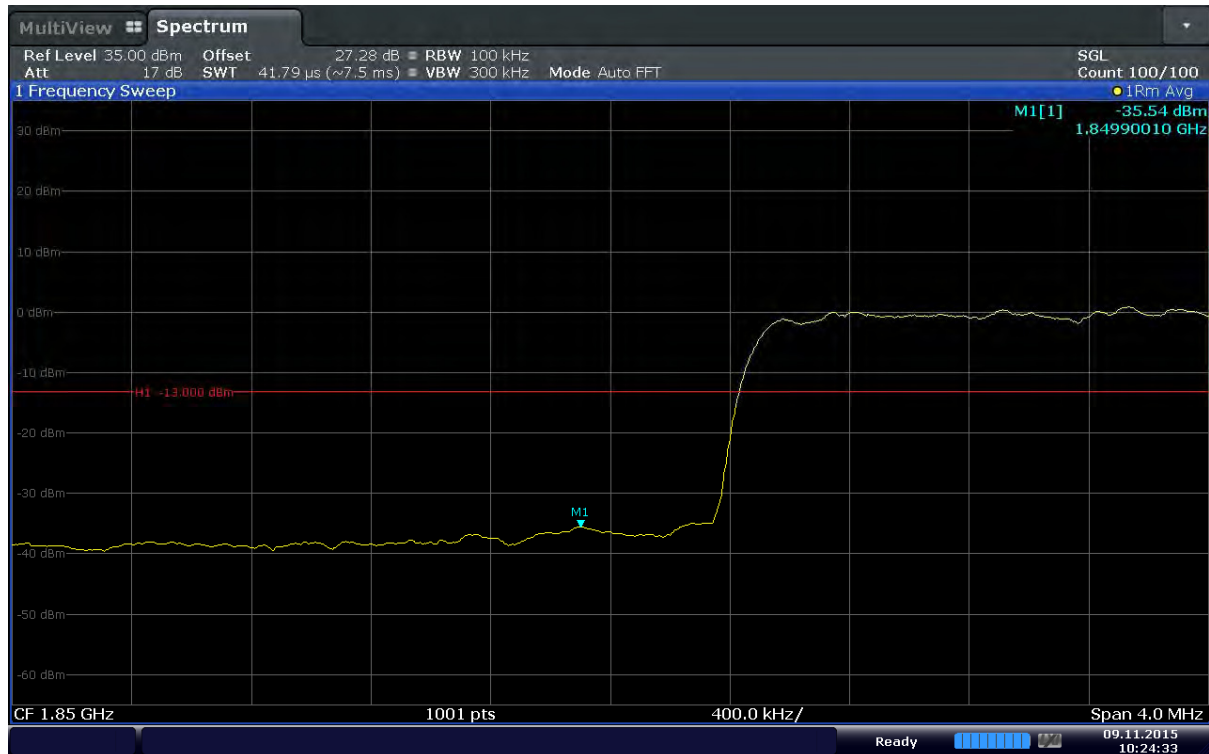
Plot 6-111. Lower Band Edge Plot (Band2 – 10.0MHz – QPSK – RB Size 50)
