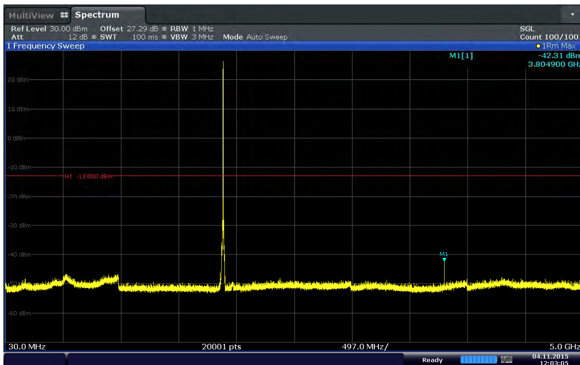
Plot 6-63. Conducted Spurious Plot (Band 2–15.0MHz–QPSK–RB Size 1–RB Offset 37–Ch.19125)
