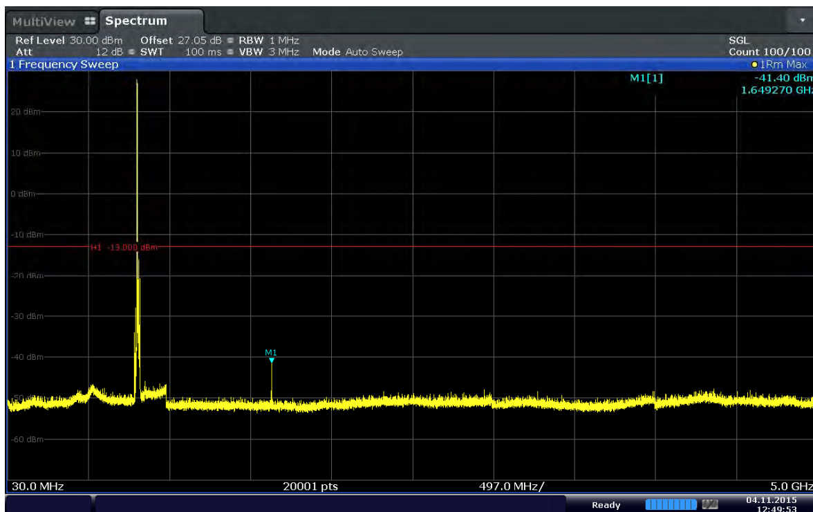
Plot 6-93. Conducted Spurious Plot (Band 5–10.0MHz–QPSK–RB Size 1–RB Offset 0–Ch.20450)
