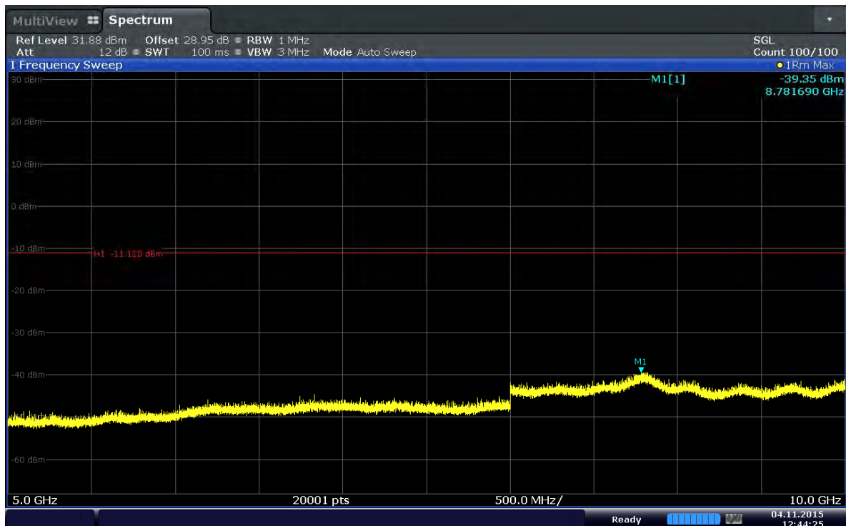
Plot 6-86. Conducted Spurious Plot (Band 5–3.0MHz–QPSK–RB Size 1–RB Offset 7–Ch.20635)
