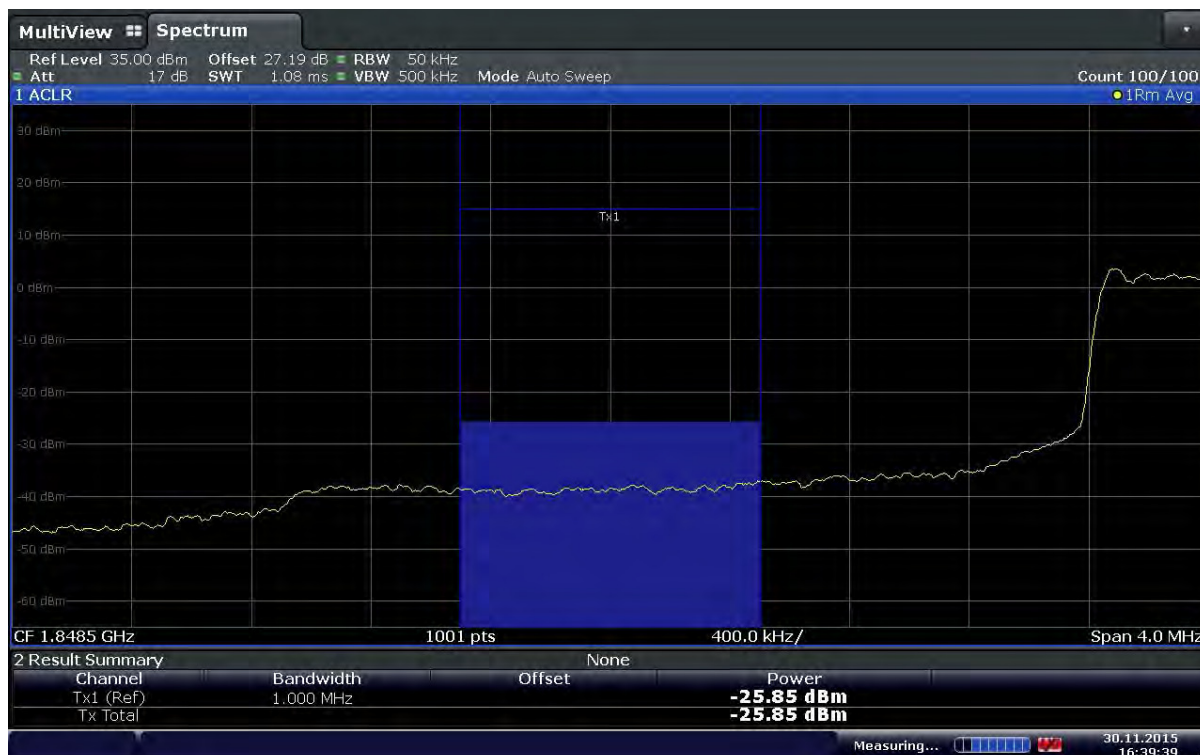
Plot 6-104. Extended Lower Band Edge Plot (Band2 – 3.0MHz – QPSK – RB Size 15)
