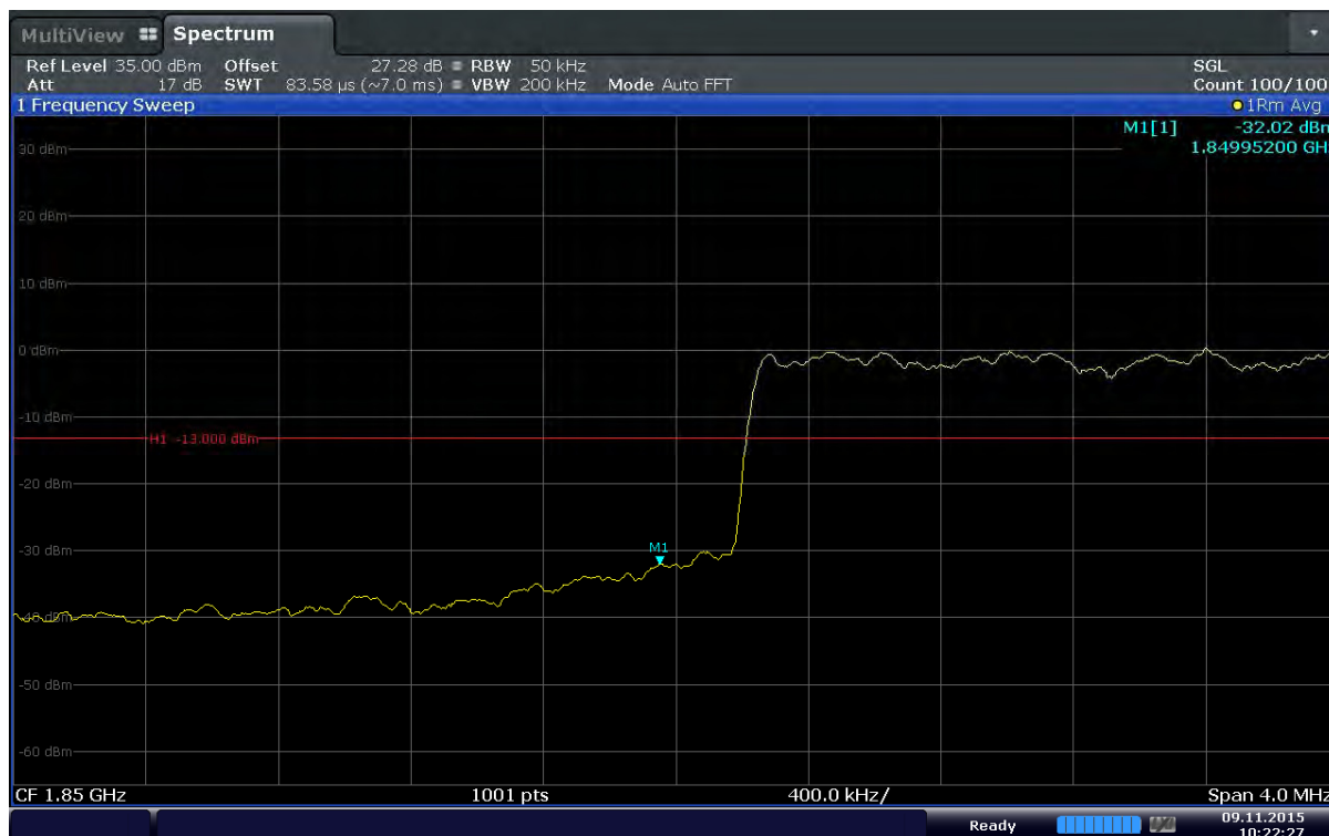
Plot 6-107. Lower Band Edge Plot (Band2 – 5.0MHz – QPSK – RB Size 25)
