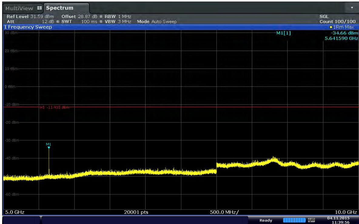
Plot 6-25. Conducted Spurious Plot (Band 2–1.4MHz–QPSK–RB Size 1–RB Offset 5–Ch.18900)
