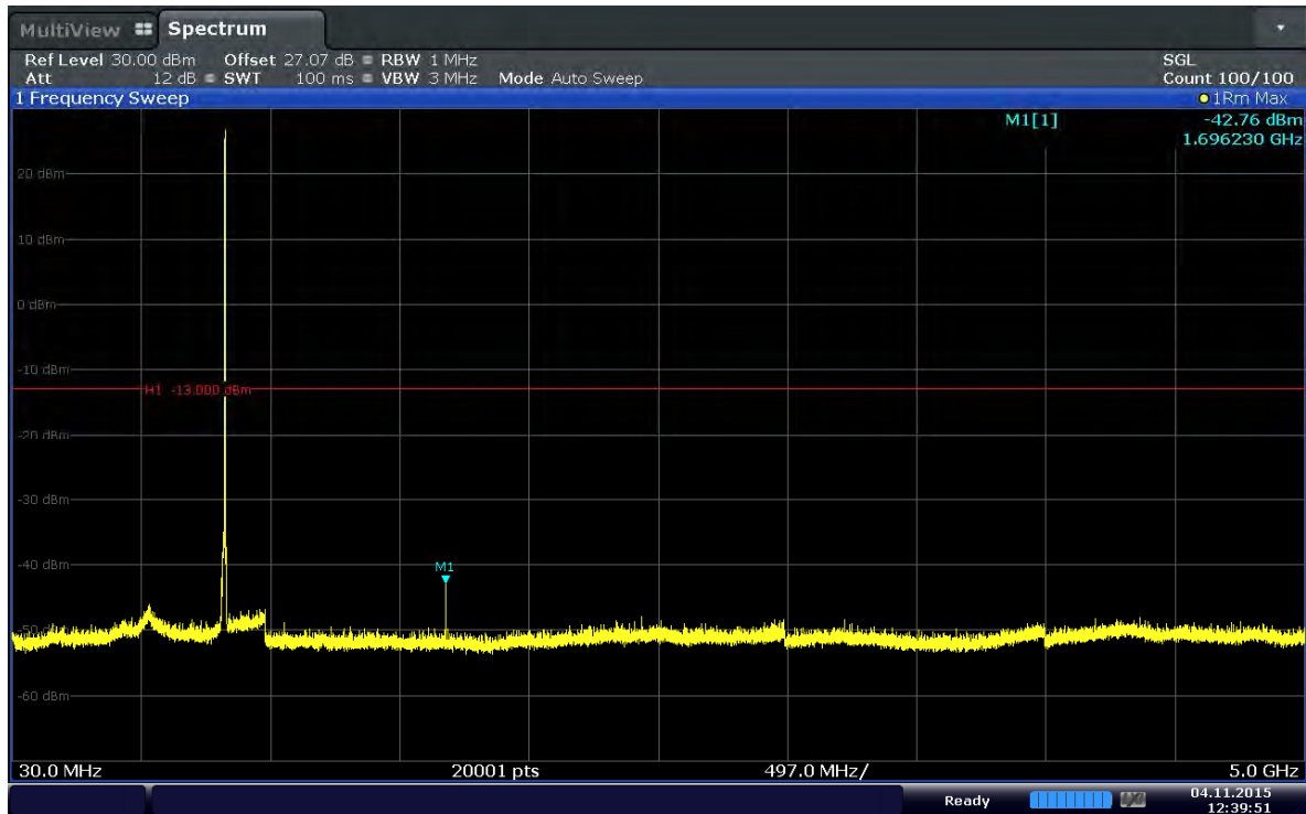
Plot 6-79. Conducted Spurious Plot (Band 5–1.4MHz–QPSK–RB Size 1–RB Offset 2–Ch.20643)
