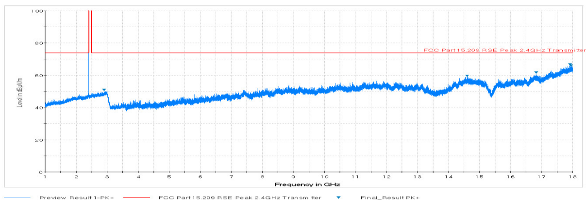
Plot 6-43. Radiated Spurious Plot above 1GHz (BT – Ch. 0, Ant. Pol. V)
