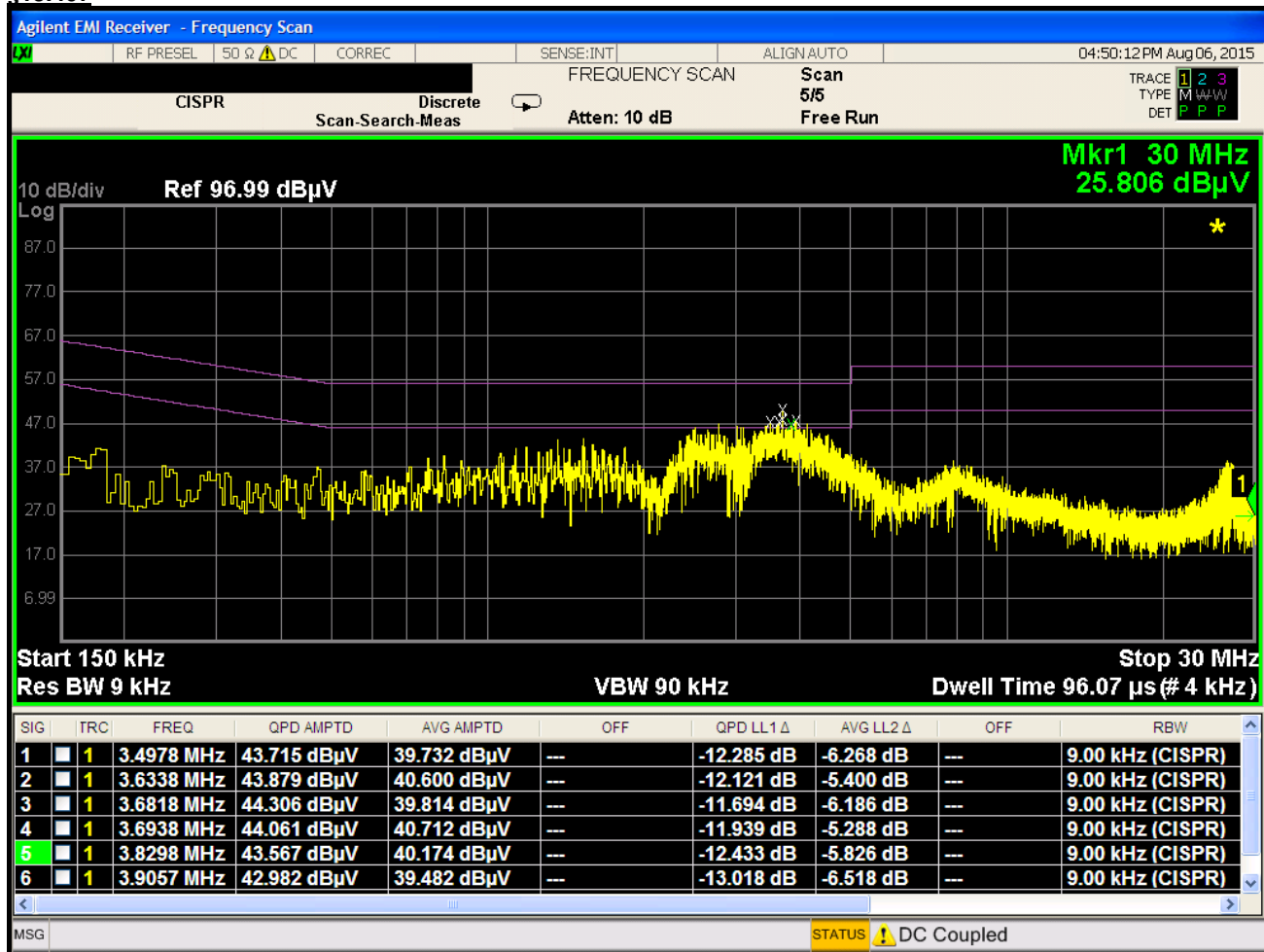
Plot 6-97. Line Conducted Plot with 802.11a UNII Band 2C (L1)
