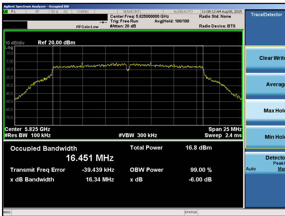
Plot 6-28. 6dB Bandwidth Plot (802.11a (UNII Band 3) – Ch. 165)
