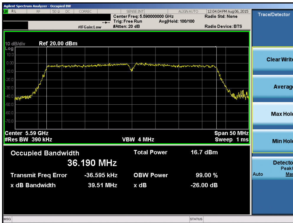
Plot 6-24. 26dB Bandwidth Plot (40MHz BW 802.11n (UNII Band 2C) – Ch. 118)
