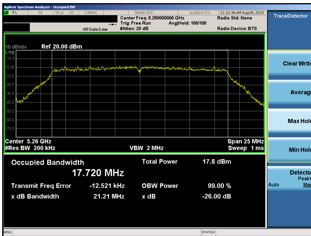
Plot 6-12. 26dB Bandwidth Plot (20MHz BW 802.11n (UNII Band 2A) – Ch. 52)
