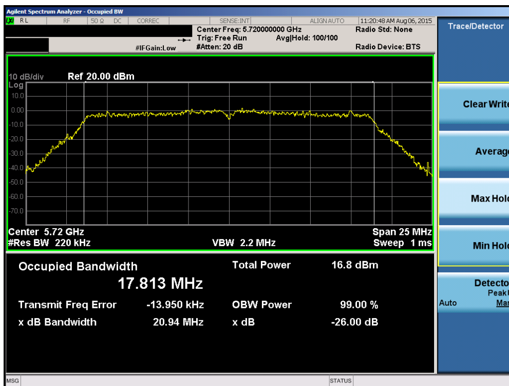
Plot 6-22. 26dB Bandwidth Plot (20MHz BW 802.11n (UNII Band 2C) – Ch. 144)
