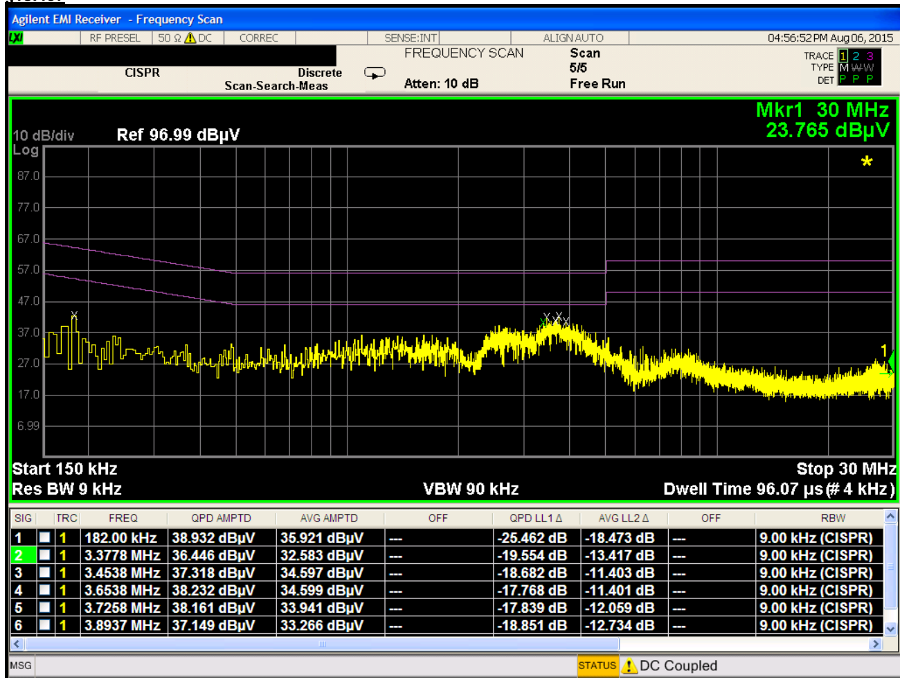
Plot 6-100. Line Conducted Plot with 802.11a UNII Band 3 (N)
