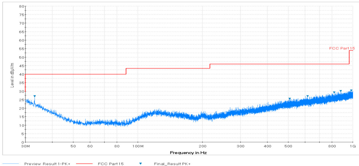
Plot 6-91. Radiated Spurious Plot below 1GHz (802.11a – U3 Ch. 157, Ant. Pol. H)
