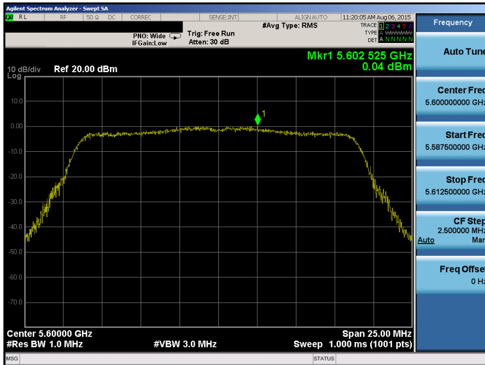
Plot 6-54. Power Spectral Density Plot (20MHz BW 802.11n (UNII Band 2C) – Ch. 120)
