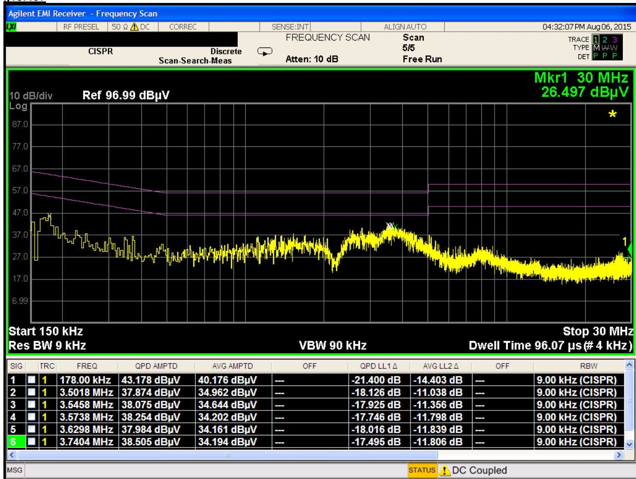
Plot 6-94. Line Conducted Plot with 802.11a UNII Band 1 (N)
