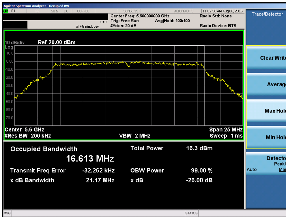
Plot 6-18. 26dB Bandwidth Plot (802.11a (UNII Band 2C) – Ch. 120)
