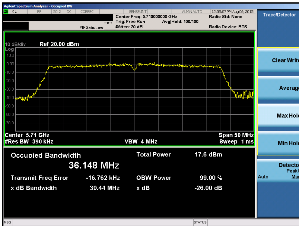
Plot 6-25. 26dB Bandwidth Plot (40MHz BW 802.11n (UNII Band 2C) – Ch. 142)
