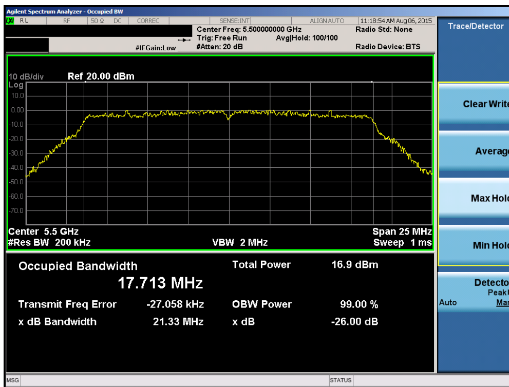
Plot 6-20. 26dB Bandwidth Plot (20MHz BW 802.11n (UNII Band 2C) – Ch. 100)
