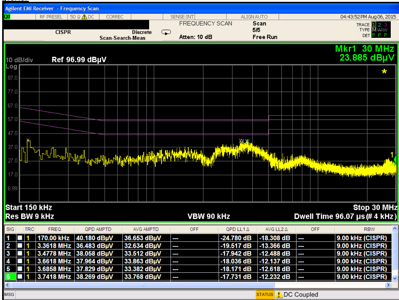
Plot 6-96. Line Conducted Plot with 802.11a UNII Band 2A (N)
