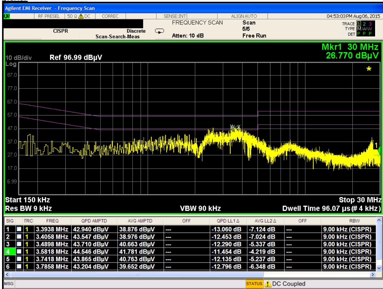
Plot 6-99. Line Conducted Plot with 802.11a UNII Band 3 (L1)
