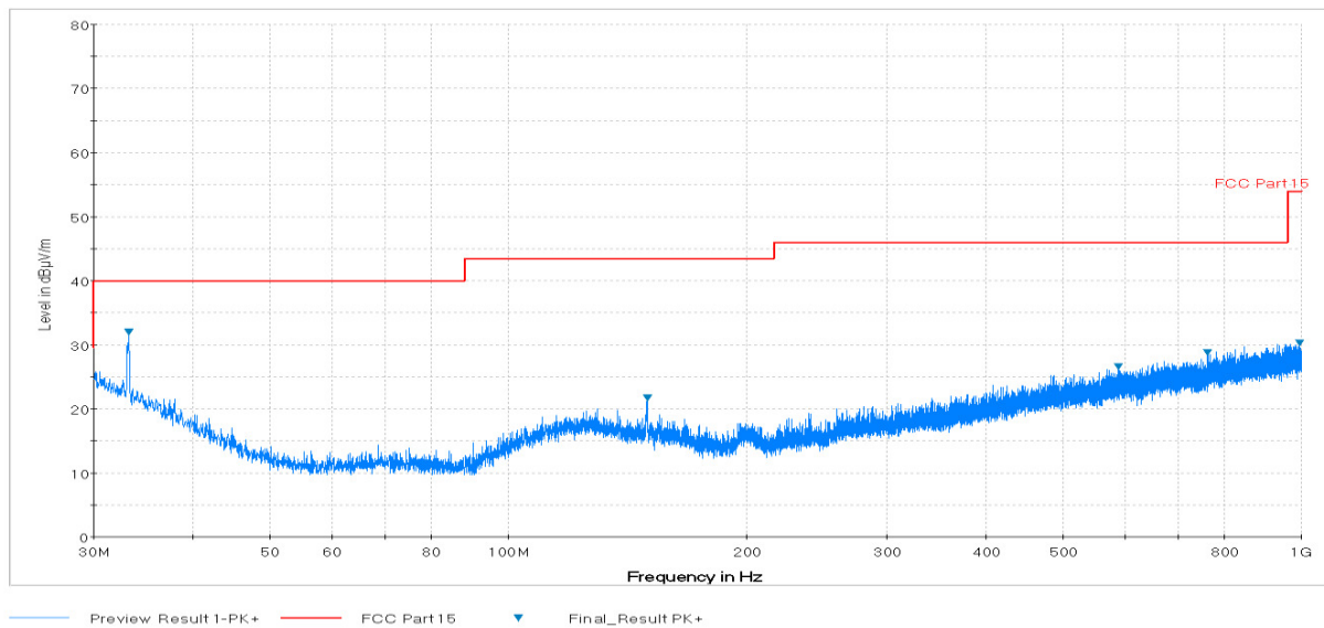
Plot 6-92. Radiated Spurious Plot below 1GHz (802.11a – U3 Ch. 157, Ant. Pol. V)
