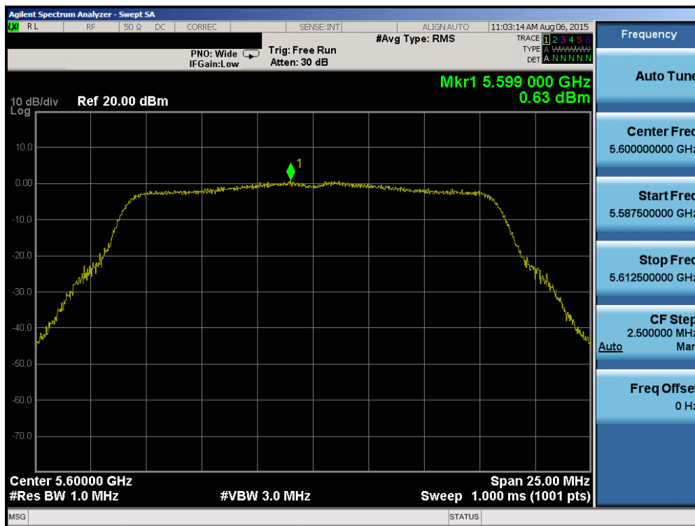
Plot 6-51. Power Spectral Density Plot (802.11a (UNII Band 2C) – Ch. 120)
