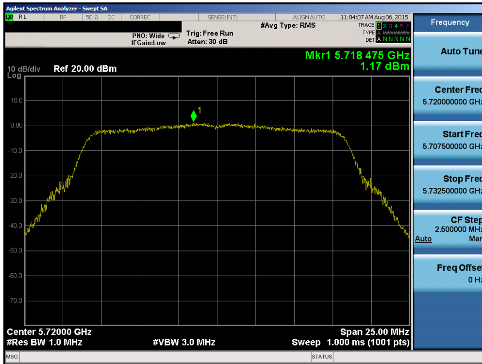
Plot 6-52. Power Spectral Density Plot (802.11a (UNII Band 2C) – Ch. 144)
