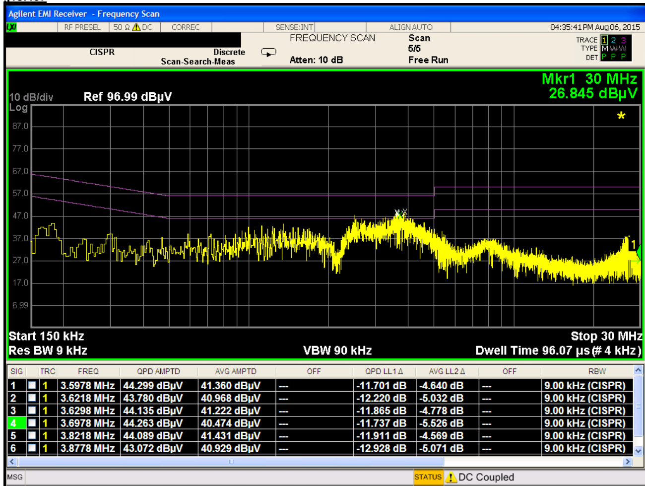
Plot 6-93. Line Conducted Plot with 802.11a UNII Band 1 (L1)
