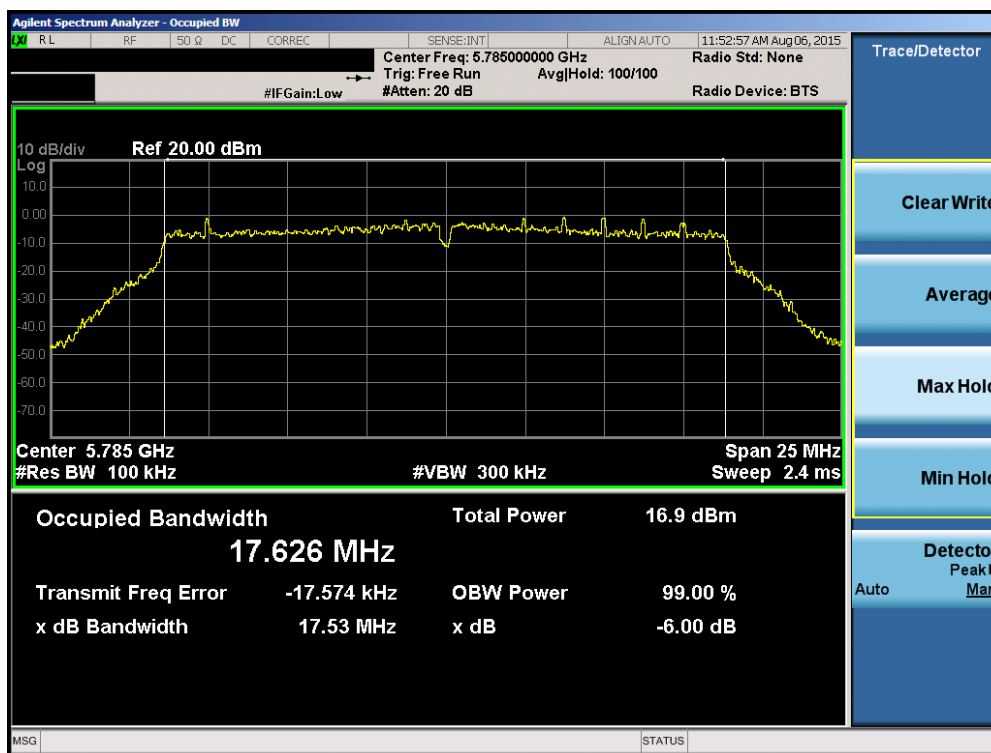
Plot 6-30. 6dB Bandwidth Plot (20MHz BW 802.11n (UNII Band 3) – Ch. 157)
