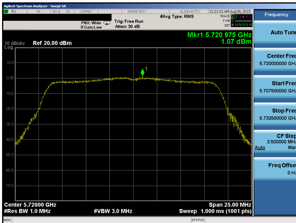
Plot 6-55. Power Spectral Density Plot (20MHz BW 802.11n (UNII Band 2C) – Ch. 144)
