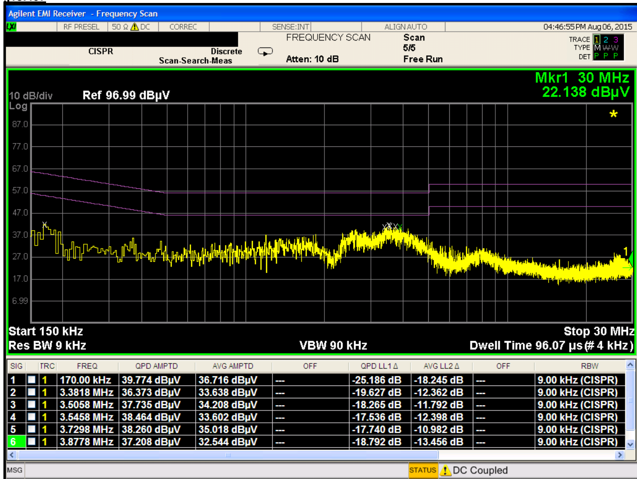
Plot 6-98. Line Conducted Plot with 802.11a UNII Band 2C (N)
