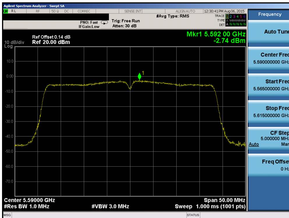
Plot 6-57. Power Spectral Density Plot (40MHz BW 802.11n (UNII Band 2C) – Ch. 118)
