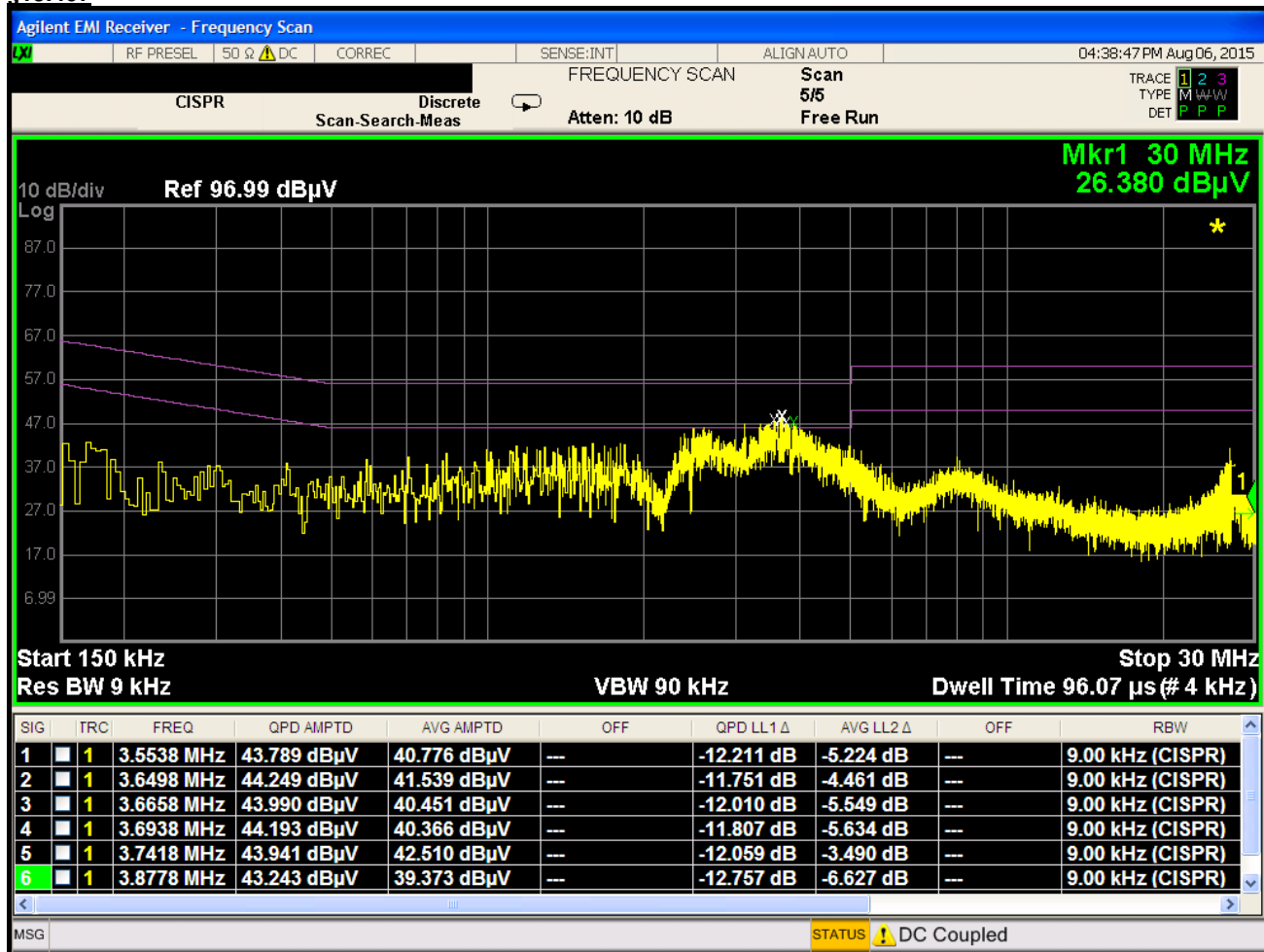
Plot 6-95. Line Conducted Plot with 802.11a UNII Band 2A (L1)
