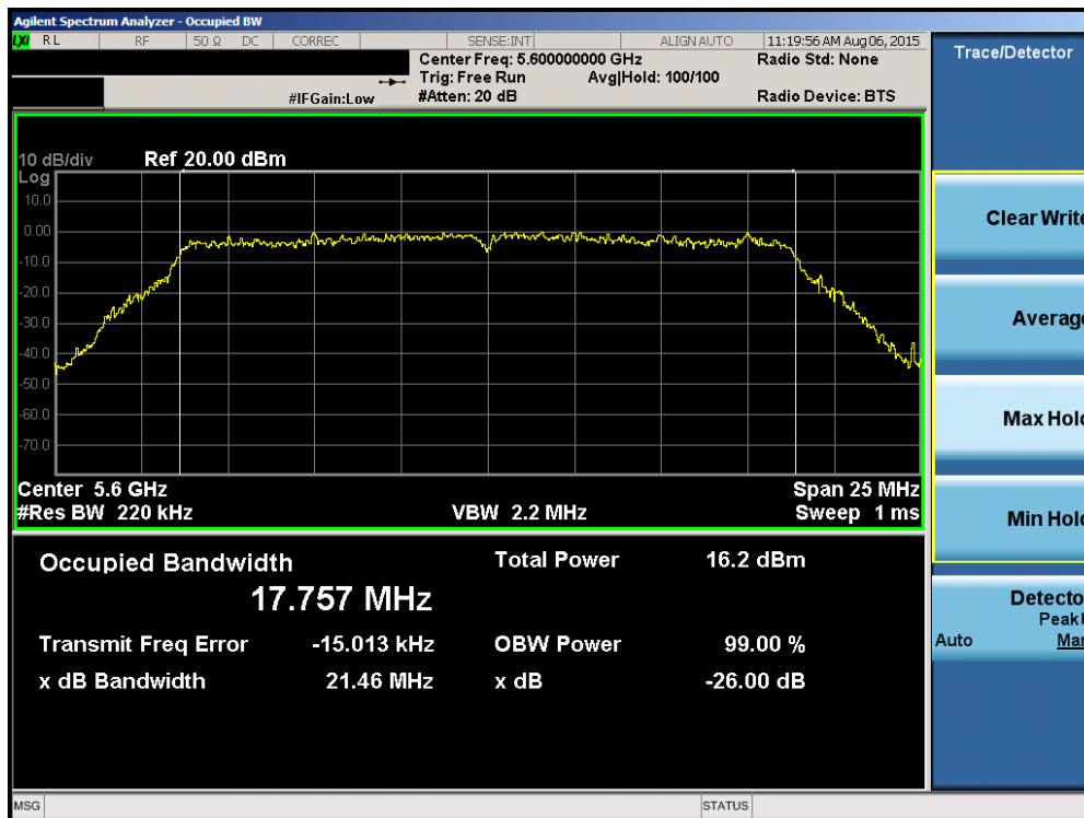
Plot 6-21. 26dB Bandwidth Plot (20MHz BW 802.11n (UNII Band 2C) – Ch. 120)
