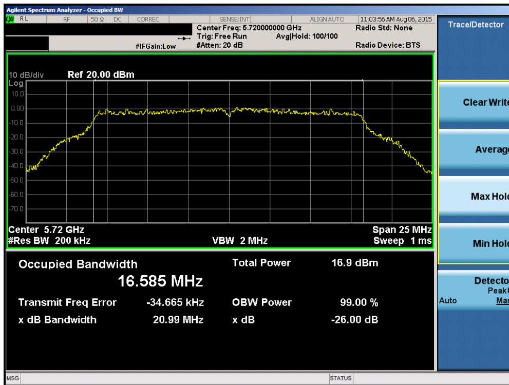
Plot 6-19. 26dB Bandwidth Plot (802.11a (UNII Band 2C) – Ch. 144)
