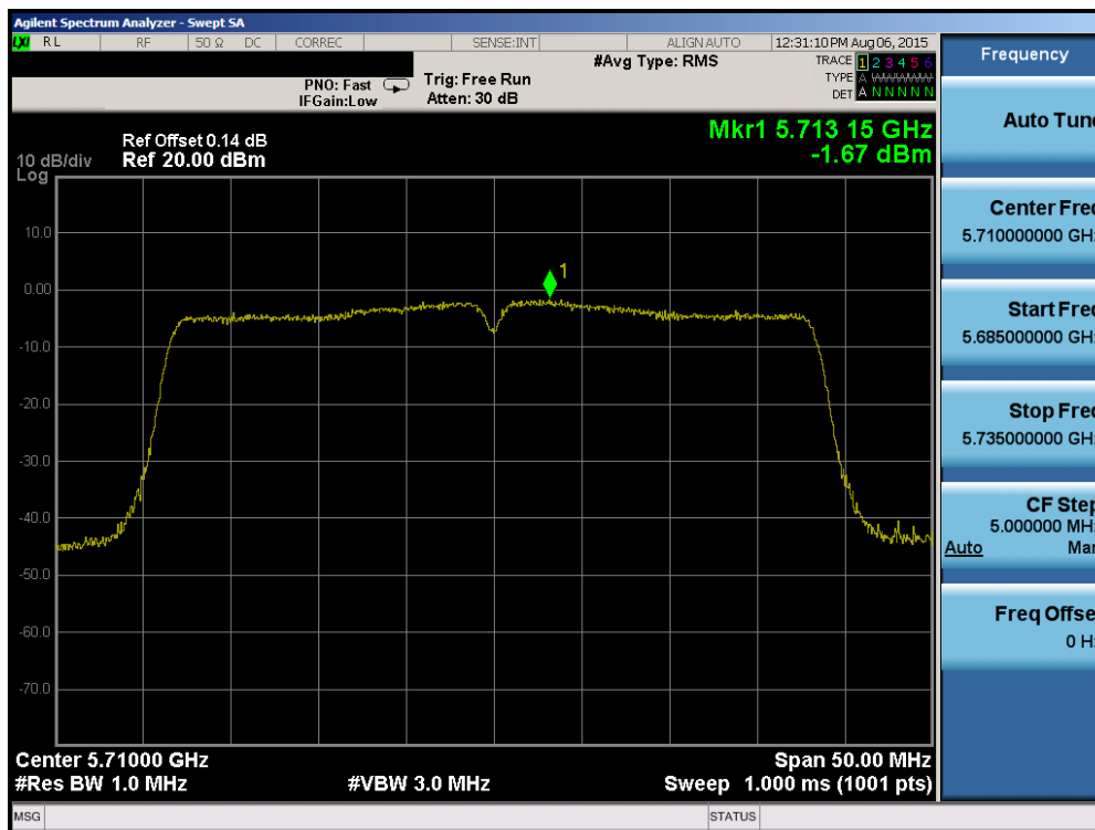
Plot 6-58. Power Spectral Density Plot (40MHz BW 802.11n (UNII Band 2C) – Ch. 142)
