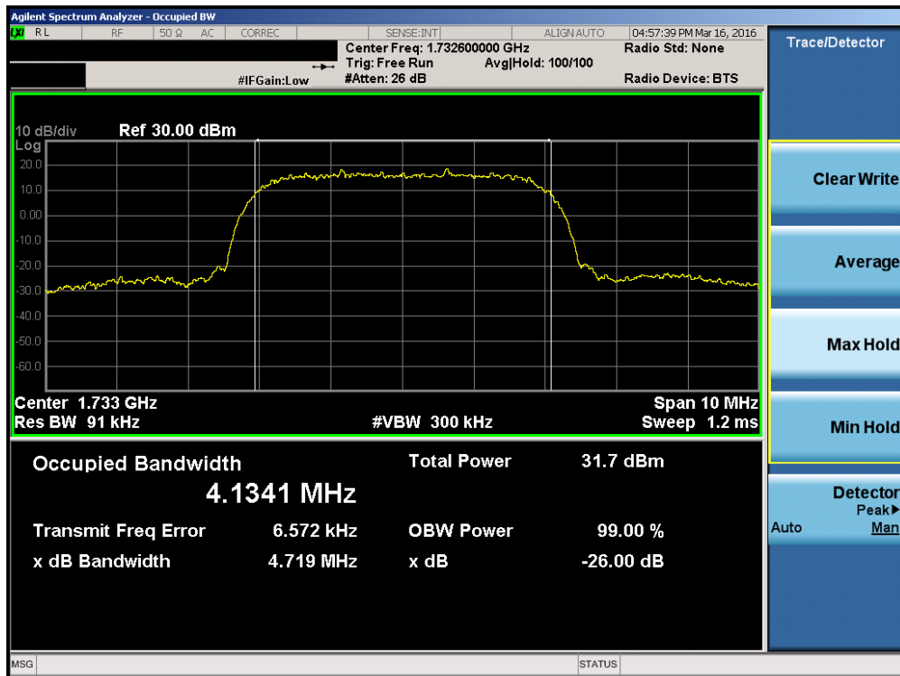
Plot 7-2. Occupied Bandwidth Plot (AWS WCDMA Mode – Ch. 1412)
