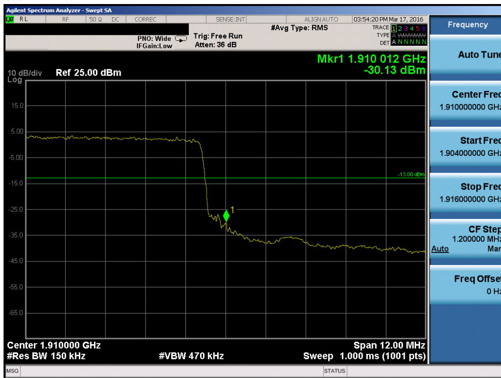
Plot 7-160. Upper Band Edge Plot (Band 2 – 15.0MHz QPSK – RB Size 75)
