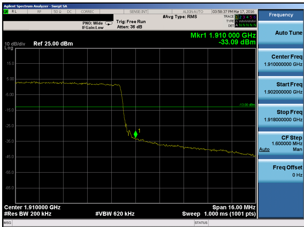
Plot 7-164. Upper Band Edge Plot (Band 2 – 20.0MHz QPSK – RB Size 100)
