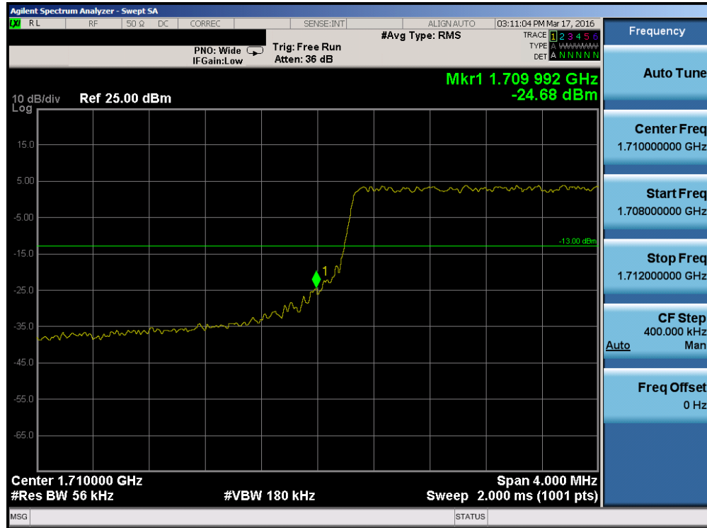
Plot 7-126. Lower Band Edge Plot (Band 4 – 5.0MHz QPSK – RB Size 25)
