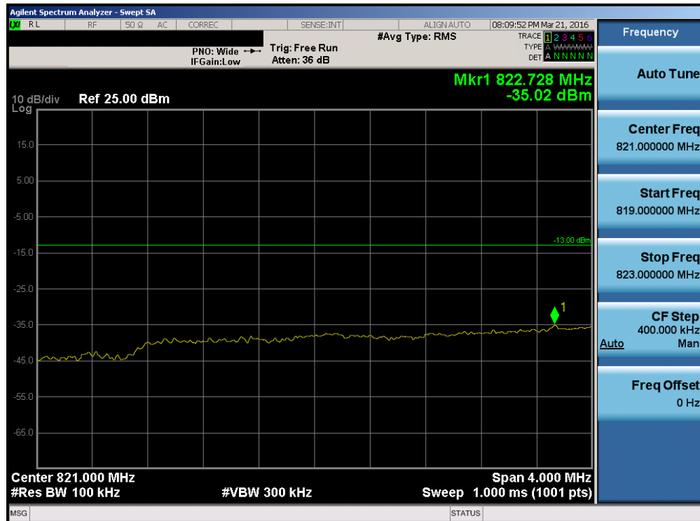
Plot 7-113. Lower Extended Band Edge Plot (Band 5 - 5.0MHz QPSK - RB Size 25)
