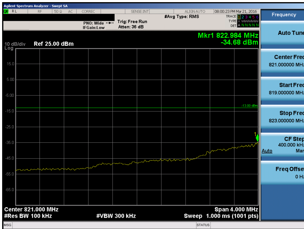
Plot 7-105. Lower Extended Band Edge Plot (Band 5 – 1.4MHz QPSK – RB Size 6)
