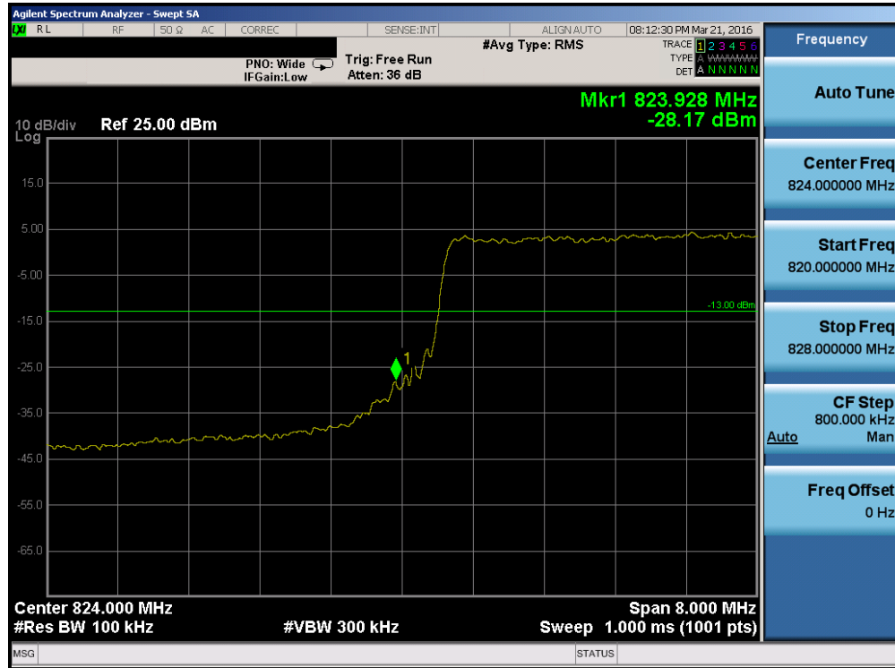
Plot 7-116. Lower Band Edge Plot (Band 5 – 10.0MHz QPSK – RB Size 50)
