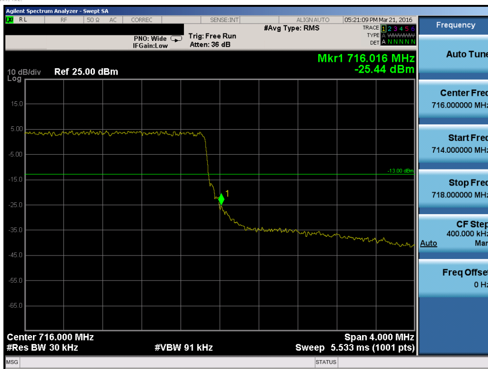
Plot 7-96. Upper Band Edge Plot (Band 12 – 3.0MHz QPSK – RB Size 15)
