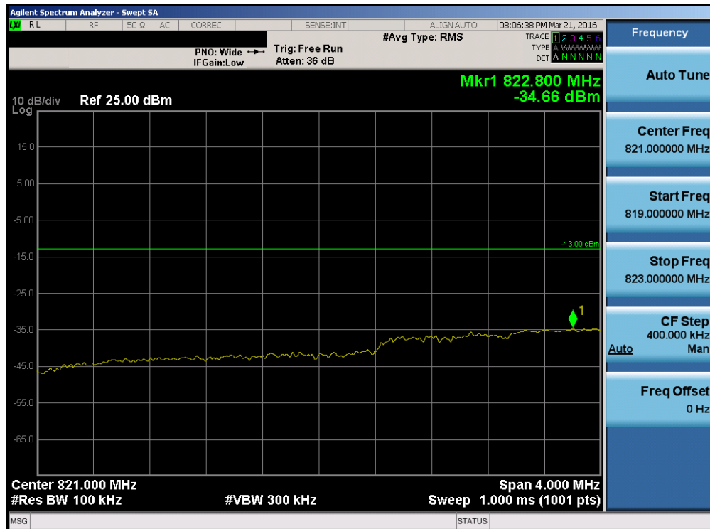
Plot 7-109. Lower Extended Band Edge Plot (Band 5 – 3.0MHz QPSK – RB Size 15)
