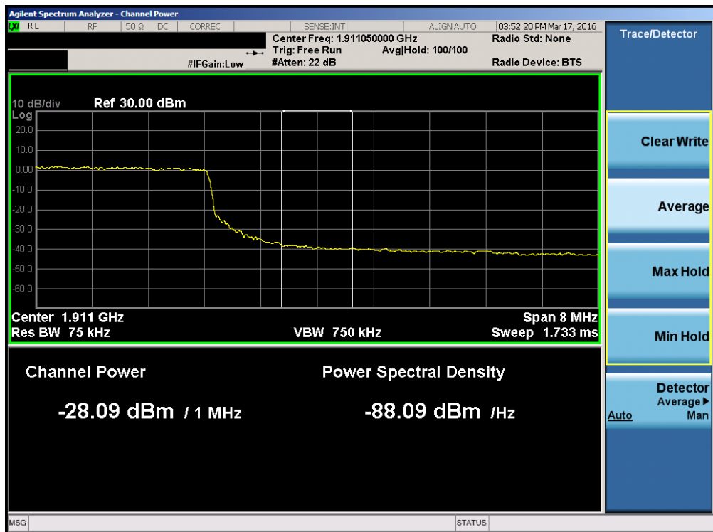
Plot 7-157. Upper Extended Band Edge Plot (Band 2 – 10.0MHz QPSK – RB Size 50)
