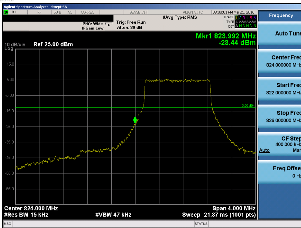
Plot 7-104. Lower Band Edge Plot (Band 5 – 1.4MHz QPSK – RB Size 6)
