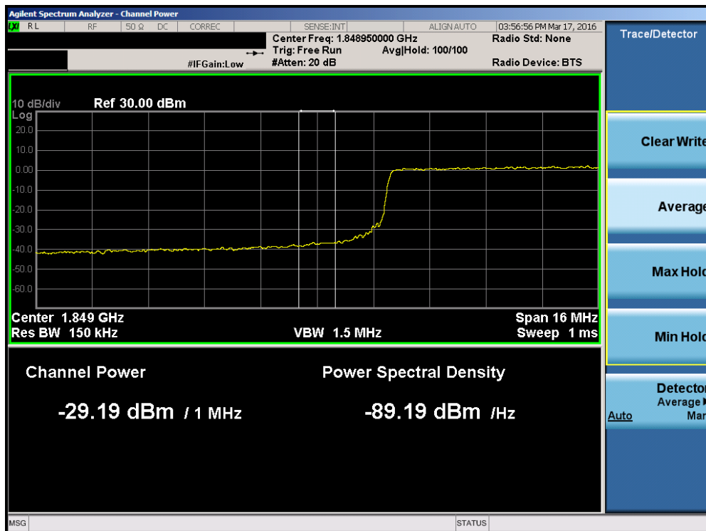
Plot 7-163. Lower Extended Band Edge Plot (Band 2 – 20.0MHz QPSK – RB Size 100)
