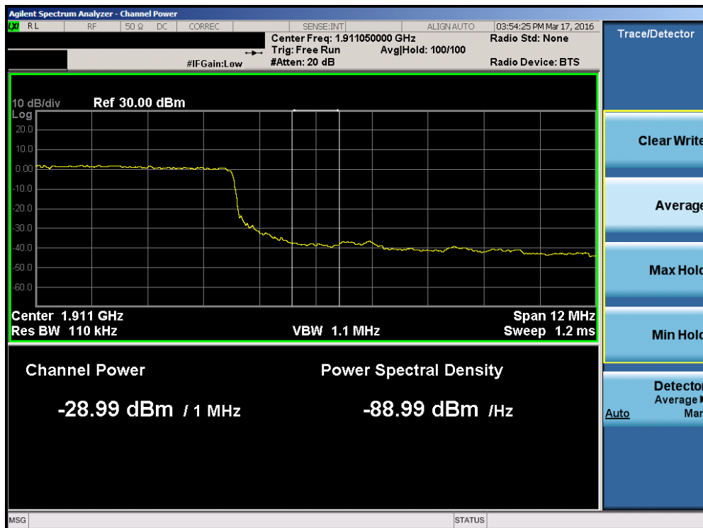
Plot 7-161. Upper Extended Band Edge Plot (Band 2 – 15.0MHz QPSK – RB Size 75)
