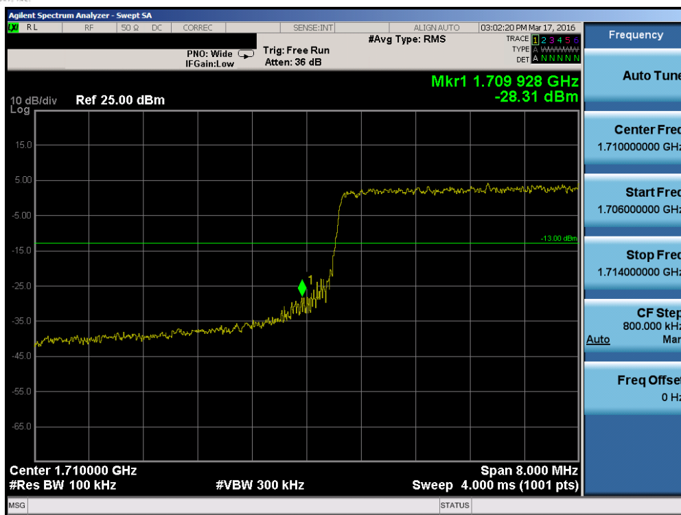
Plot 7-130. Lower Band Edge Plot (Band 4 – 10.0MHz QPSK – RB Size 50)
