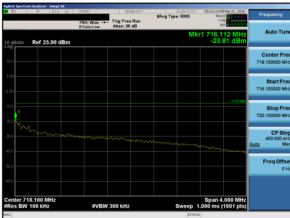
Plot 7-101. Upper Extended Band Edge Plot (Band 12/17 – 5.0MHz QPSK – RB Size 25)
