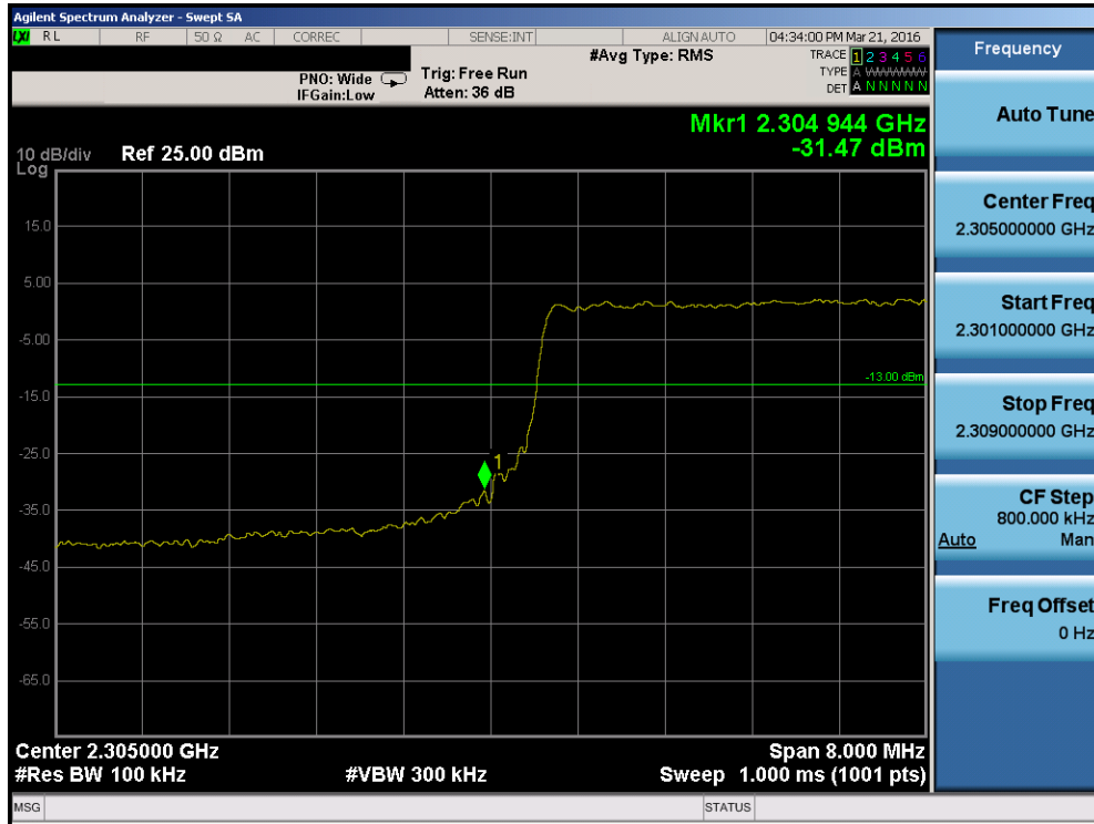
Plot 7-170. Lower Band Edge Plot (Band 30 – 10.0MHz QPSK – RB Size 50)
