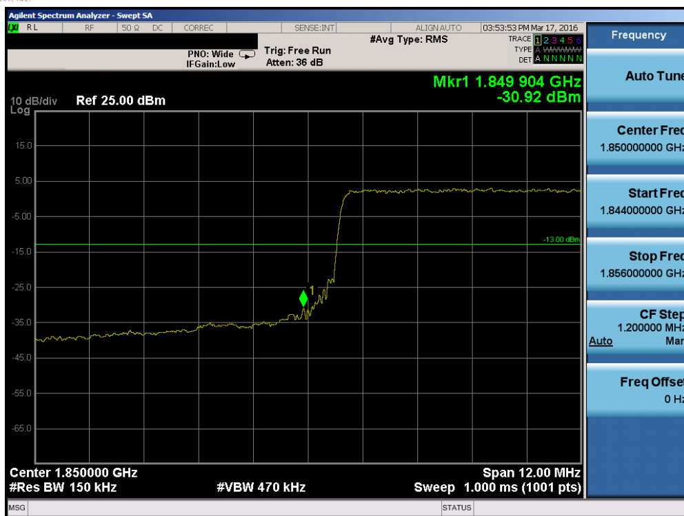
Plot 7-158. Lower Band Edge Plot (Band 2 – 15.0MHz QPSK – RB Size 75)
