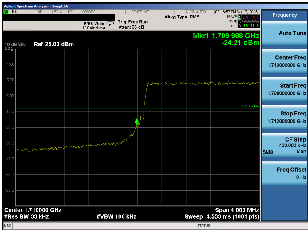
Plot 7-122. Lower Band Edge Plot (Band 4 – 3.0MHz QPSK – RB Size 15)
