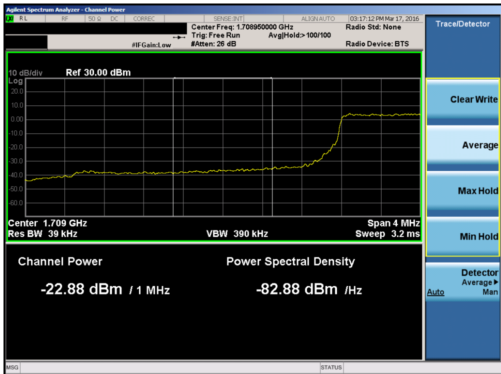
Plot 7-123. Lower Extended Band Edge Plot (Band 4 – 3.0MHz QPSK – RB Size 15)
