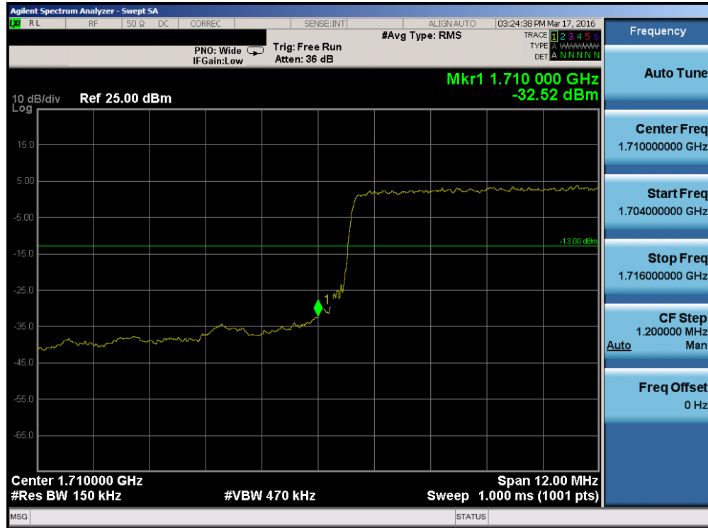
Plot 7-134. Lower Band Edge Plot (Band 4 – 15.0MHz QPSK – RB Size 75)
