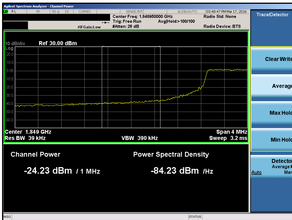
Plot 7-151. Lower Extended Band Edge Plot (Band 2 – 5.0MHz QPSK – RB Size 25)
