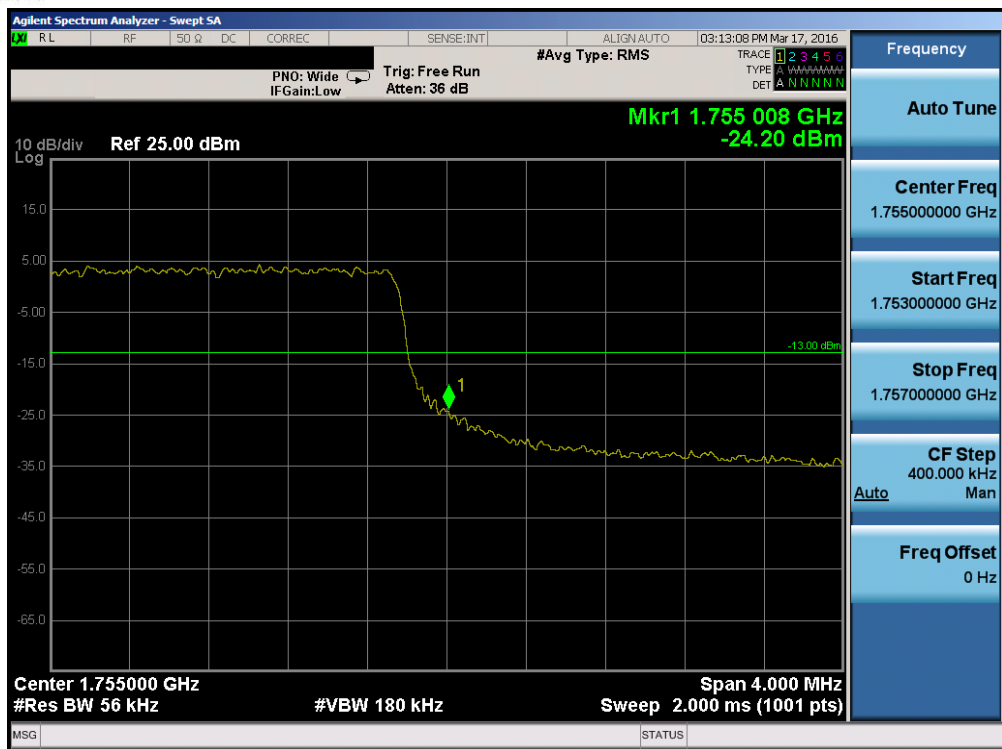
Plot 7-128. Upper Band Edge Plot (Band 4 – 5.0MHz QPSK – RB Size 25)
