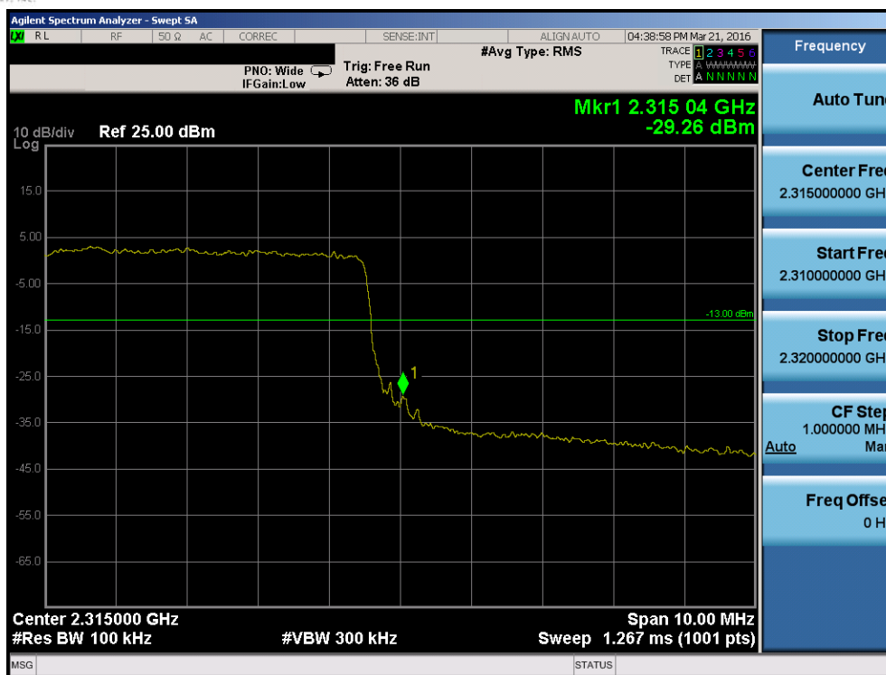
Plot 7-172. Upper Band Edge Plot (Band 30 – 10.0MHz QPSK – RB Size 50)
