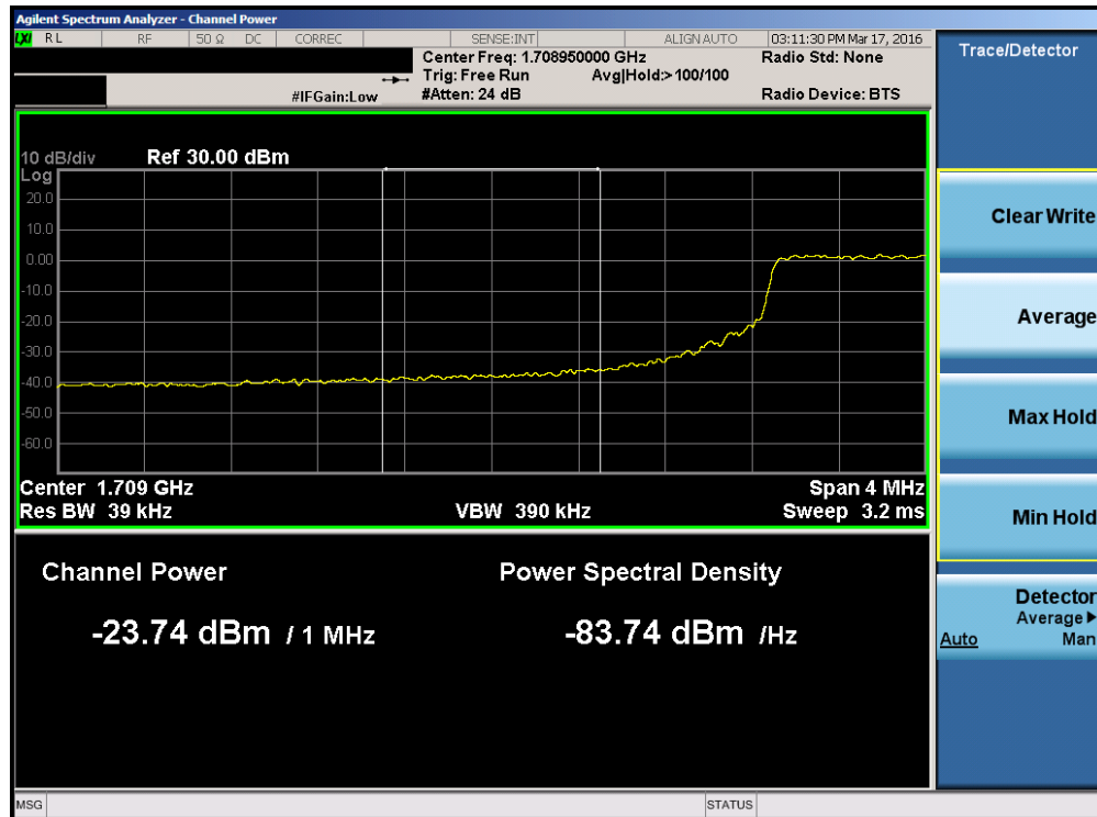
Plot 7-127. Lower Extended Band Edge Plot (Band 4 – 5.0MHz QPSK – RB Size 25)
