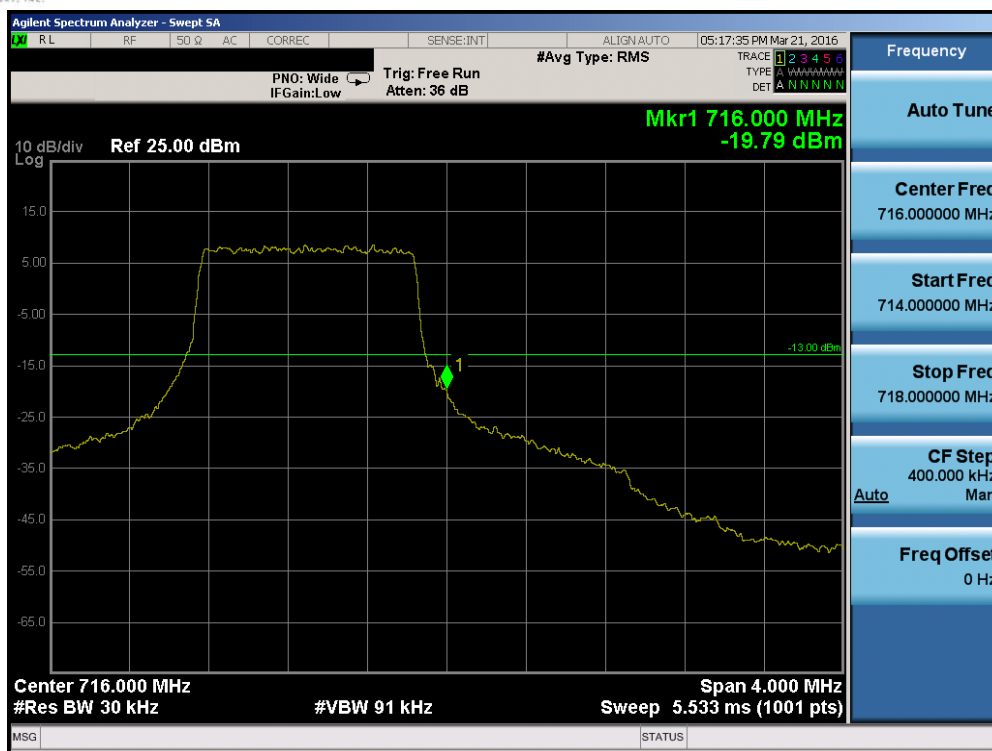
Plot 7-92. Upper Band Edge Plot (Band 12 – 1.4MHz QPSK – RB Size 6)
