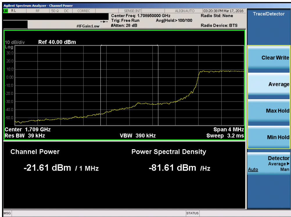
Plot 7-119. Lower Extended Band Edge Plot (Band 4 – 1.4MHz QPSK – RB Size 6)
