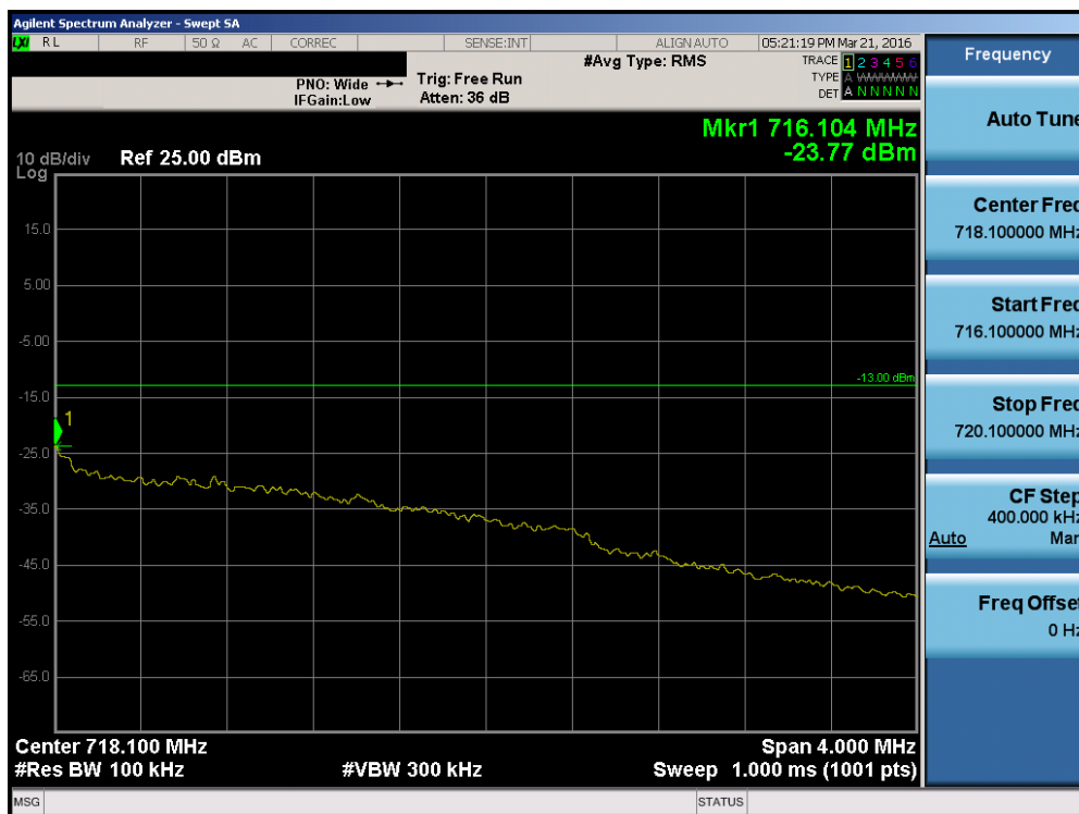
Plot 7-97. Upper Extended Band Edge Plot (Band 12 – 3.0MHz QPSK – RB Size 15)
