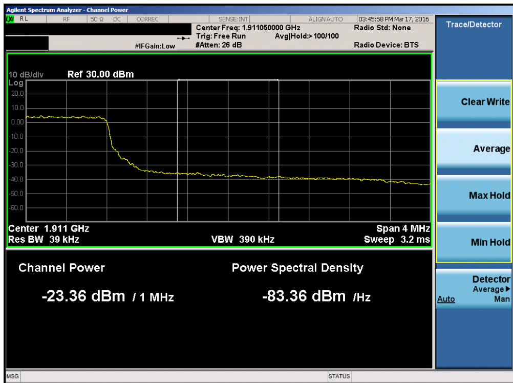
Plot 7-149. Upper Extended Band Edge Plot (Band 2 – 3.0MHz QPSK – RB Size 15)
