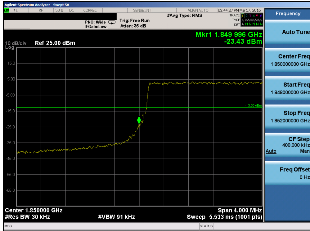
Plot 7-146. Lower Band Edge Plot (Band 2 – 3.0MHz QPSK – RB Size 15)
