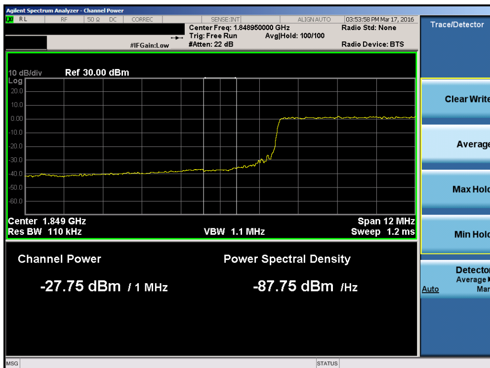
Plot 7-159. Lower Extended Band Edge Plot (Band 2 – 15.0MHz QPSK – RB Size 75)
