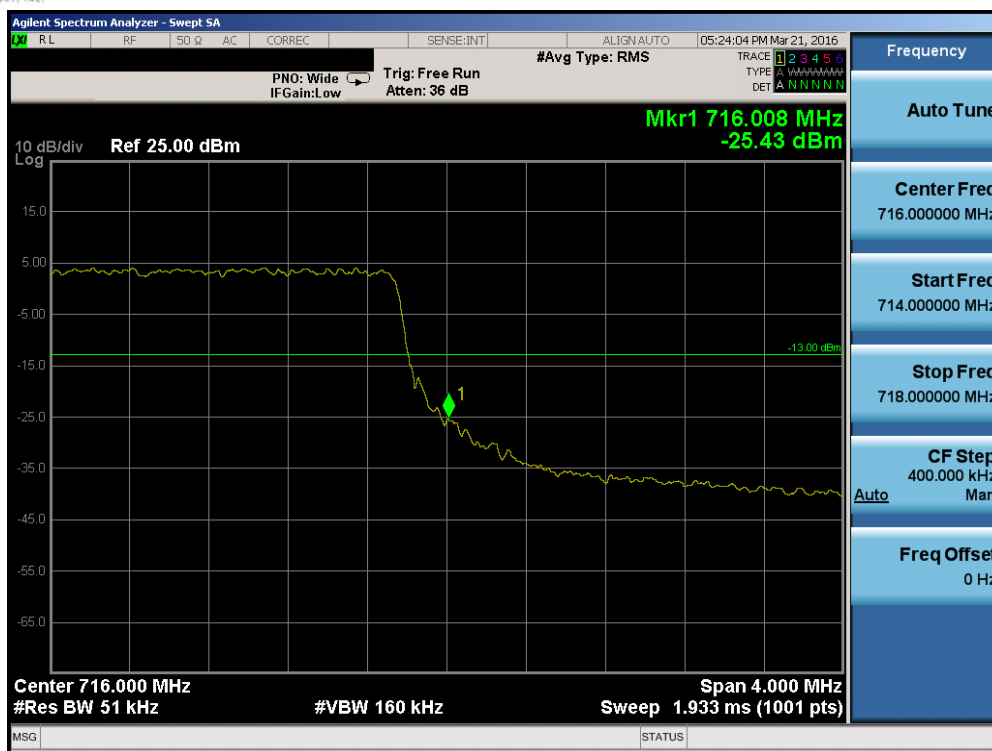
Plot 7-100. Upper Band Edge Plot (Band 12/17 – 5.0MHz QPSK – RB Size 25)
