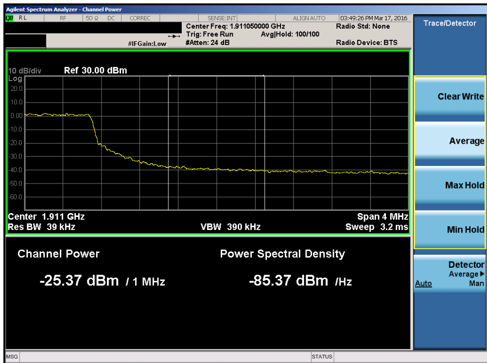
Plot 7-153. Upper Extended Band Edge Plot (Band 2 – 5.0MHz QPSK – RB Size 25)
