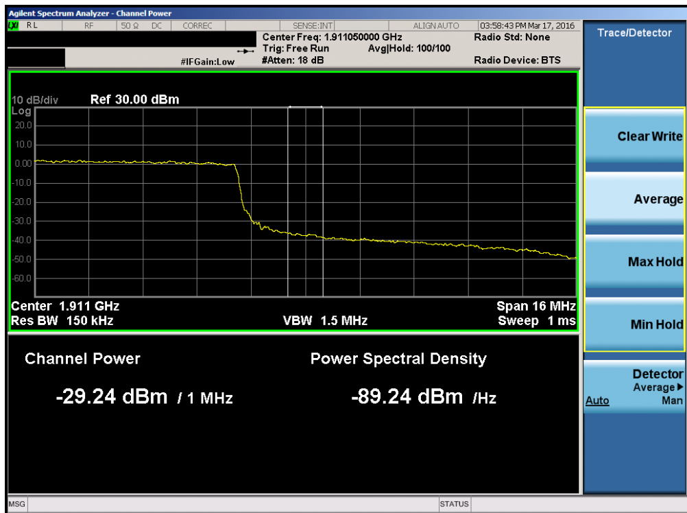
Plot 7-165. Upper Extended Band Edge Plot (Band 2 – 20.0MHz QPSK – RB Size 100)
