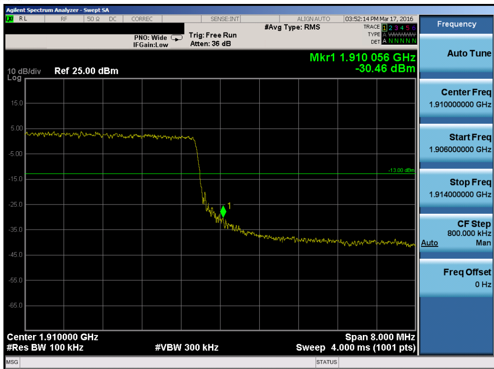
Plot 7-156. Upper Band Edge Plot (Band 2 – 10.0MHz QPSK – RB Size 50)
