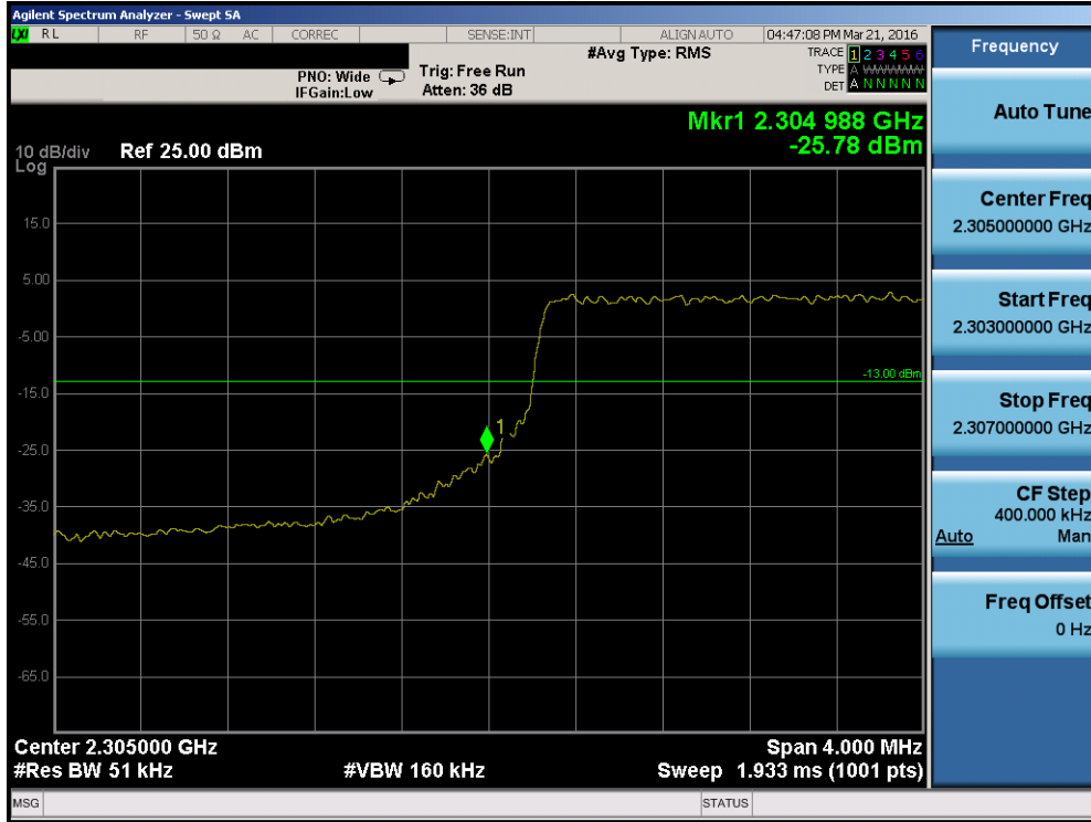
Plot 7-166. Lower Band Edge Plot (Band 30 – 5.0MHz QPSK – RB Size 25)
