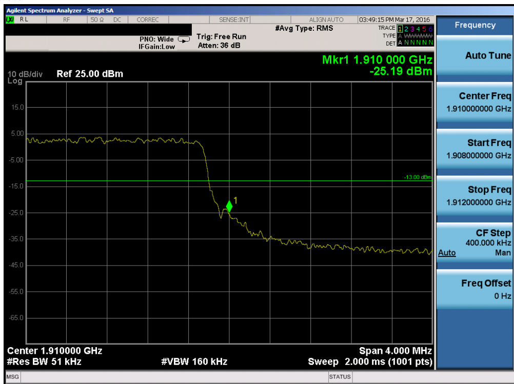
Plot 7-152. Upper Band Edge Plot (Band 2 – 5.0MHz QPSK – RB Size 25)
