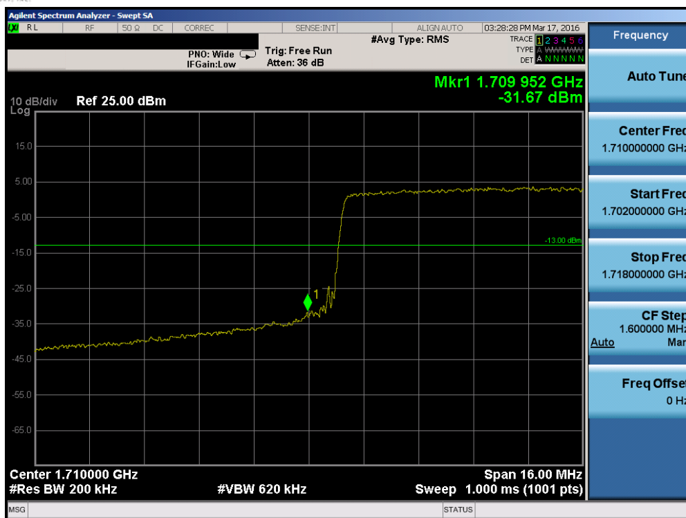
Plot 7-138. Lower Band Edge Plot (Band 4 – 20.0MHz QPSK – RB Size 100)
