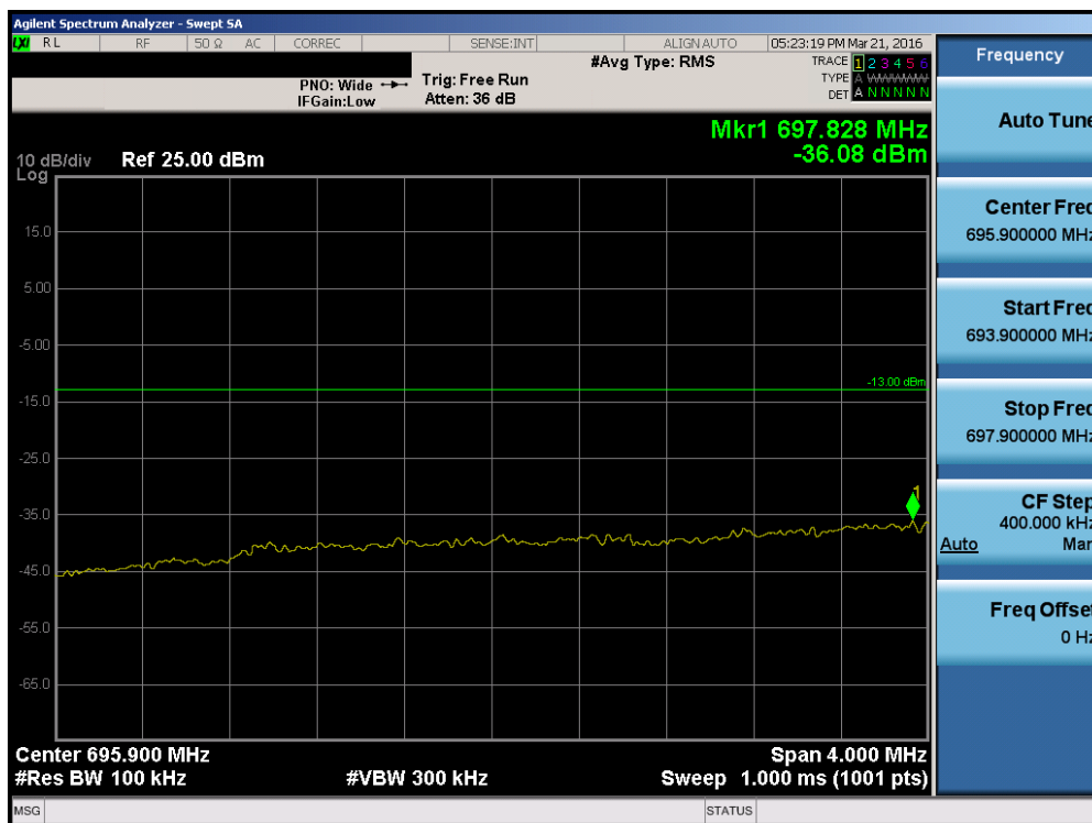
Plot 7-99. Lower Extended Band Edge Plot (Band 12/17 - 5.0MHz QPSK - RB Size 25)
