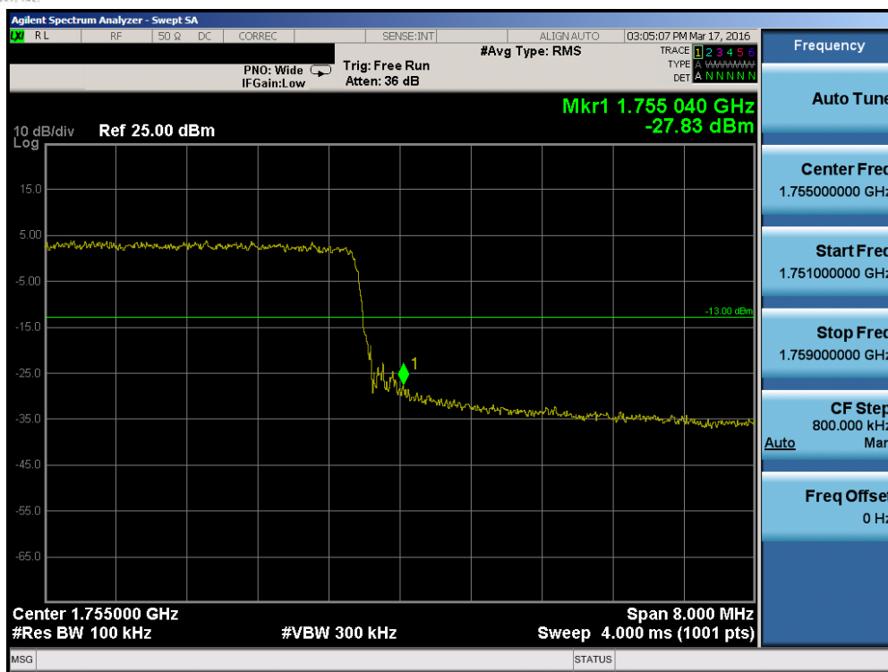
Plot 7-132. Upper Band Edge Plot (Band 4 – 10.0MHz QPSK – RB Size 50)
