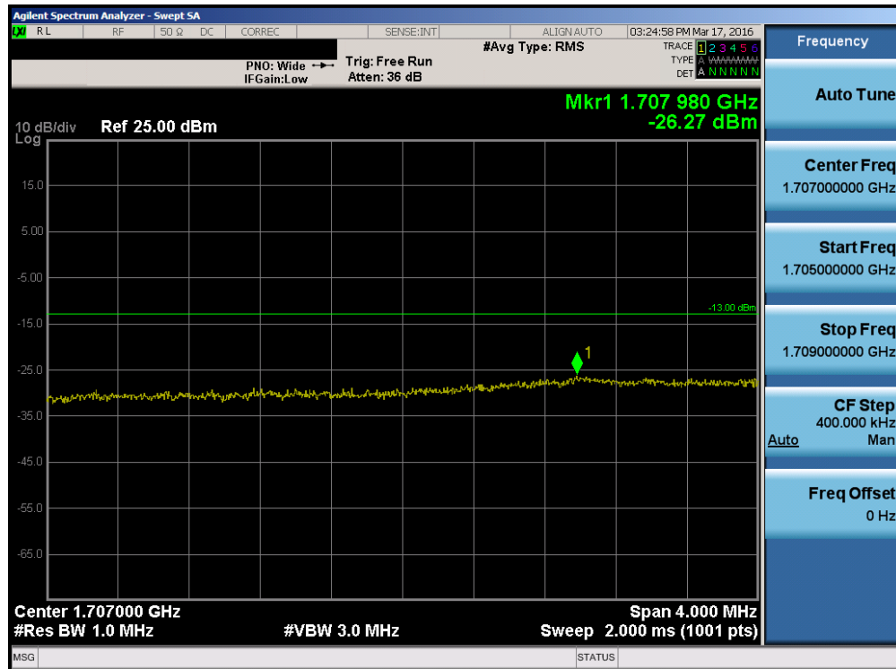
Plot 7-135. Lower Extended Band Edge Plot (Band 4 – 15.0MHz QPSK – RB Size 75)
