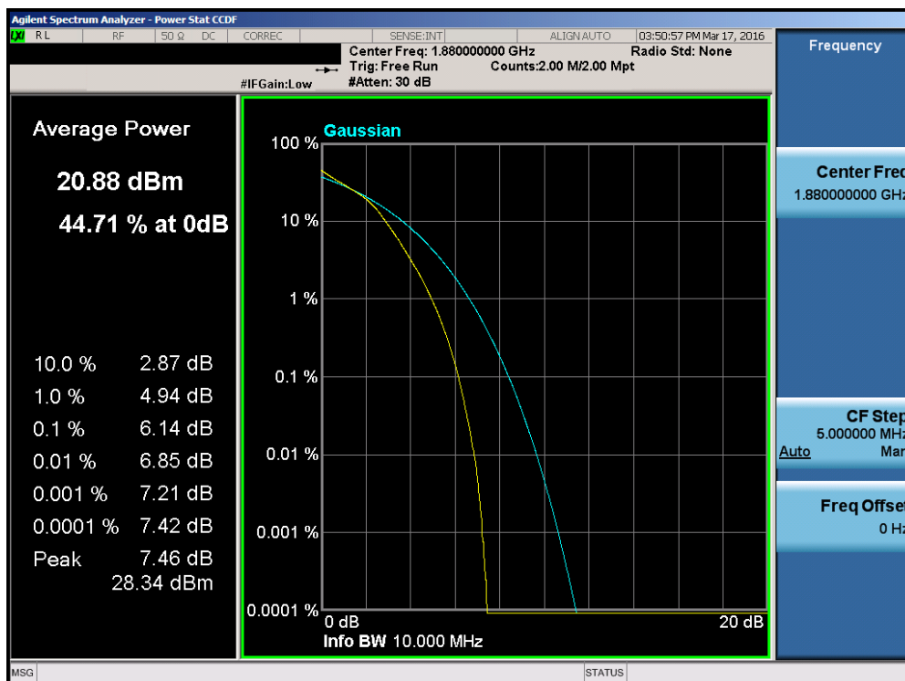
Plot 7-181. PAR Plot (Band 2 – 10.0MHz 16-QAM – RB Size 50)
