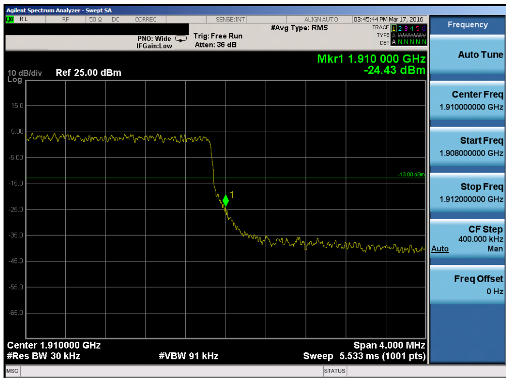
Plot 7-148. Upper Band Edge Plot (Band 2 – 3.0MHz QPSK – RB Size 15)
