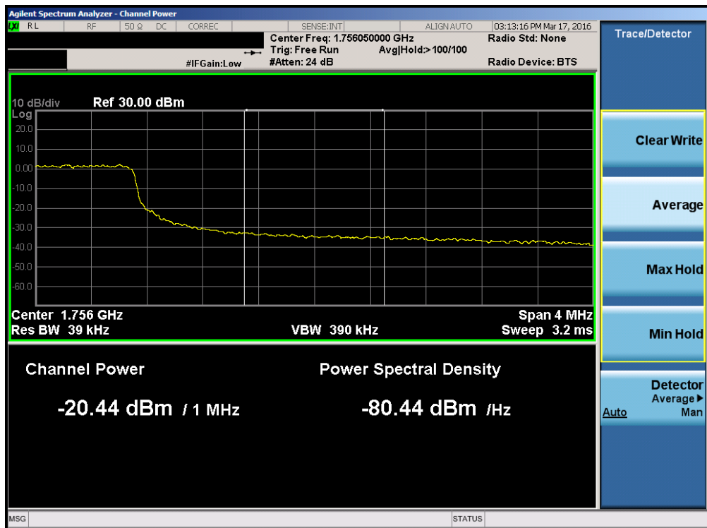
Plot 7-129. Upper Extended Band Edge Plot (Band 4 – 5.0MHz QPSK – RB Size 25)
