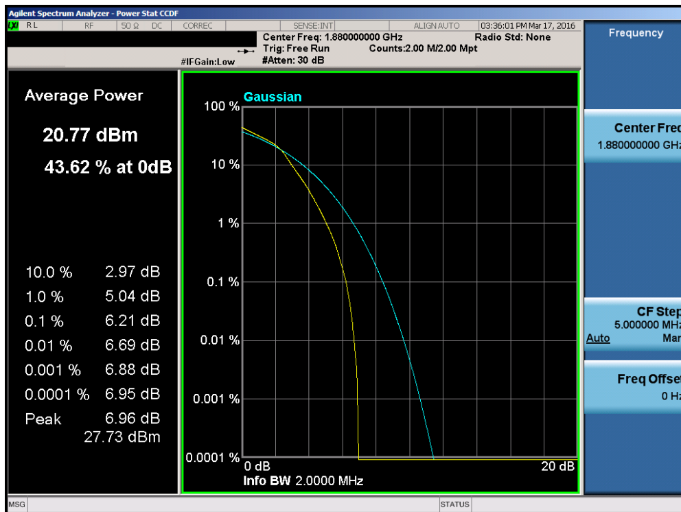
Plot 7-175. PAR Plot (Band 2 – 1.4MHz 16-QAM – RB Size 6)
