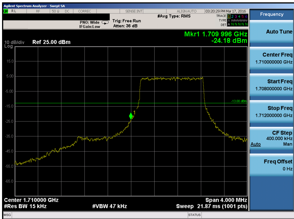
Plot 7-118. Lower Band Edge Plot (Band 4 – 1.4MHz QPSK – RB Size 6)
