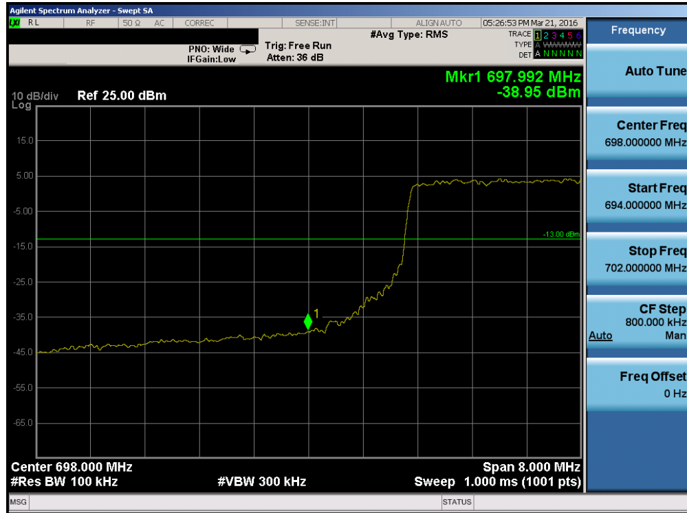
Plot 7-102. Lower Band Edge Plot (Band 12/17 – 10.0MHz QPSK – RB Size 50)
