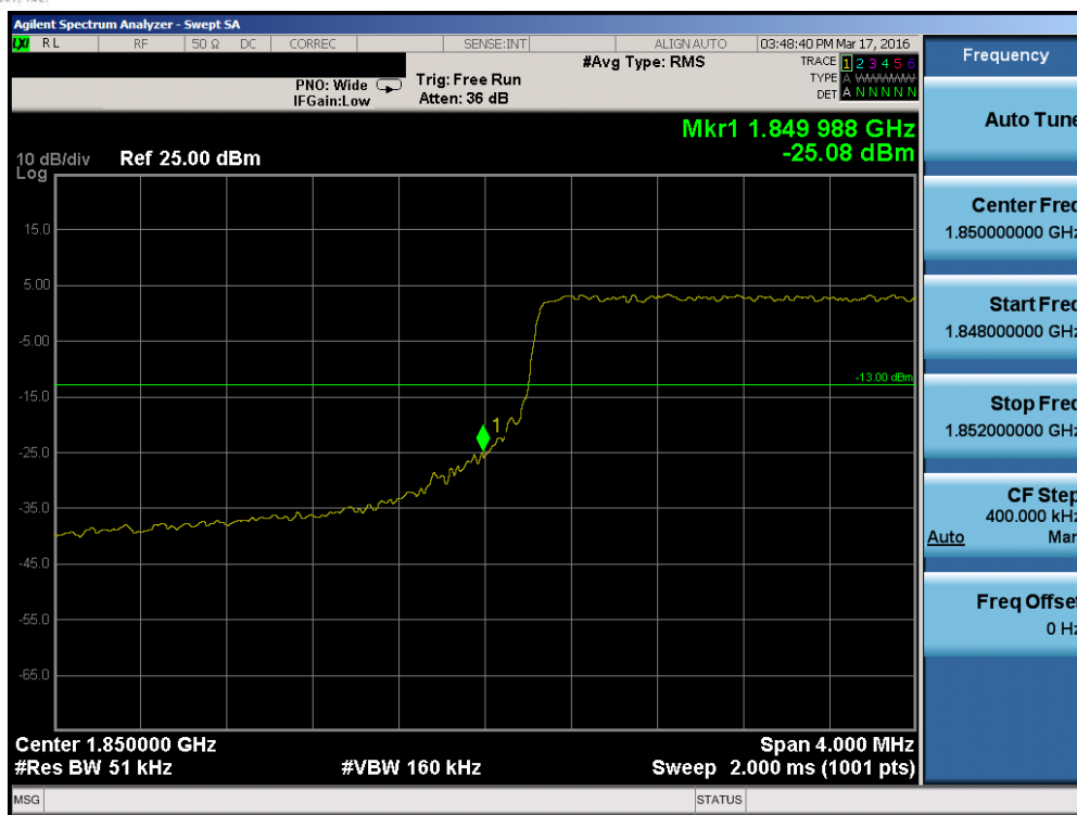
Plot 7-150. Lower Band Edge Plot (Band 2 – 5.0MHz QPSK – RB Size 25)
