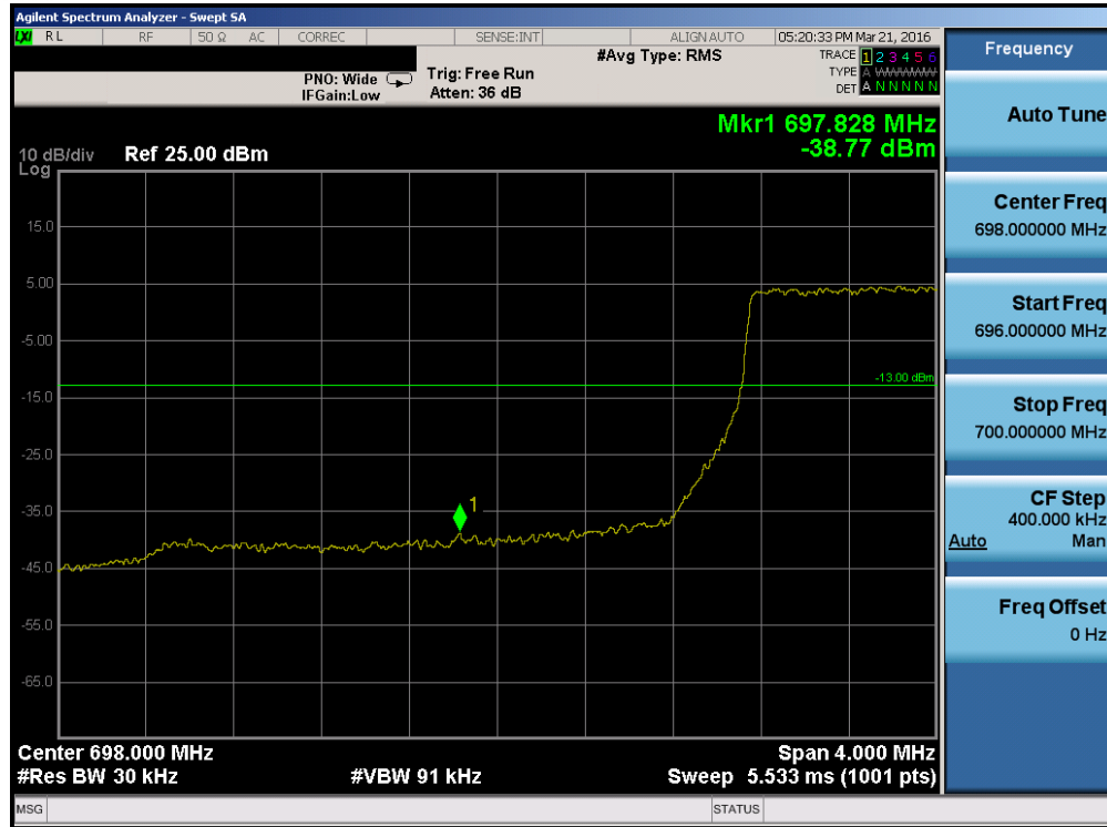
Plot 7-94. Lower Band Edge Plot (Band 12 – 3.0MHz QPSK – RB Size 15)
