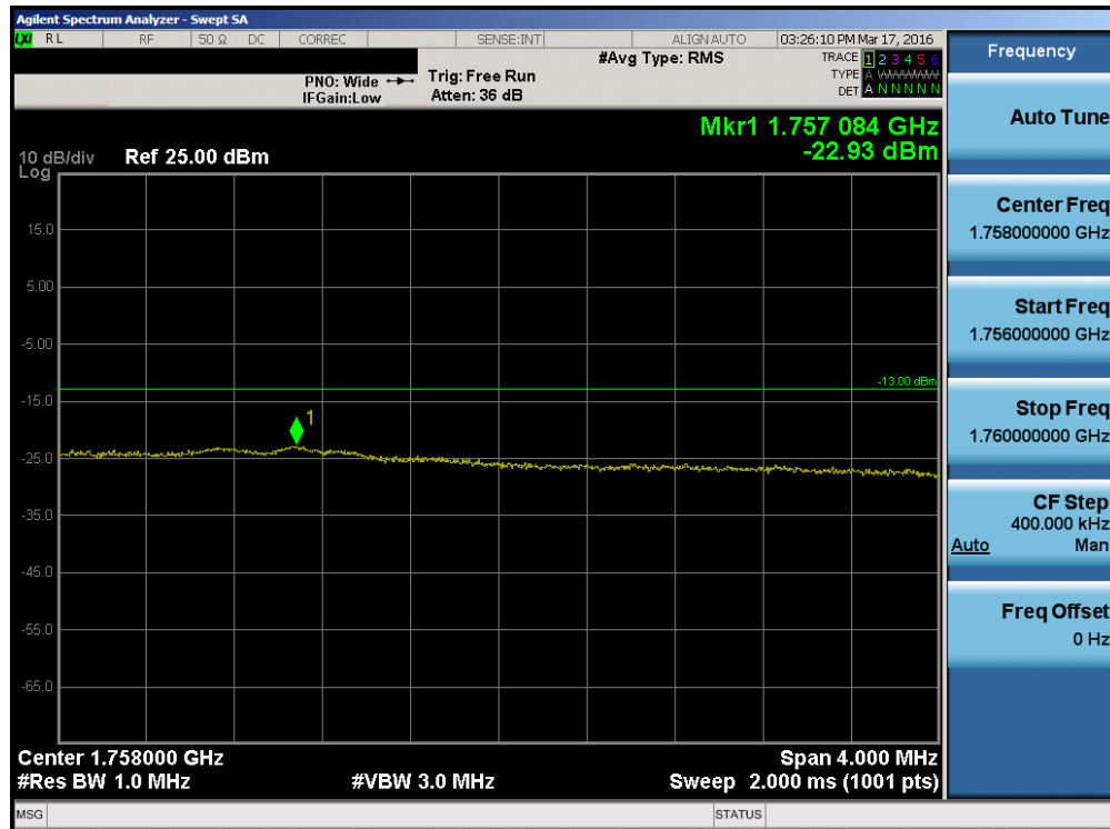
Plot 7-137. Upper Extended Band Edge Plot (Band 4 – 15.0MHz QPSK – RB Size 75)
