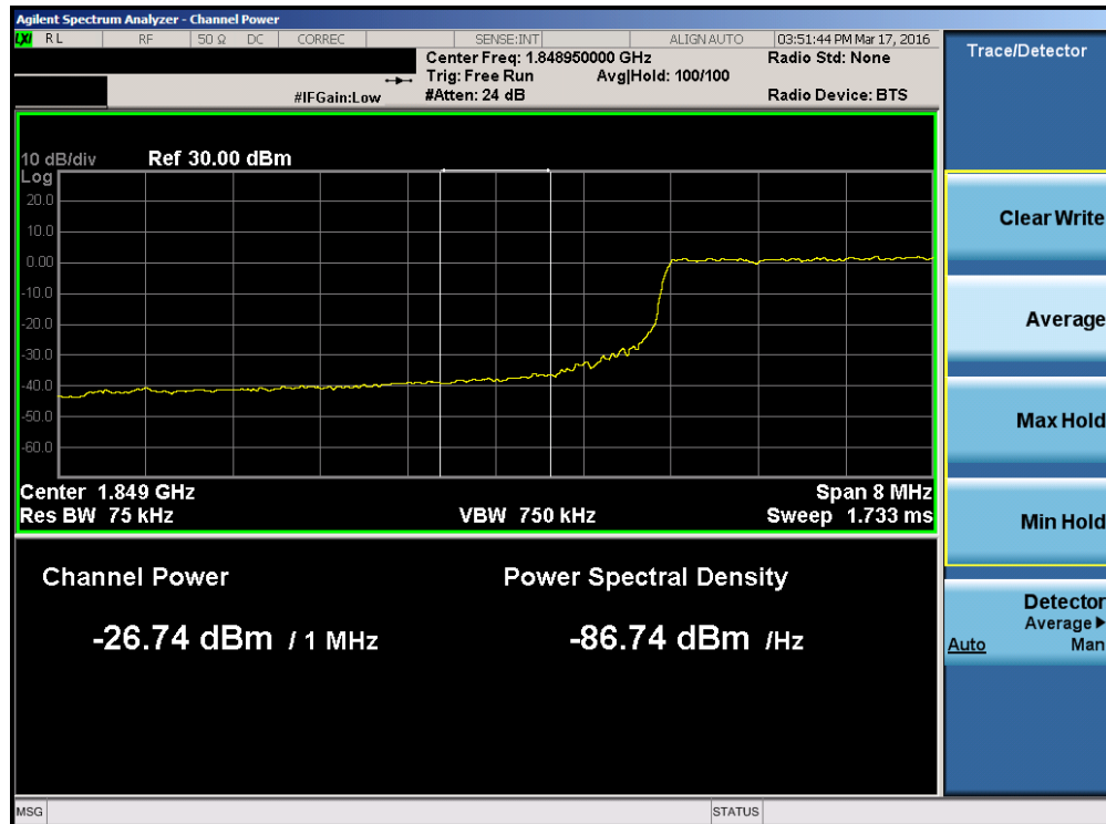
Plot 7-155. Lower Extended Band Edge Plot (Band 2 – 10.0MHz QPSK – RB Size 50)
