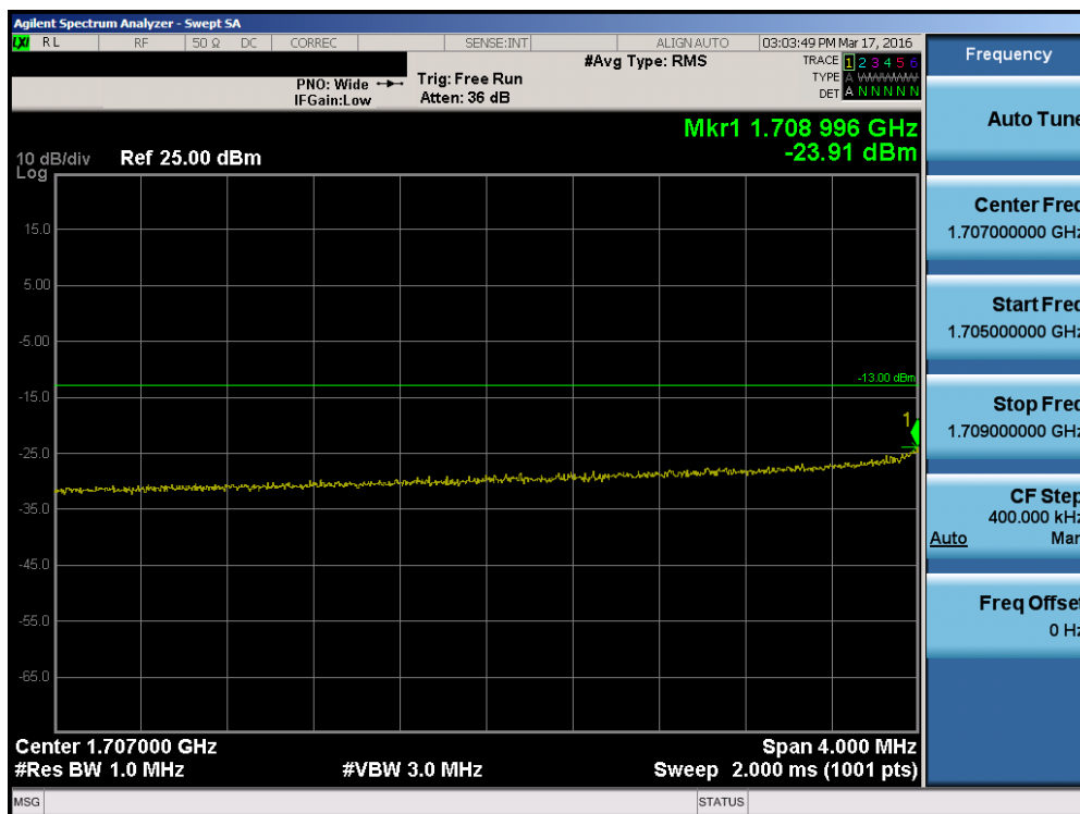
Plot 7-131. Lower Extended Band Edge Plot (Band 4 – 10.0MHz QPSK – RB Size 50)
