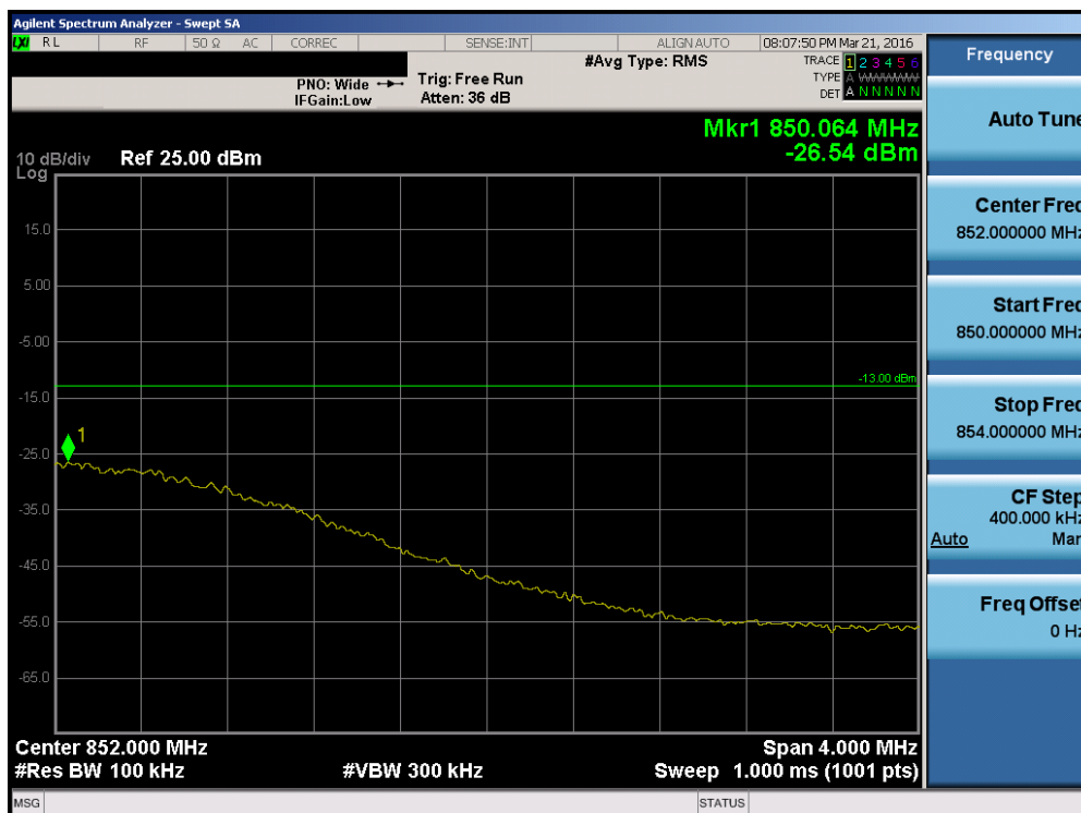
Plot 7-111. Upper Extended Band Edge Plot (Band 5 – Band 5 – 3.0MHz QPSK – RB Size 15)
