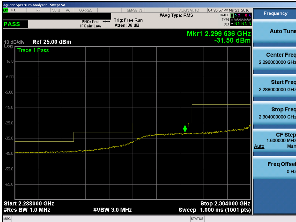
Plot 7-171. Lower Extended Band Edge Plot (Band 30 – 10.0MHz QPSK – RB Size 50)
