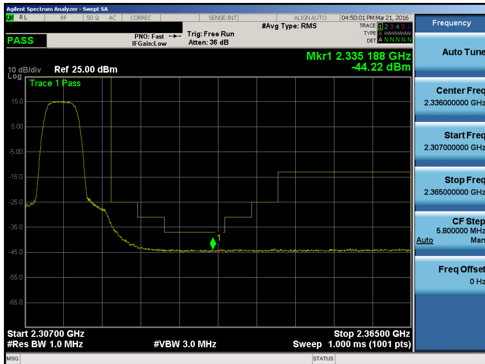
Plot 7-169. Upper Extended Band Edge Plot (Band 30 – 5.0MHz QPSK – RB Size 25)
