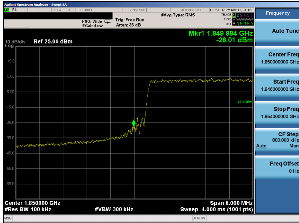
Plot 7-154. Lower Band Edge Plot (Band 2 – 10.0MHz QPSK – RB Size 50)
