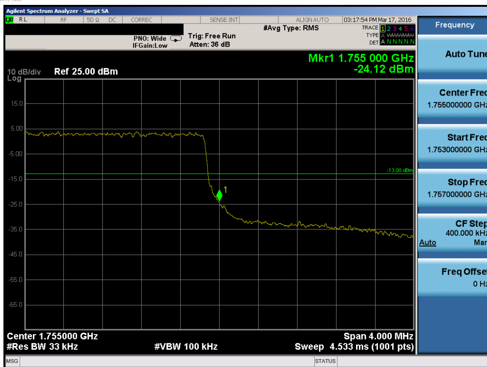
Plot 7-124. Upper Band Edge Plot (Band 4 – 3.0MHz QPSK – RB Size 15)
