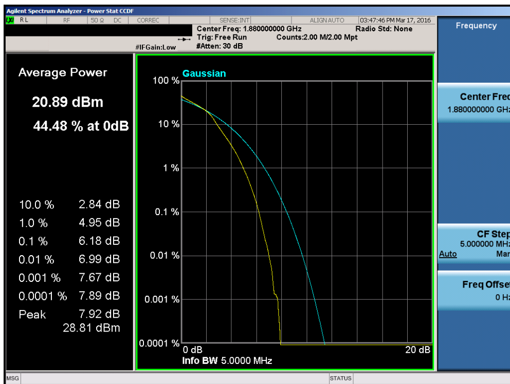
Plot 7-179. PAR Plot (Band 2 – 5.0MHz 16-QAM – RB Size 25)
