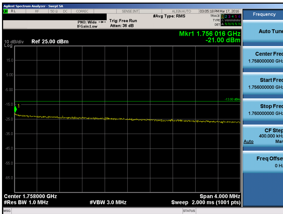
Plot 7-133. Upper Extended Band Edge Plot (Band 4 – 10.0MHz QPSK – RB Size 50)
