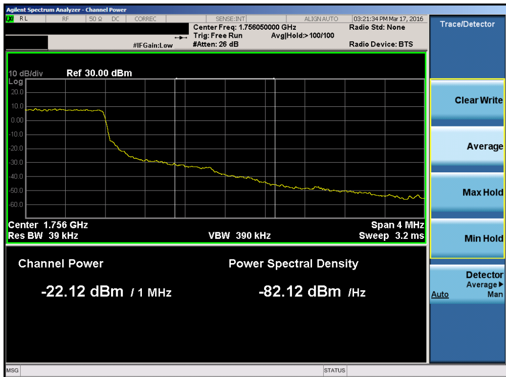
Plot 7-121. Upper Extended Band Edge Plot (Band 4 – 1.4MHz QPSK – RB Size 6)
