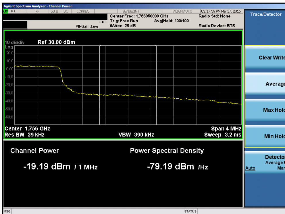
Plot 7-125. Upper Extended Band Edge Plot (Band 4 – 3.0MHz QPSK – RB Size 15)
