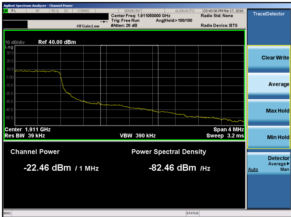
Plot 7-145. Upper Extended Band Edge Plot (Band 2 – 1.4MHz QPSK – RB Size 6)
