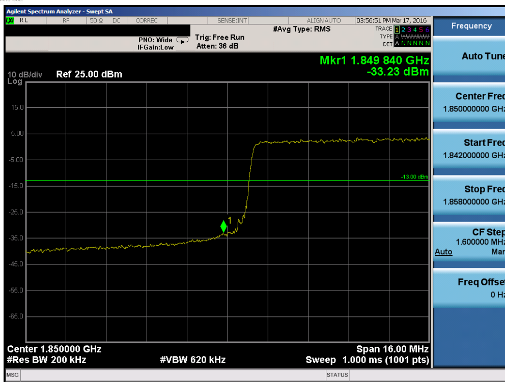
Plot 7-162. Lower Band Edge Plot (Band 2 – 20.0MHz QPSK – RB Size 100)
