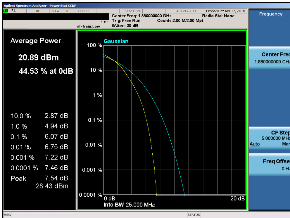
Plot 7-185. PAR Plot (Band 2 – 20.0MHz 16-QAM – RB Size 100)
