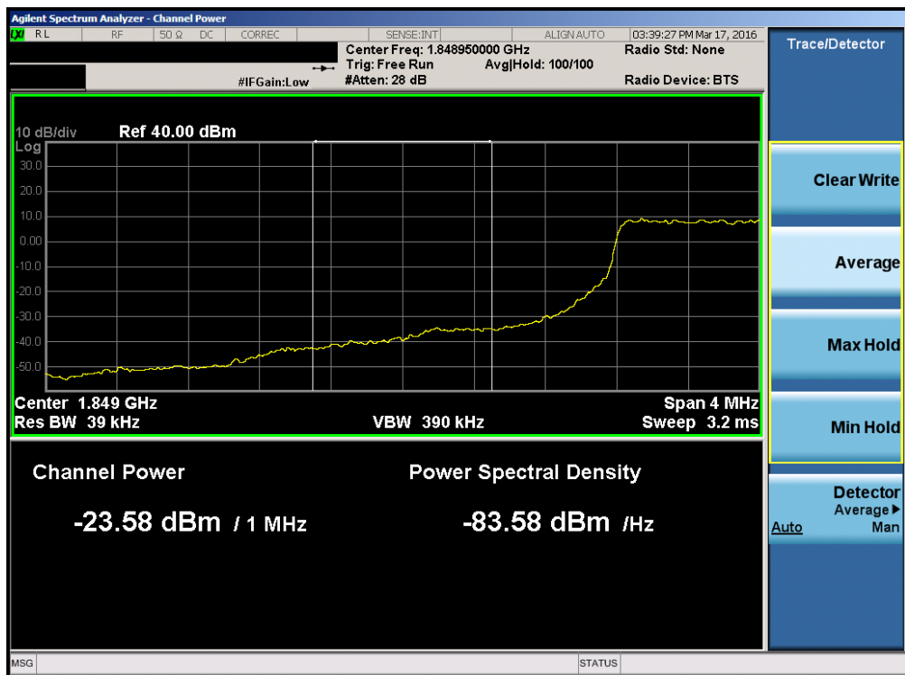
Plot 7-143. Lower Extended Band Edge Plot (Band 2 – 1.4MHz QPSK – RB Size 6)
