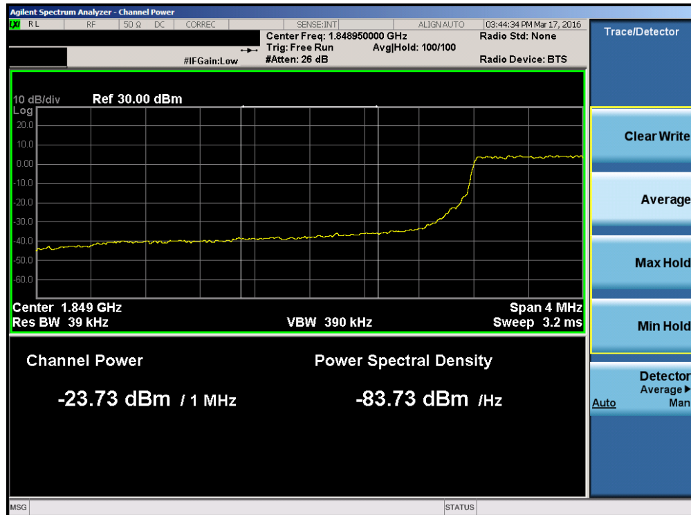
Plot 7-147. Lower Extended Band Edge Plot (Band 2 – 3.0MHz QPSK – RB Size 15)
