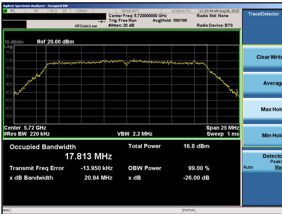
Plot 6-22. 26dB Bandwidth Plot (20MHz BW 802.11n (UNII Band 2C) – Ch. 144)
