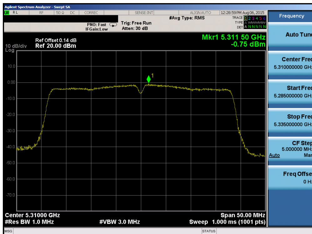
Plot 6-49. Power Spectral Density Plot (40MHz BW 802.11a/n (UNII Band 2A) – Ch. 62)
