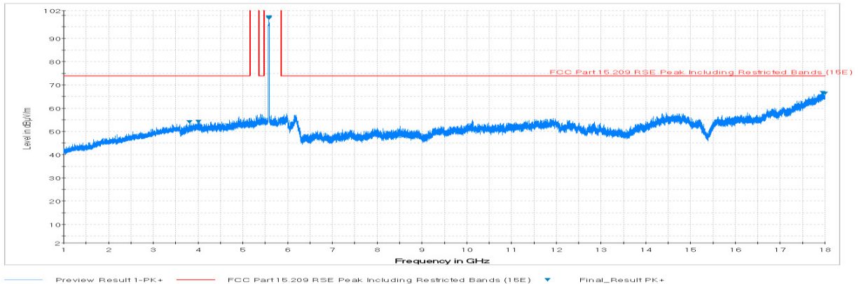
Plot 6-72. Radiated Spurious Plot above 1GHz (802.11a – U2C Ch. 120, Ant. Pol. V)
