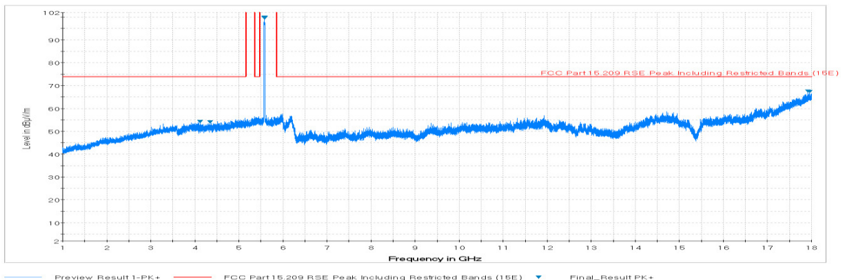
Plot 6-71. Radiated Spurious Plot above 1GHz (802.11a – U2C Ch. 120, Ant. Pol. H)
