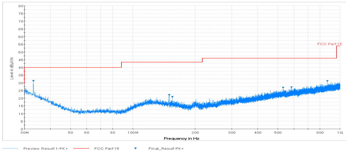
Plot 6-44. Radiated Spurious Plot below 1GHz (Pol. V)
