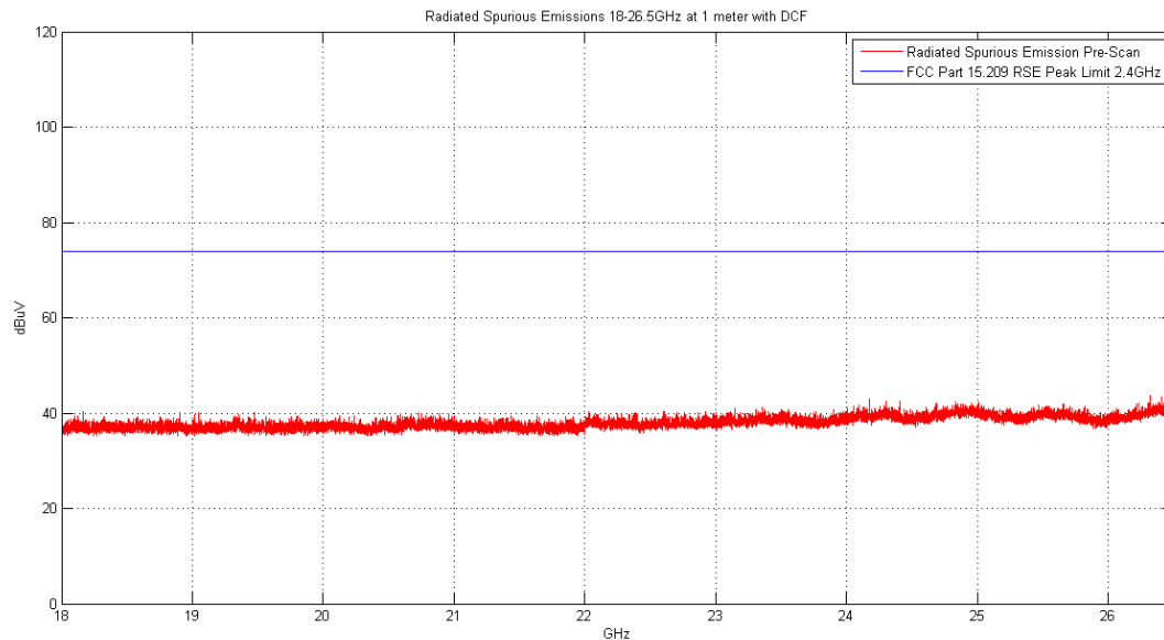
Plot 6-38. Radiated Spurious Plot above 18GHz (Pol. V)
