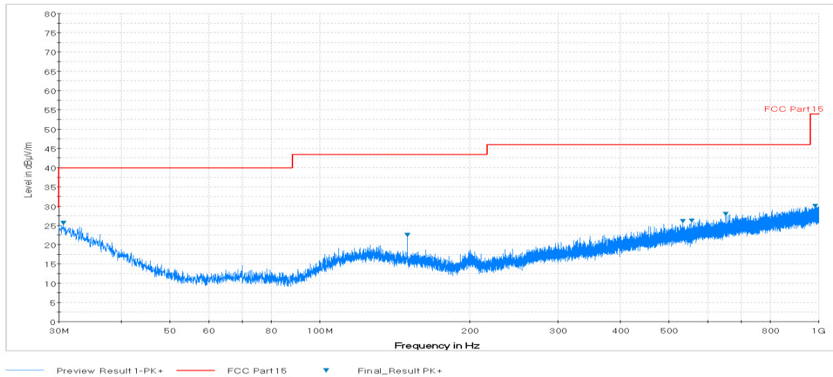
Plot 6-43. Radiated Spurious Plot below 1GHz (Pol. H)
