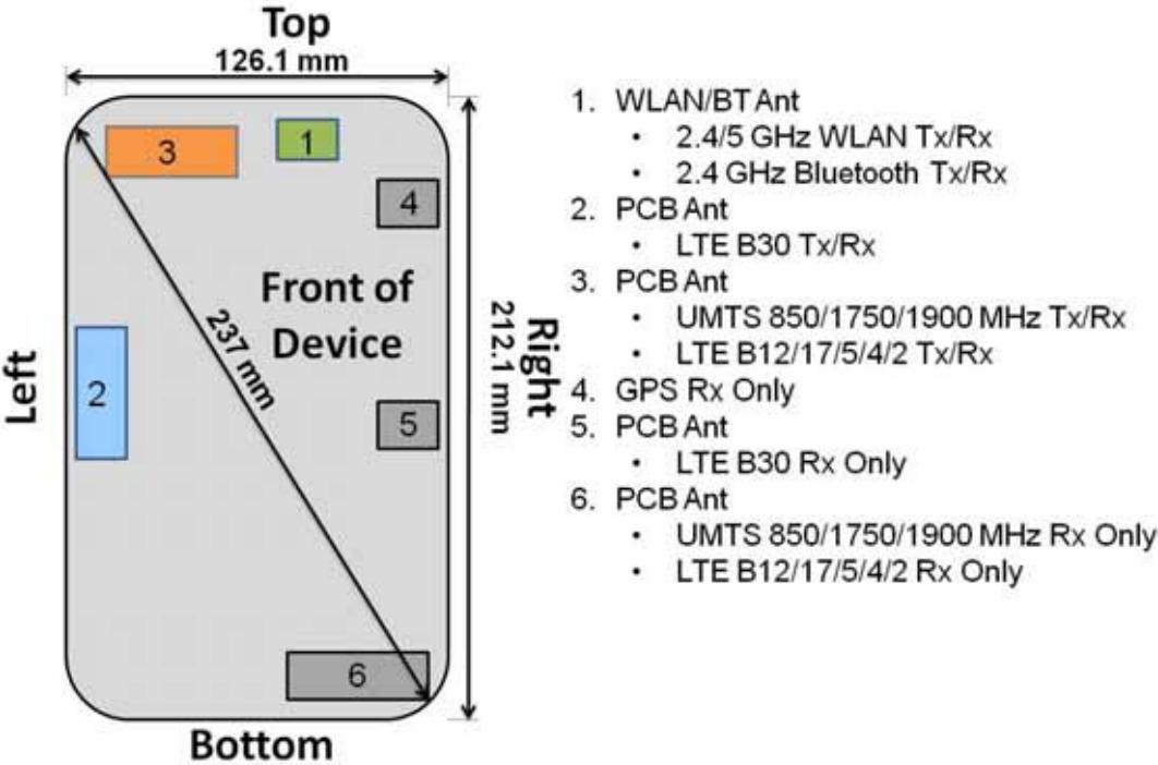
Figure F-1 DUT Antenna Locations
