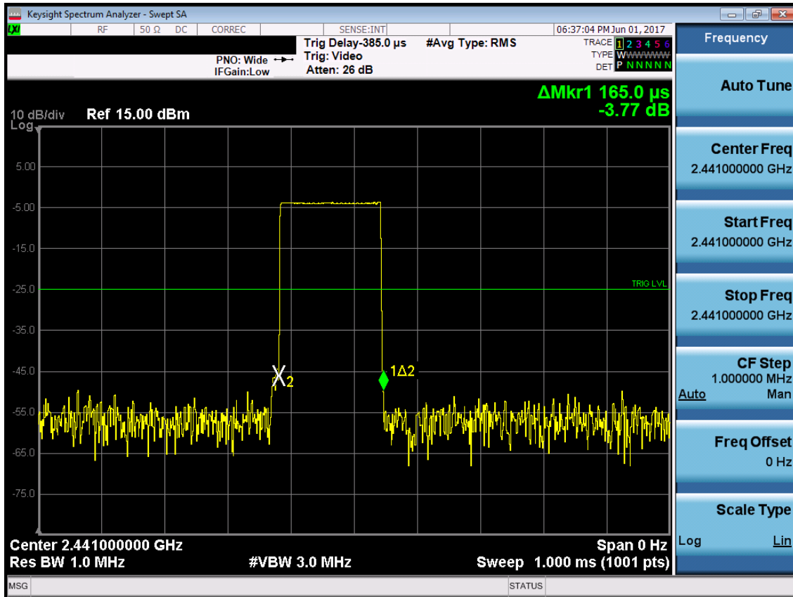
Plot 7-2. Pulse Width Measurement
