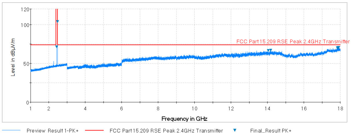
Plot 7-47. Radiated Spurious Plot above 1GHz (BT – Ch. 78, Ant. Pol. V)
