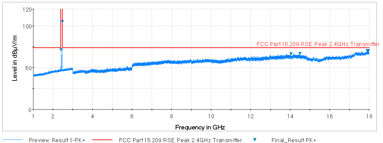
Plot 7-46. Radiated Spurious Plot above 1GHz (BT – Ch. 78, Ant. Pol. H)
