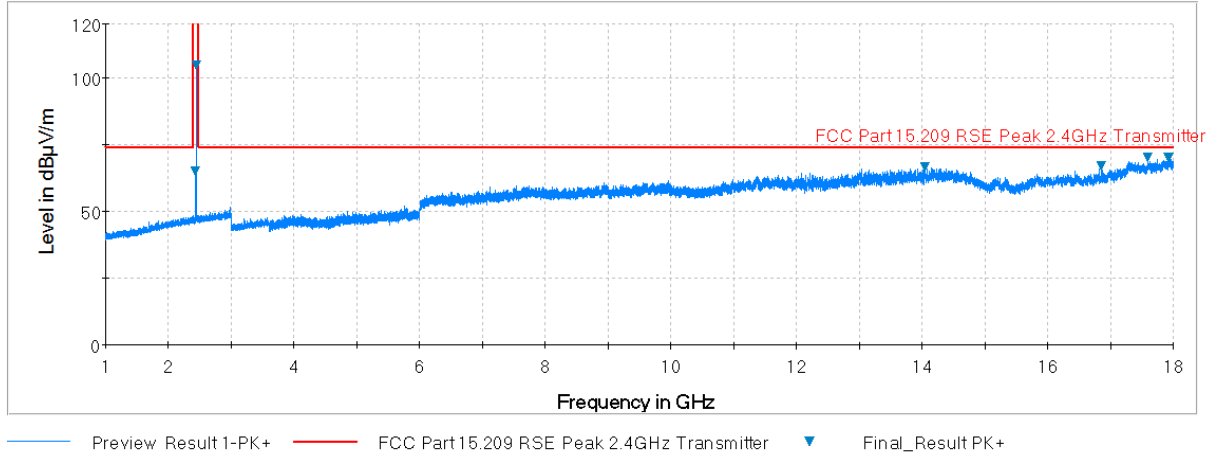
Plot 7-45. Radiated Spurious Plot above 1GHz (BT – Ch. 39, Ant. Pol. V)
