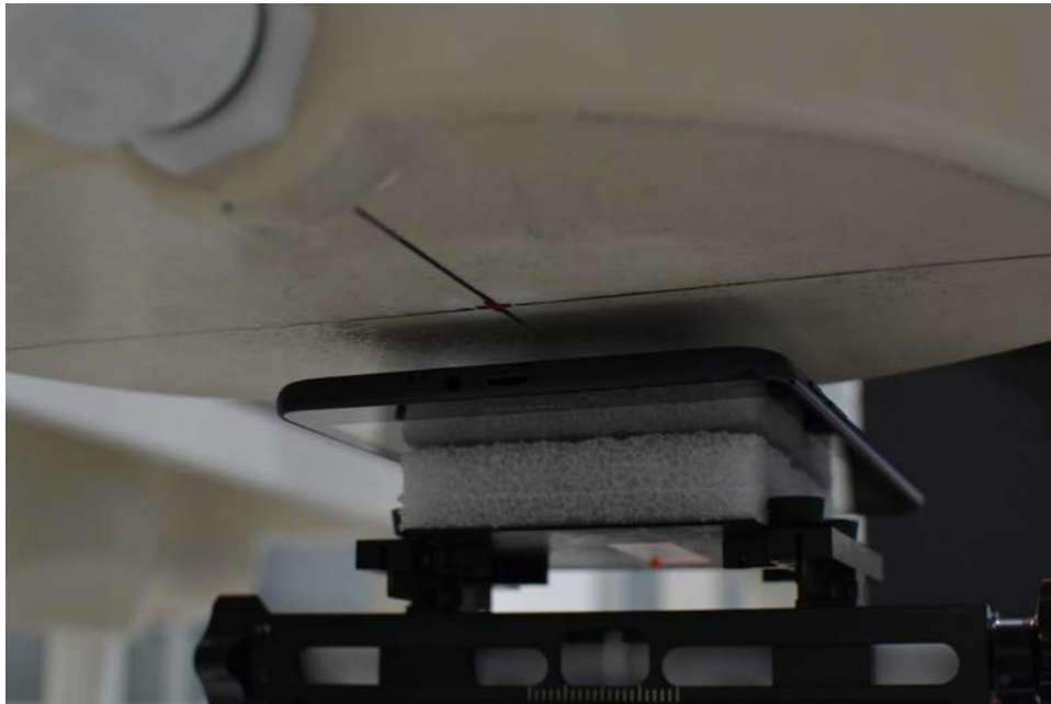
SAR Test Setup Photo 2: Back Side at 11 mm (5 GHz WLAN testing)
