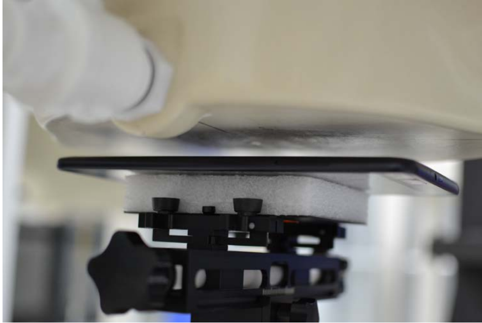
SAR Test Setup Photo 1: Back Side at 11 mm
