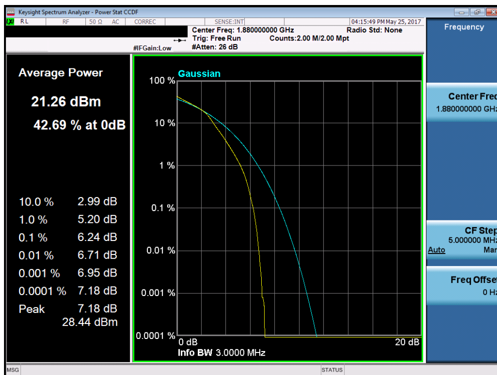
Plot 7-186. PAR Plot (Band 2 – 3.0MHz 16-QAM – RB Size 15)
