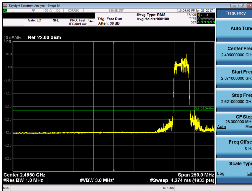
Plot 7-181. Lower Band Edge Plot (Band 38 – 20.0MHz QPSK – RB Size 100)
