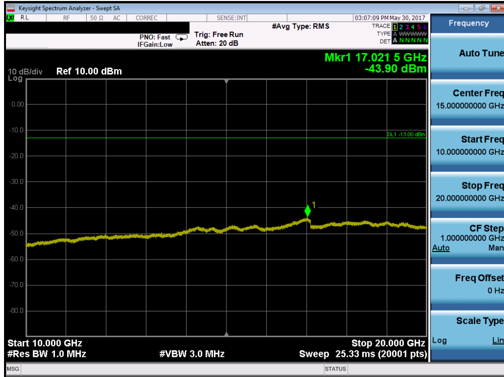
Plot 7-44. Conducted Spurious Plot (AWS WCDMA Mode – Ch. 1513)
