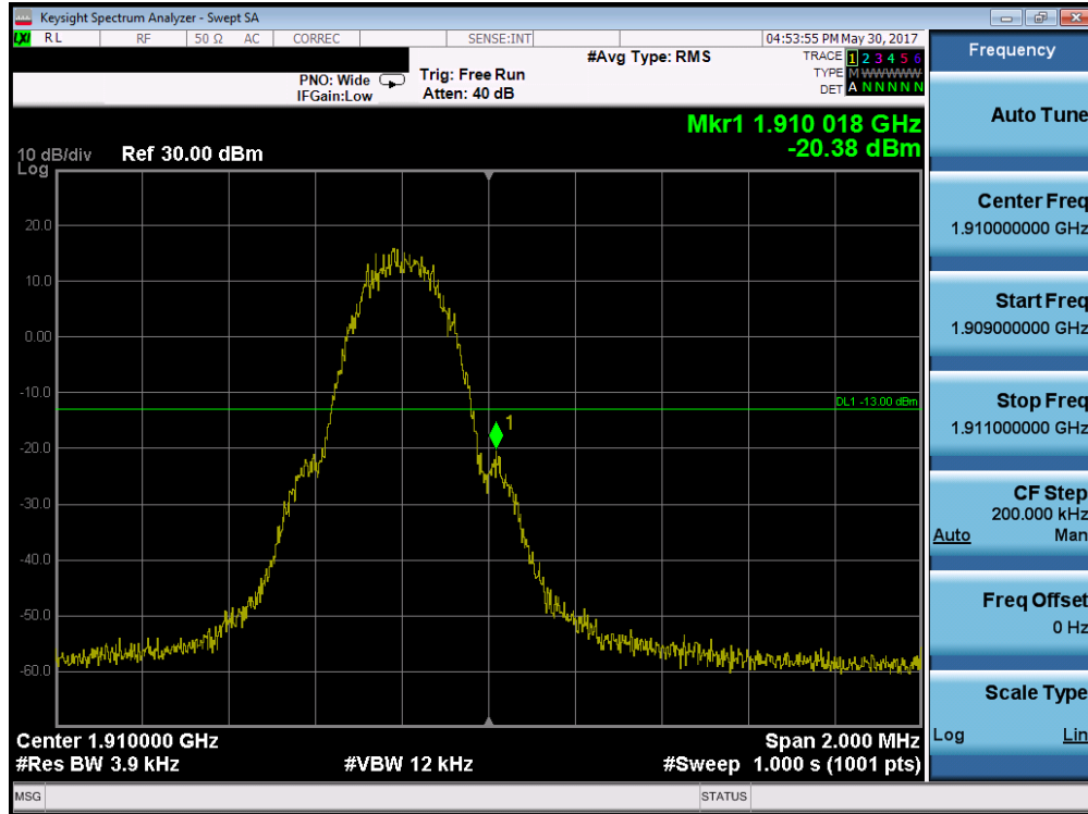
Plot 7-58. Band Edge Plot (PCS GPRS Mode – Ch. 810)
