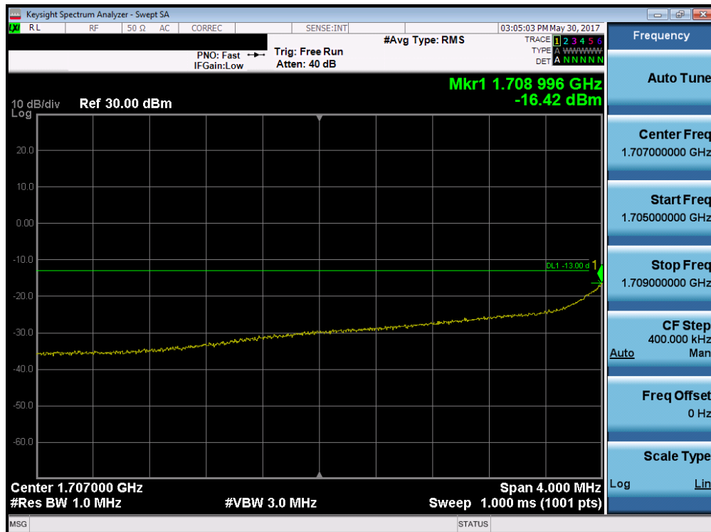
Plot 7-63. 4MHz Span Plot (AWS WCDMA Mode – Ch. 1312)
