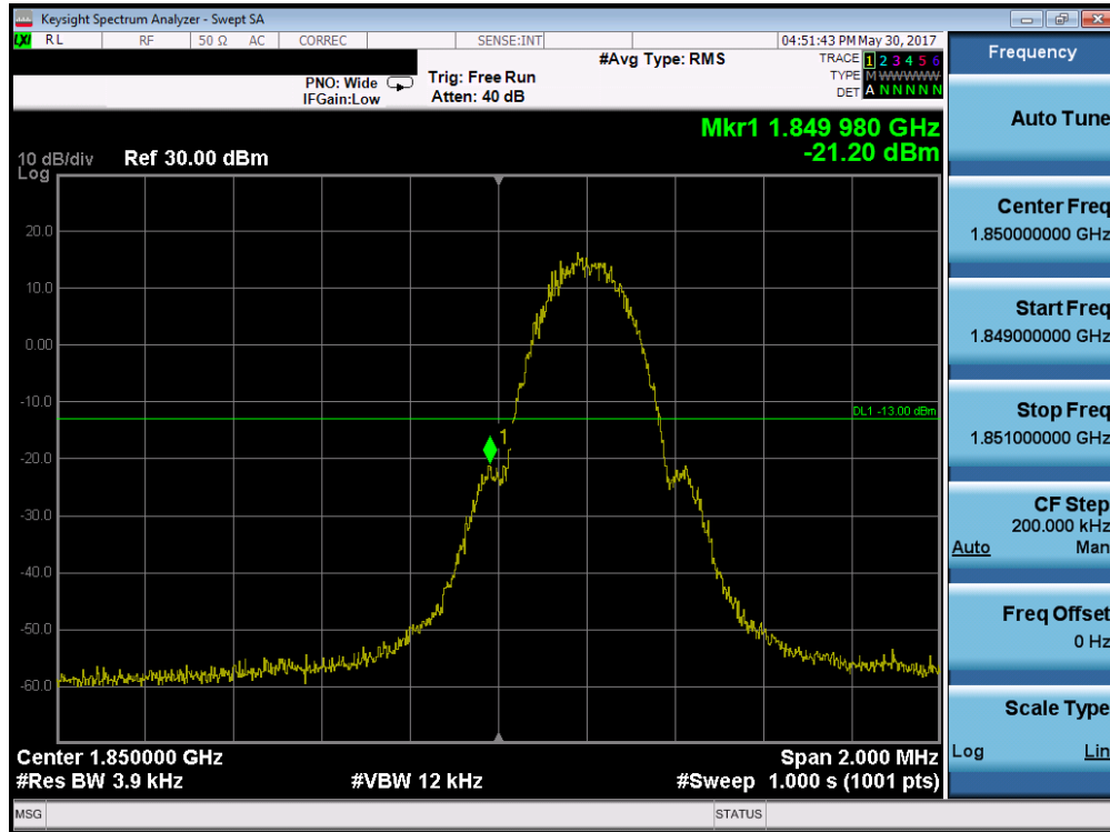
Plot 7-56. Band Edge Plot (PCS GPRS Mode – Ch. 512)
