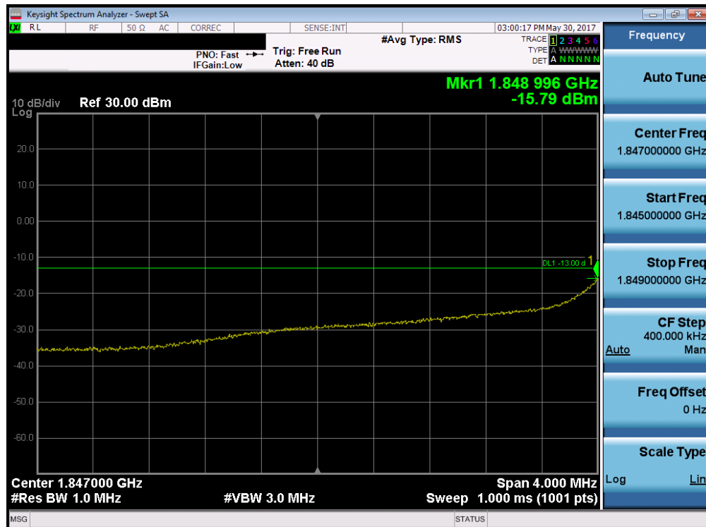
Plot 7-67. 4MHz Span Plot (PCS WCDMA Mode – Ch. 9262)
