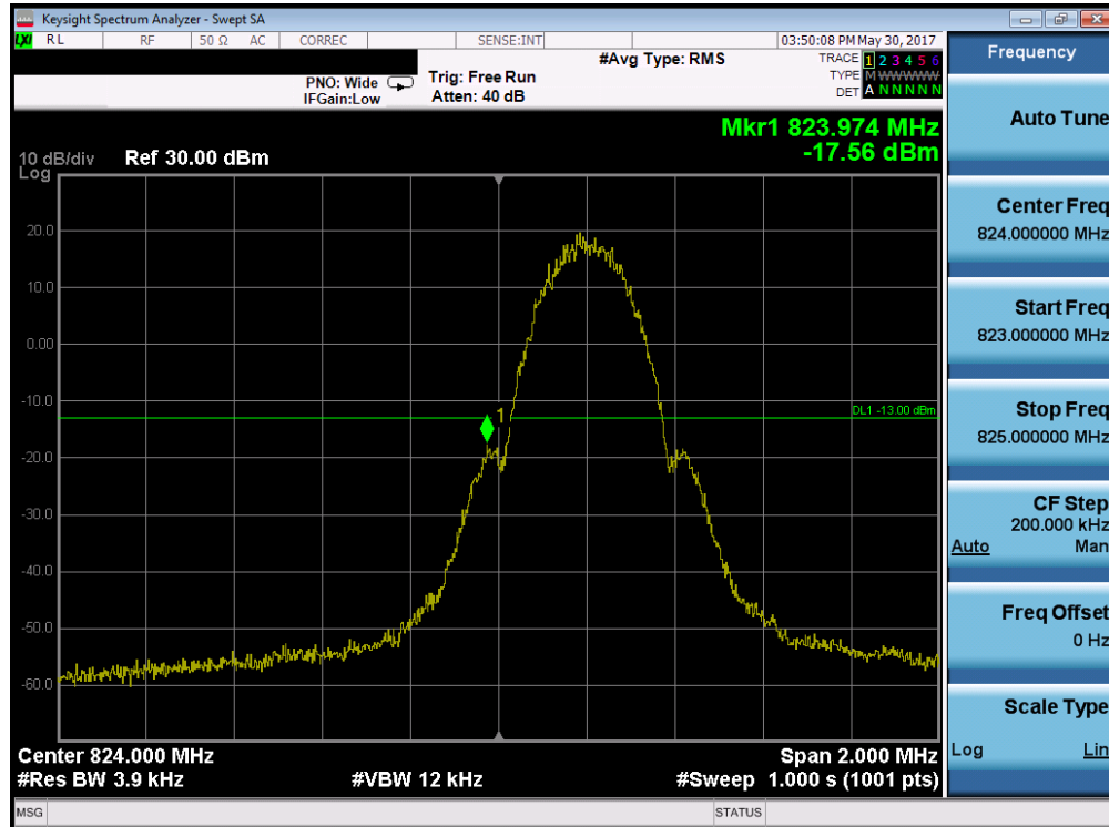
Plot 7-54. Band Edge Plot (Cellular GPRS Mode – Ch. 128)
