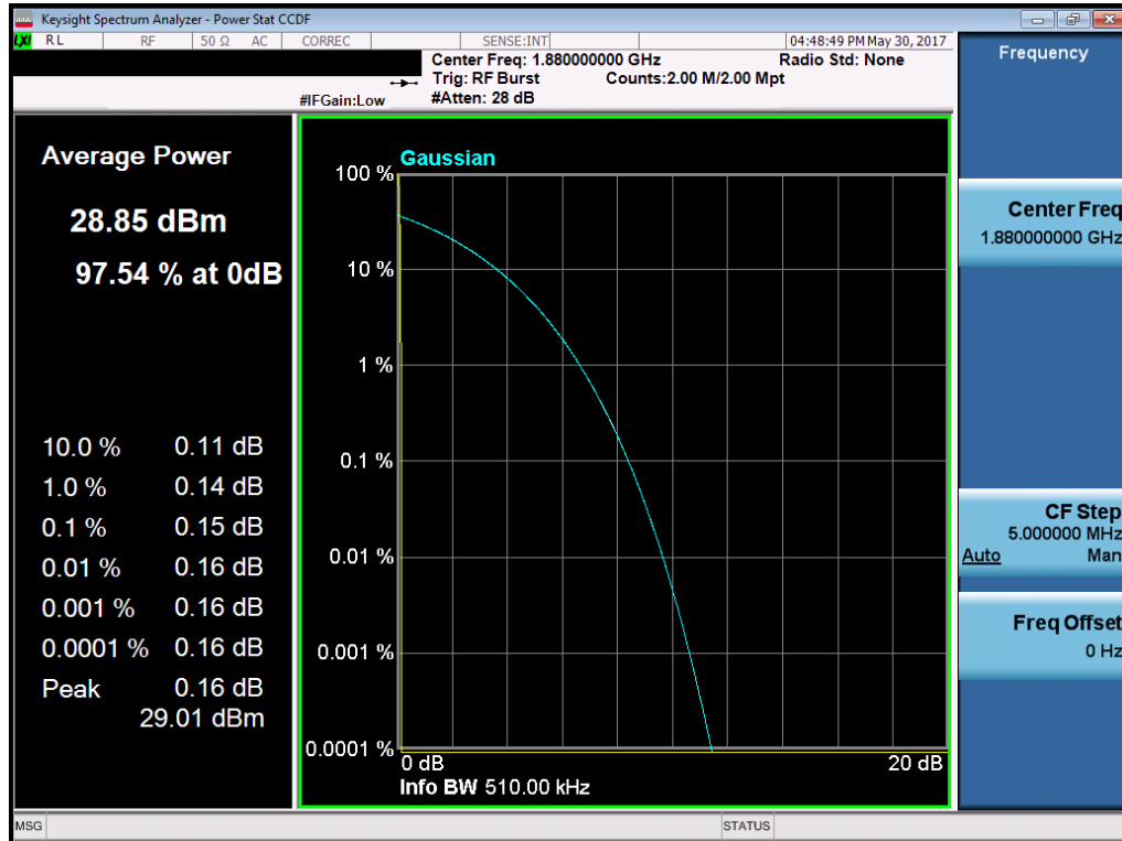
Plot 7-70. Peak-Average Ratio Plot (PCS GPRS Mode – Ch. 661)
