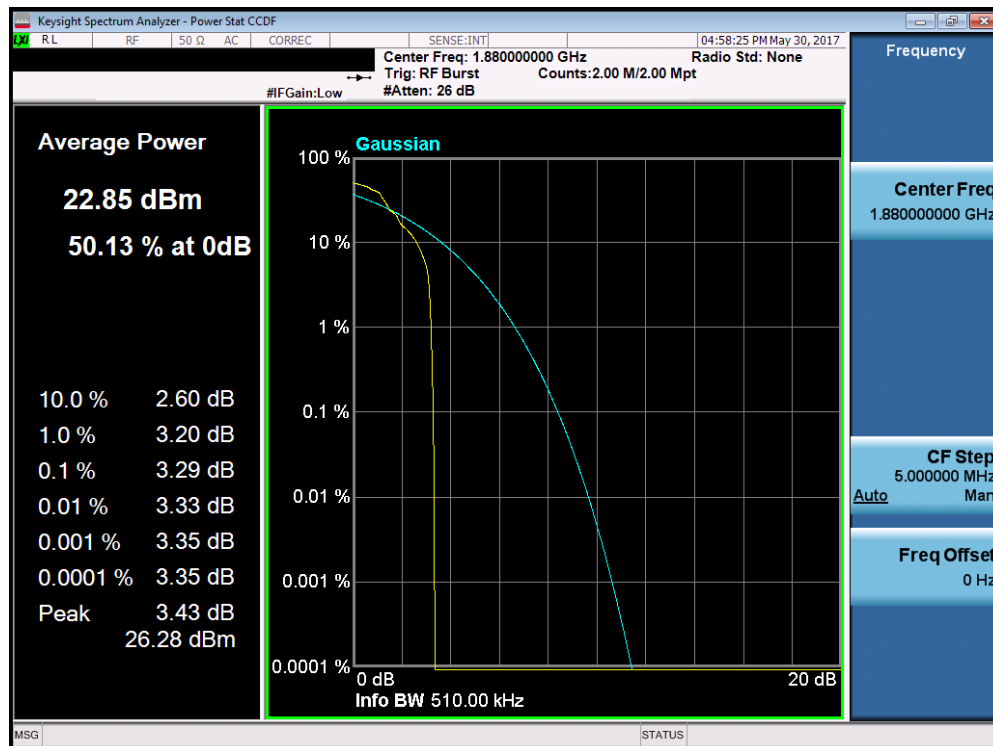
Plot 7-71. Peak-Average Ratio Plot (EDGE1900 Mode – Ch. 661)
