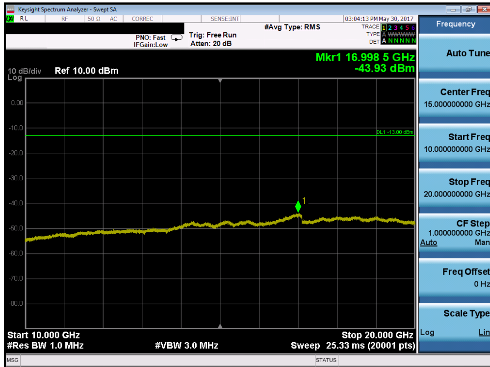
Plot 7-41. Conducted Spurious Plot (AWS WCDMA Mode – Ch. 1413)
