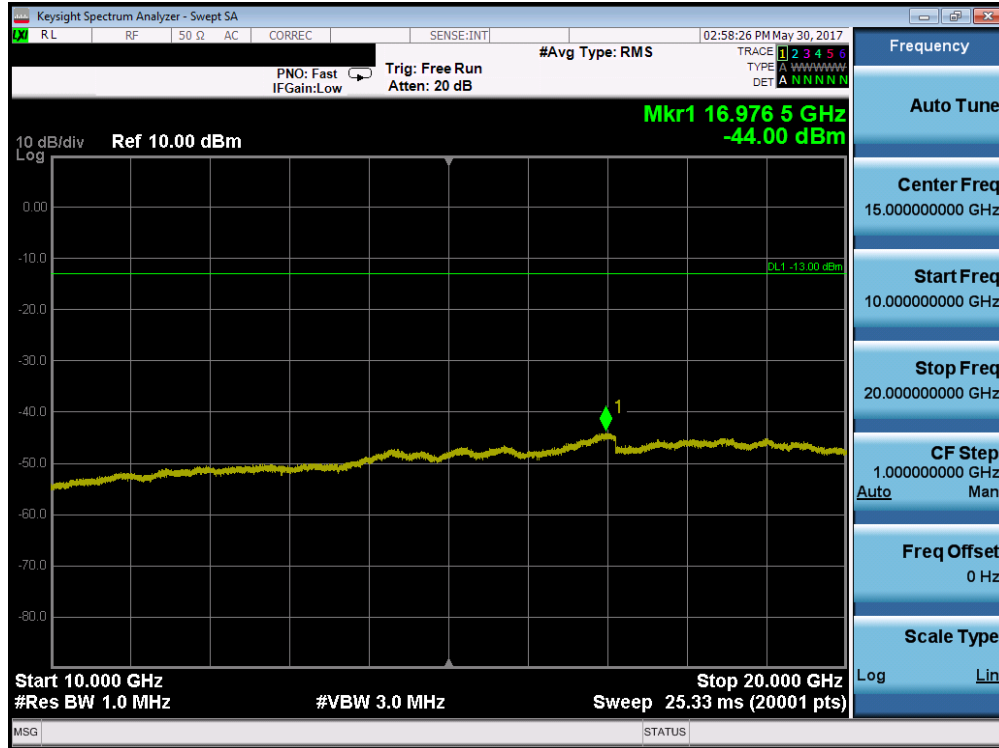
Plot 7-50. Conducted Spurious Plot (PCS WCDMA Mode – Ch. 9400)
