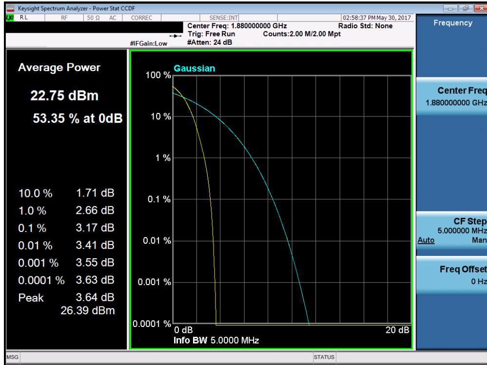
Plot 7-72. Peak-Average Ratio Plot (PCS WCDMA Mode – Ch. 9400)
