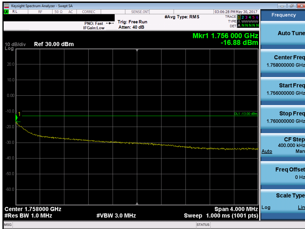
Plot 7-65. 4MHz Span Plot (AWS WCDMA Mode – Ch. 1513)
