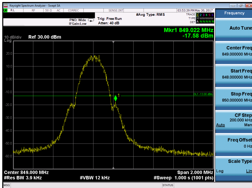
Plot 7-55. Band Edge Plot (Cellular GPRS Mode – Ch. 251)
