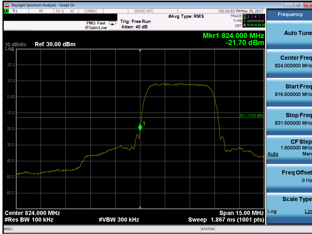
Plot 7-60. Band Edge Plot (Cellular WCDMA Mode – Ch. 4132)
