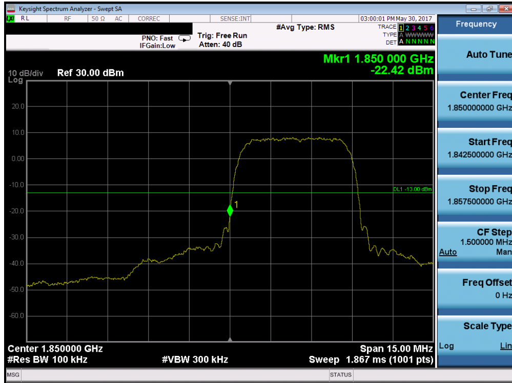
Plot 7-66. Band Edge Plot (PCS WCDMA Mode – Ch. 9262)
