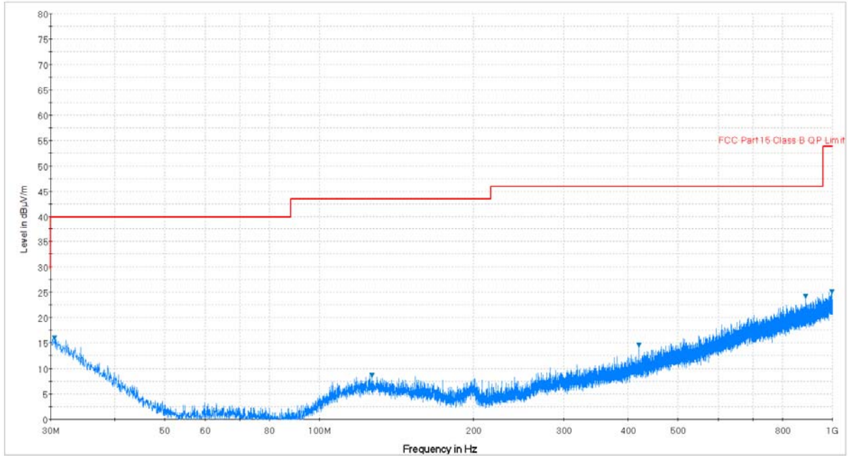
Plot 7-41. Radiated Spurious Plot below 1GHz (Pol. H)
