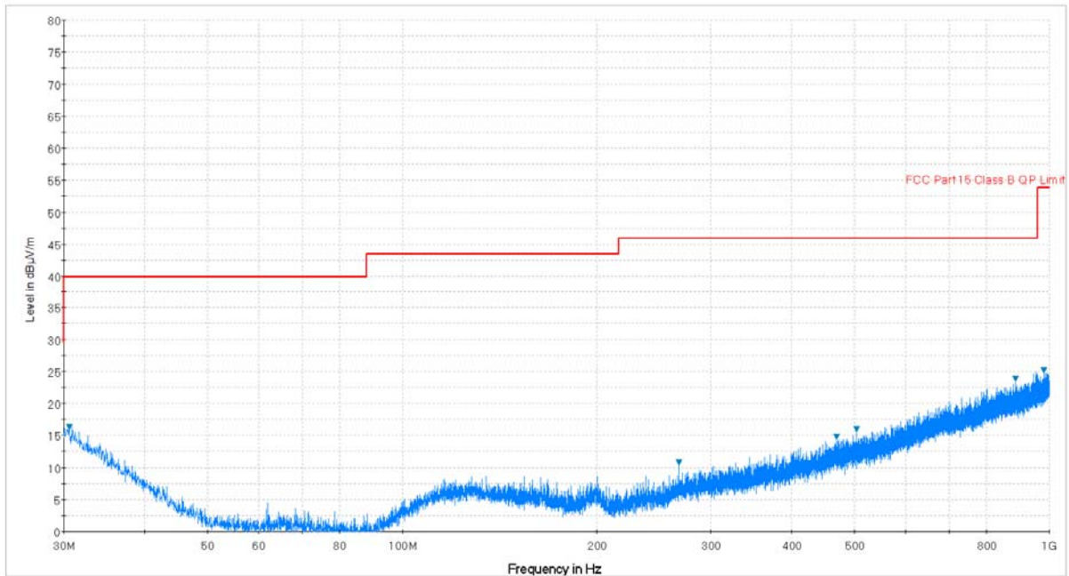
Plot 7-42. Radiated Spurious Plot below 1GHz (Pol. V)
