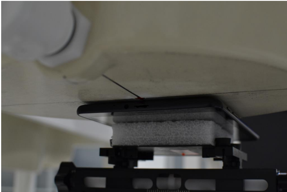
SAR Test Setup Photo 9: Back 0 mm (5 GHz WLAN and Bluetooth testing)
