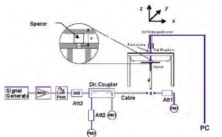
Figure 11-1 System Verification Setup Diagram
