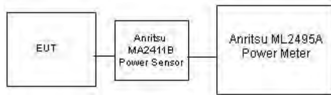
Figure 10-3 Power Measurement Setup
