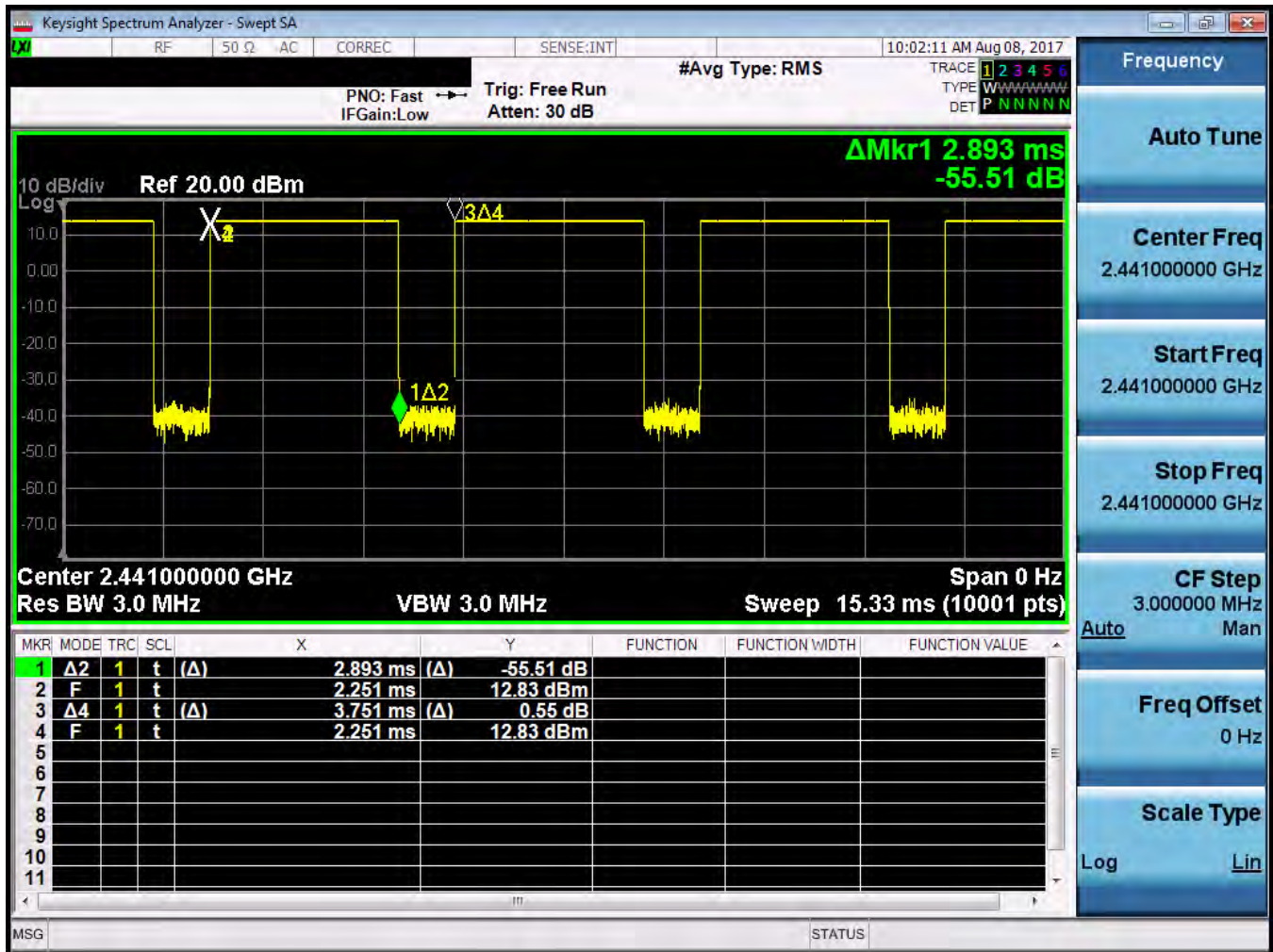
Figure 10-4 Bluetooth Transmission Plot
