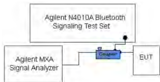
Figure 10-5 Power Measurement Setup
