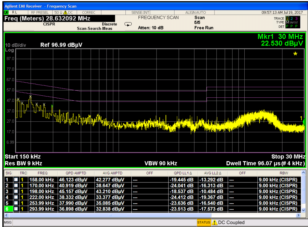
Plot 7-6. Line-Conducted Test Plot (L1)
