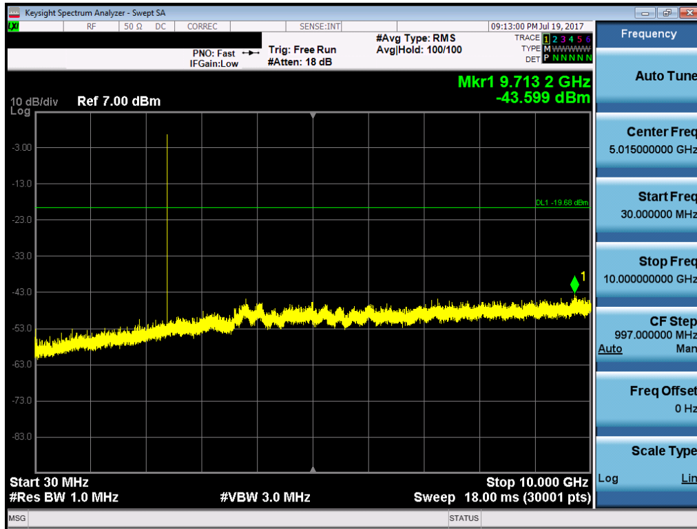
Plot 7-12. Conducted Spurious Plot (Bluetooth (LE), 1Mbps – Ch. 0)
