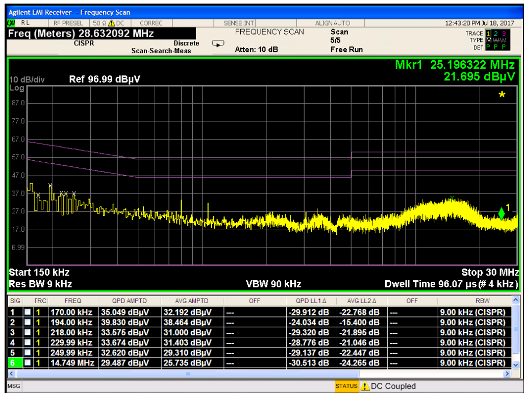
Plot 7-55. Line-Conducted Test Plot (N)
