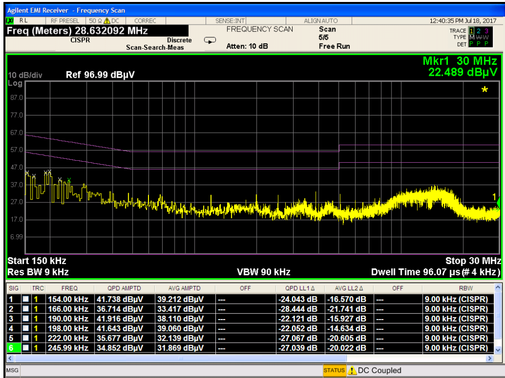
Plot 7-54. Line-Conducted Test Plot (L1)
