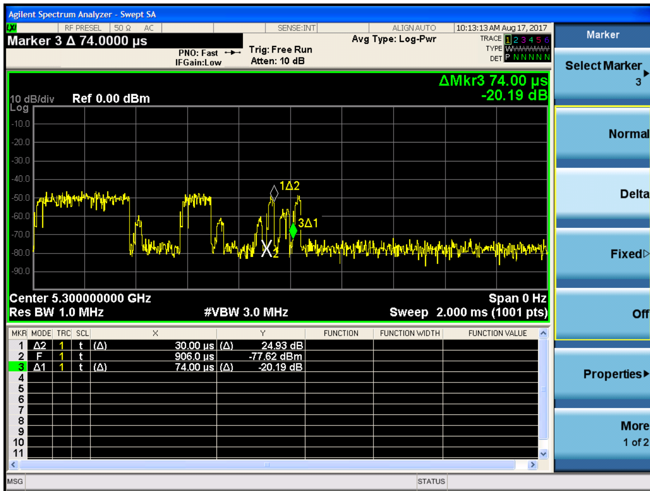
Figure 5-1. Band 2A Pulse Width & Period
