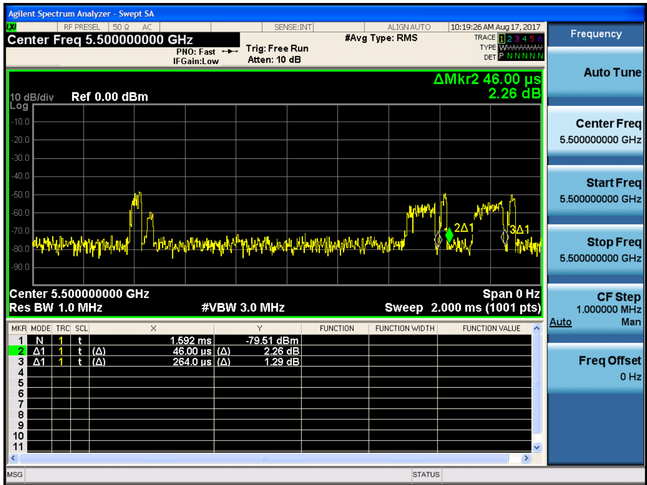
Figure 5-2. Band 2C Pulse Width & Period
