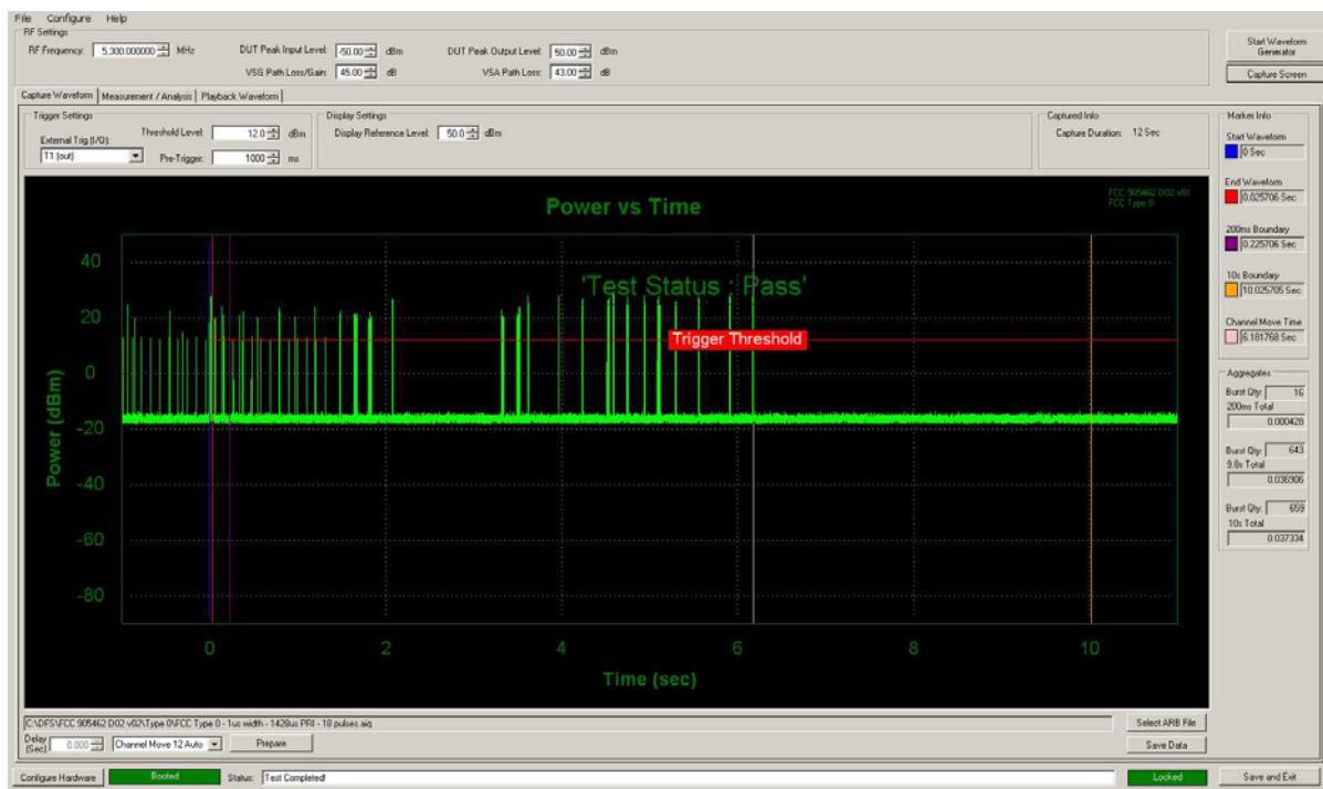
Figure 5-3. Band 2A Move Time and Aggregate Time
