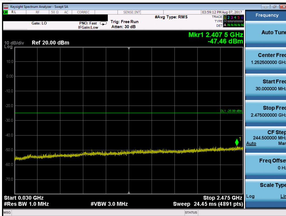
Plot 7-43. Conducted Spurious Plot (Band 38/41 – 10.0MHz QPSK – RB Size 1, RB Offset 0– Low Channel)
