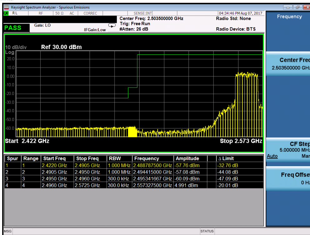
Plot 7-72. Lower ACP Plot (Band 41 – 15.0MHz QPSK – RB Size 75)
