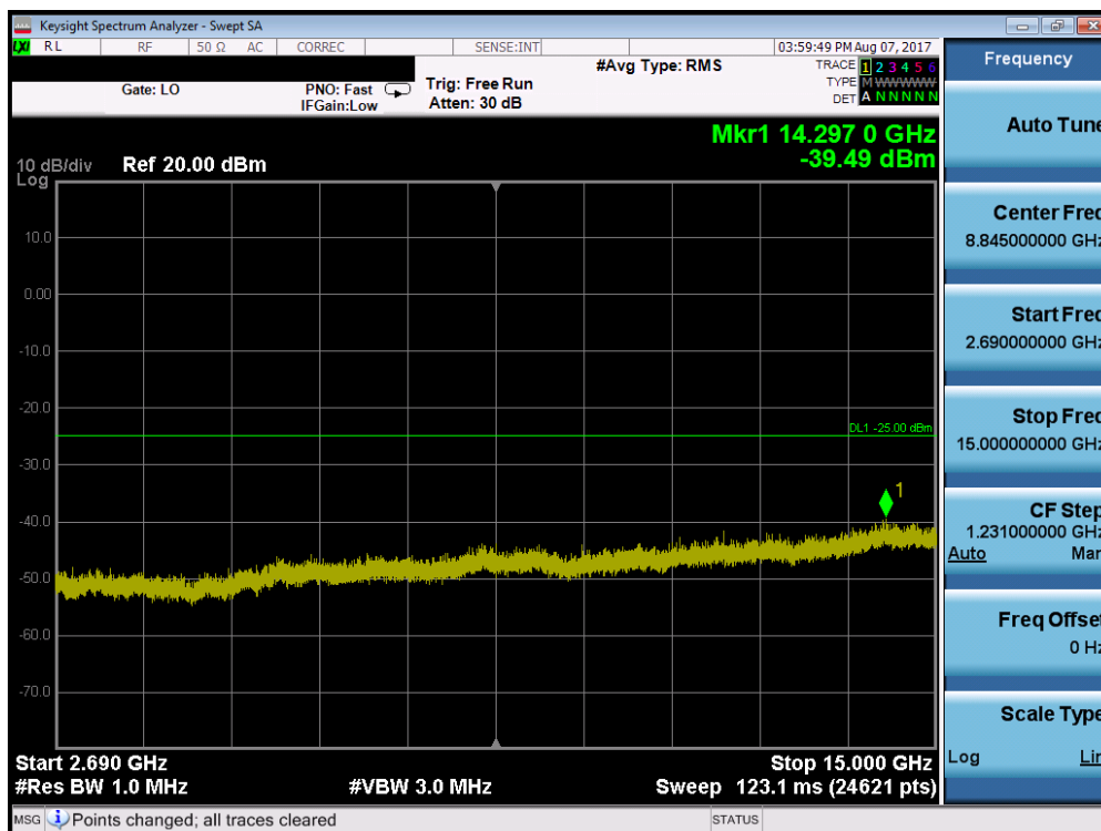
Plot 7-44. Conducted Spurious Plot (Band 38/41 – 10.0MHz QPSK – RB Size 1, RB Offset 0 – Low Channel)
