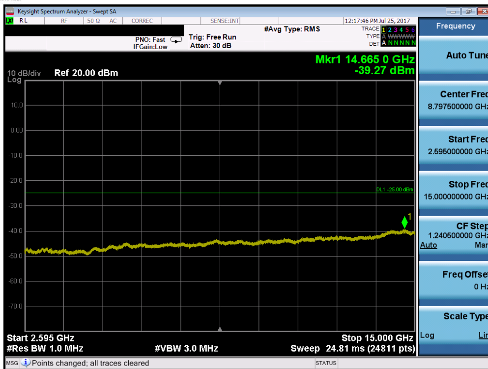
Plot 7-41. Conducted Spurious Plot (Band 7 – 5.0MHz QPSK – RB Size 1, RB Offset 0 – High Channel)
