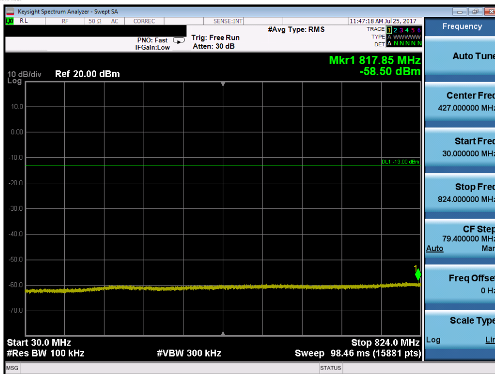
Plot 7-31. Conducted Spurious Plot (Band 5 – 3.0MHz QPSK – RB Size 1, RB Offset 0 – High Channel)
