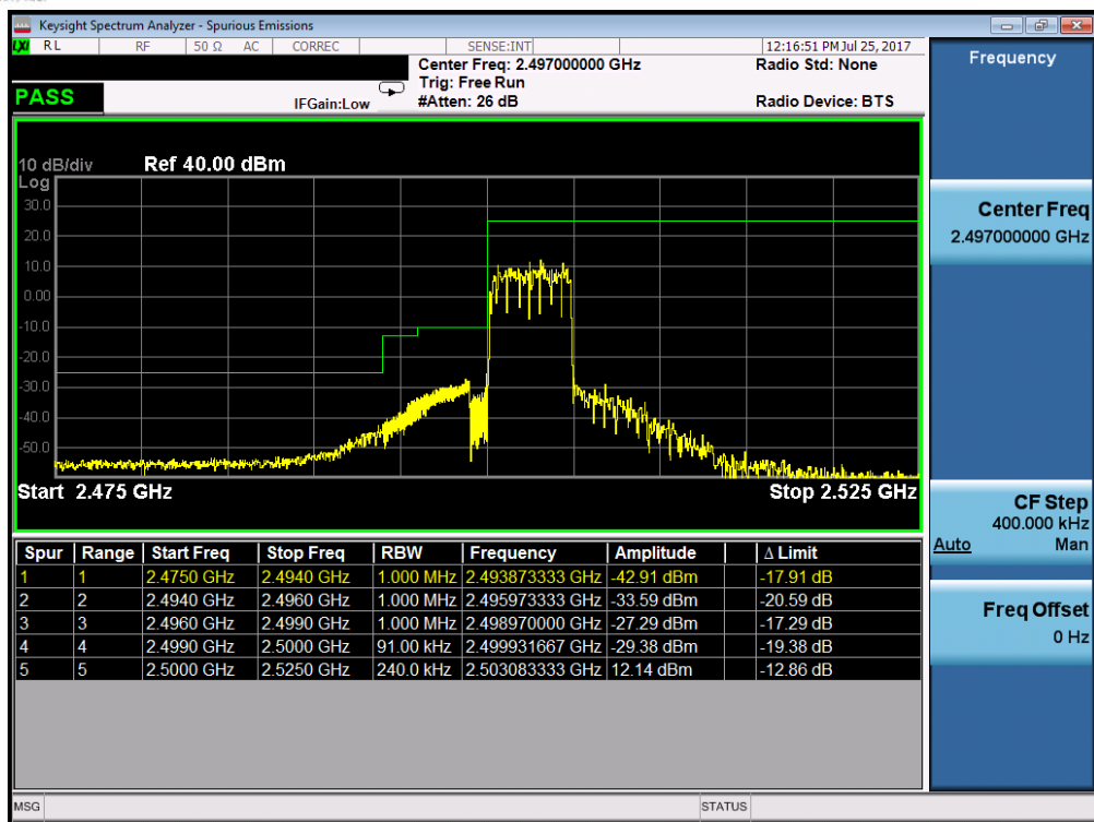
Plot 7-60. Lower ACP Plot (Band 7 – 5.0MHz QPSK – RB Size 25)
