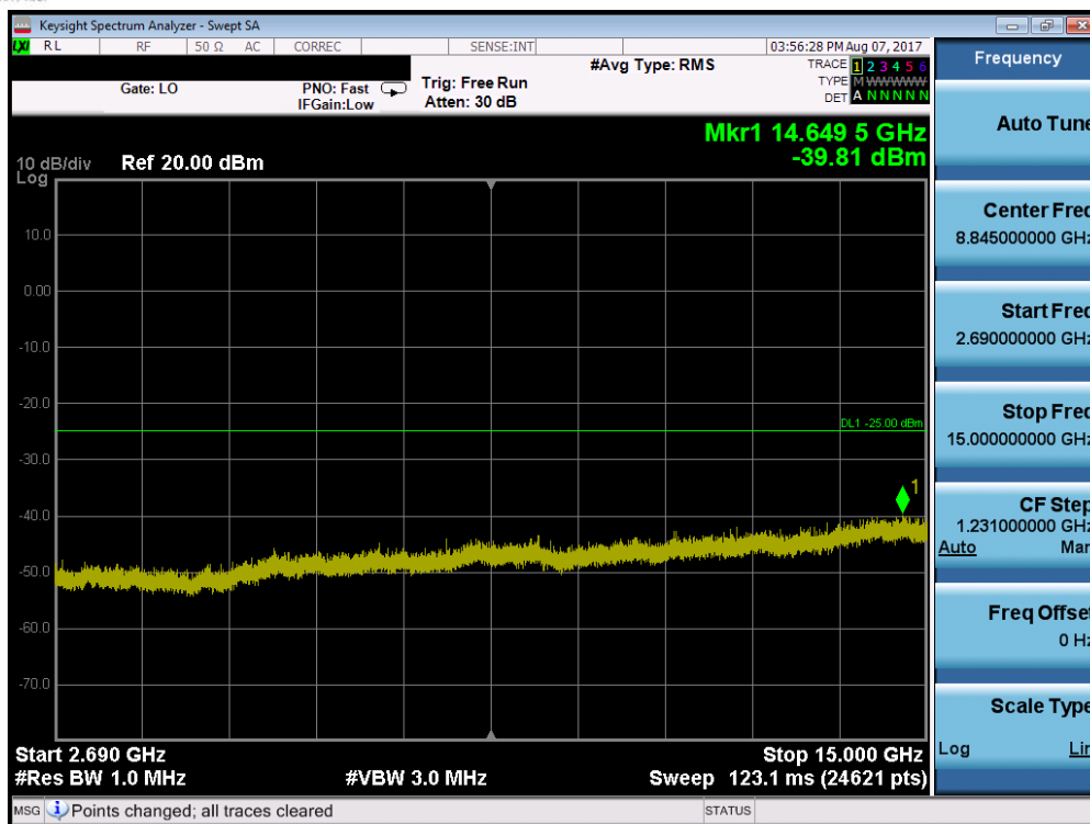
Plot 7-47. Conducted Spurious Plot (Band 38/41 – 10.0MHz QPSK – RB Size 1, RB Offset 0 – Mid Channel)
