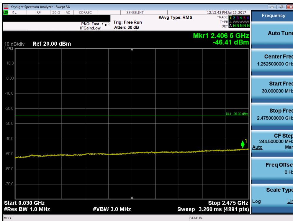
Plot 7-34. Conducted Spurious Plot (Band 7 – 5.0MHz QPSK – RB Size 1, RB Offset 0 – Low Channel)
