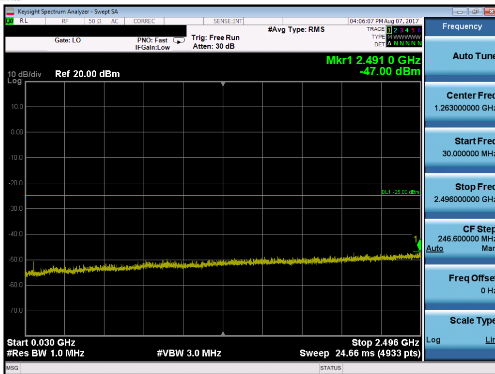
Plot 7-49. Conducted Spurious Plot (Band 38/41 – 10.0MHz QPSK – RB Size 1, RB Offset 0 – High Channel)
