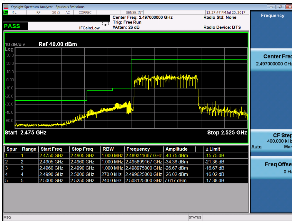
Plot 7-64. Lower ACP Plot (Band 7 – 15.0MHz QPSK – RB Size 75)
