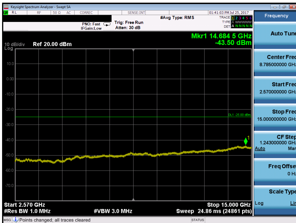
Plot 7-38. Conducted Spurious Plot (Band 7 – 5.0MHz QPSK – RB Size 1, RB Offset 0 – Mid Channel)
