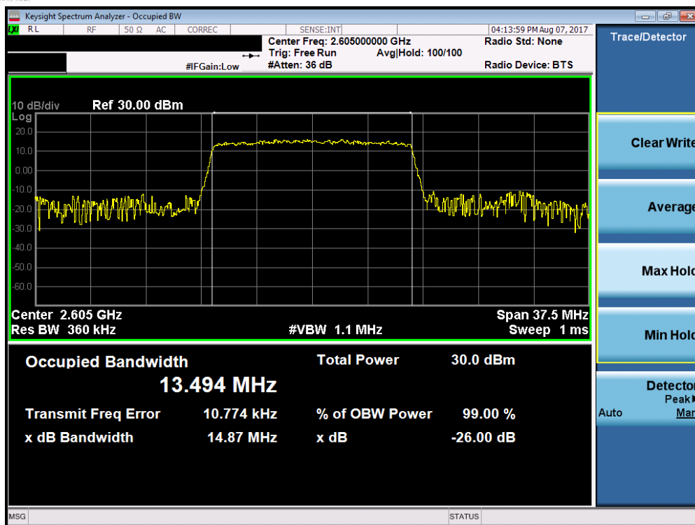
Plot 7-21. Occupied Bandwidth Plot (Band 38/41 – 15.0MHz QPSK – RB Size 75)
