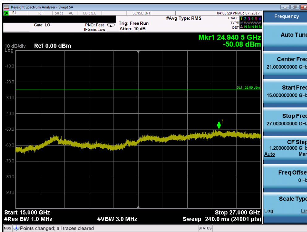
Plot 7-45. Conducted Spurious Plot (Band 38/41 – 10.0MHz QPSK – RB Size 1, RB Offset 0 – Low Channel)
