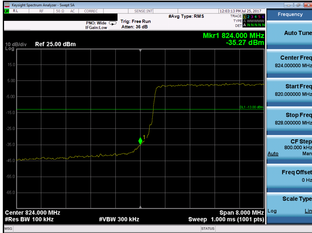
Plot 7-58. Lower Band Edge Plot (Band 5 - 10.0MHz QPSK - RB Size 50)
