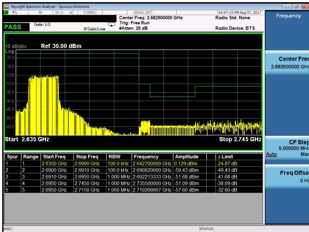
Plot 7-73. Upper ACP Plot (Band 41 – 15.0MHz QPSK – RB Size 75)
