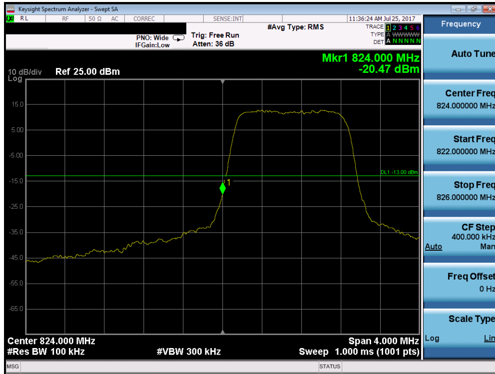
Plot 7-52. Lower Band Edge Plot (Band 5 – 1.4MHz QPSK – RB Size 6)
