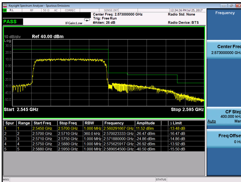
Plot 7-67. Upper ACP Plot (Band 7 – 20.0MHz QPSK – RB Size 100)
