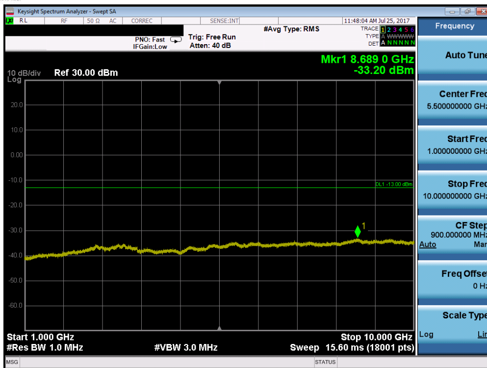
Plot 7-33. Conducted Spurious Plot (Band 5 – 3.0MHz QPSK – RB Size 1, RB Offset 0 – High Channel)
