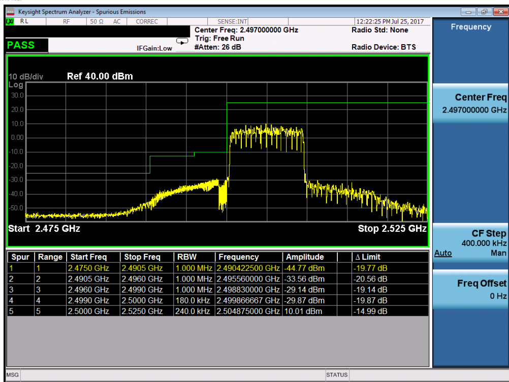
Plot 7-62. Lower ACP Plot (Band 7 – 10.0MHz QPSK – RB Size 50)
