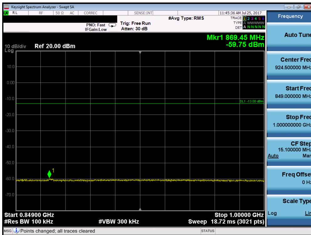
Plot 7-26. Conducted Spurious Plot (Band 5 – 3.0MHz QPSK – RB Size 1, RB Offset 0 – Low Channel)
