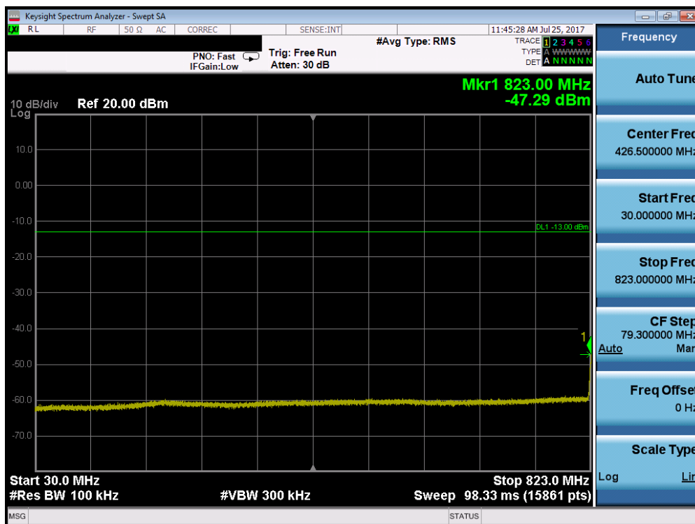
Plot 7-25. Conducted Spurious Plot (Band 5 – 3.0MHz QPSK – RB Size 1, RB Offset 0 – Low Channel)
