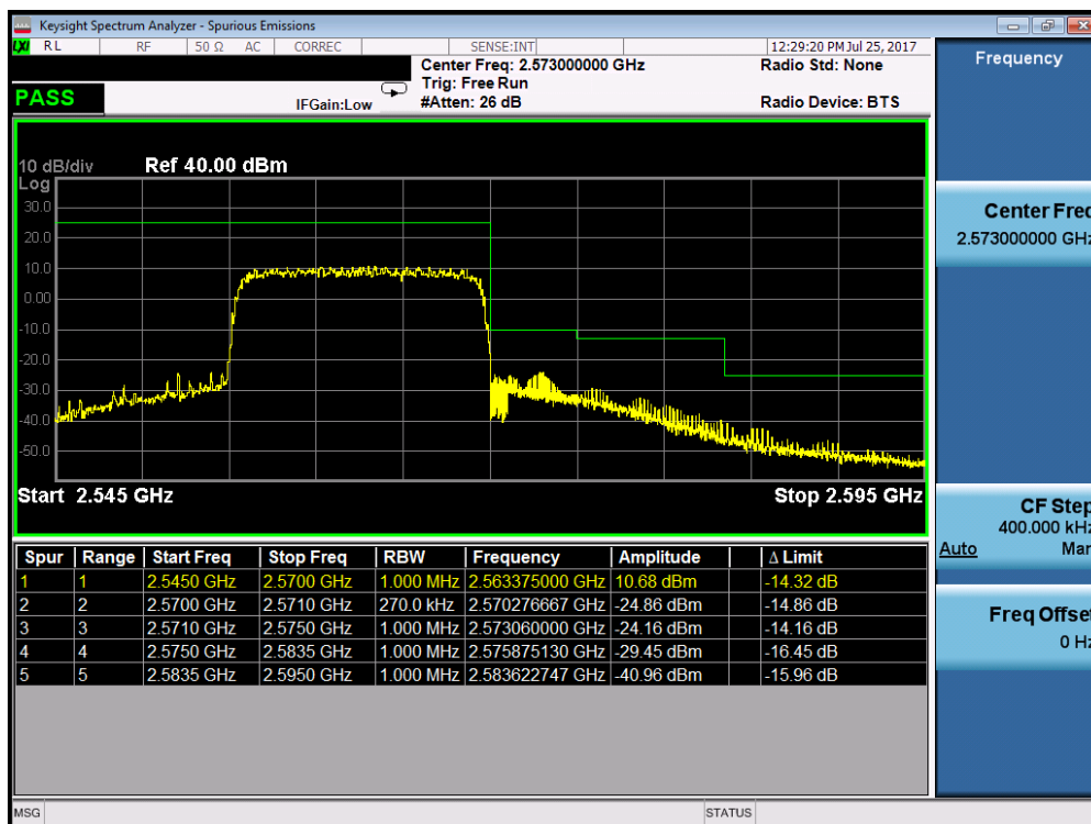
Plot 7-65. Upper ACP Plot (Band 7 – 15.0MHz QPSK – RB Size 75)
