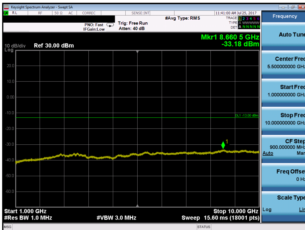
Plot 7-30. Conducted Spurious Plot (Band 5 – 3.0MHz QPSK – RB Size 1, RB Offset 0 – Mid Channel)
