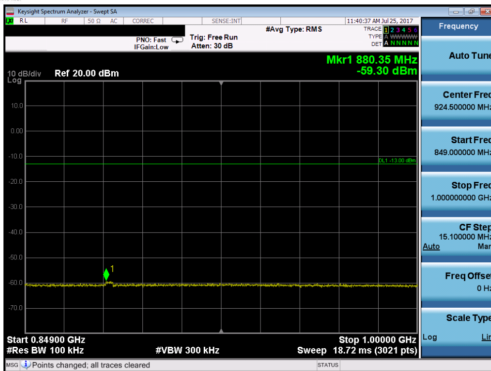
Plot 7-29. Conducted Spurious Plot (Band 5 – 3.0MHz QPSK – RB Size 1, RB Offset 0 – Mid Channel)
