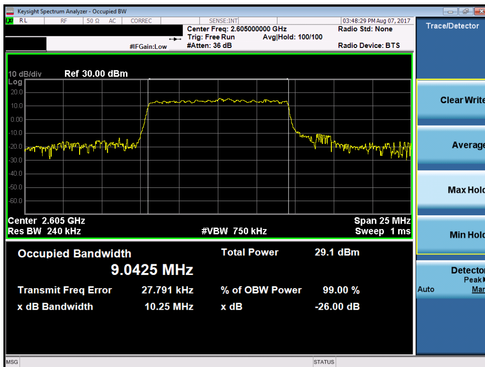
Plot 7-20. Occupied Bandwidth Plot (Band 38/41 – 10.0MHz 16-QAM – RB Size 50)
