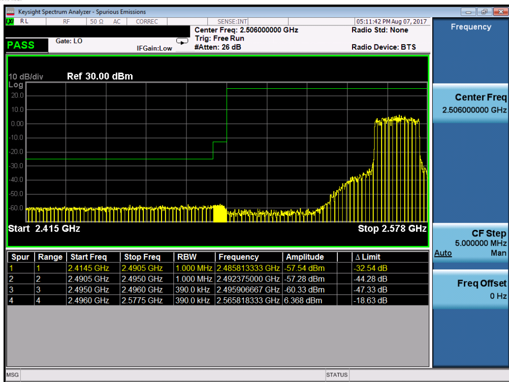
Plot 7-74. Lower ACP Plot (Band 41 – 20.0MHz QPSK – RB Size 100)
