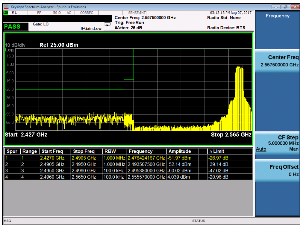
Plot 7-68. Lower ACP Plot (Band 41 – 5.0MHz QPSK – RB Size 25)
