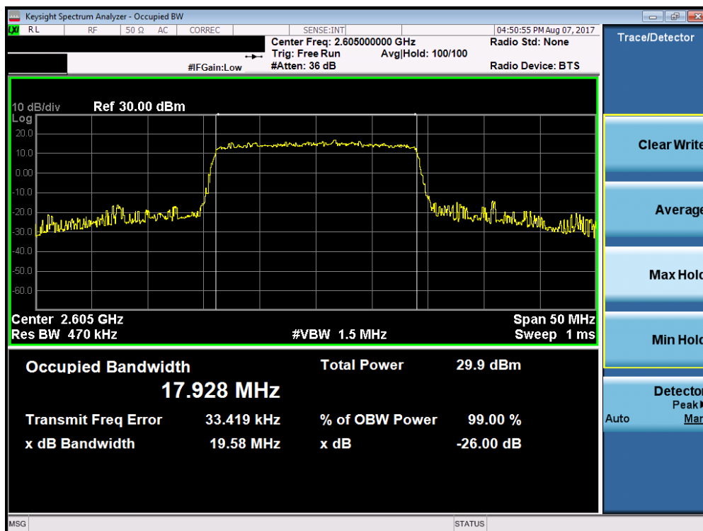
Plot 7-24. Occupied Bandwidth Plot (Band 38/41 – 20.0MHz 16-QAM – RB Size 100)
