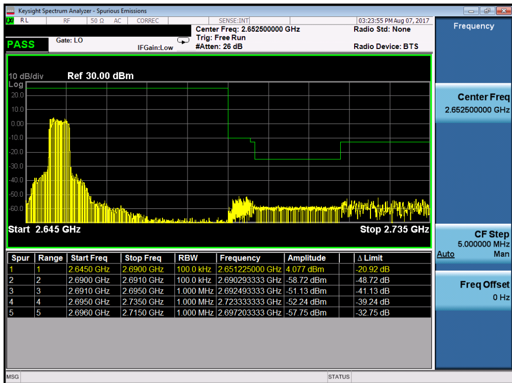
Plot 7-69. Upper ACP Plot (Band 41 – 5.0MHz QPSK – RB Size 25)
