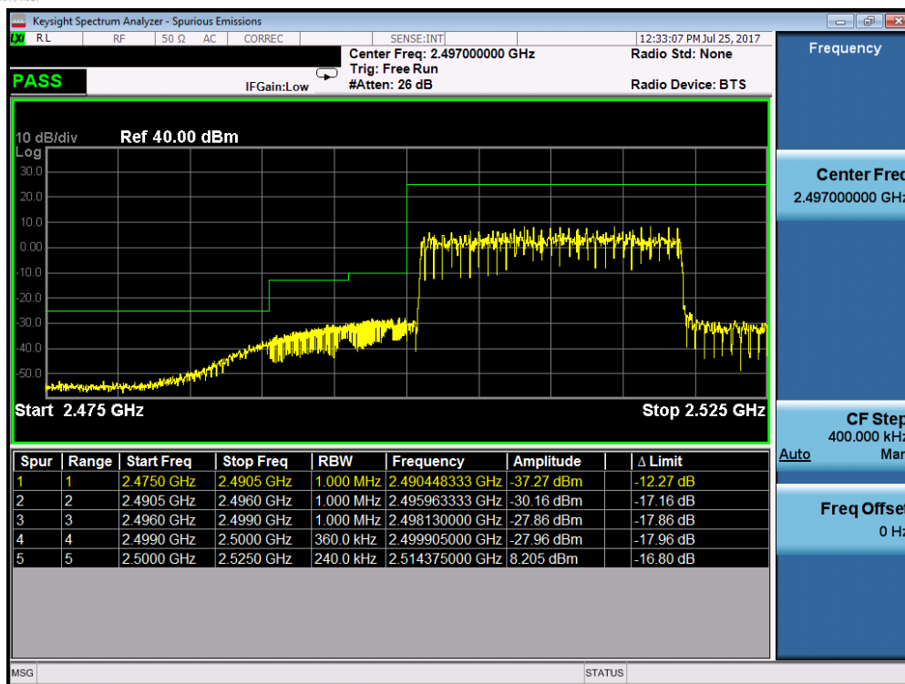
Plot 7-66. Lower ACP Plot (Band 7 – 20.0MHz QPSK – RB Size 100)
