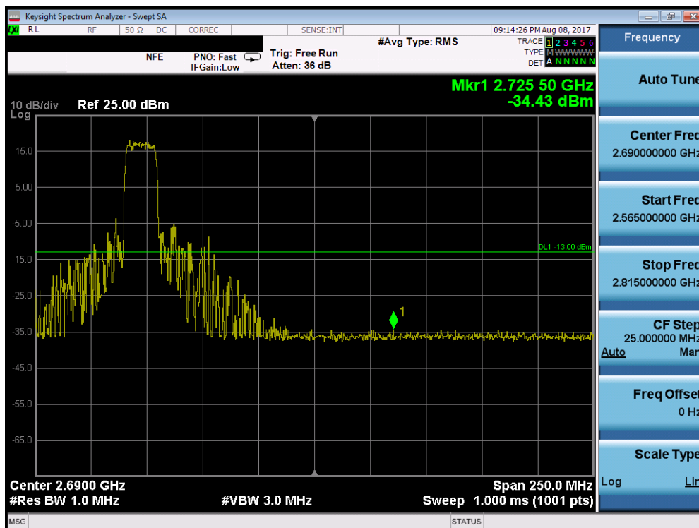
Plot 7-81. Lower Band Edge Plot (Band 38 – 15.0MHz QPSK – RB Size 6)
