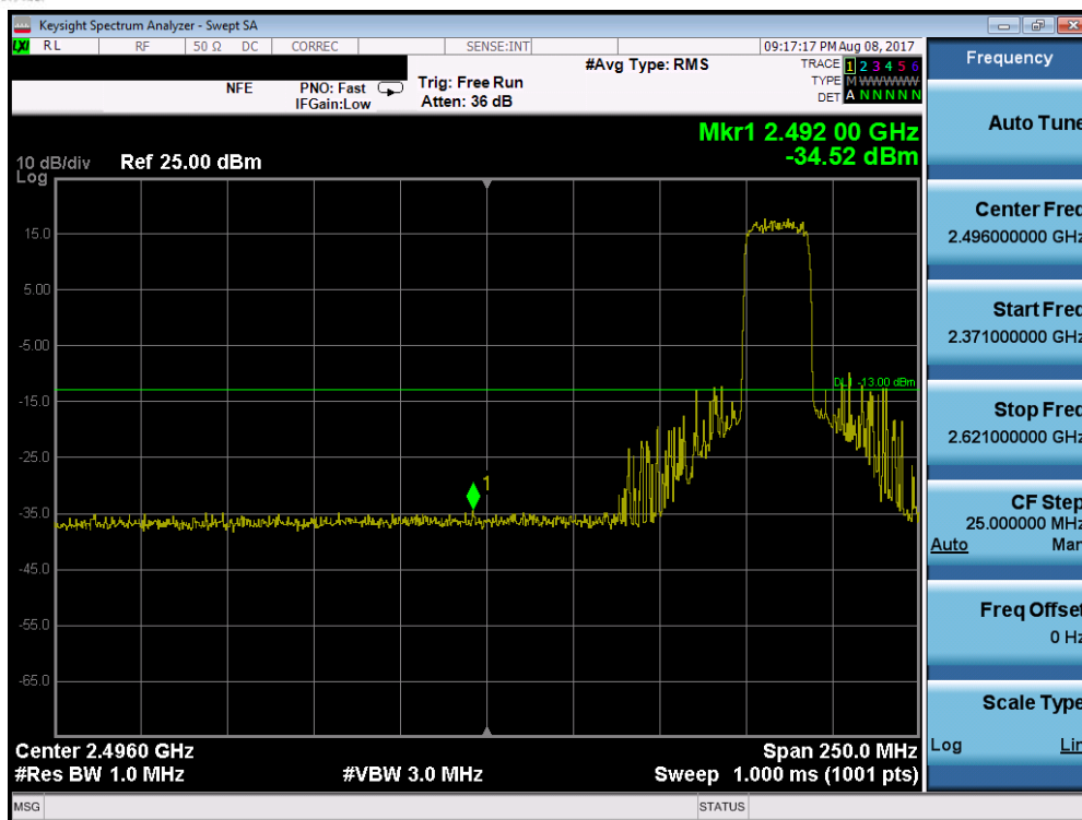
Plot 7-82. Lower Band Edge Plot (Band 38 – 200.MHz QPSK – RB Size 6)
