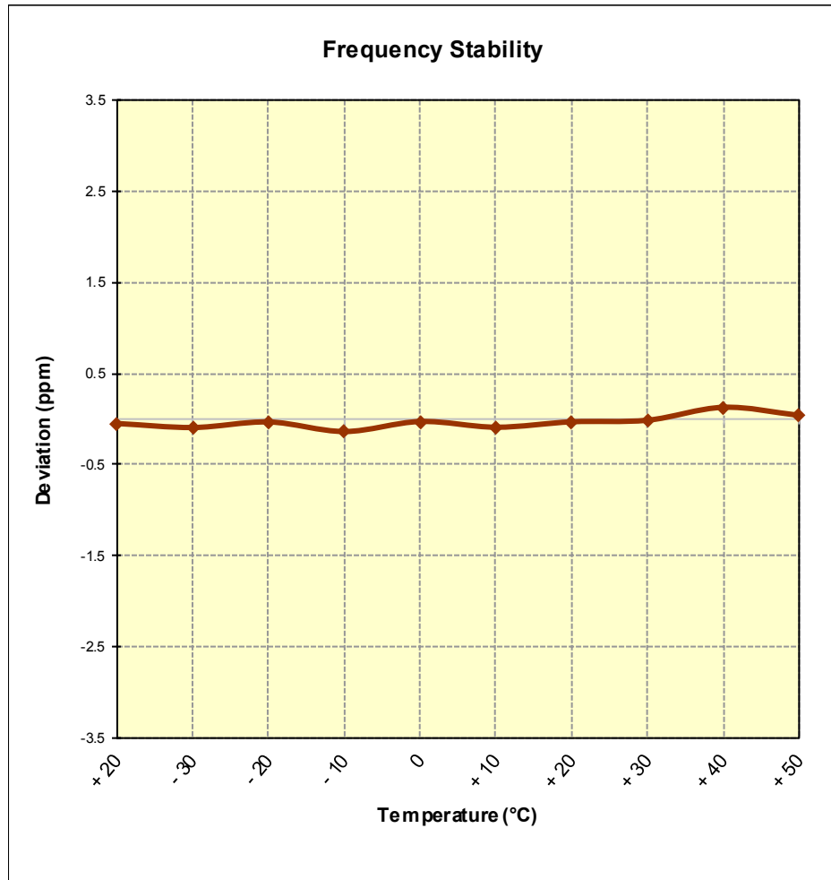
Figure 7-9. Frequency Stability Graph (Band 38/41)
