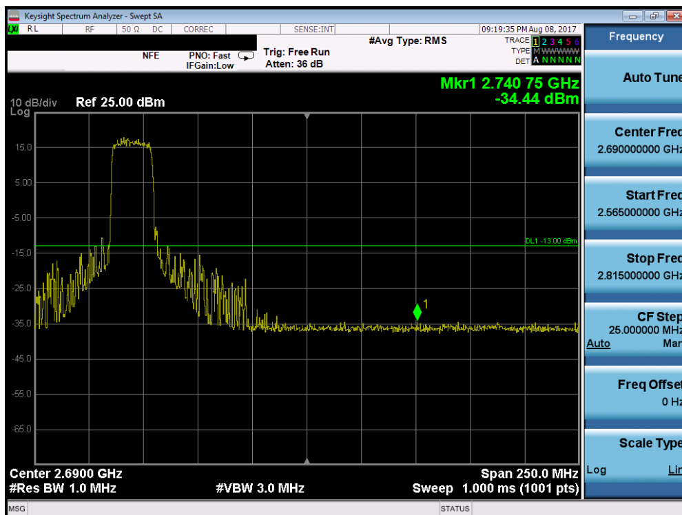
Plot 7-83. Lower Band Edge Plot (Band 38 – 20.0MHz QPSK – RB Size 6)
