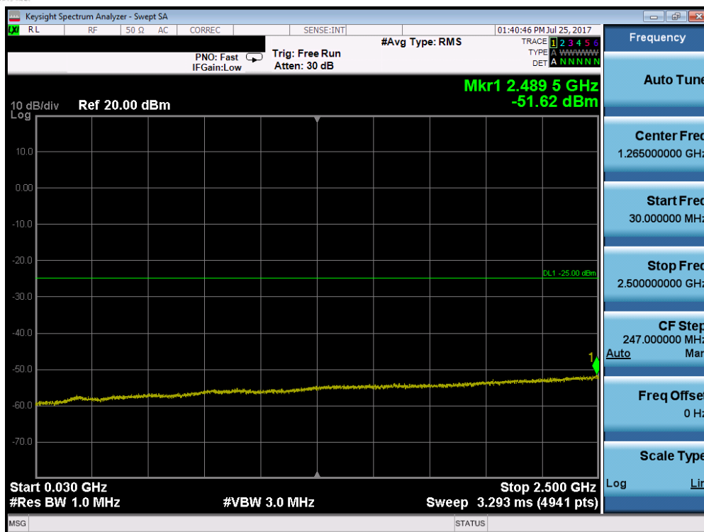
Plot 7-37. Conducted Spurious Plot (Band 7 – 5.0MHz QPSK – RB Size 1, RB Offset 0 – Mid Channel)
