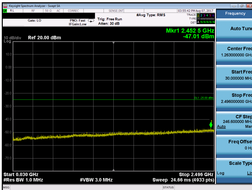
Plot 7-46. Conducted Spurious Plot (Band 38/41 – 10.0MHz QPSK – RB Size 1, RB Offset 0 – Mid Channel)
