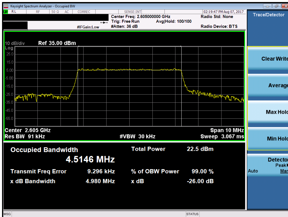
Plot 7-18. Occupied Bandwidth Plot (Band 38/41 – 5.0MHz 16-QAM – RB Size 25)
