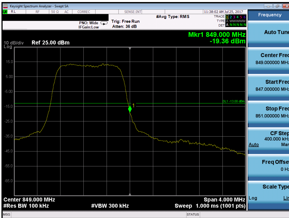
Plot 7-53. Upper Band Edge Plot (Band 5 – 1.4MHz QPSK – RB Size 6)
