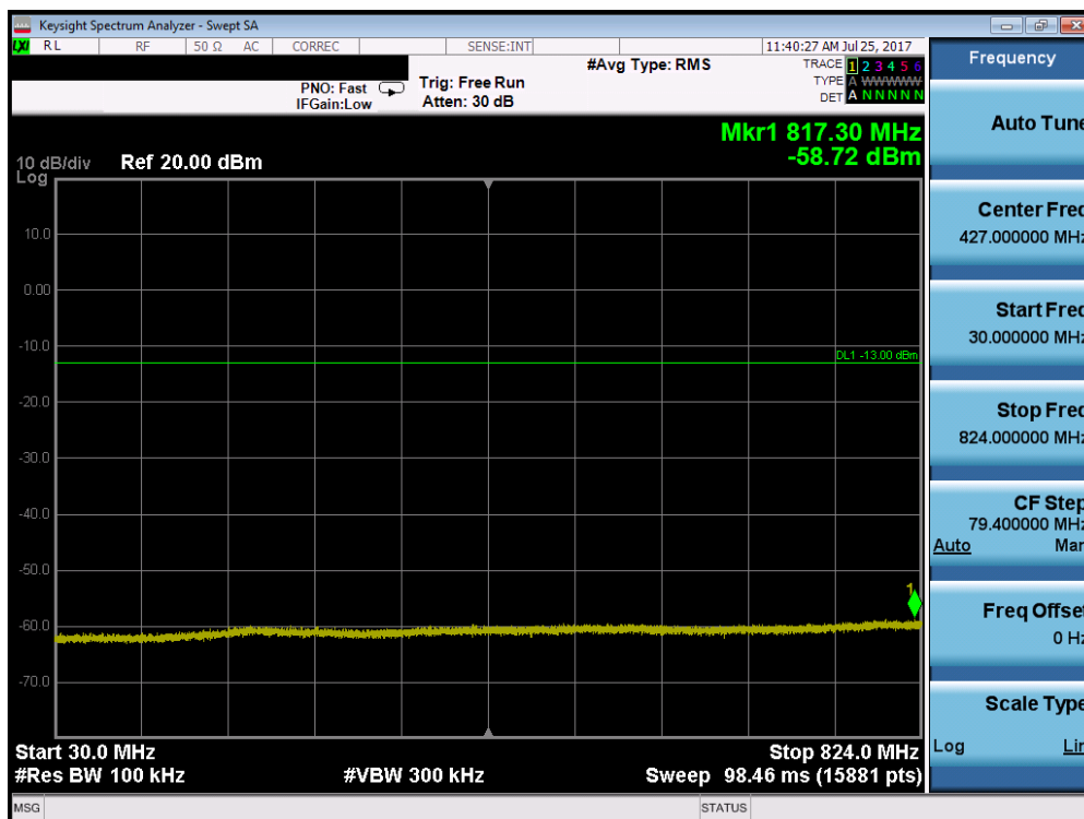
Plot 7-28. Conducted Spurious Plot (Band 5 – 3.0MHz QPSK – RB Size 1, RB Offset 0 – Mid Channel)
