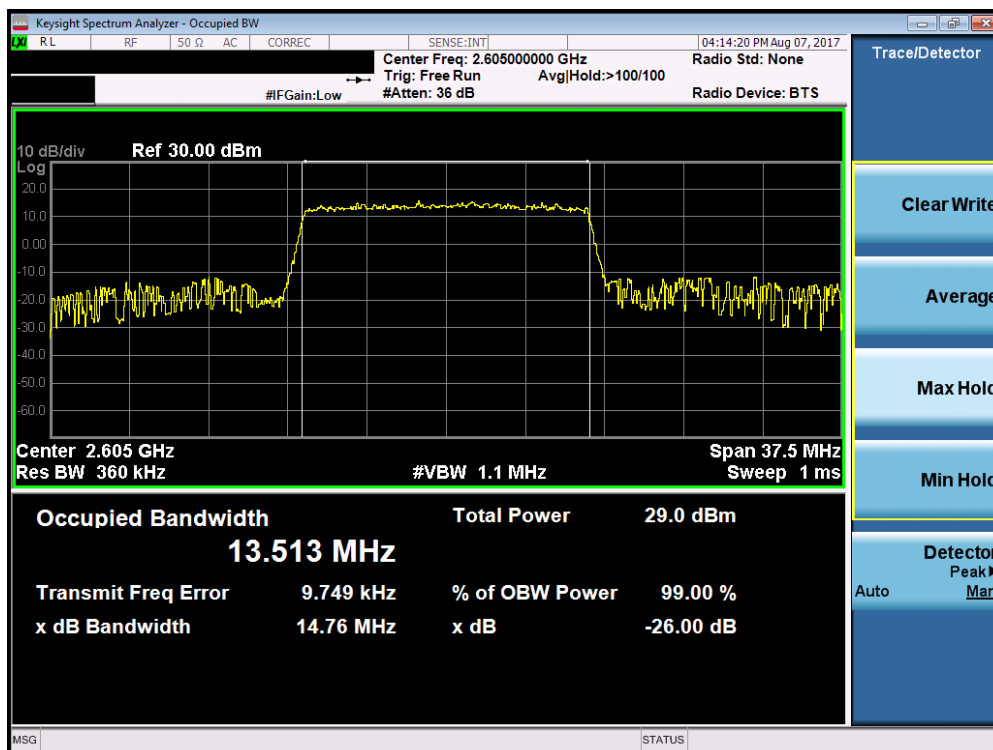
Plot 7-22. Occupied Bandwidth Plot (Band 38/41 – 15.0MHz 16-QAM – RB Size 75)
