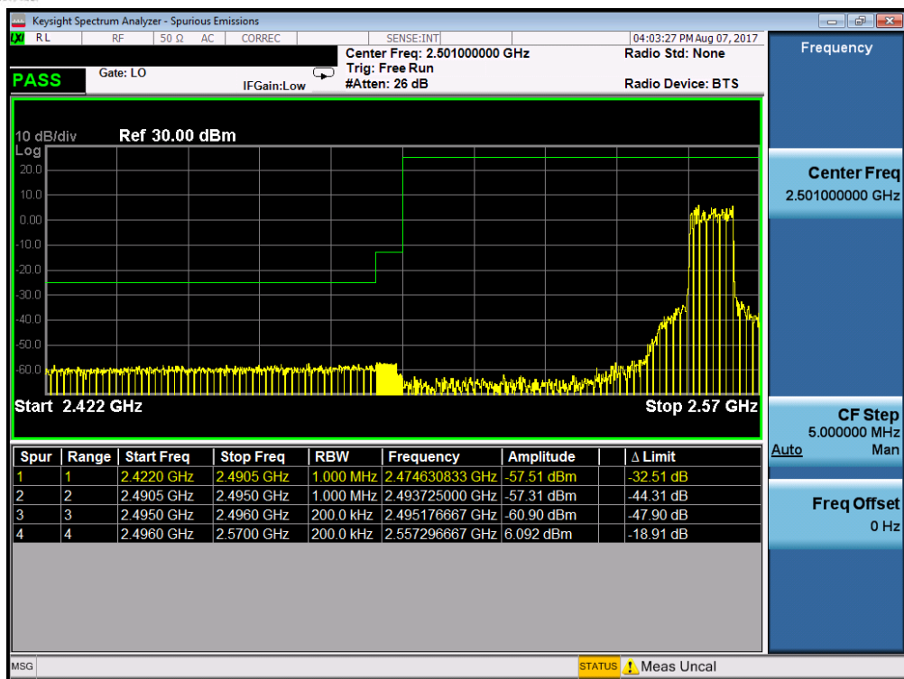
Plot 7-70. Lower ACP Plot (Band 41 – 10.0MHz QPSK – RB Size 50)
