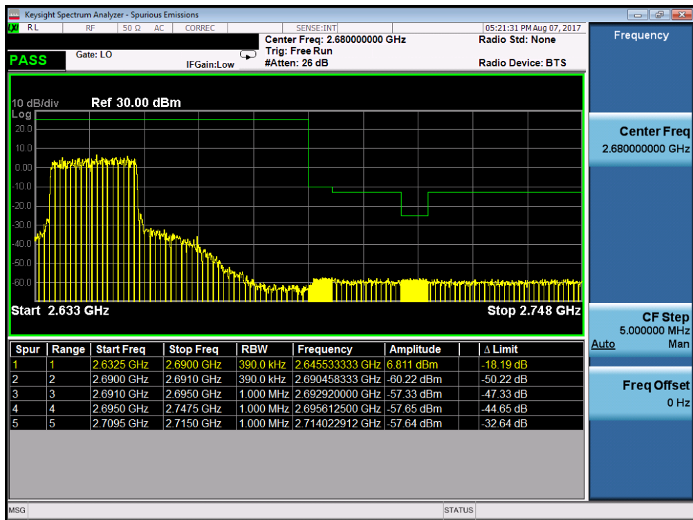
Plot 7-75. Upper ACP Plot (Band 41 – 20.0MHz QPSK – RB Size 100)
