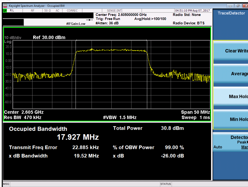
Plot 7-23. Occupied Bandwidth Plot (Band 38/41 – 20.0MHz QPSK – RB Size 100)
