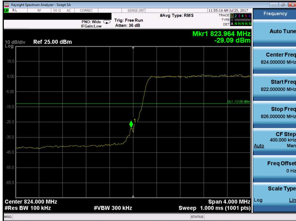
Plot 7-56. Lower Band Edge Plot (Band 5 - 5.0MHz QPSK - RB Size 25)
