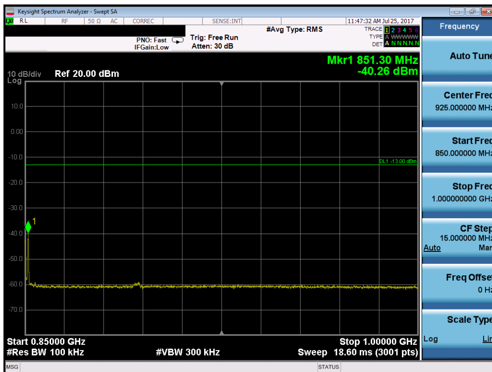
Plot 7-32. Conducted Spurious Plot (Band 5 – 3.0MHz QPSK – RB Size 1, RB Offset 0 – High Channel)
