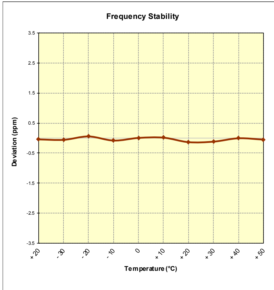
Figure 7-8. Frequency Stability Graph (Band 7)
