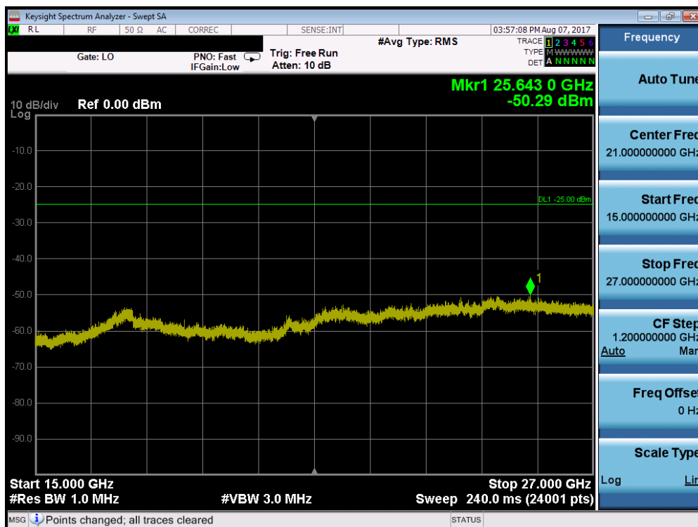
Plot 7-48. Conducted Spurious Plot (Band 38/41 – 10.0MHz QPSK – RB Size 1, RB Offset 0 – Mid Channel)
