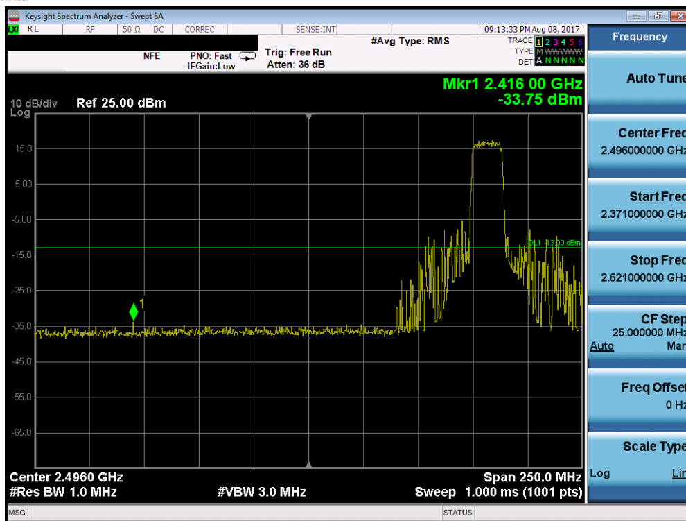
Plot 7-80. Lower Band Edge Plot (Band 38 – 15.0MHz QPSK – RB Size 6)
