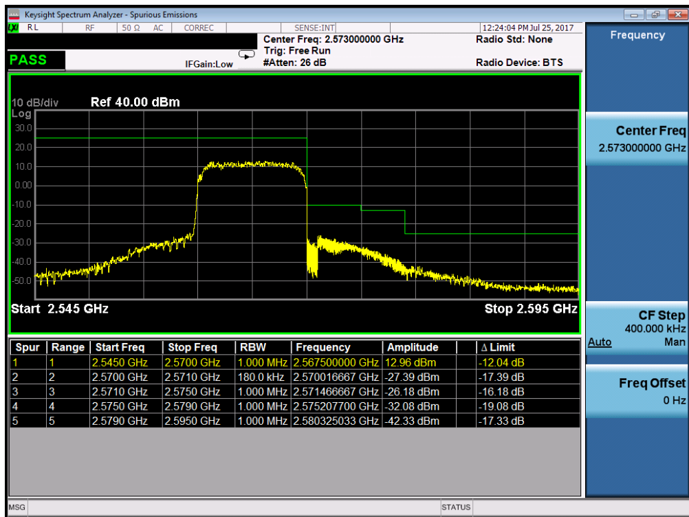
Plot 7-63. Upper ACP Plot (Band 7 – 10.0MHz QPSK – RB Size 50)
