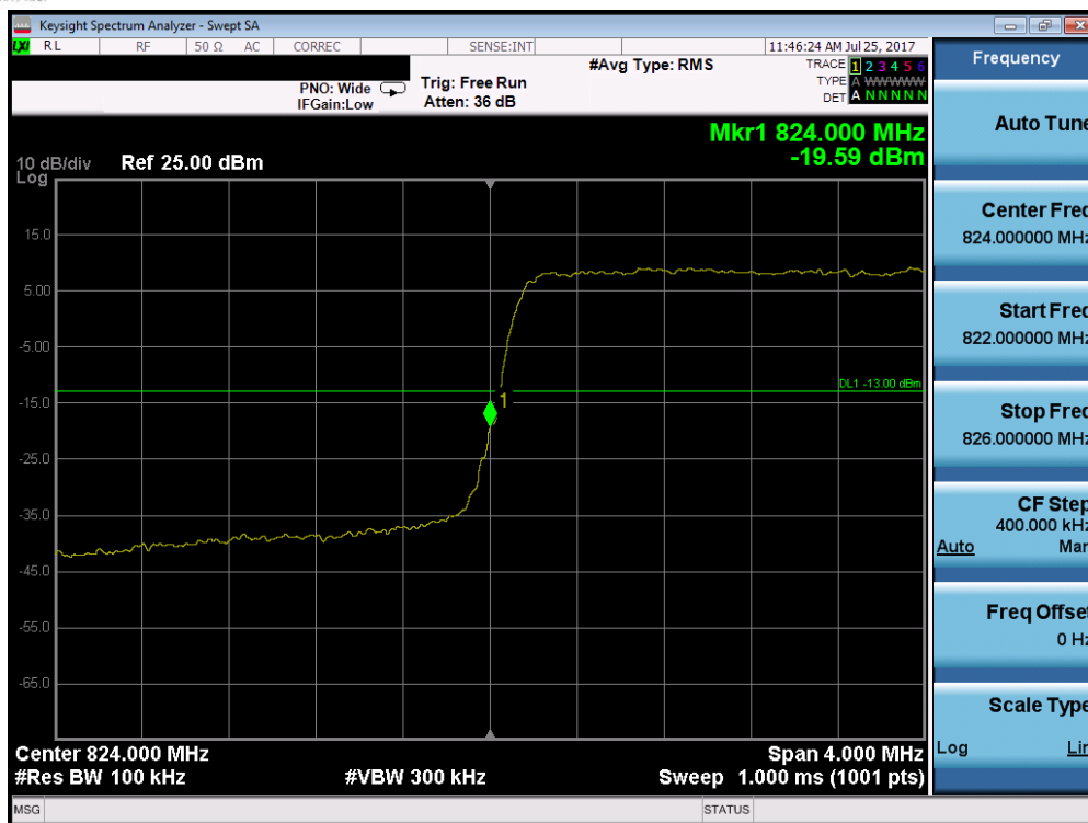
Plot 7-54. Lower Band Edge Plot (Band 5 - 3.0MHz QPSK - RB Size 15)
