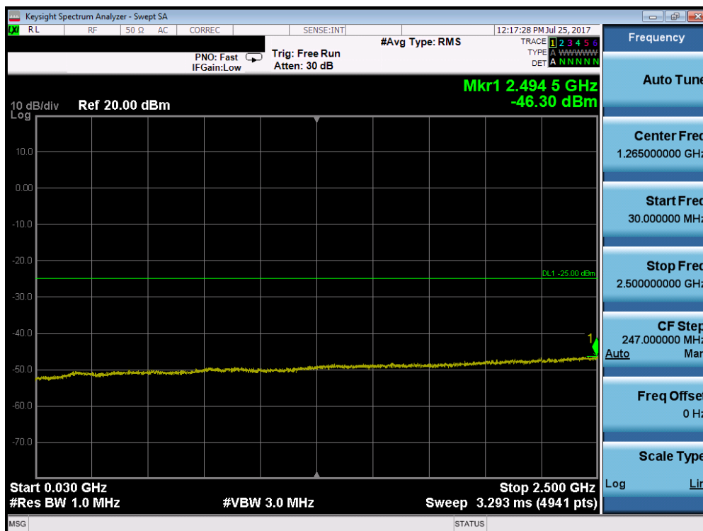
Plot 7-40. Conducted Spurious Plot (Band 7 – 5.0MHz QPSK – RB Size 1, RB Offset 0 – High Channel)
