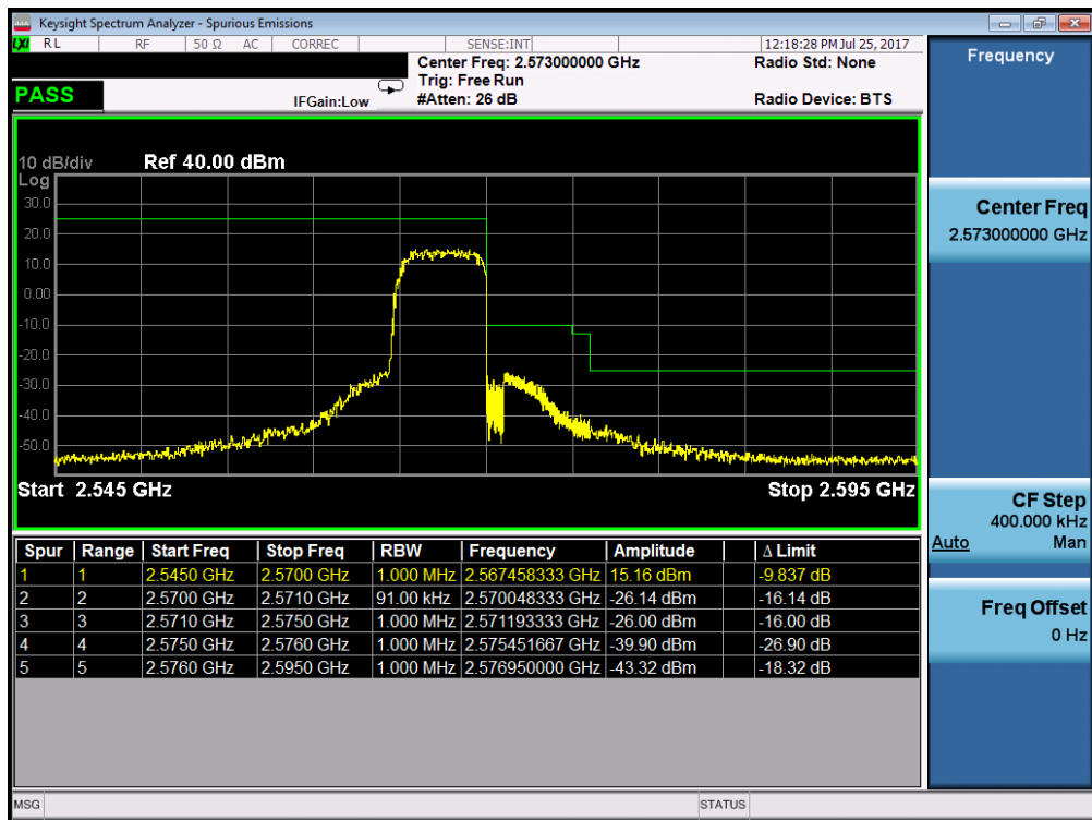
Plot 7-61. Upper ACP Plot (Band 7 – 5.0MHz QPSK – RB Size 25)
