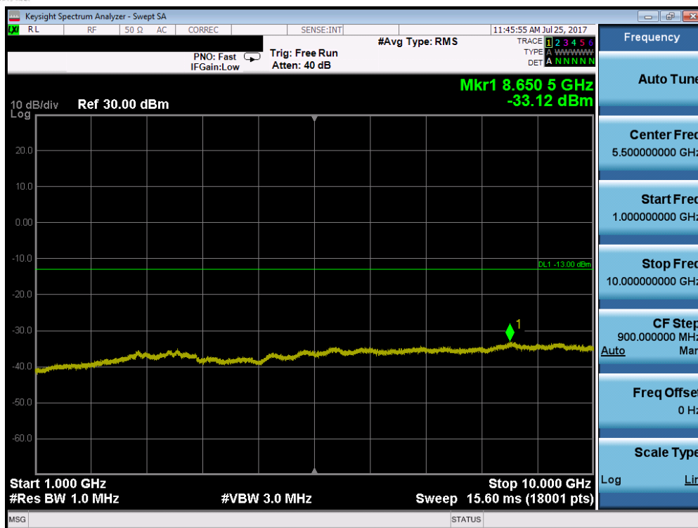
Plot 7-27. Conducted Spurious Plot (Band 5 – 3.0MHz QPSK – RB Size 1, RB Offset 0 – Low Channel)
