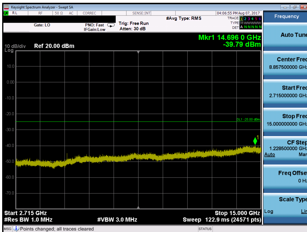
Plot 7-50. Conducted Spurious Plot (Band 38/41 – 10.0MHz QPSK – RB Size 1, RB Offset 0 – High Channel)
