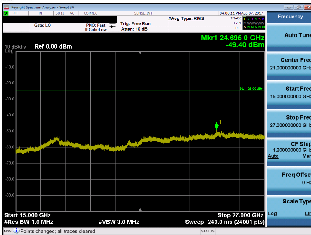
Plot 7-51. Conducted Spurious Plot (Band 38/41 – 10.0MHz QPSK – RB Size 1, RB Offset 0 – High Channel)
