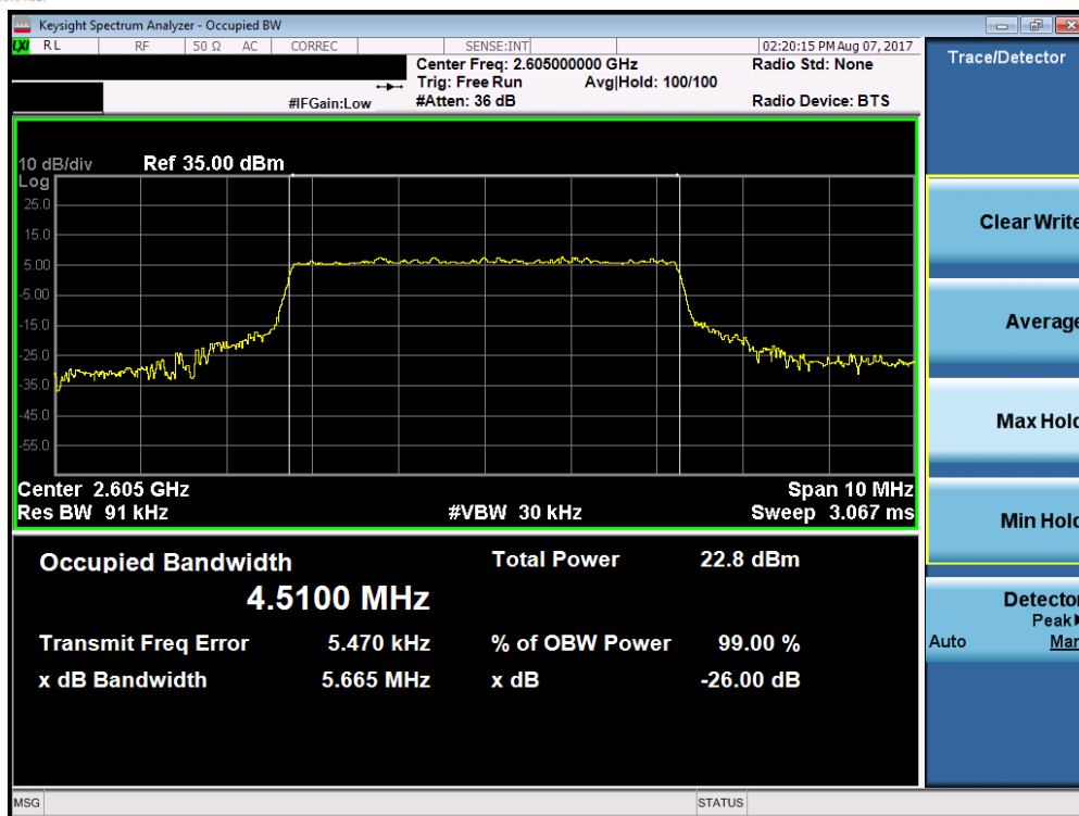
Plot 7-17. Occupied Bandwidth Plot (Band 38/41 – 5.0MHz QPSK – RB Size 25)
