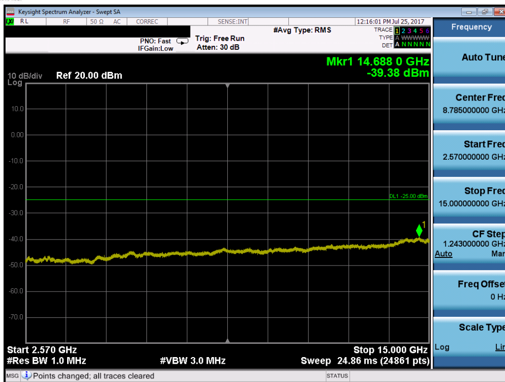
Plot 7-35. Conducted Spurious Plot (Band 7 – 5.0MHz QPSK – RB Size 1, RB Offset 0 – Low Channel)
