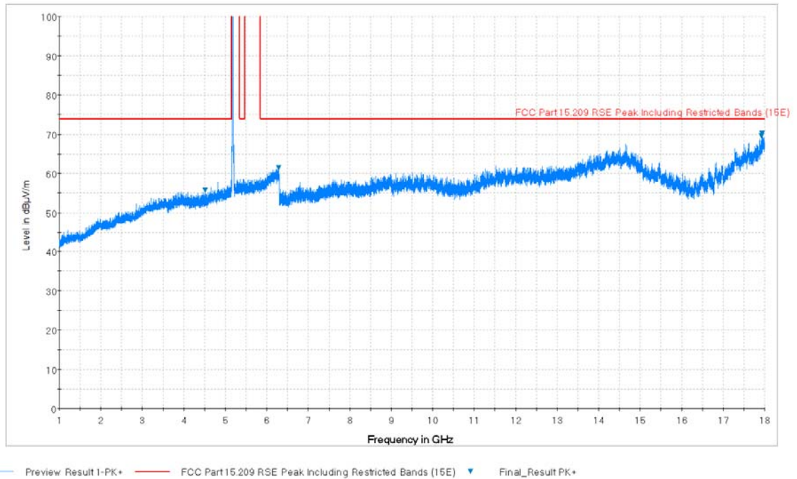
Plot 7-67. Radiated Spurious Plot above 1GHz (802.11a – U1 Ch. 40, Ant. Pol. H)
