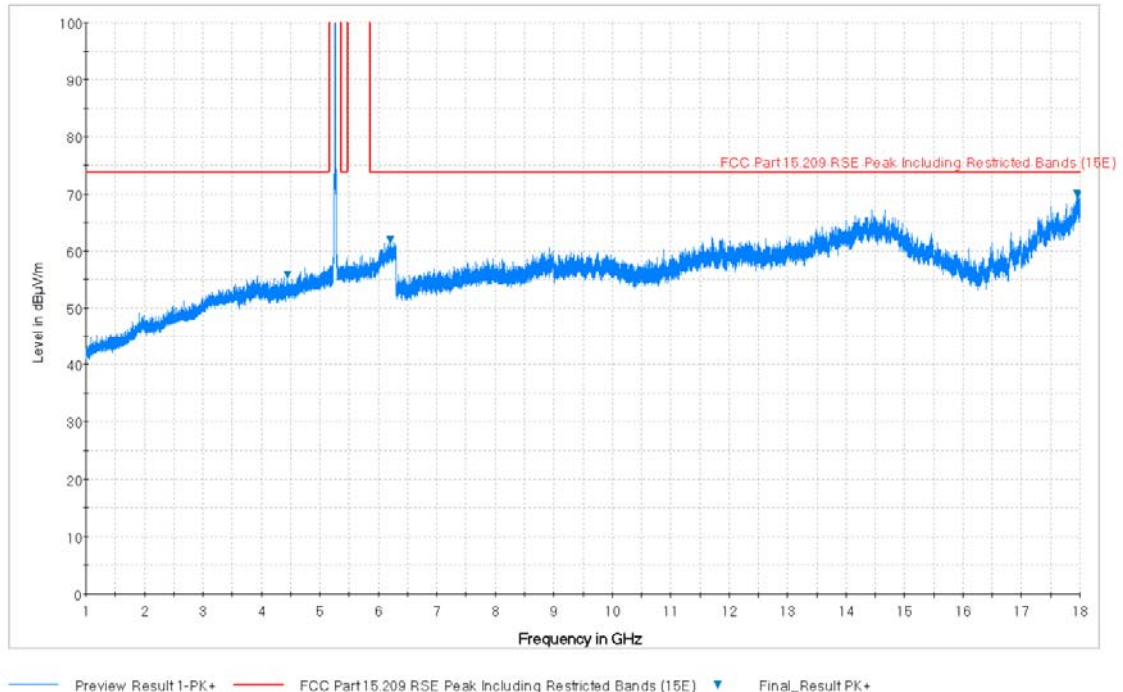
Plot 7-68. Radiated Spurious Plot above 1GHz (802.11a – U1 Ch. 40, Ant. Pol. V)
