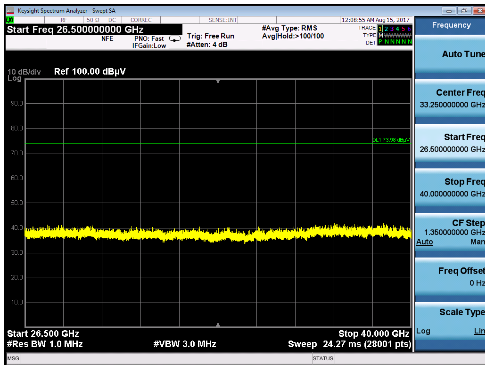
Plot 7-77. Radiated Spurious Plot 26.5GHz - 40GHz (802.11a – Ant. Pol. H)
