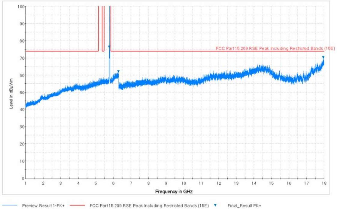
Plot 7-73. Radiated Spurious Plot above 1GHz (802.11a – U3 Ch. 157, Ant. Pol. H)
