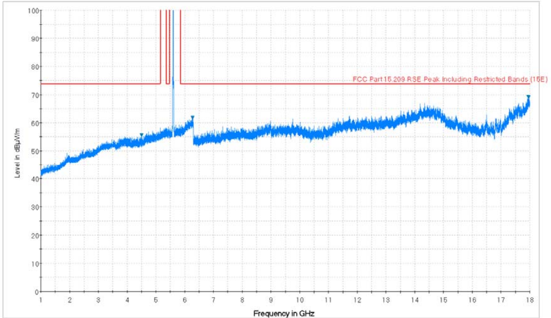
Plot 7-71. Radiated Spurious Plot above 1GHz (802.11a – U2C Ch. 120, Ant. Pol. H)
