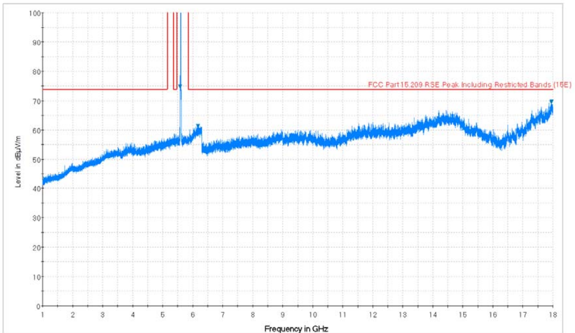
Plot 7-72. Radiated Spurious Plot above 1GHz (802.11a – U2C Ch. 120, Ant. Pol. V)
