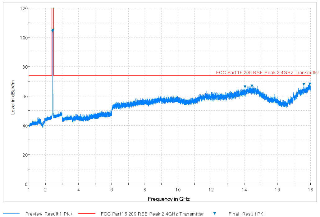
Plot 7-39. Radiated Spurious Plot above 1GHz (802.11b – Ch. 6, Ant. Pol. H)
