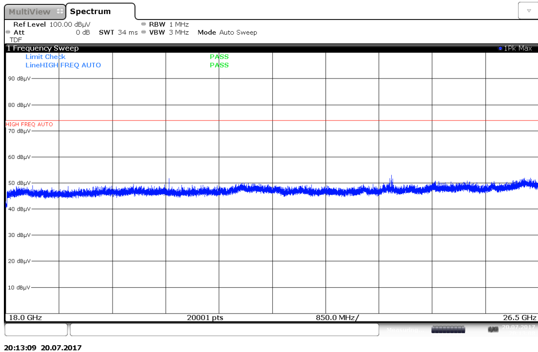
Plot 7-44. Radiated Spurious Plot above 18GHz (Pol. V)
