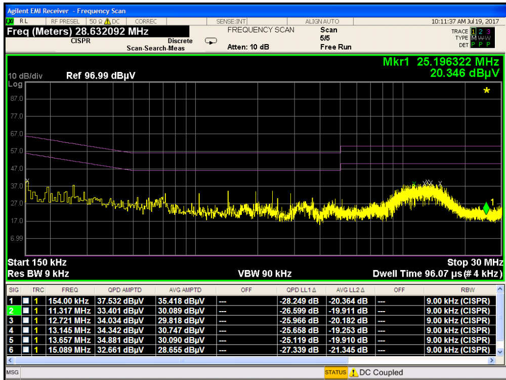
Plot 7-55. Line Conducted Plot with 802.11b (L1)
