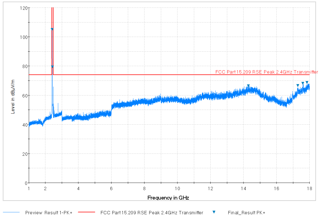
Plot 7-37. Radiated Spurious Plot above 1GHz (802.11b – Ch. 1, Ant. Pol. H)
