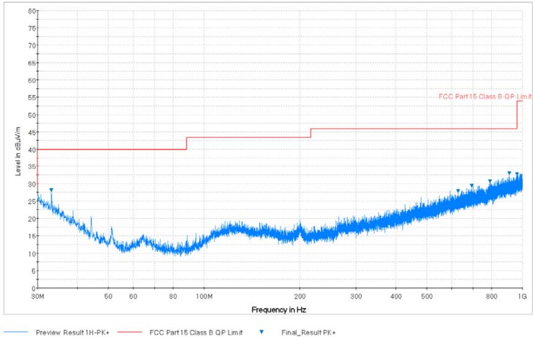
Plot 7-54. Radiated Spurious Plot below 1GHz (Pol. V)
