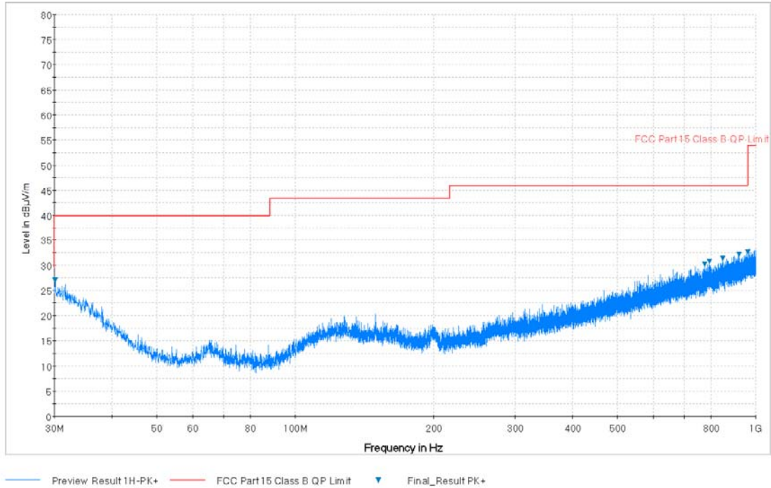
Plot 7-53. Radiated Spurious Plot below 1GHz (Pol. H)
