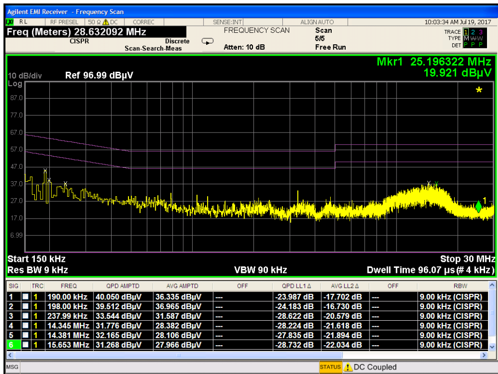
Plot 7-56. Line Conducted Plot with 802.11b (N)
