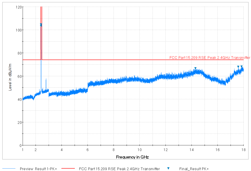
Plot 7-38. Radiated Spurious Plot above 1GHz (802.11b – Ch. 1, Ant. Pol. V)
