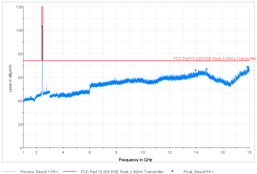
Plot 7-40. Radiated Spurious Plot above 1GHz (802.11b – Ch. 6, Ant. Pol. V)
