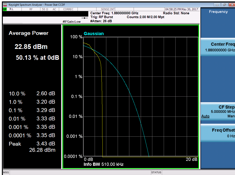
Plot 7-43. Peak-Average Ratio Plot (EDGE1900 Mode – Ch. 661)
