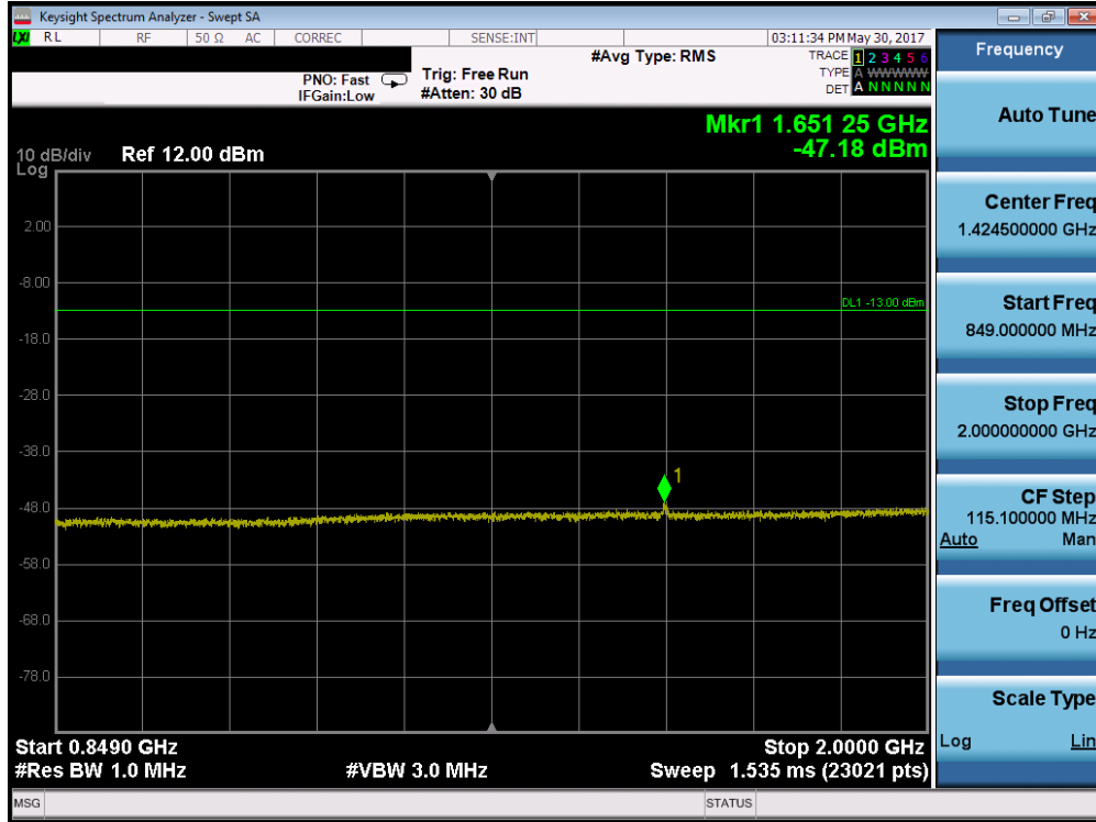
Plot 7-15. Conducted Spurious Plot (Cellular WCDMA Mode – Ch. 4132)
