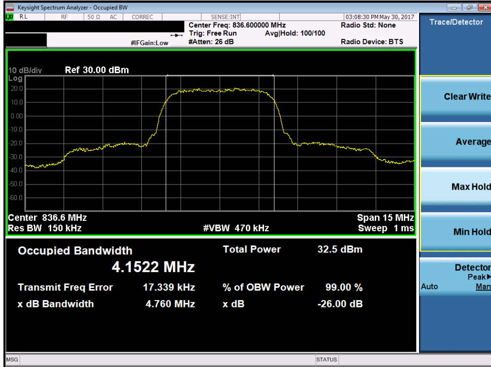
Plot 7-3. Occupied Bandwidth Plot (Cellular WCDMA Mode – Ch. 4183)
