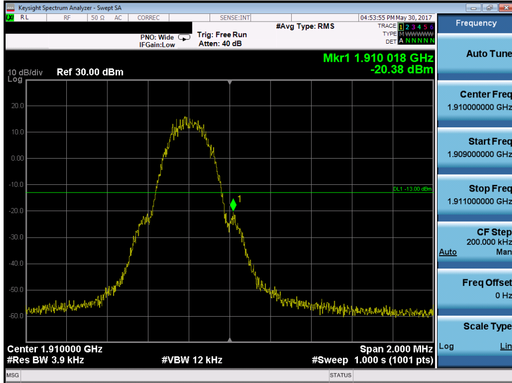
Plot 7-34. Band Edge Plot (PCS GPRS Mode – Ch. 810)
