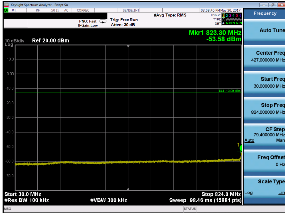
Plot 7-17. Conducted Spurious Plot (Cellular WCDMA Mode – Ch. 4183)
