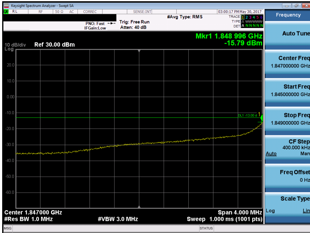
Plot 7-39. 4MHz Span Plot (PCS WCDMA Mode – Ch. 9262)
