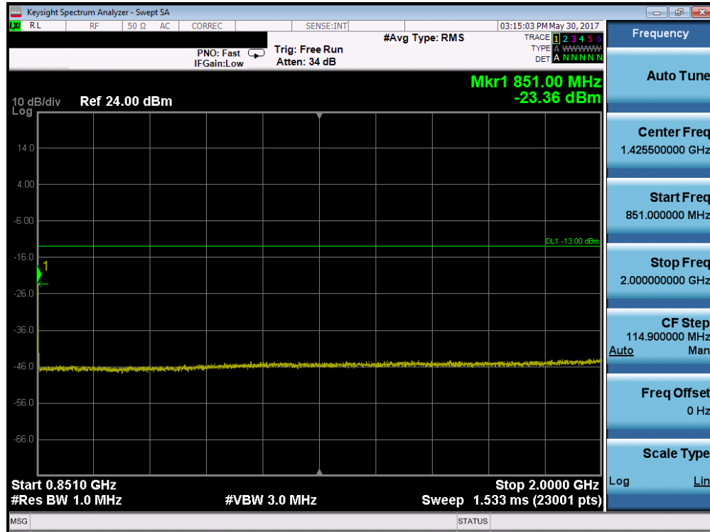
Plot 7-21. Conducted Spurious Plot (Cellular WCDMA Mode – Ch. 4233)
