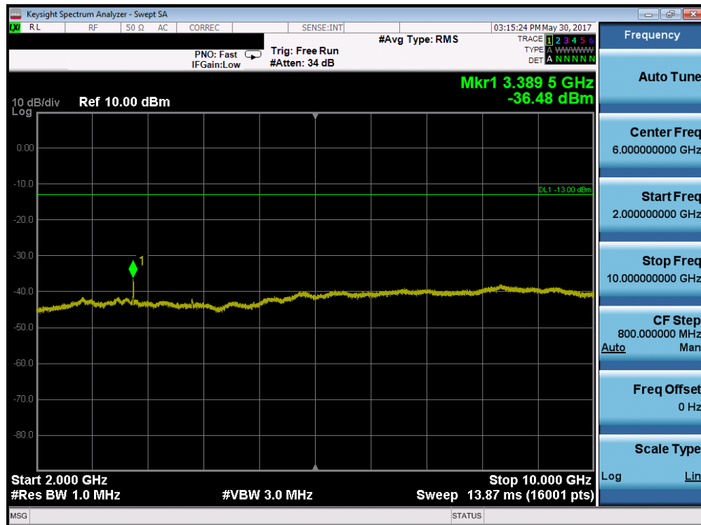
Plot 7-22. Conducted Spurious Plot (Cellular WCDMA Mode – Ch. 4233)
