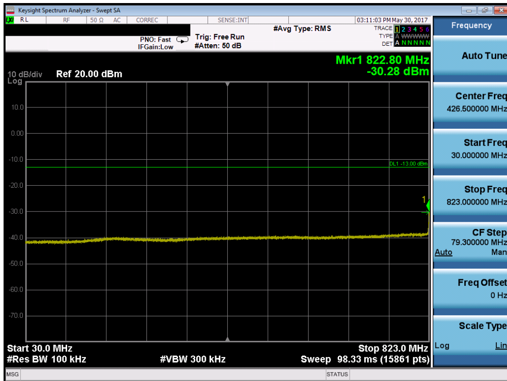
Plot 7-14. Conducted Spurious Plot (Cellular WCDMA Mode – Ch. 4132)
