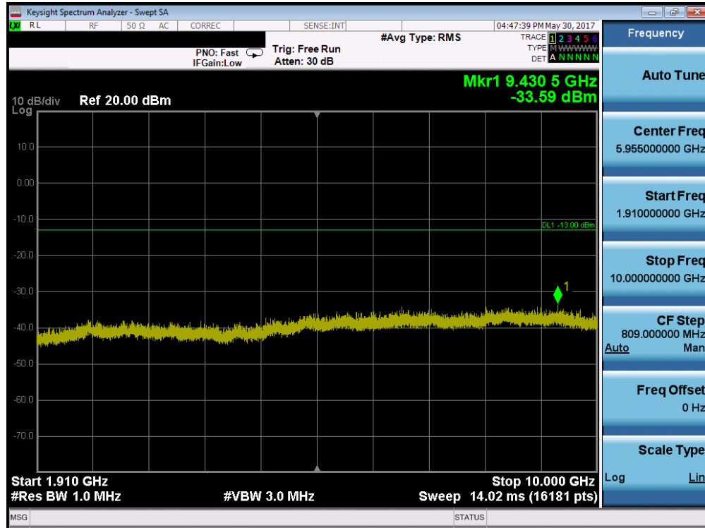
Plot 7-9. Conducted Spurious Plot (PCS GPRS Mode – Ch. 661)
