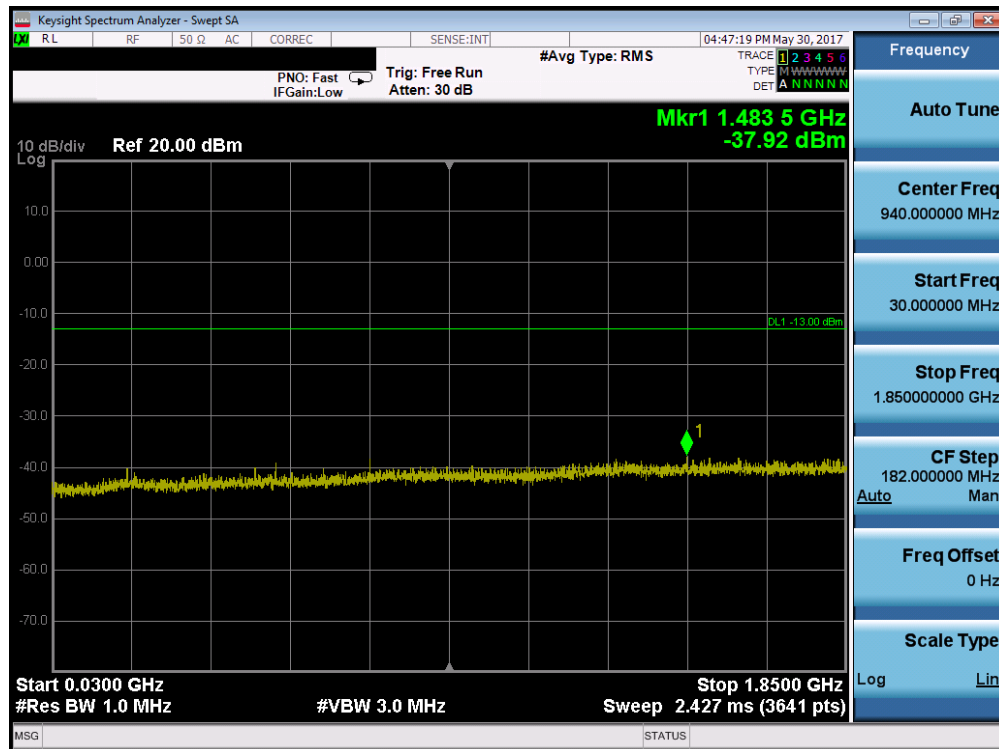
Plot 7-8. Conducted Spurious Plot (PCS GPRS Mode – Ch. 661)
