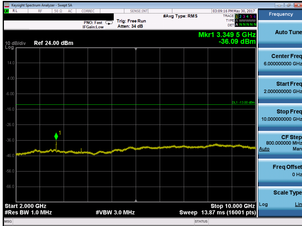
Plot 7-19. Conducted Spurious Plot (Cellular WCDMA Mode – Ch. 4183)
