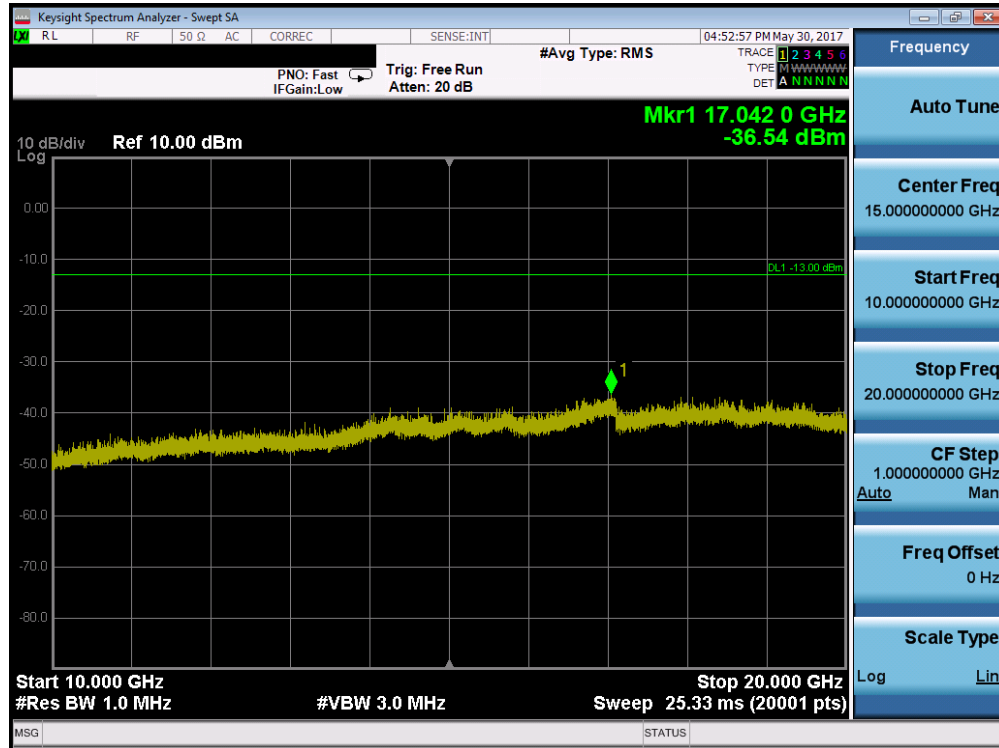
Plot 7-7. Conducted Spurious Plot (PCS GPRS Mode – Ch. 512)
