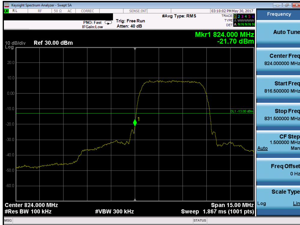
Plot 7-36. Band Edge Plot (Cellular WCDMA Mode – Ch. 4132)
