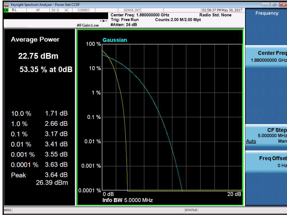
Plot 7-44. Peak-Average Ratio Plot (PCS WCDMA Mode – Ch. 9400)
