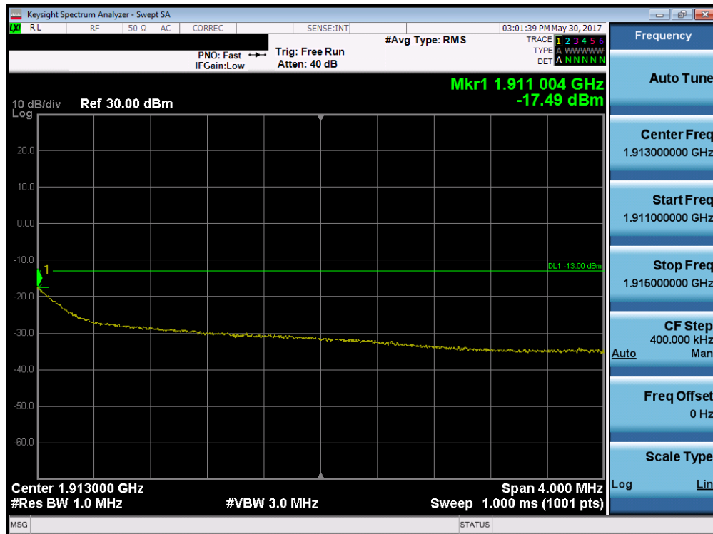
Plot 7-41. 4MHz Span Plot (PCS WCDMA Mode – Ch. 9538)
