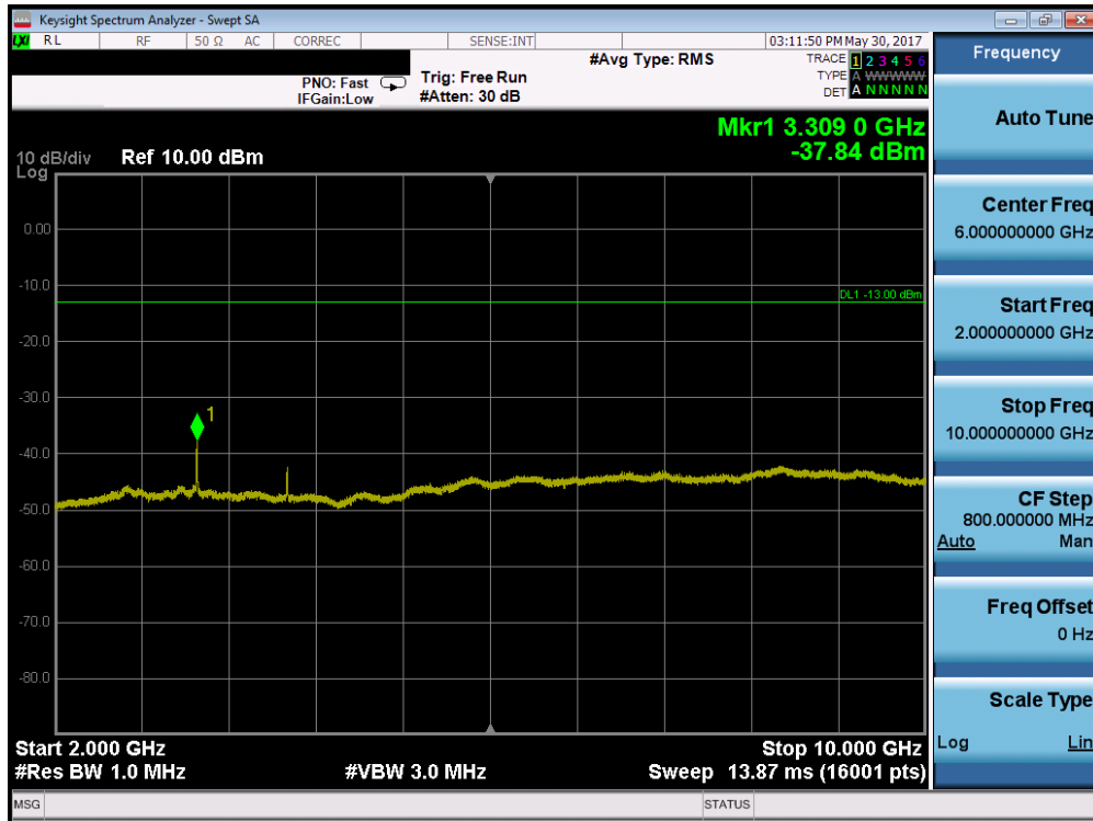
Plot 7-16. Conducted Spurious Plot (Cellular WCDMA Mode – Ch. 4132)
