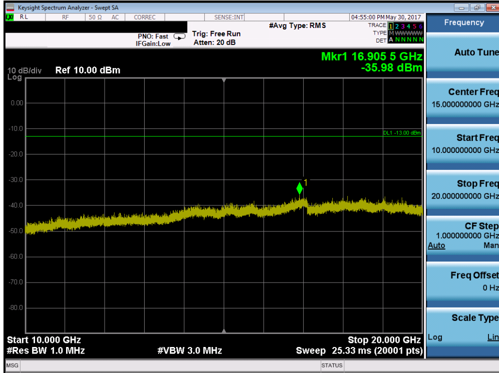
Plot 7-13. Conducted Spurious Plot (PCS GPRS Mode – Ch. 810)
