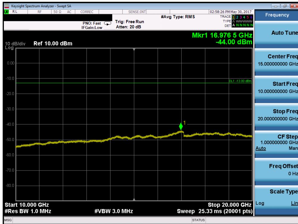
Plot 7-28. Conducted Spurious Plot (PCS WCDMA Mode – Ch. 9400)
