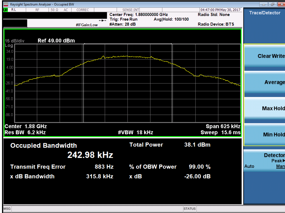
Plot 7-1. Occupied Bandwidth Plot (PCS GPRS Mode – Ch. 661)
