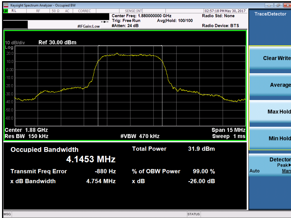
Plot 7-4. Occupied Bandwidth Plot (PCS WCDMA Mode – Ch. 9400)
