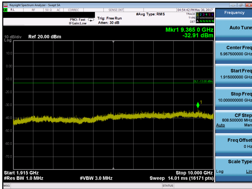
Plot 7-12. Conducted Spurious Plot (PCS GPRS Mode – Ch. 810)
