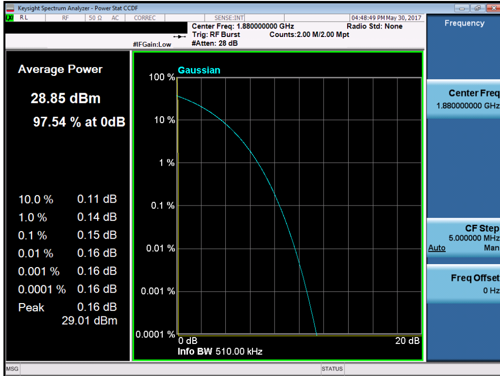
Plot 7-42. Peak-Average Ratio Plot (PCS GPRS Mode – Ch. 661)
