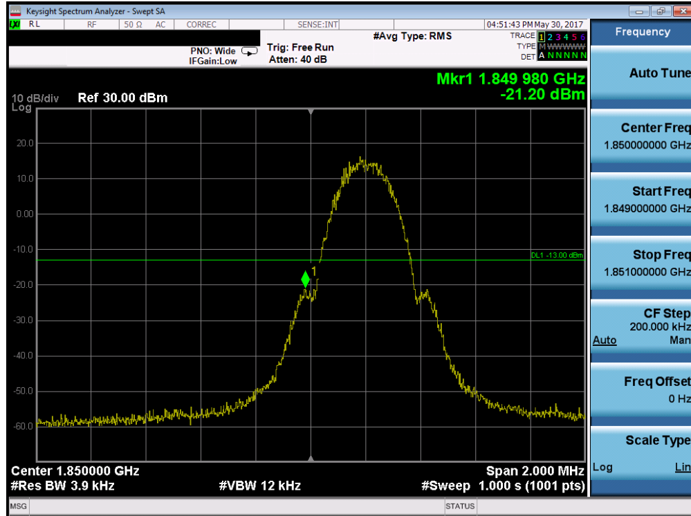
Plot 7-32. Band Edge Plot (PCS GPRS Mode – Ch. 512)
