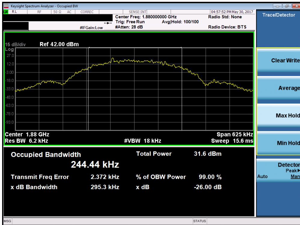
Plot 7-2. Occupied Bandwidth Plot (EDGE1900 Mode – Ch. 661)
