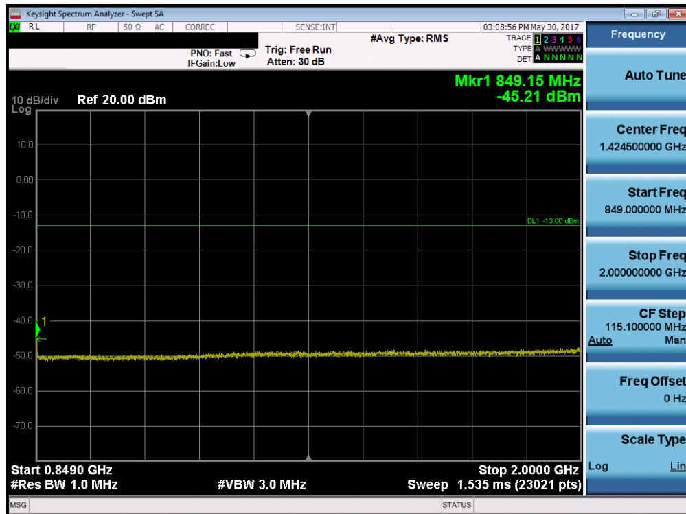
Plot 7-18. Conducted Spurious Plot (Cellular WCDMA Mode – Ch. 4183)
