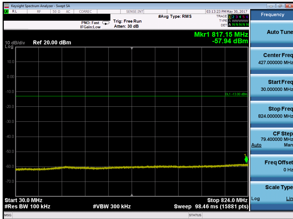
Plot 7-20. Conducted Spurious Plot (Cellular WCDMA Mode – Ch. 4233)
