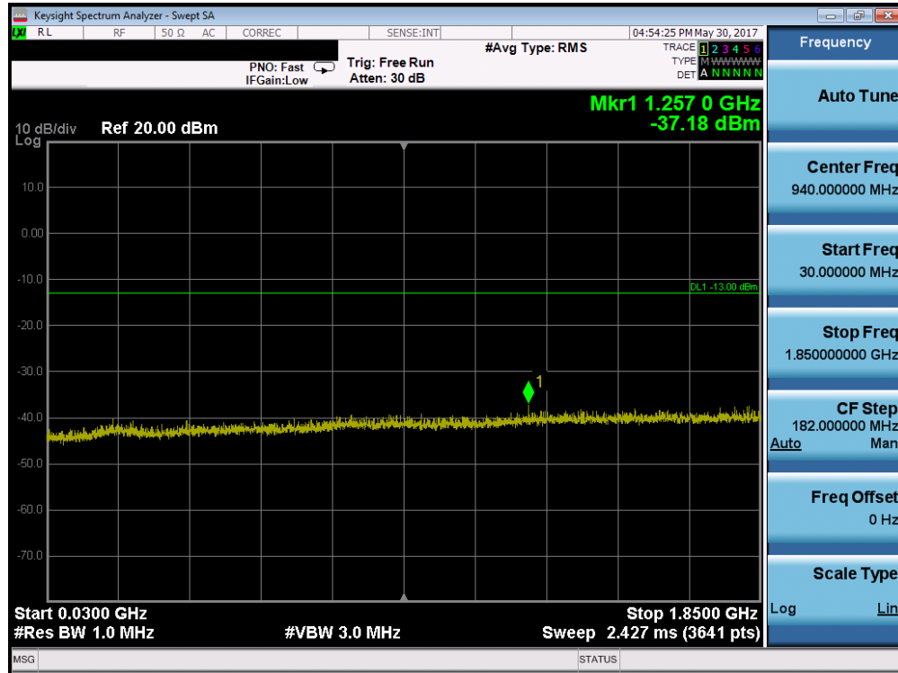
Plot 7-11. Conducted Spurious Plot (PCS GPRS Mode – Ch. 810)
