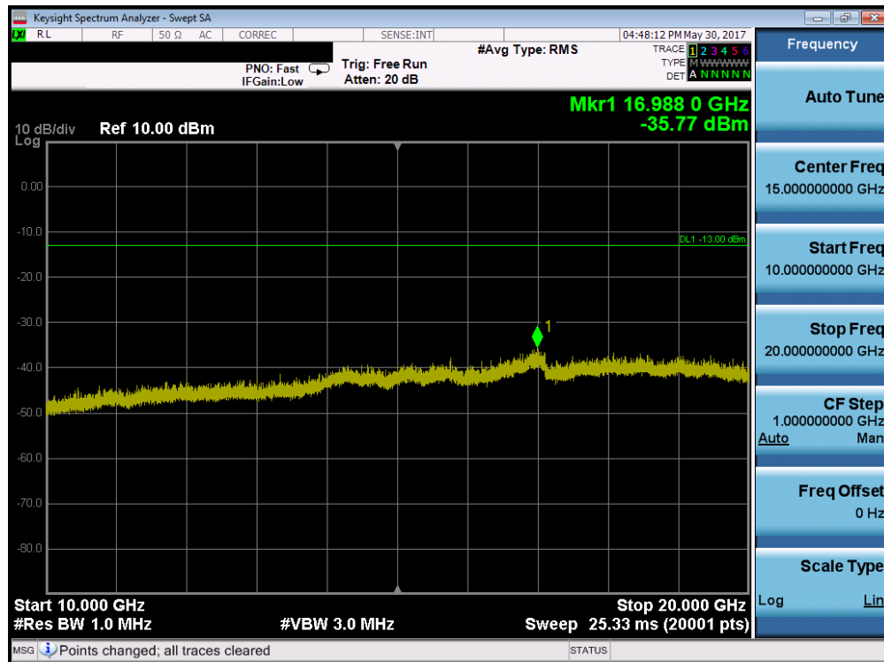
Plot 7-10. Conducted Spurious Plot (PCS GPRS Mode – Ch. 661)
