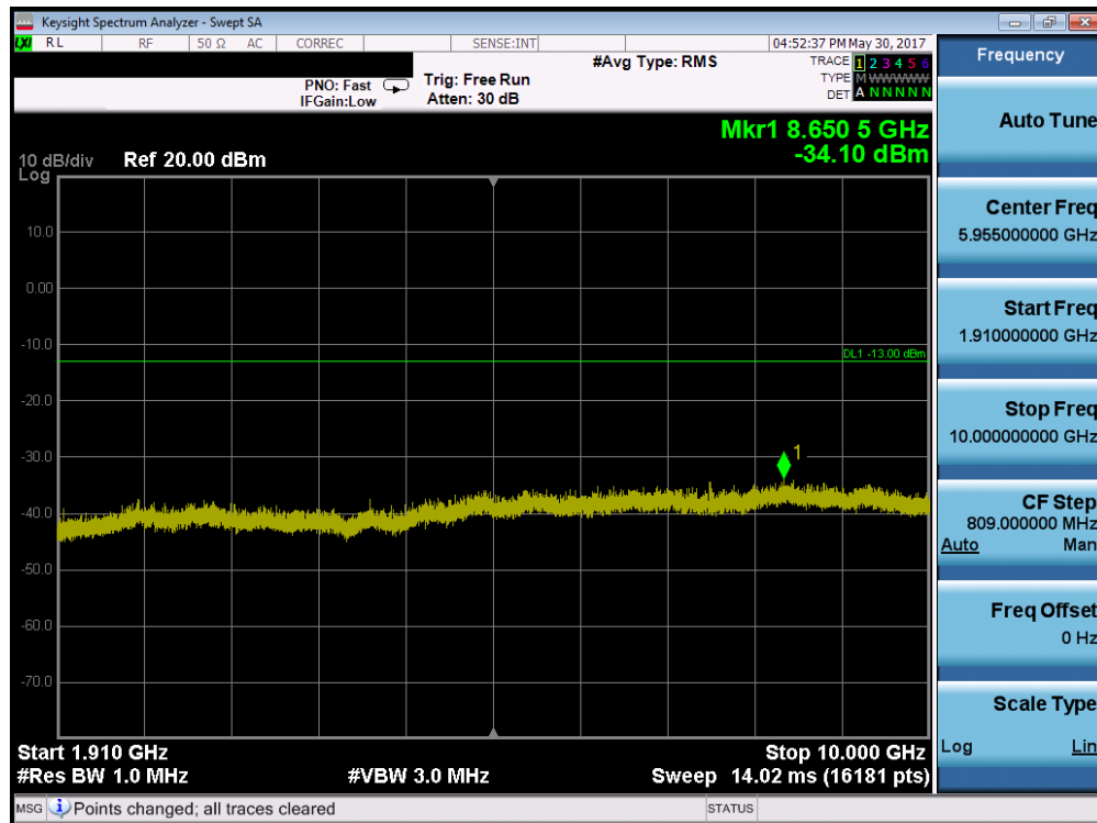
Plot 7-6. Conducted Spurious Plot (PCS GPRS Mode – Ch. 512)
