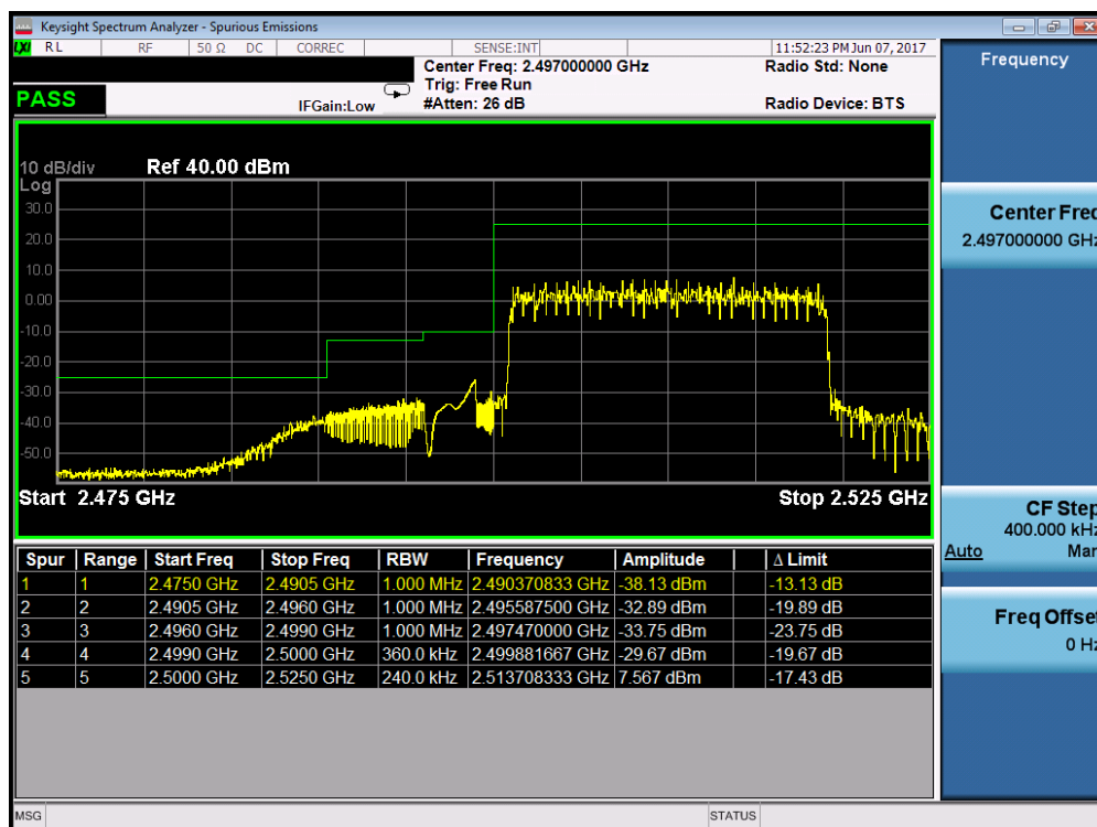
Plot 7-83. Lower ACP Plot (Band 7 – 20.0MHz QPSK – RB Size 100)
