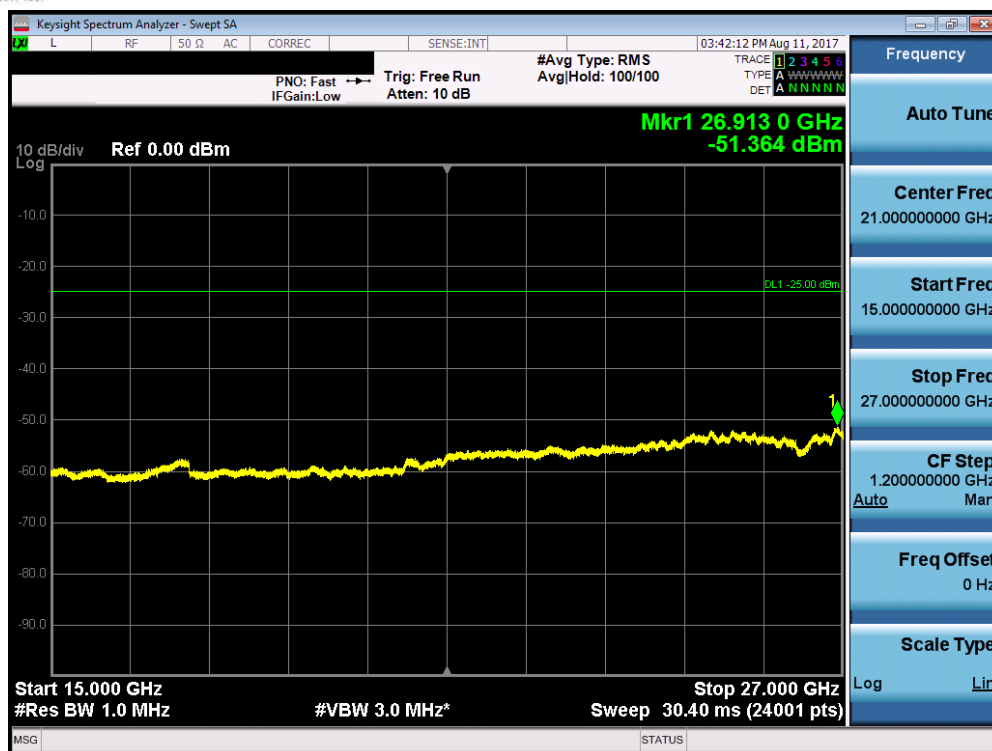
Plot 7-55. Conducted Spurious Plot (Band 7 – 5.0MHz QPSK – RB Size 1, RB Offset 0 – High Channel)
