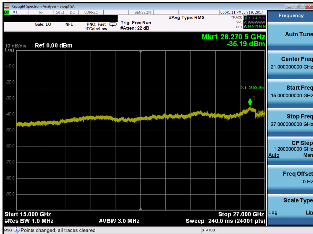
Plot 7-64. Conducted Spurious Plot (Band 38 – 5.0MHz QPSK – RB Size 1, RB Offset 0 – High Channel)
