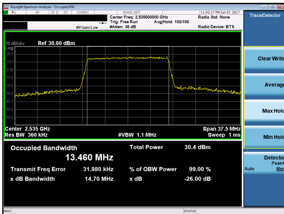
Plot 7-18. Occupied Bandwidth Plot (Band 7 – 15.0MHz 16-QAM – RB Size 75)
