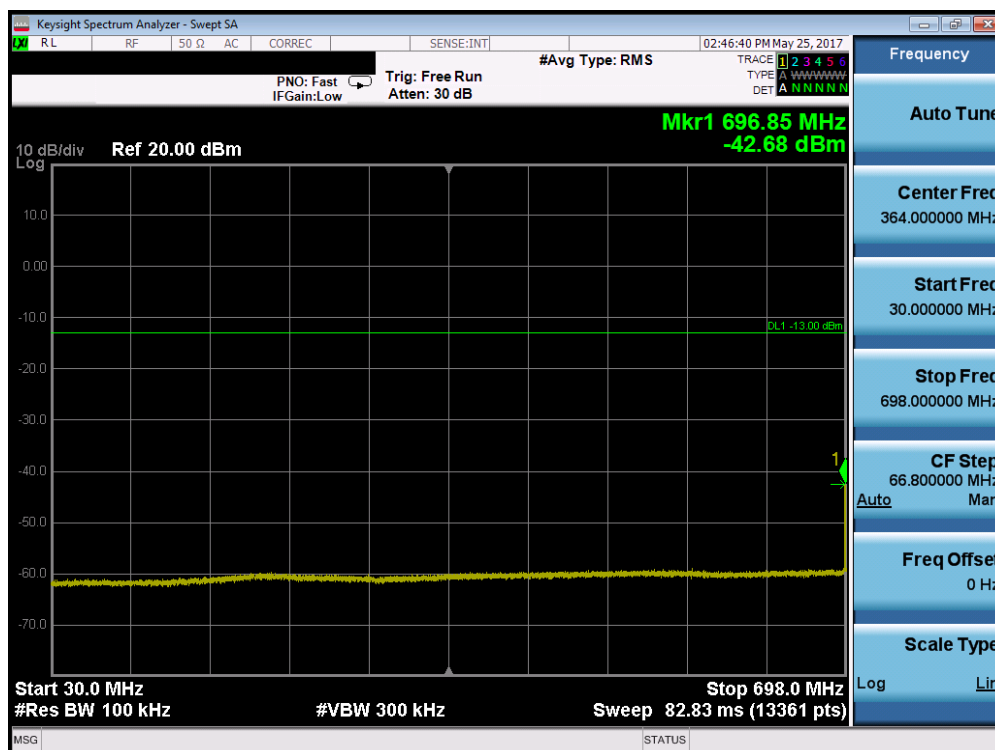
Plot 7-32. Conducted Spurious Plot (Band 17 – 10.0MHz QPSK – RB Size 1, RB Offset 0 – Mid Channel)
