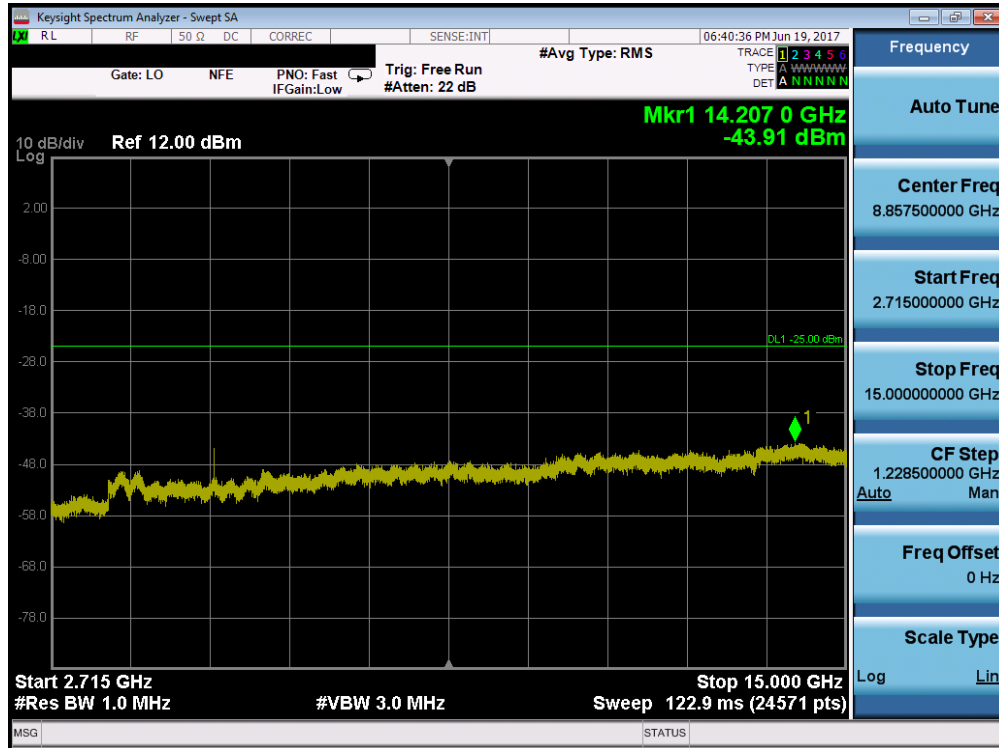
Plot 7-63. Conducted Spurious Plot (Band 38 – 5.0MHz QPSK – RB Size 1, RB Offset 0 – High Channel)
