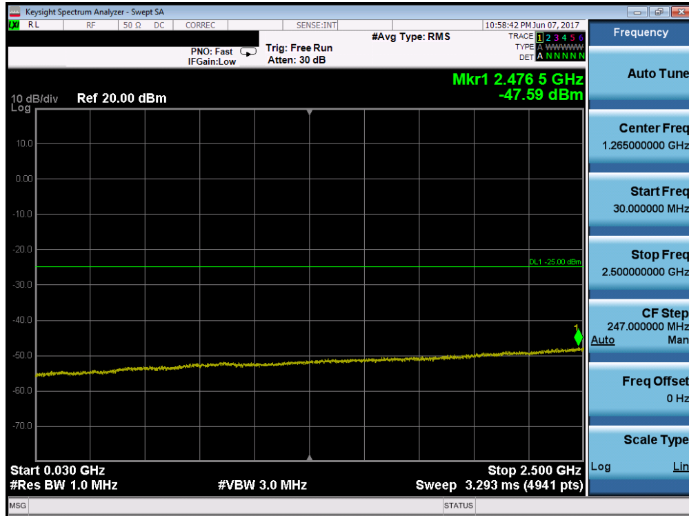
Plot 7-53. Conducted Spurious Plot (Band 7 – 5.0MHz QPSK – RB Size 1, RB Offset 0 – High Channel)
