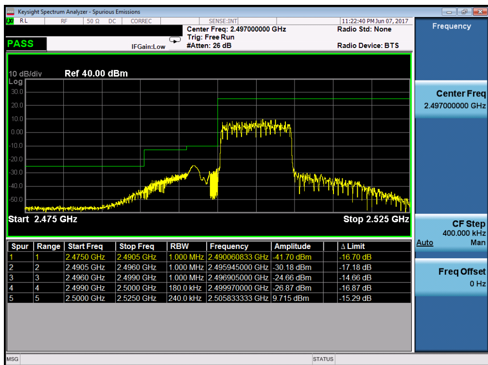
Plot 7-79. Lower ACP Plot (Band 7 – 10.0MHz QPSK – RB Size 50)
