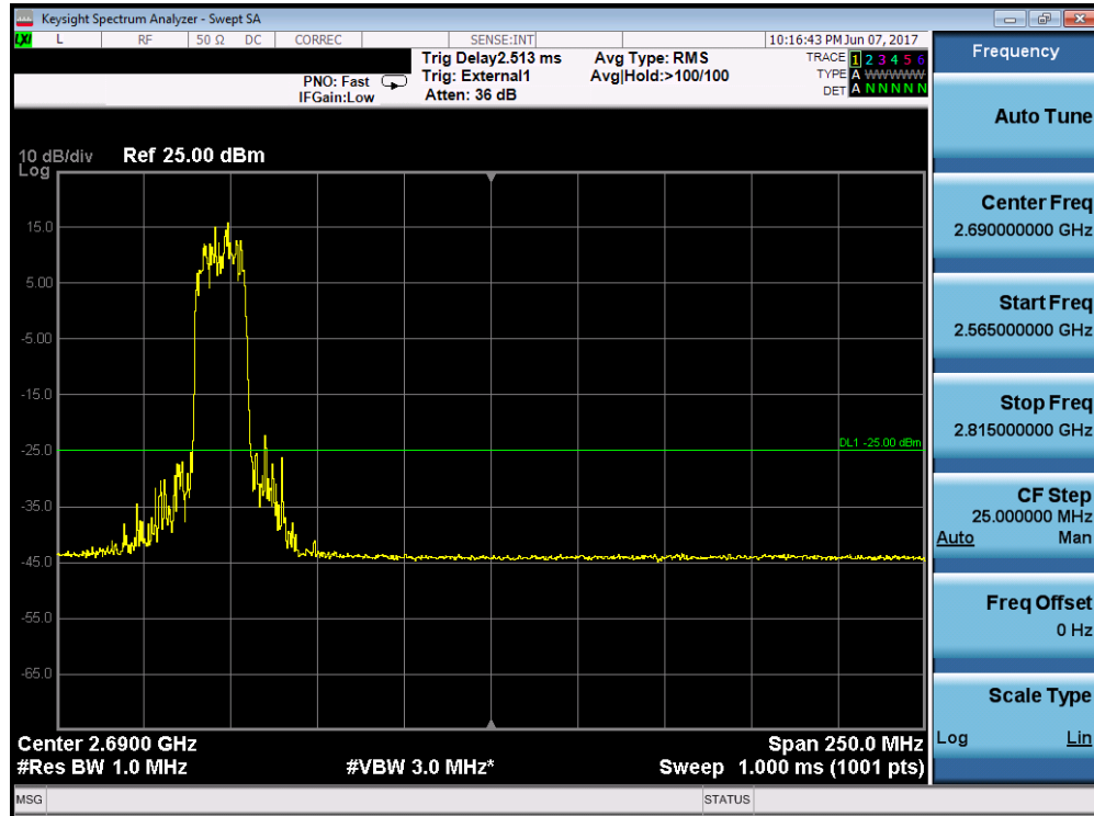
Plot 7-90. Upper Band Edge Plot (Band 38 – 15.0MHz QPSK – RB Size 75)
