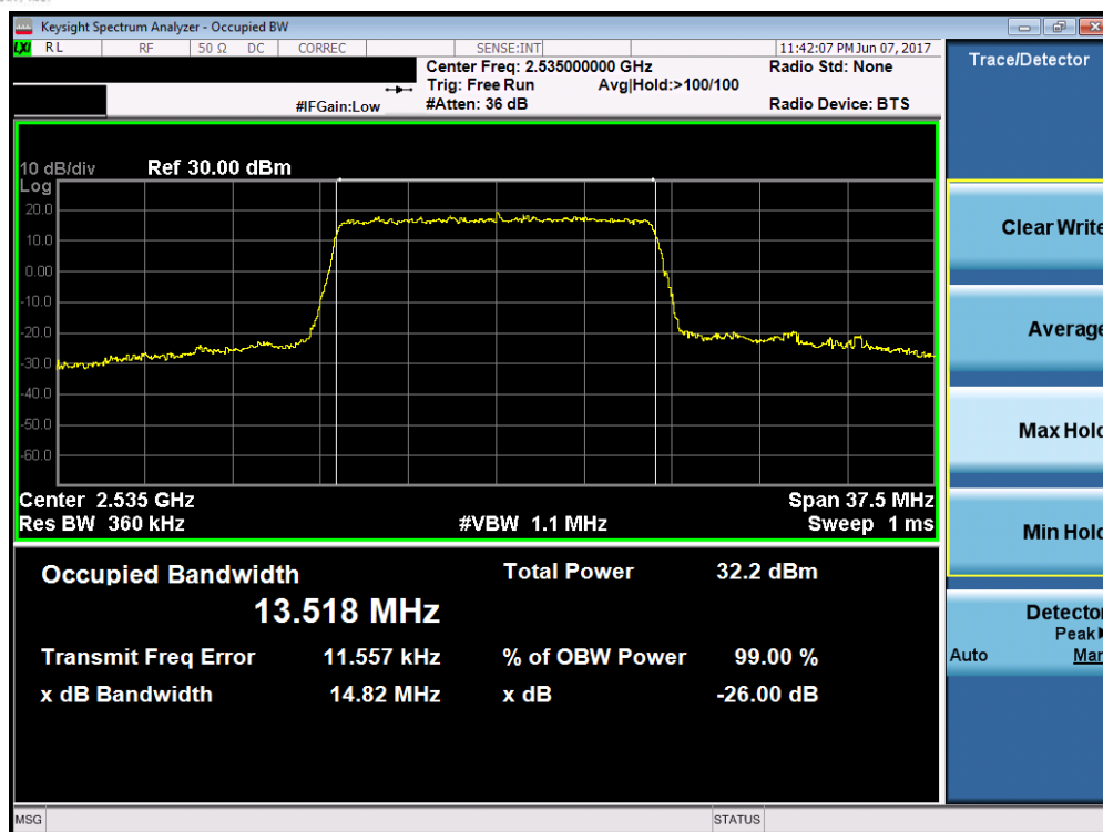
Plot 7-17. Occupied Bandwidth Plot (Band 7 – 15.0MHz QPSK – RB Size 75)
