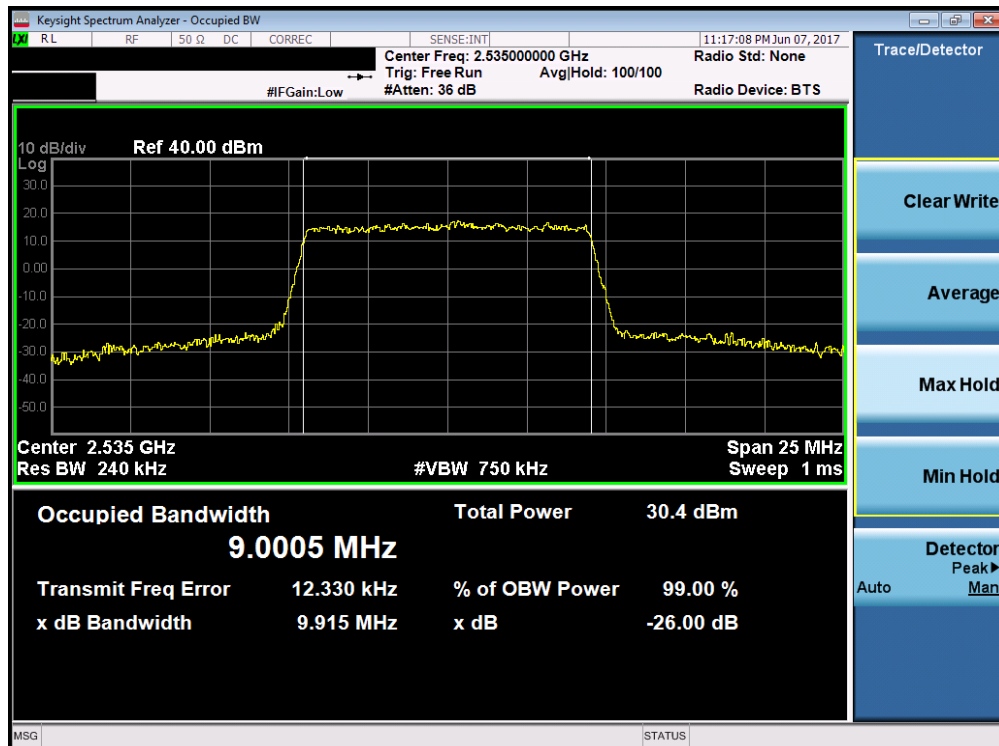
Plot 7-16. Occupied Bandwidth Plot (Band 7 – 10.0MHz 16-QAM – RB Size 50)
