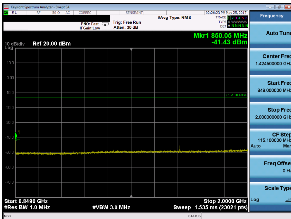
Plot 7-42. Conducted Spurious Plot (Band 5 – 10.0MHz QPSK – RB Size 1, RB Offset 0 – Mid Channel)
