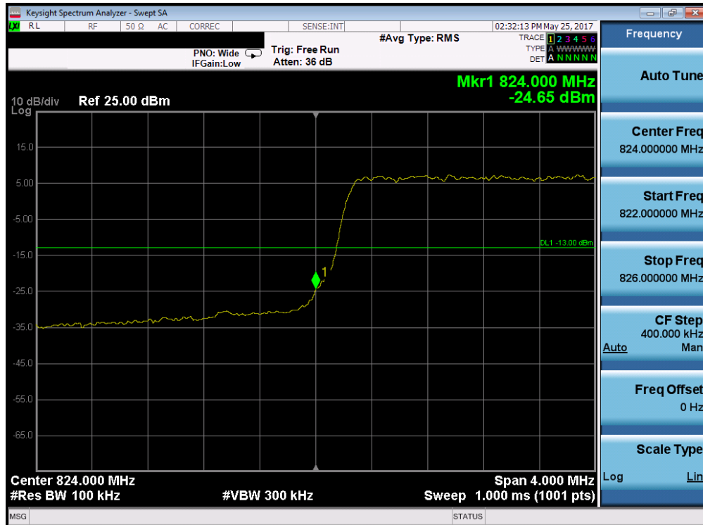
Plot 7-73. Lower Band Edge Plot (Band 5 – 5.0MHz QPSK – RB Size 25)
