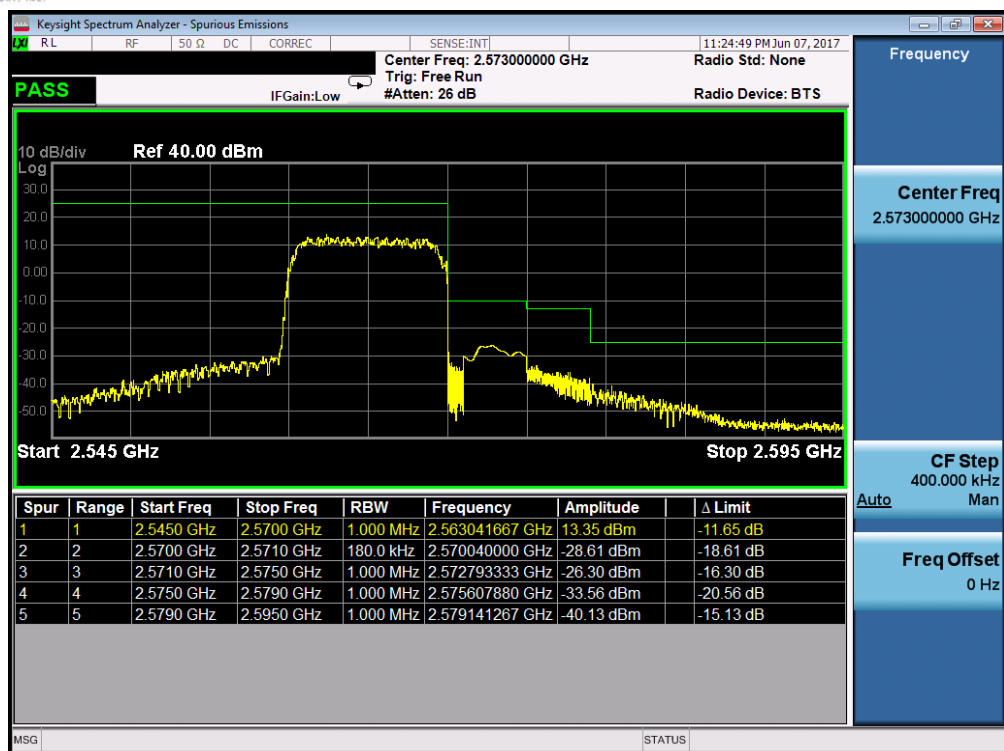
Plot 7-80. Upper ACP Plot (Band 7 – 10.0MHz QPSK – RB Size 50)
