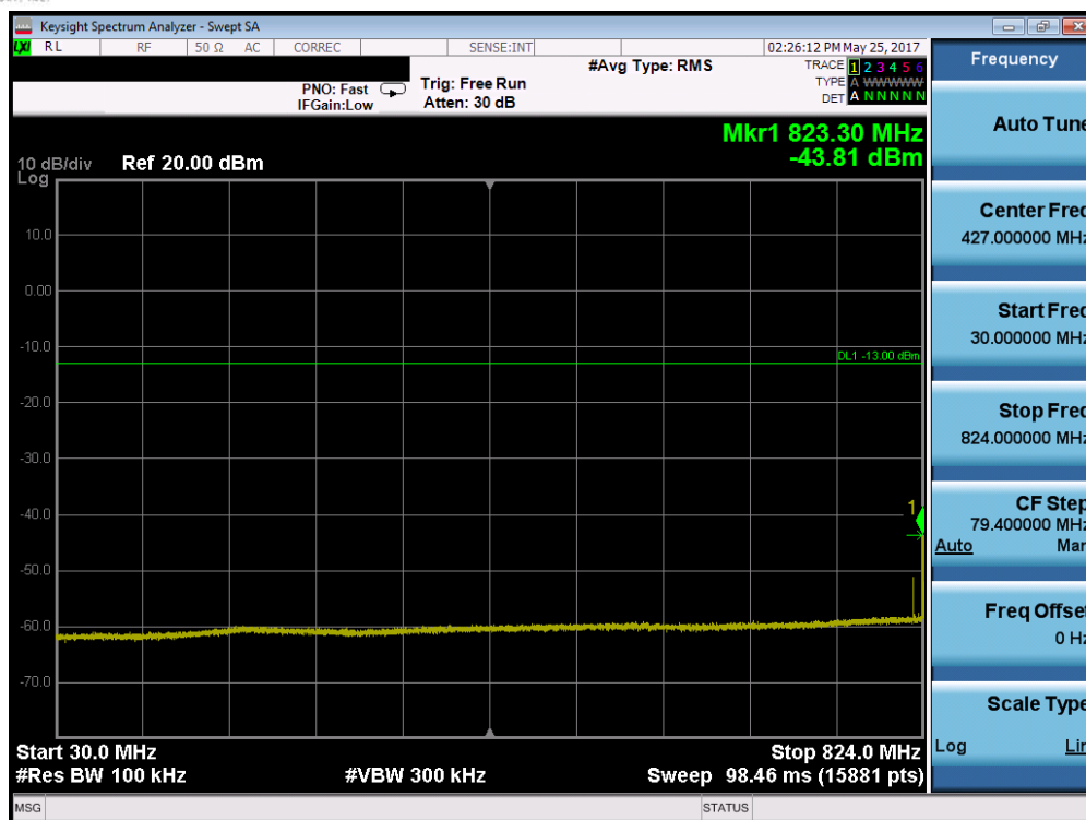
Plot 7-41. Conducted Spurious Plot (Band 5 – 10.0MHz QPSK – RB Size 1, RB Offset 0 – Mid Channel)
