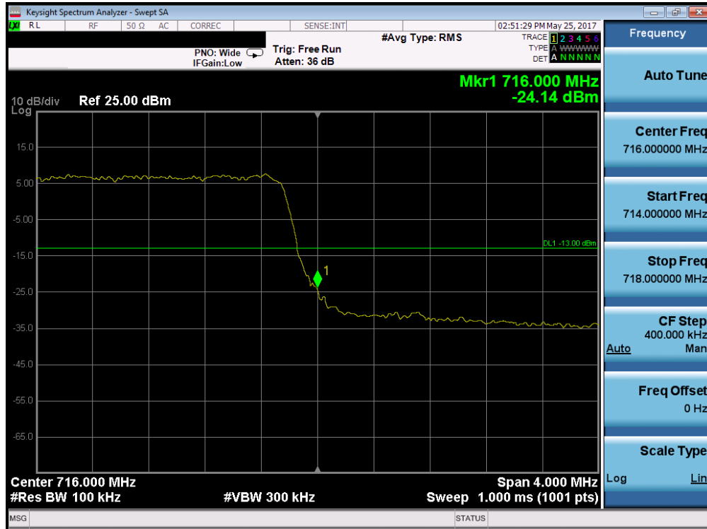
Plot 7-66. Upper Band Edge Plot (Band 17 – 5.0MHz QPSK – RB Size 25)
