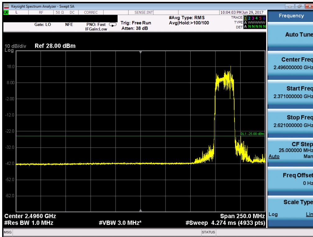
Plot 7-91. Lower Band Edge Plot (Band 38 – 20.0MHz QPSK – RB Size 100)
