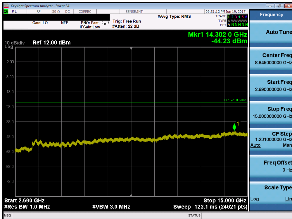
Plot 7-60. Conducted Spurious Plot (Band 38 – 5.0MHz QPSK – RB Size 1, RB Offset 0 – Mid Channel)
