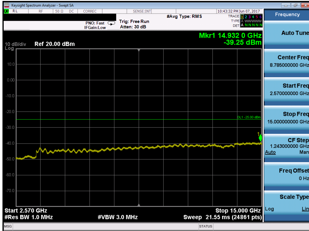
Plot 7-51. Conducted Spurious Plot (Band 7 – 5.0MHz QPSK – RB Size 1, RB Offset 0 – Mid Channel)
