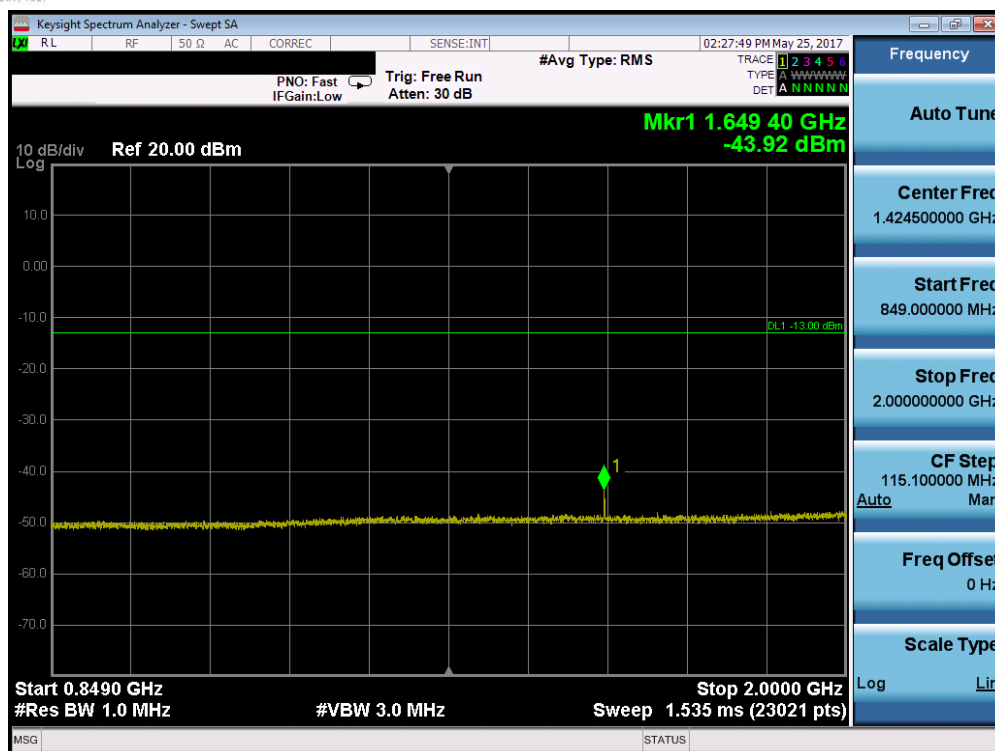
Plot 7-39. Conducted Spurious Plot (Band 5 – 10.0MHz QPSK – RB Size 1, RB Offset 0 – Low Channel)
