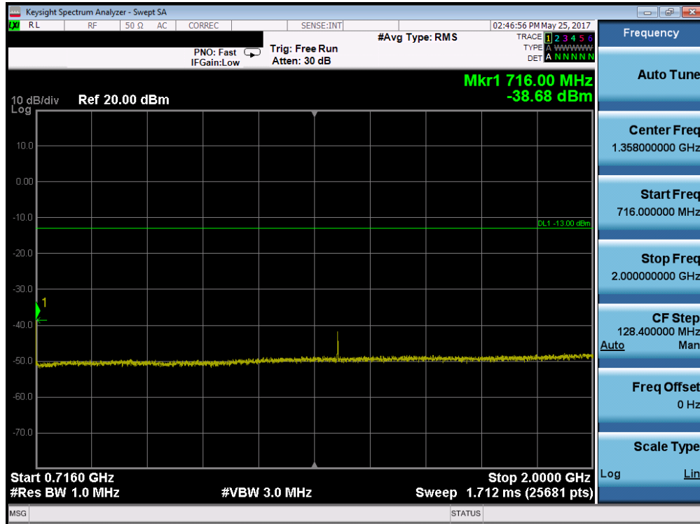
Plot 7-33. Conducted Spurious Plot (Band 17 – 10.0MHz QPSK – RB Size 1, RB Offset 0 – Mid Channel)
