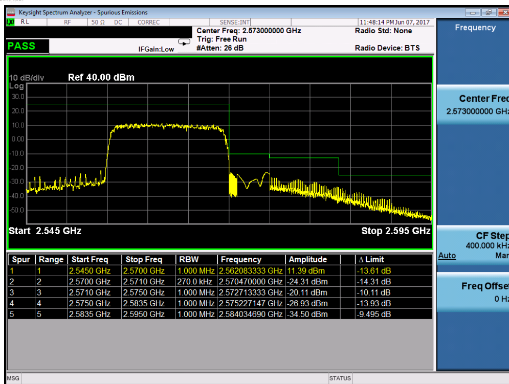
Plot 7-82. Upper ACP Plot (Band 7 – 15.0MHz QPSK – RB Size 75)
