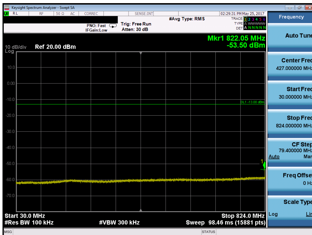
Plot 7-44. Conducted Spurious Plot (Band 5 – 10.0MHz QPSK – RB Size 1, RB Offset 0 – High Channel)
