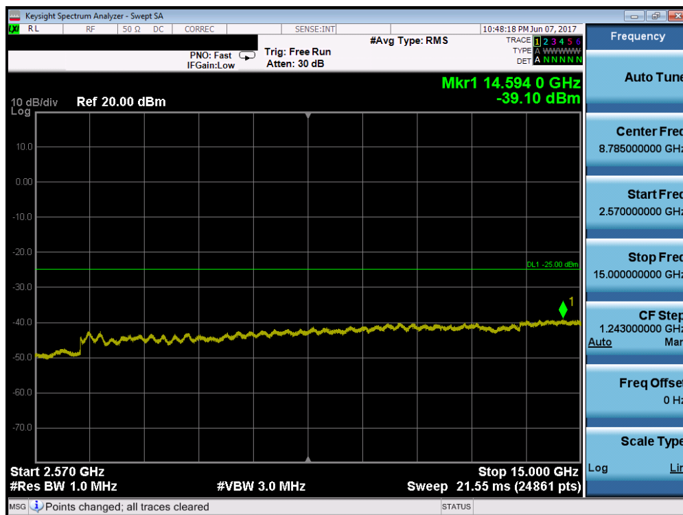
Plot 7-48. Conducted Spurious Plot (Band 7 – 5.0MHz QPSK – RB Size 1, RB Offset 0 – Low Channel)
