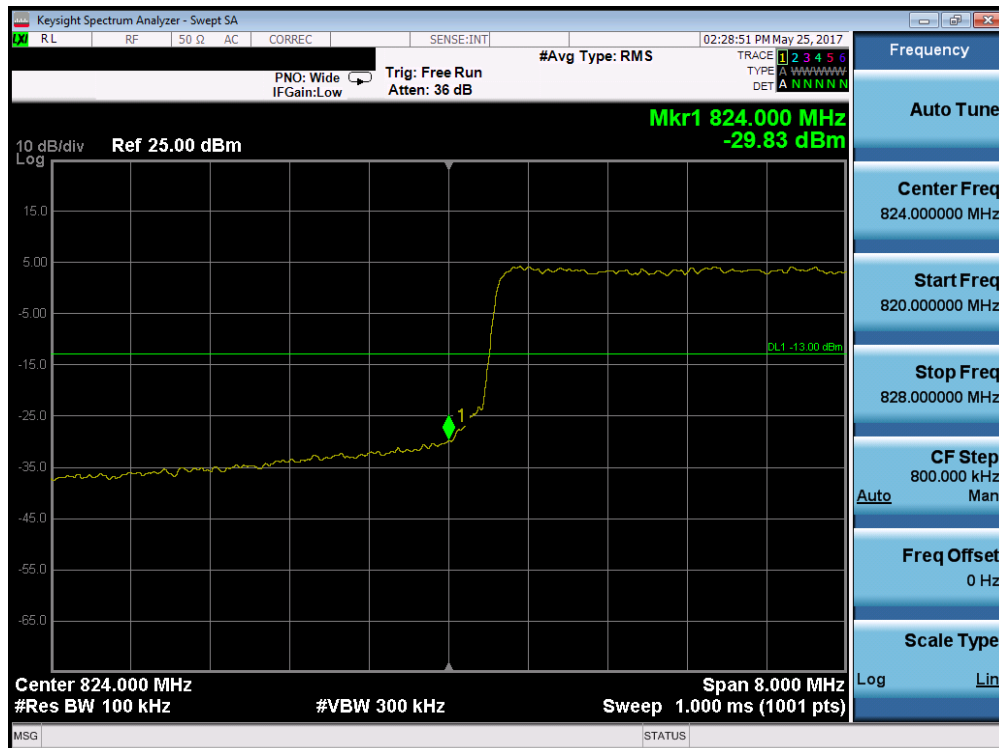
Plot 7-75. Lower Band Edge Plot (Band 5 – 10.0MHz QPSK – RB Size 50)
