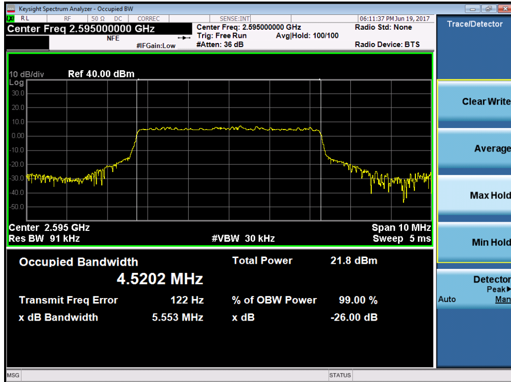
Plot 7-21. Occupied Bandwidth Plot (Band 38 – 5.0MHz QPSK – RB Size 25)
