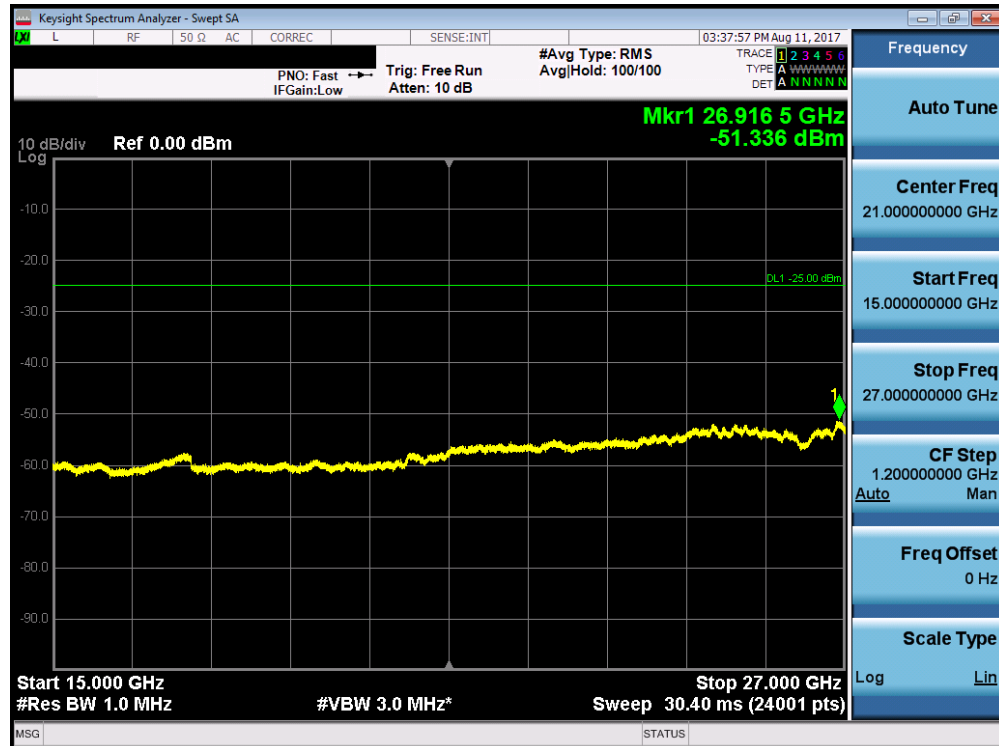
Plot 7-52. Conducted Spurious Plot (Band 7 – 5.0MHz QPSK – RB Size 1, RB Offset 0 – Mid Channel)
