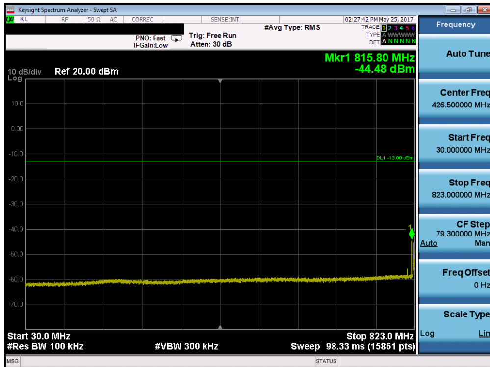
Plot 7-38. Conducted Spurious Plot (Band 5 – 10.0MHz QPSK – RB Size 1, RB Offset 0– Low Channel)
