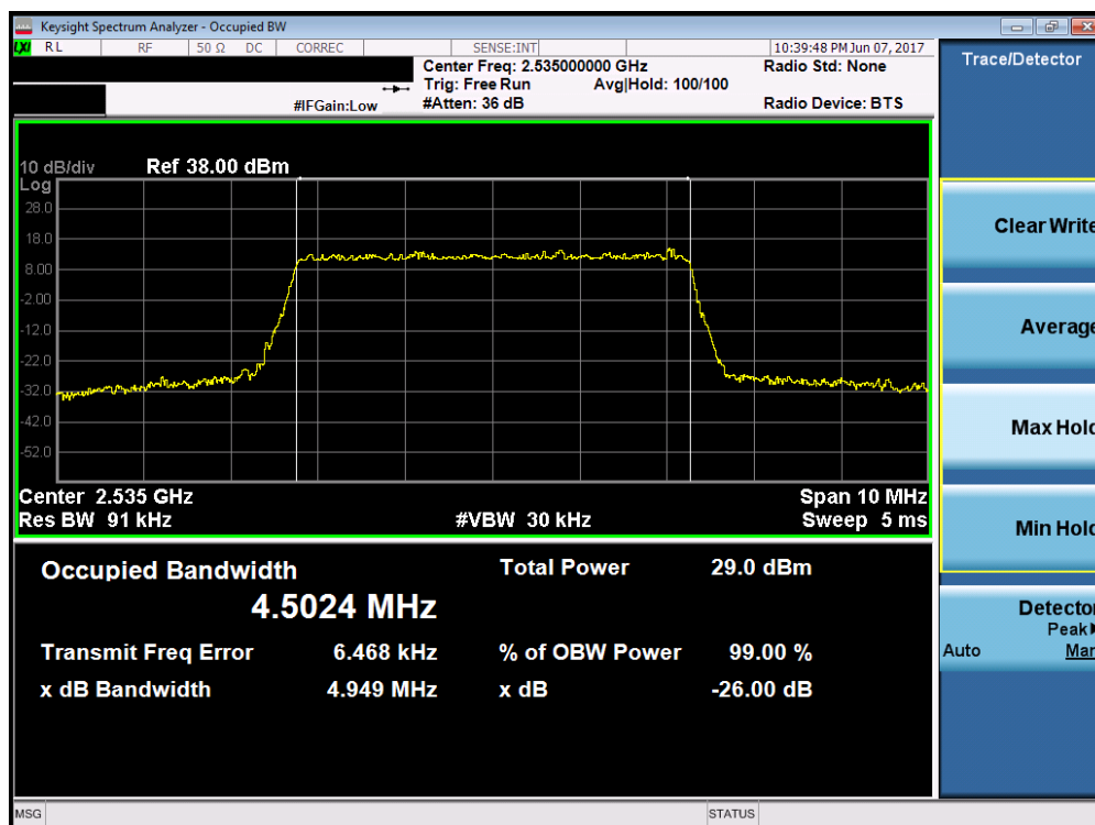
Plot 7-14. Occupied Bandwidth Plot (Band 7 – 5.0MHz 16-QAM – RB Size 25)
