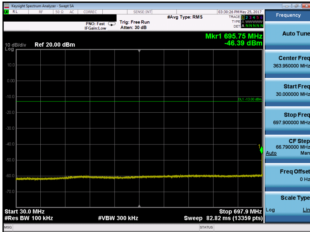
Plot 7-29. Conducted Spurious Plot (Band 17 – 10.0MHz QPSK – RB Size 1, RB Offset 0– Low Channel)
