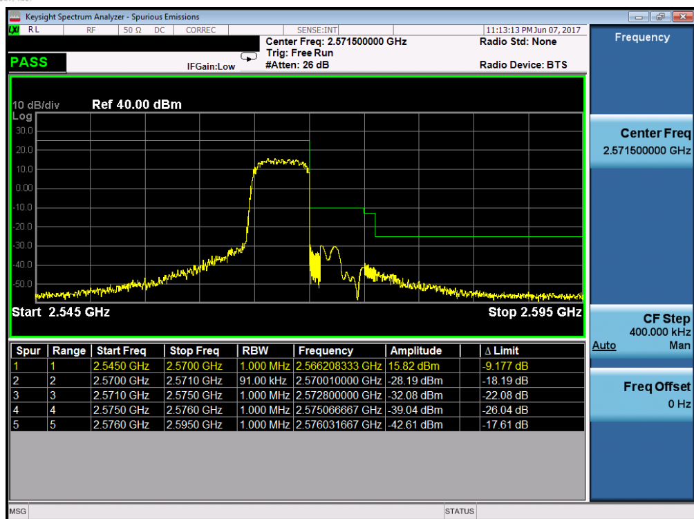
Plot 7-78. Upper ACP Plot (Band 7 – 5.0MHz QPSK – RB Size 25)
