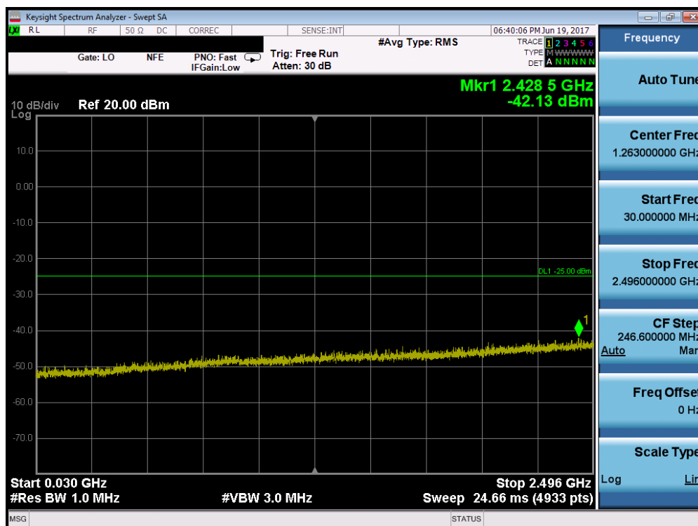
Plot 7-62. Conducted Spurious Plot (Band 38 – 5.0MHz QPSK – RB Size 1, RB Offset 0 – High Channel)
