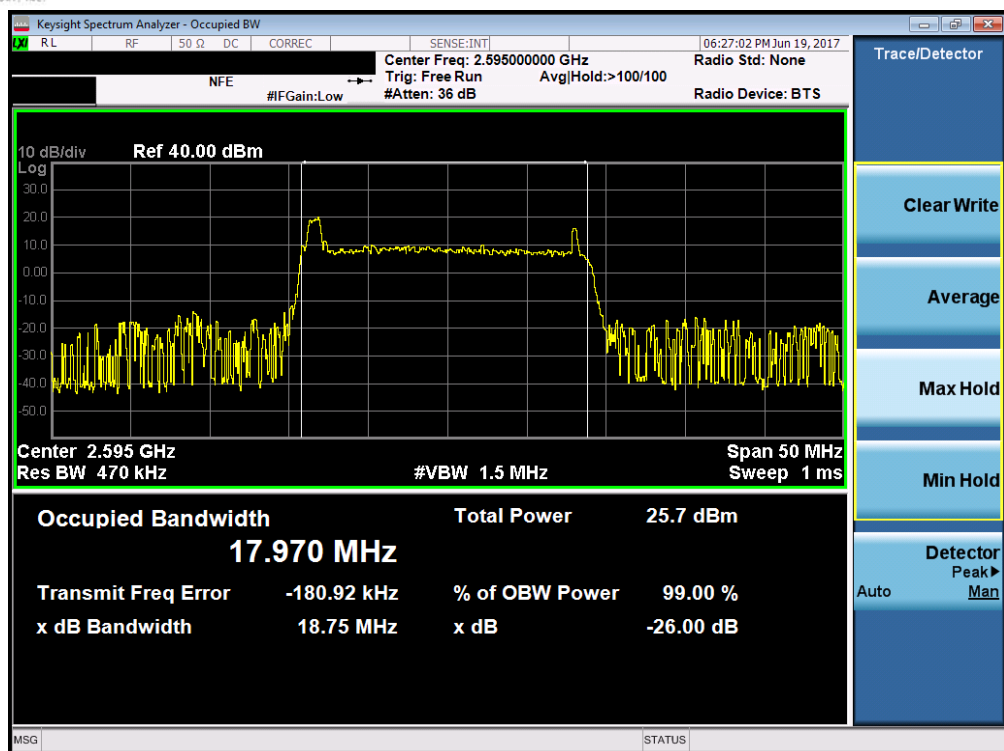
Plot 7-27. Occupied Bandwidth Plot (Band 38 – 20.0MHz QPSK – RB Size 100)
