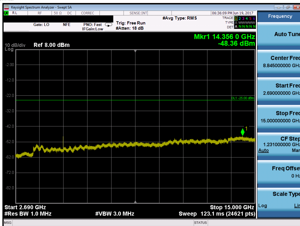
Plot 7-57. Conducted Spurious Plot (Band 38 – 5.0MHz QPSK – RB Size 1, RB Offset 0 – Low Channel)
