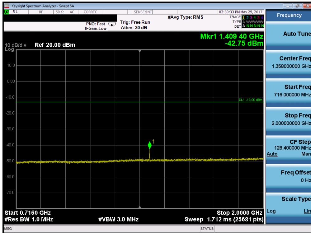
Plot 7-30. Conducted Spurious Plot (Band 17 – 10.0MHz QPSK – RB Size 1, RB Offset 0 – Low Channel)
