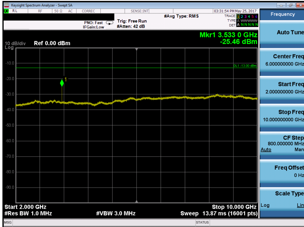
Plot 7-37. Conducted Spurious Plot (Band 17 – 10.0MHz QPSK – RB Size 1, RB Offset 0 – High Channel)
