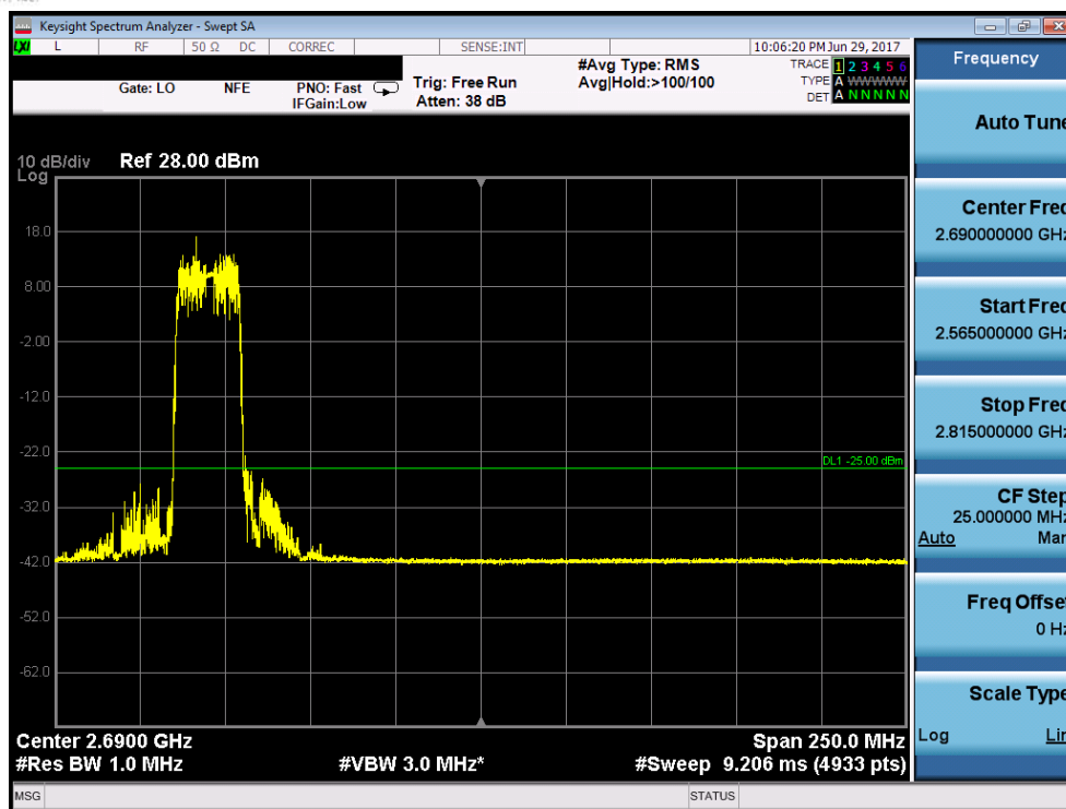
Plot 7-92. Upper Band Edge Plot (Band 38 – 20.0MHz QPSK – RB Size 100)
