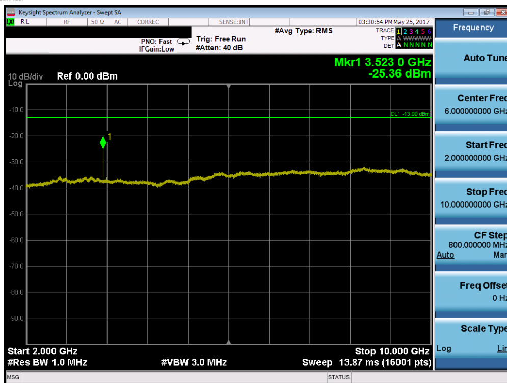
Plot 7-31. Conducted Spurious Plot (Band 17 – 10.0MHz QPSK – RB Size 1, RB Offset 0 – Low Channel)
