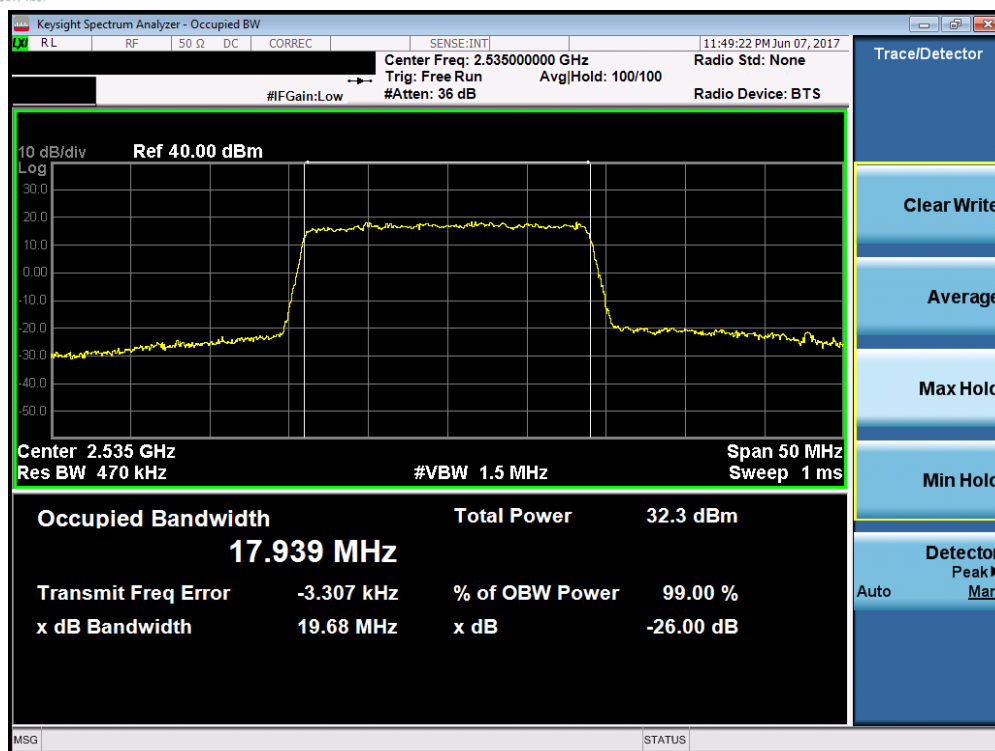
Plot 7-19. Occupied Bandwidth Plot (Band 7 – 20.0MHz QPSK – RB Size 100)
