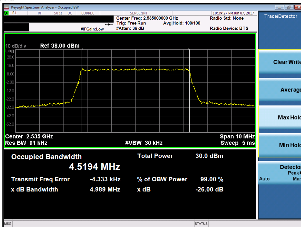
Plot 7-13. Occupied Bandwidth Plot (Band 7 – 5.0MHz QPSK – RB Size 25)
