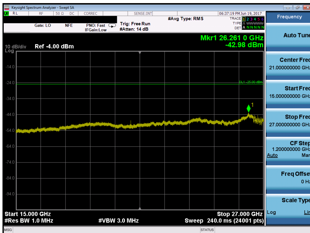
Plot 7-58. Conducted Spurious Plot (Band 38 – 5.0MHz QPSK – RB Size 1, RB Offset 0 – Low Channel)
