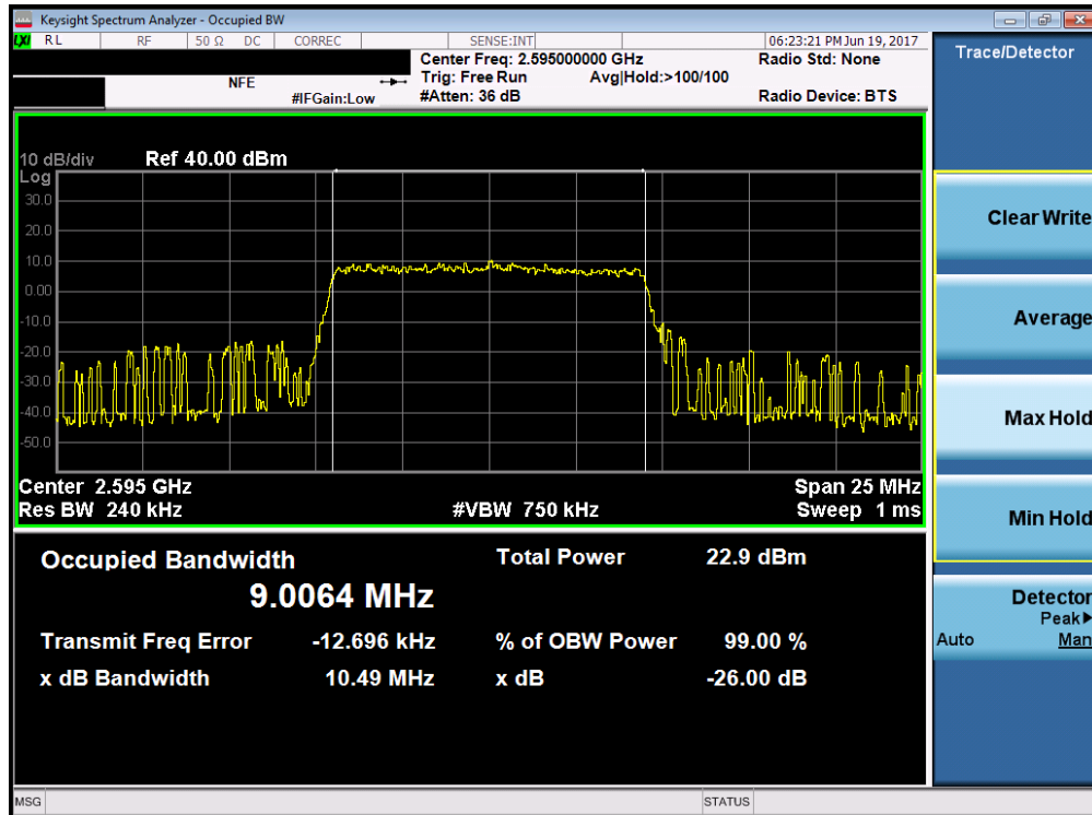
Plot 7-24. Occupied Bandwidth Plot (Band 38 – 10.0MHz 16-QAM – RB Size 50)
