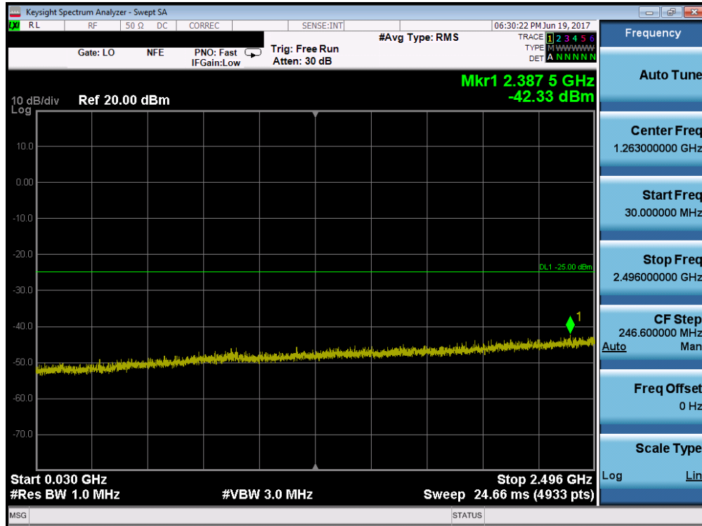
Plot 7-59. Conducted Spurious Plot (Band 38 – 5.0MHz QPSK – RB Size 1, RB Offset 0 – Mid Channel)
