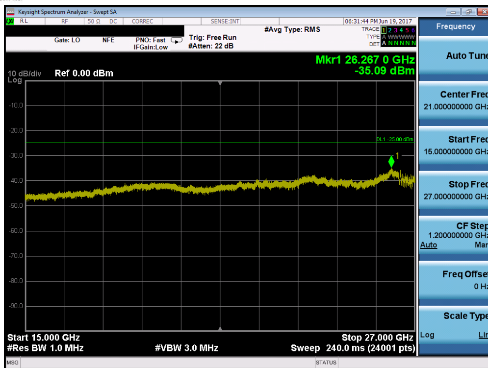
Plot 7-61. Conducted Spurious Plot (Band 38 – 5.0MHz QPSK – RB Size 1, RB Offset 0 – Mid Channel)
