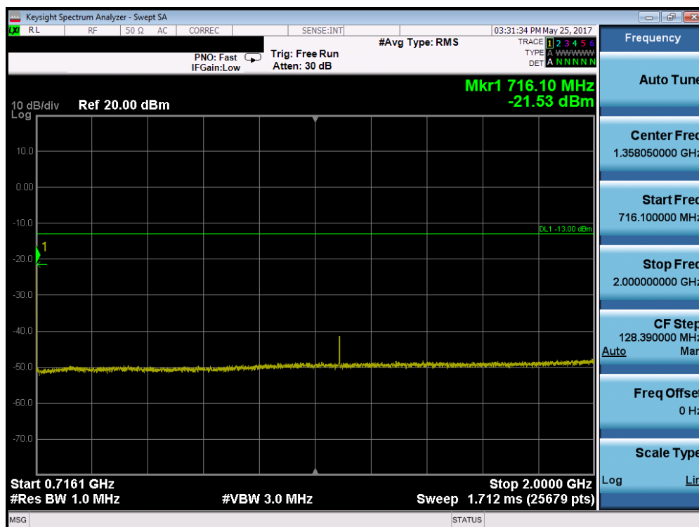
Plot 7-36. Conducted Spurious Plot (Band 17 – 10.0MHz QPSK – RB Size 1, RB Offset 0 – High Channel)
