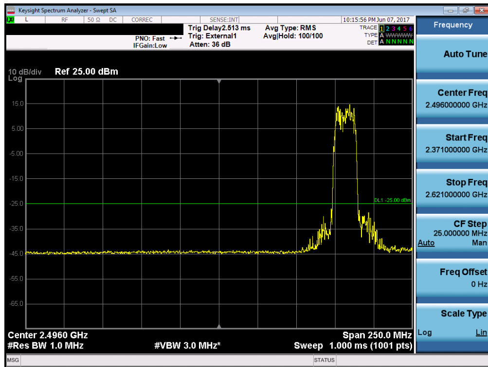
Plot 7-89. Lower Band Edge Plot (Band 38 – 15.0MHz QPSK – RB Size 75)
