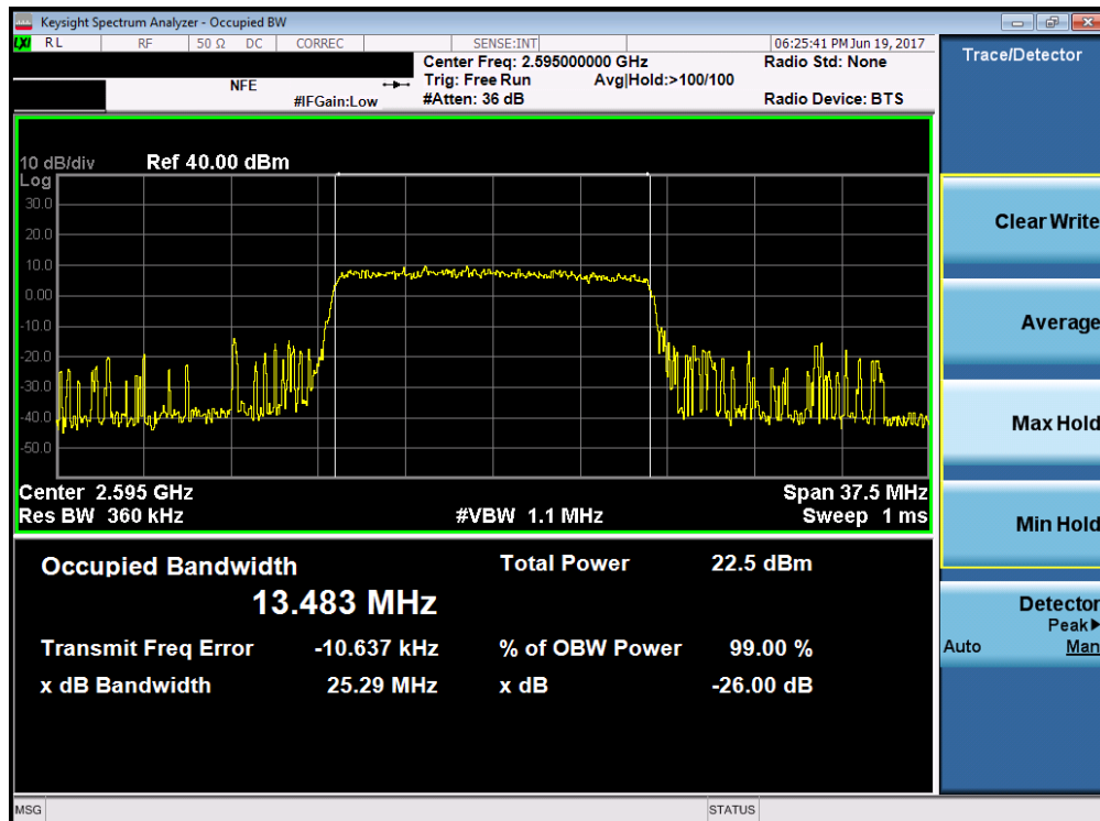
Plot 7-26. Occupied Bandwidth Plot (Band 38 – 15.0MHz 16-QAM – RB Size 75)
