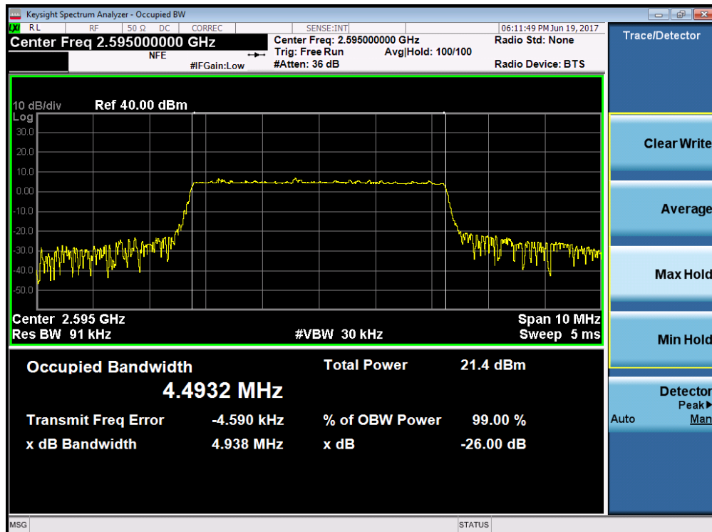
Plot 7-22. Occupied Bandwidth Plot (Band 38 – 5.0MHz 16-QAM – RB Size 25)
