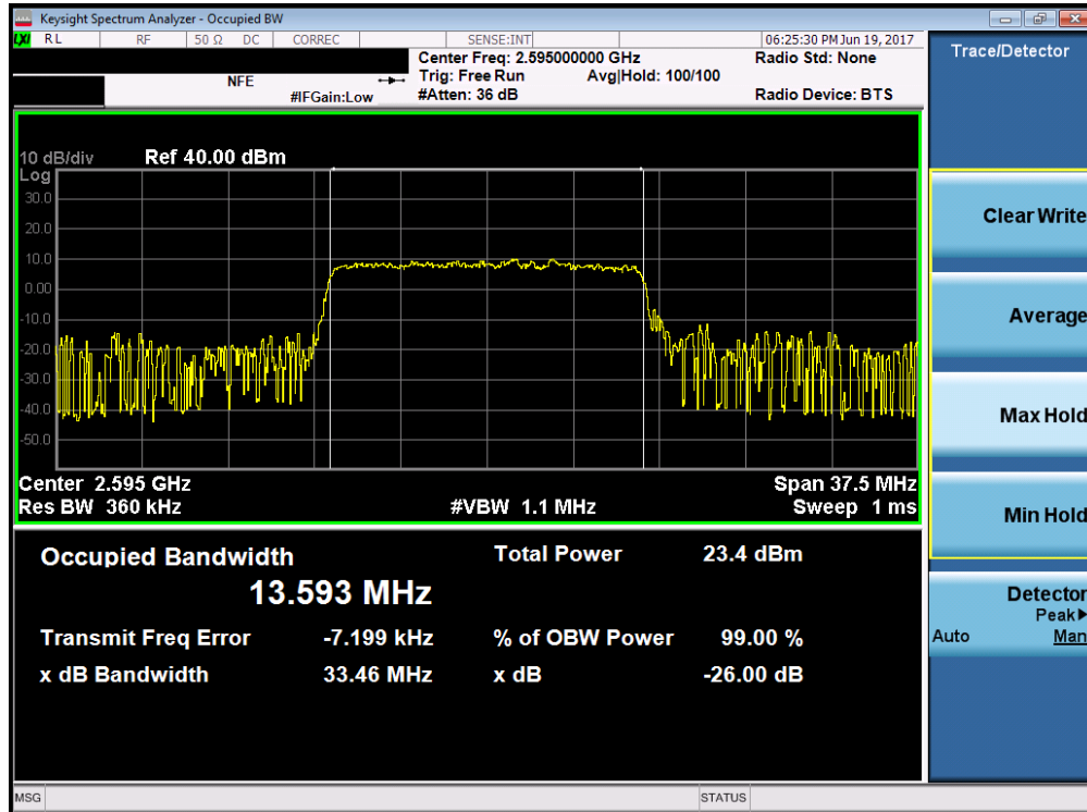
Plot 7-25. Occupied Bandwidth Plot (Band 38 – 15.0MHz QPSK – RB Size 75)
