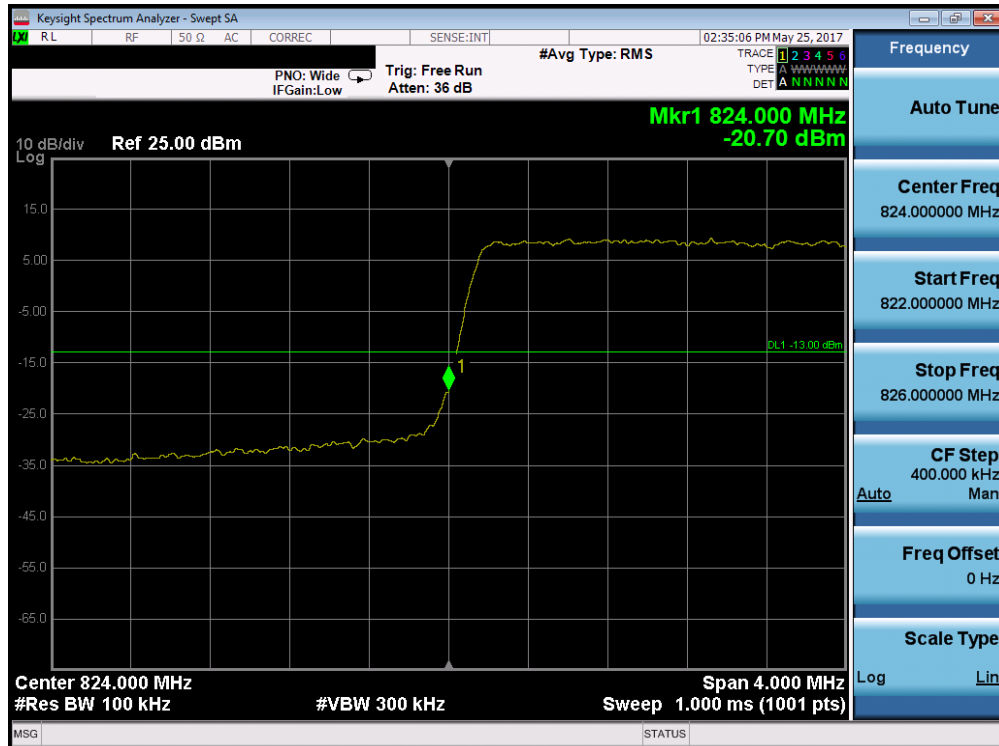
Plot 7-71. Lower Band Edge Plot (Band 5 – 3.0MHz QPSK – RB Size 15)
