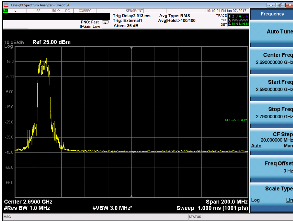
Plot 7-88. Upper Band Edge Plot (Band 38 – 10.0MHz QPSK – RB Size 50)
