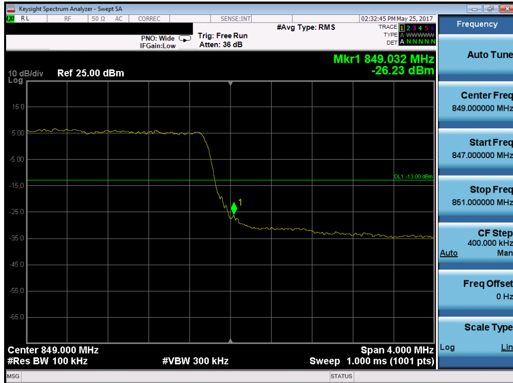
Plot 7-74. Upper Band Edge Plot (Band 5 – 5.0MHz QPSK – RB Size 25)
