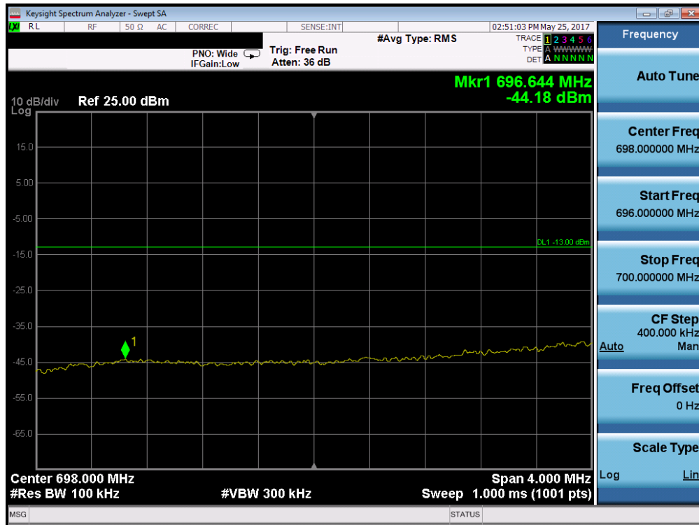
Plot 7-65. Lower Band Edge Plot (Band 17 – 5.0MHz QPSK – RB Size 25)
