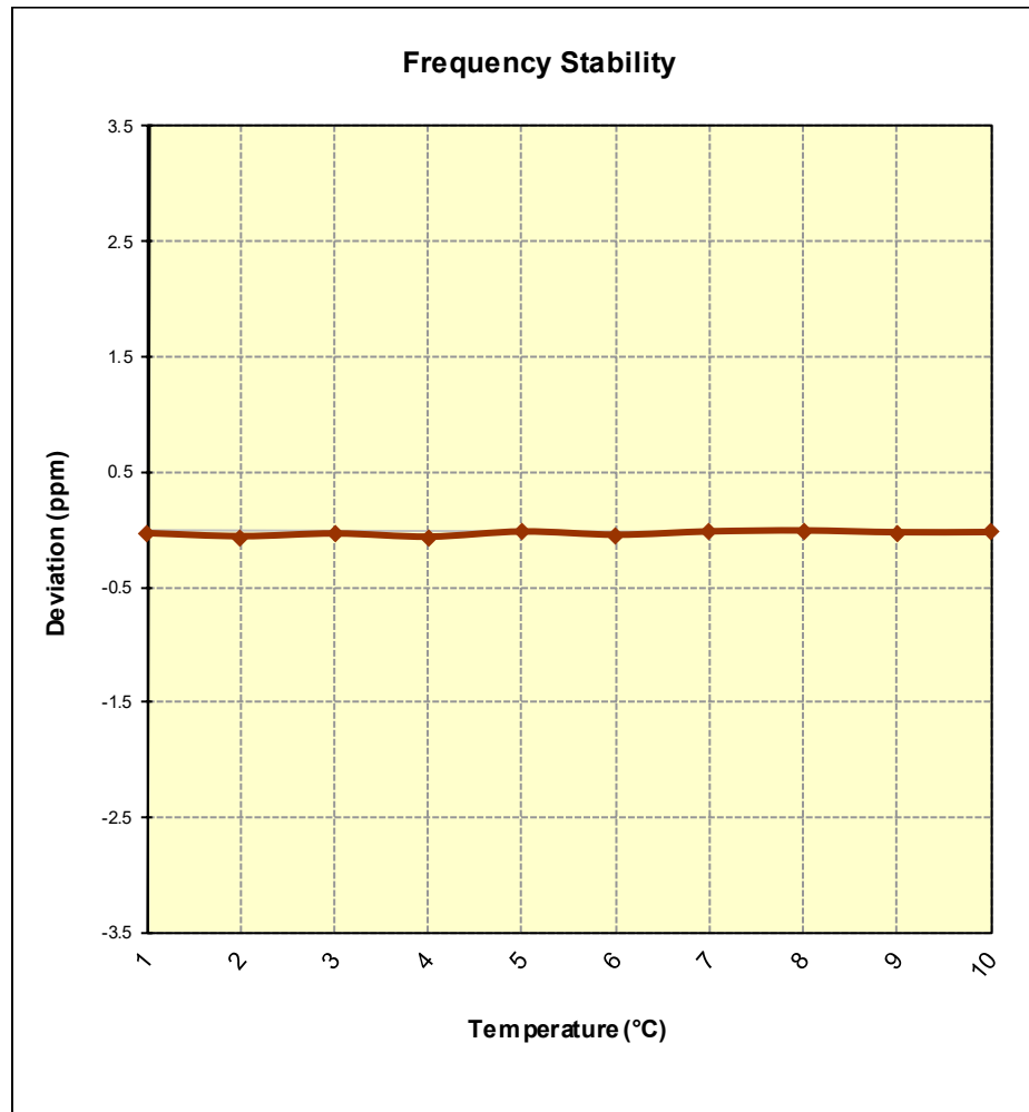
Figure 7-10. Frequency Stability Graph (Band 38)
