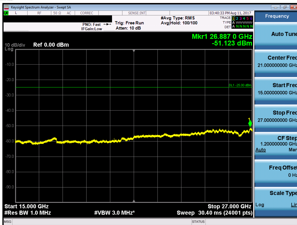
Plot 7-49. Conducted Spurious Plot (Band 7 – 5.0MHz QPSK – RB Size 1, RB Offset 0 – Low Channel)
