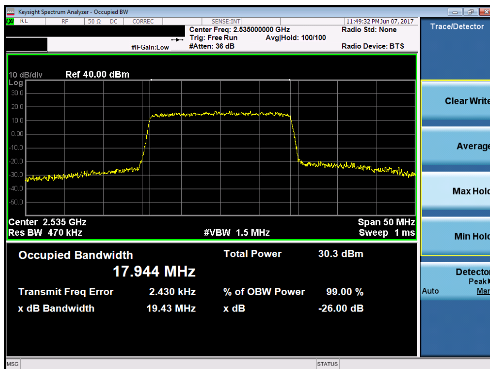
Plot 7-20. Occupied Bandwidth Plot (Band 7 – 20.0MHz 16-QAM – RB Size 100)
