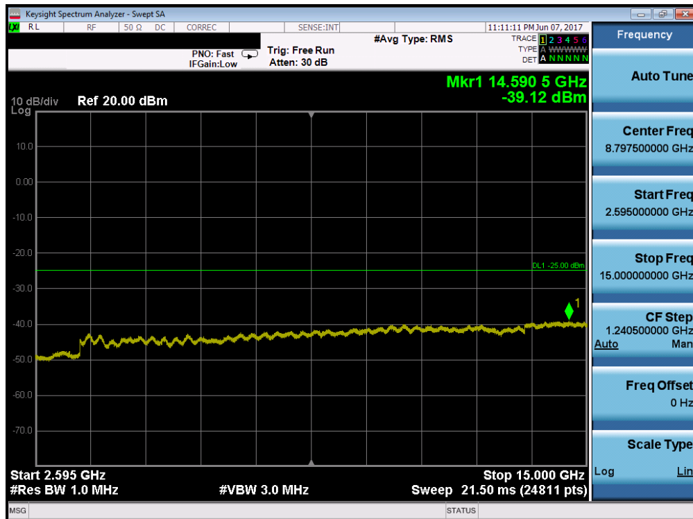
Plot 7-54. Conducted Spurious Plot (Band 7 – 5.0MHz QPSK – RB Size 1, RB Offset 0 – High Channel)
