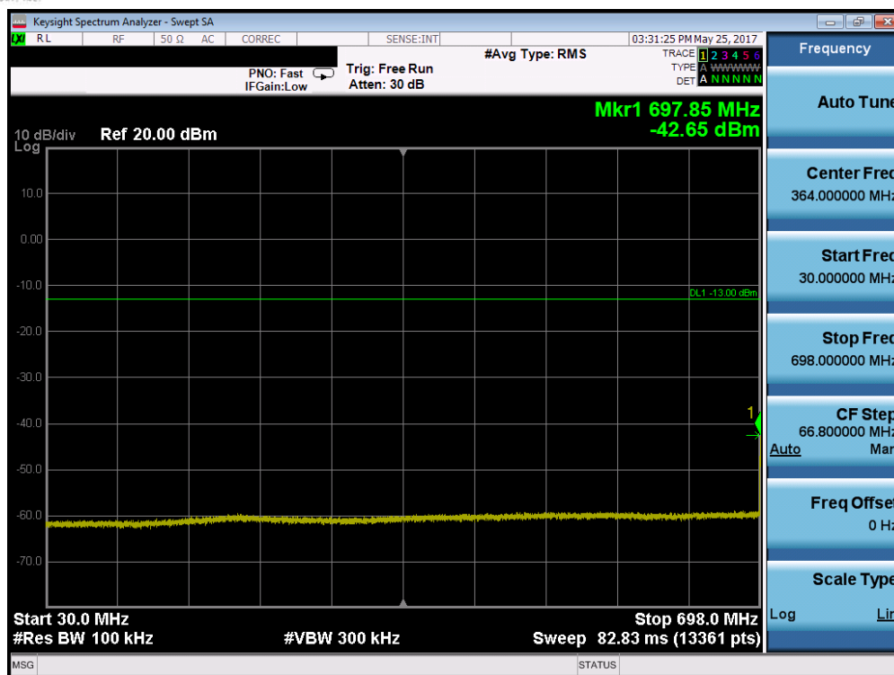
Plot 7-35. Conducted Spurious Plot (Band 17 – 10.0MHz QPSK – RB Size 1, RB Offset 0 – High Channel)
