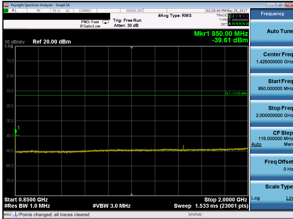
Plot 7-45. Conducted Spurious Plot (Band 5 – 10.0MHz QPSK – RB Size 1, RB Offset 0 – High Channel)
