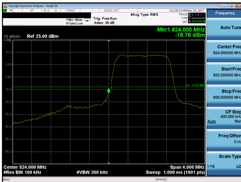
Plot 7-69. Lower Band Edge Plot (Band 5 – 1.4MHz QPSK – RB Size 6)
