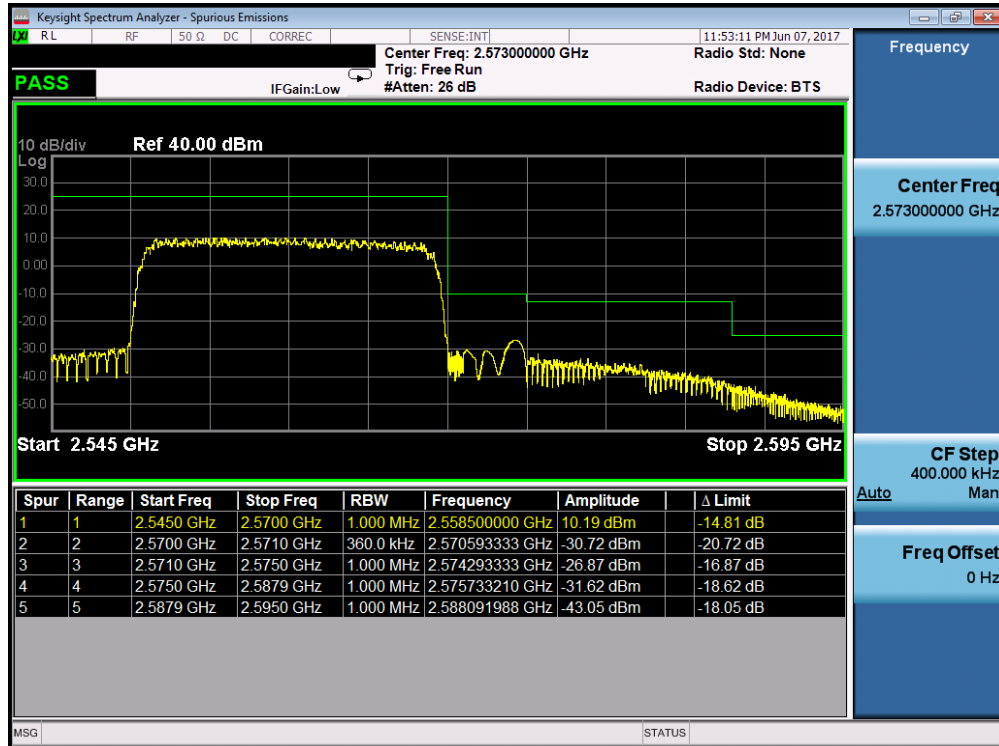
Plot 7-84. Upper ACP Plot (Band 7 – 20.0MHz QPSK – RB Size 100)
