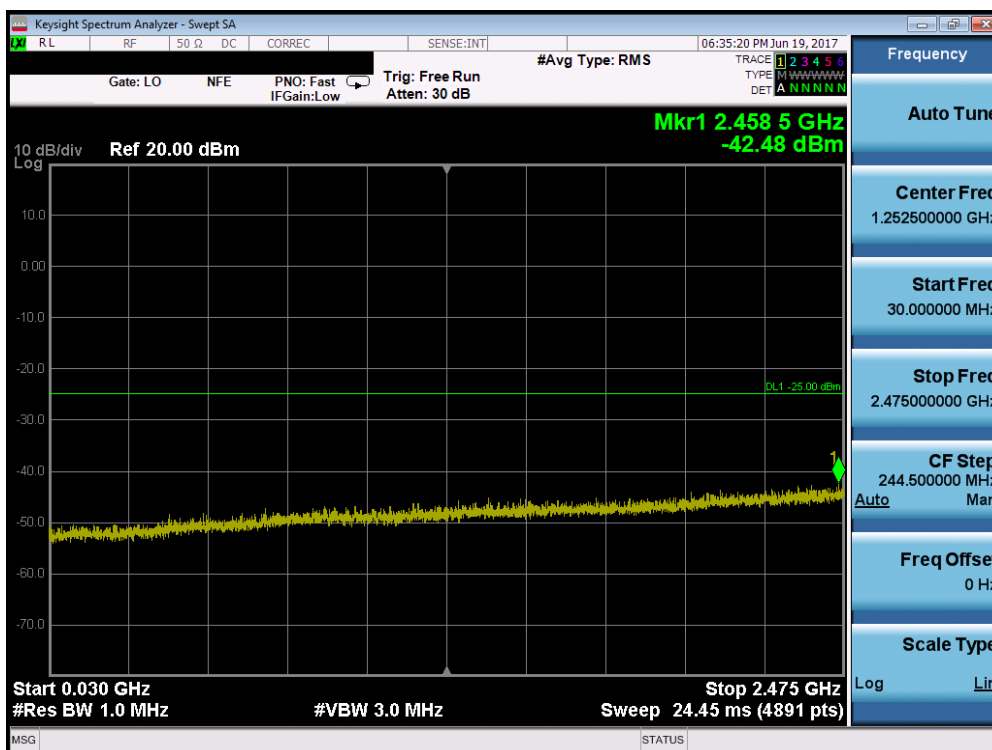
Plot 7-56. Conducted Spurious Plot (Band 38 – 5.0MHz QPSK – RB Size 1, RB Offset 0 – Low Channel)
