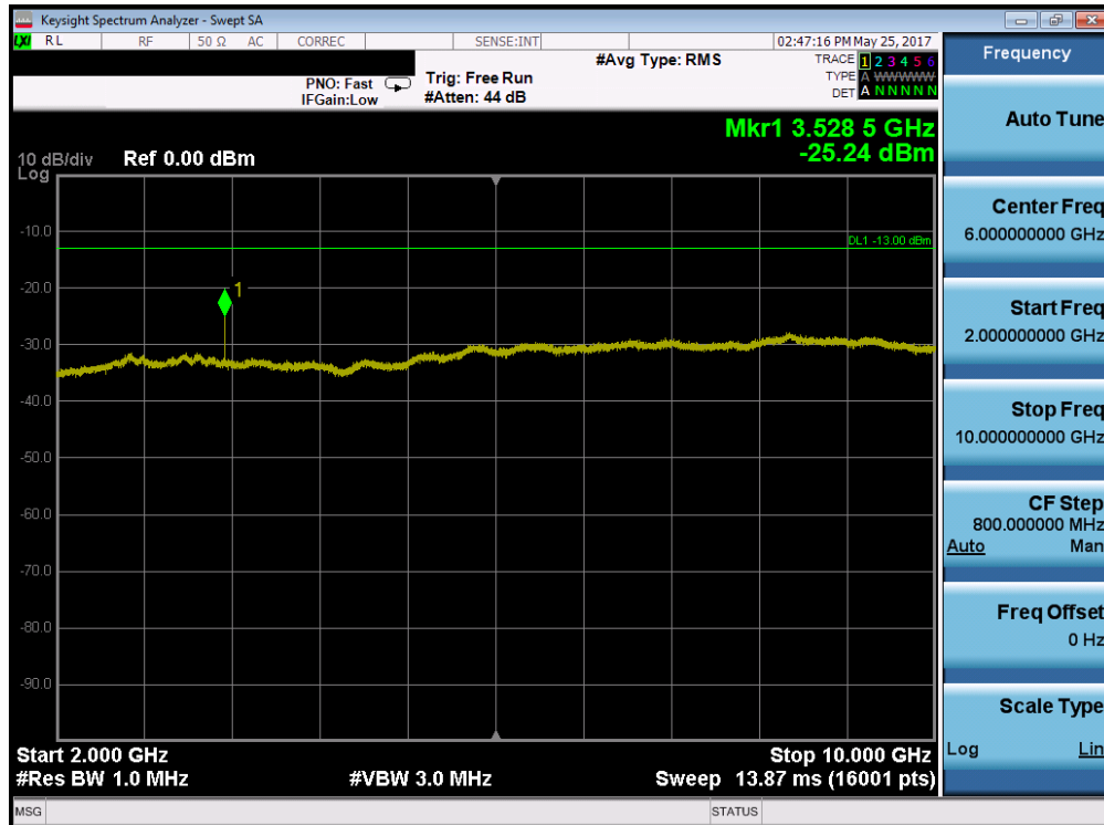
Plot 7-34. Conducted Spurious Plot (Band 17 – 10.0MHz QPSK – RB Size 1, RB Offset 0 – Mid Channel)
