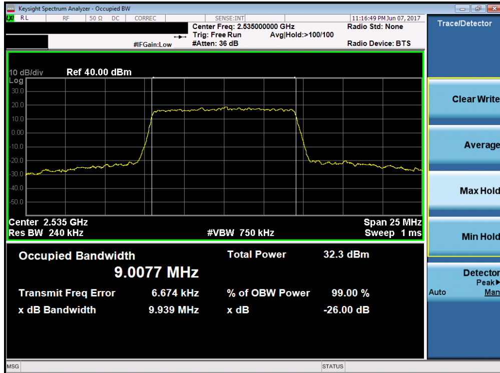
Plot 7-15. Occupied Bandwidth Plot (Band 7 – 10.0MHz QPSK – RB Size 50)
