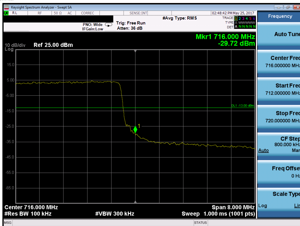
Plot 7-68. Upper Band Edge Plot (Band 17 – 10.0MHz QPSK – RB Size 50)
