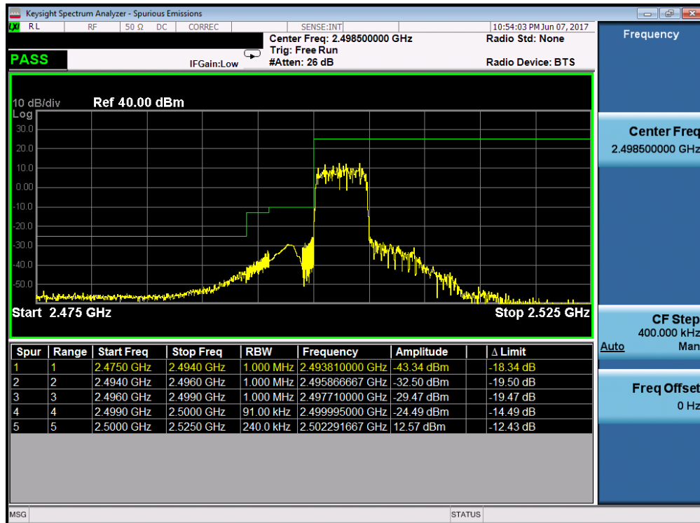
Plot 7-77. Lower ACP Plot (Band 7 – 5.0MHz QPSK – RB Size 25)
