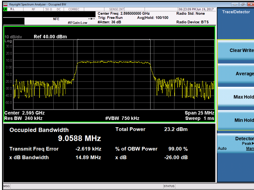
Plot 7-23. Occupied Bandwidth Plot (Band 38 – 10.0MHz QPSK – RB Size 50)
