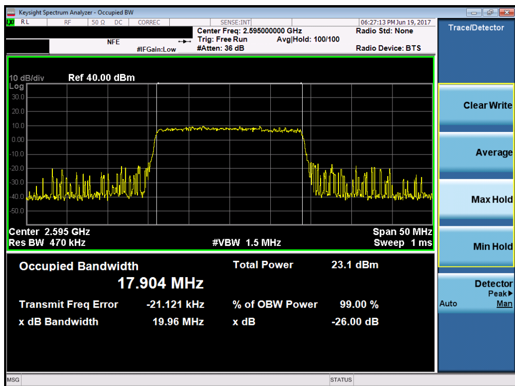
Plot 7-28. Occupied Bandwidth Plot (Band 38 – 20.0MHz 16-QAM – RB Size 100)
