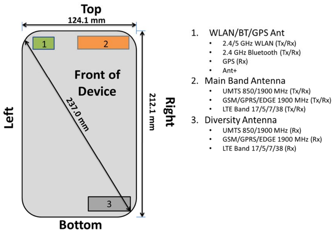
Figure F-1 DUT Antenna Locations
