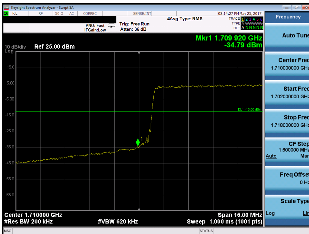
Plot 7-131. Lower Band Edge Plot (Band 4 - 20.0MHz QPSK - RB Size 100)
