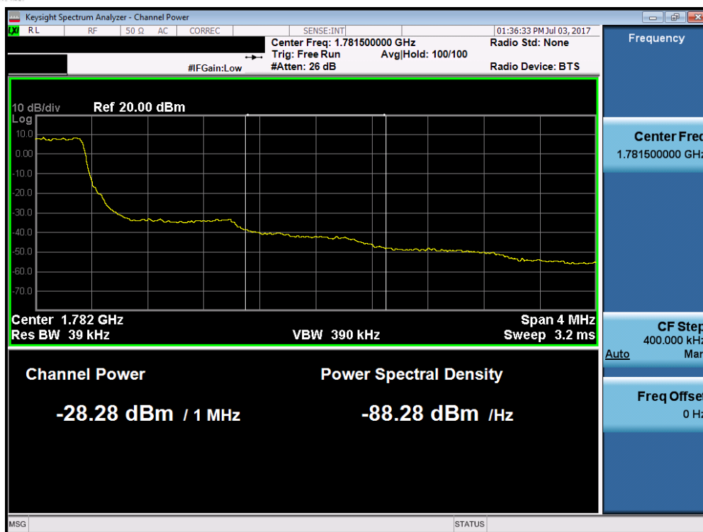
Plot 7-138. Upper Extended Band Edge Plot (Band 66 – 1.4MHz QPSK – RB Size 6)
