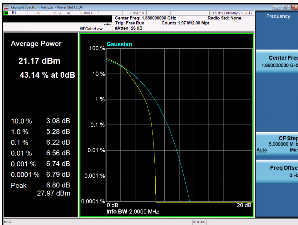
Plot 7-192. PAR Plot (Band 2 – 1.4MHz 16-QAM – RB Size 6)
