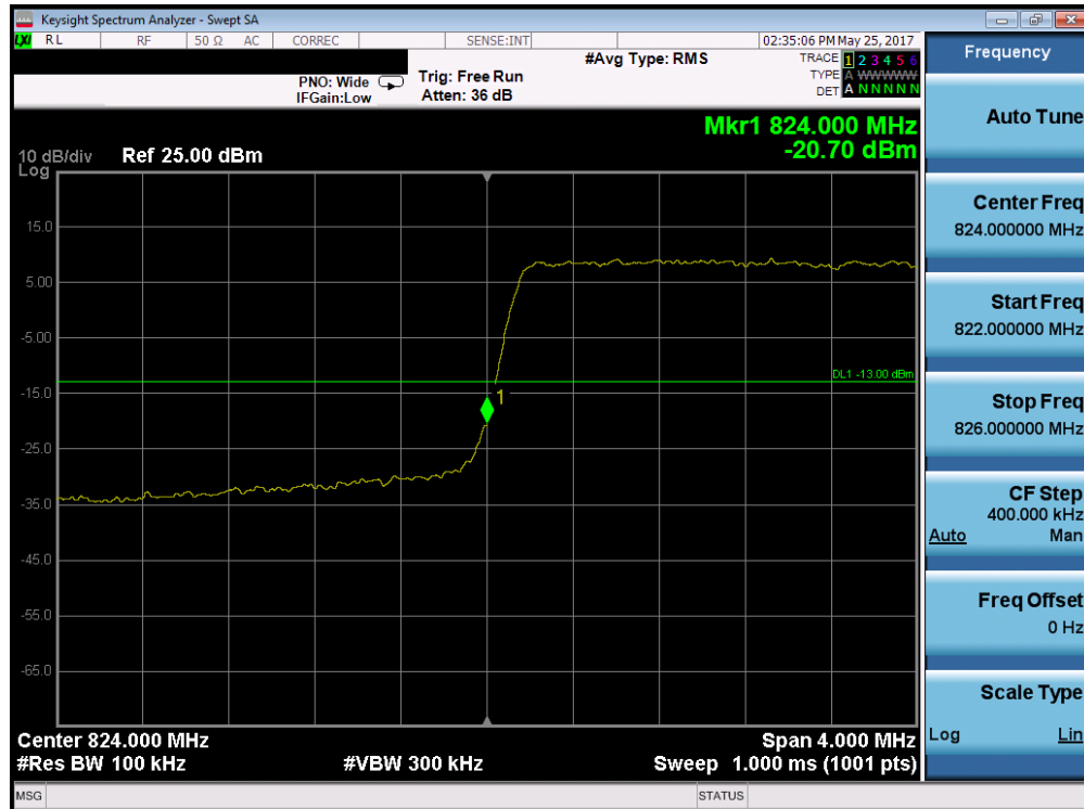
Plot 7-105. Lower Band Edge Plot (Band 5 - 3.0MHz QPSK - RB Size 15)
