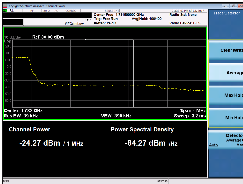
Plot 7-142. Upper Extended Band Edge Plot (Band 66 – 3.0MHz QPSK – RB Size 15)
