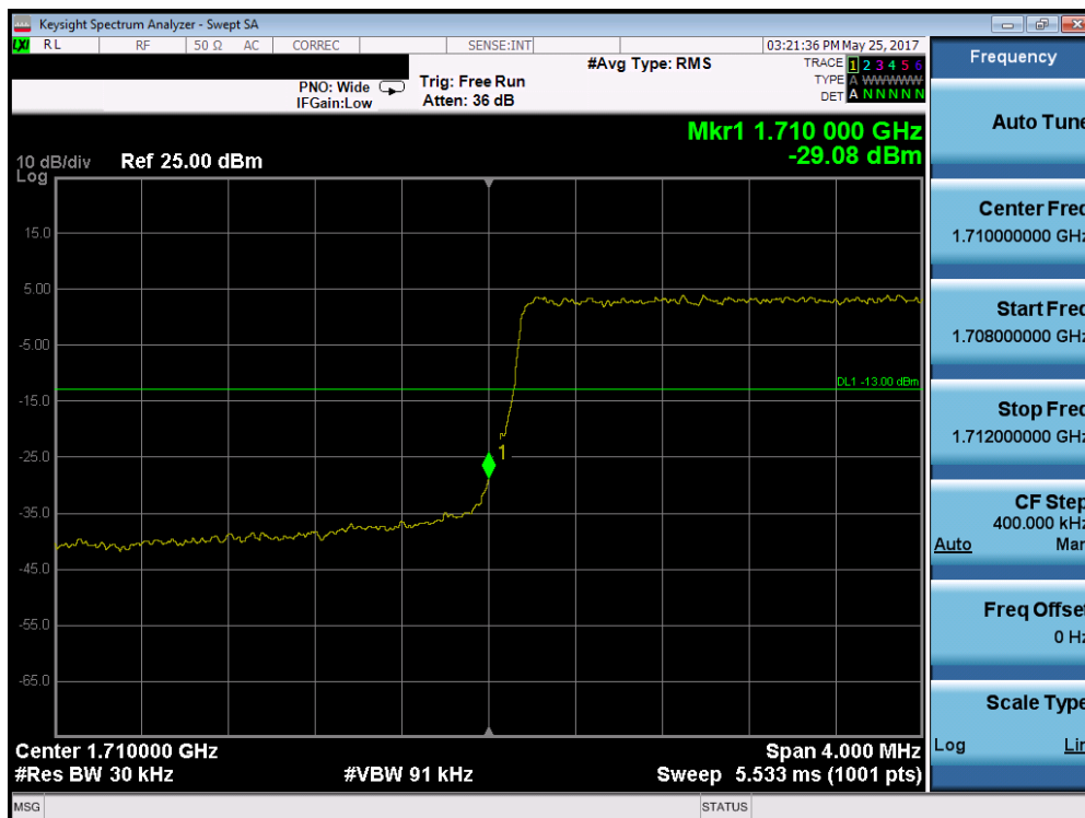
Plot 7-115. Lower Band Edge Plot (Band 4 – 3.0MHz QPSK – RB Size 15)
