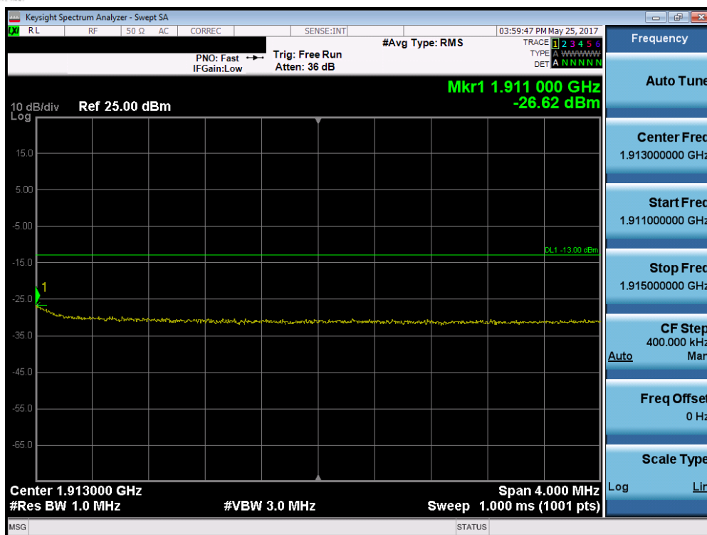
Plot 7-174. Upper Extended Band Edge Plot (Band 2 - 10.0MHz QPSK - RB Size 50)
