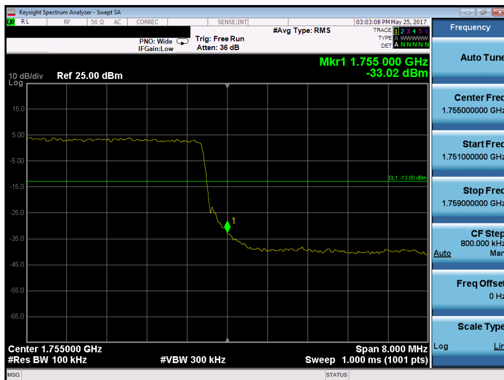
Plot 7-125. Upper Band Edge Plot (Band 4 – 10.0MHz QPSK – RB Size 50)
