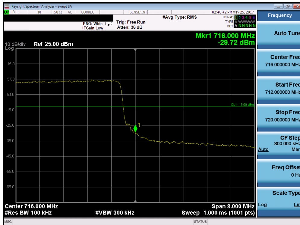
Plot 7-102. Upper Band Edge Plot (Band 17 – 10.0MHz QPSK – RB Size 50)
