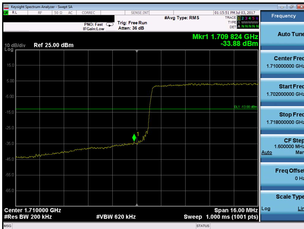
Plot 7-155. Lower Band Edge Plot (Band 66 – 20.0MHz QPSK – RB Size 100)
