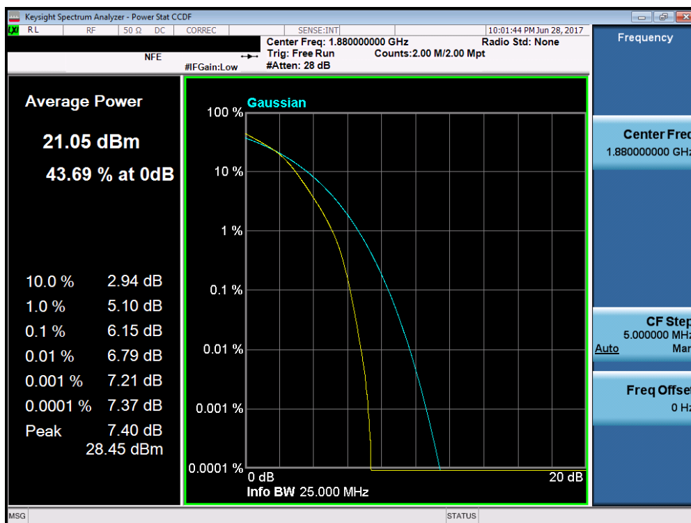
Plot 7-202. PAR Plot (Band 2 – 20.0MHz 16-QAM – RB Size 100)
