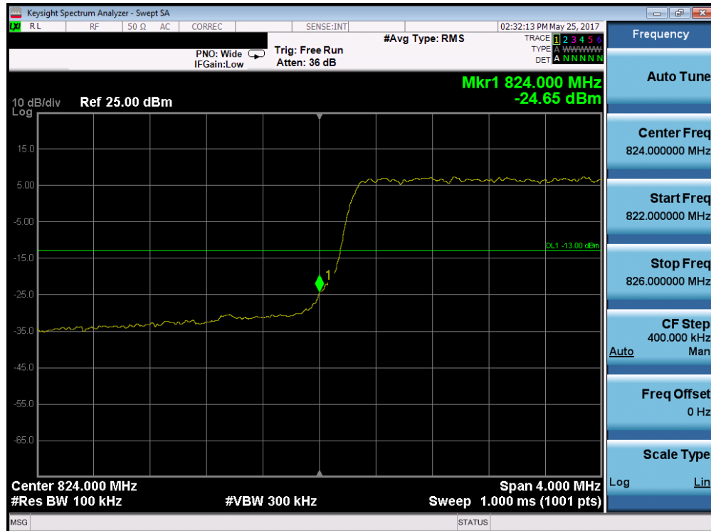
Plot 7-107. Lower Band Edge Plot (Band 5 - 5.0MHz QPSK - RB Size 25)
