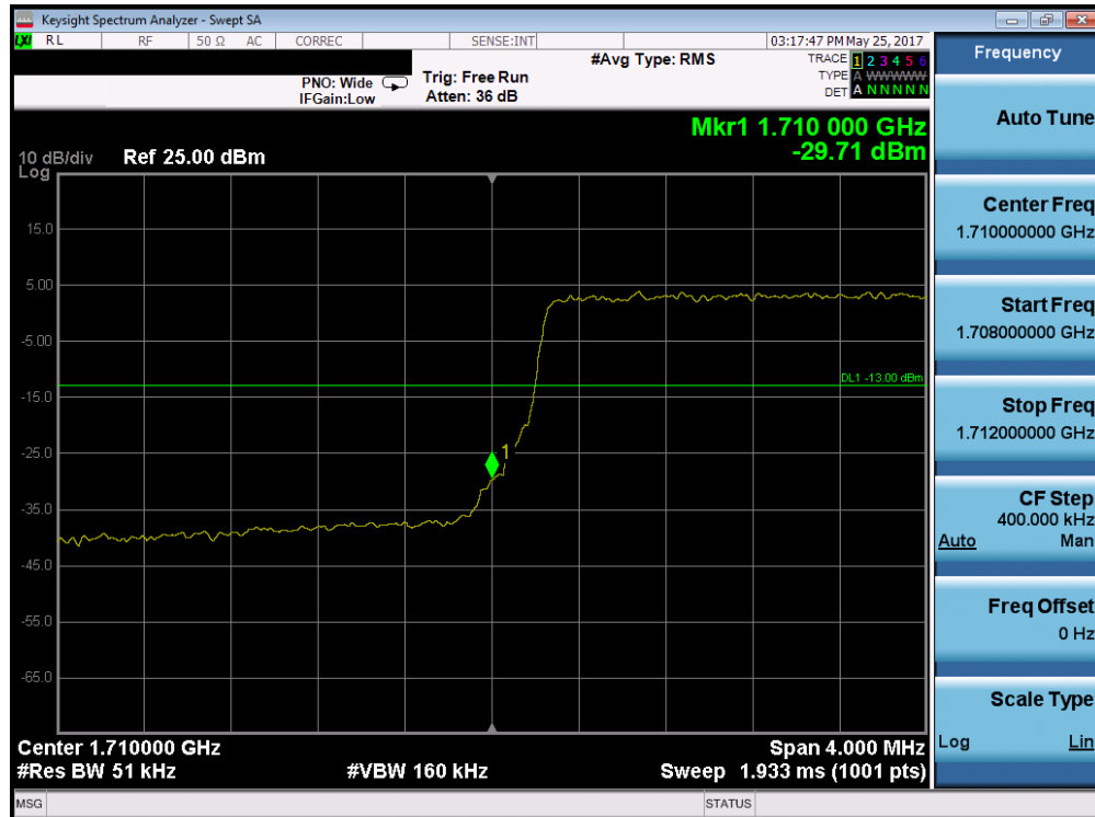
Plot 7-119. Lower Band Edge Plot (Band 4 – 5.0MHz QPSK – RB Size 25)
