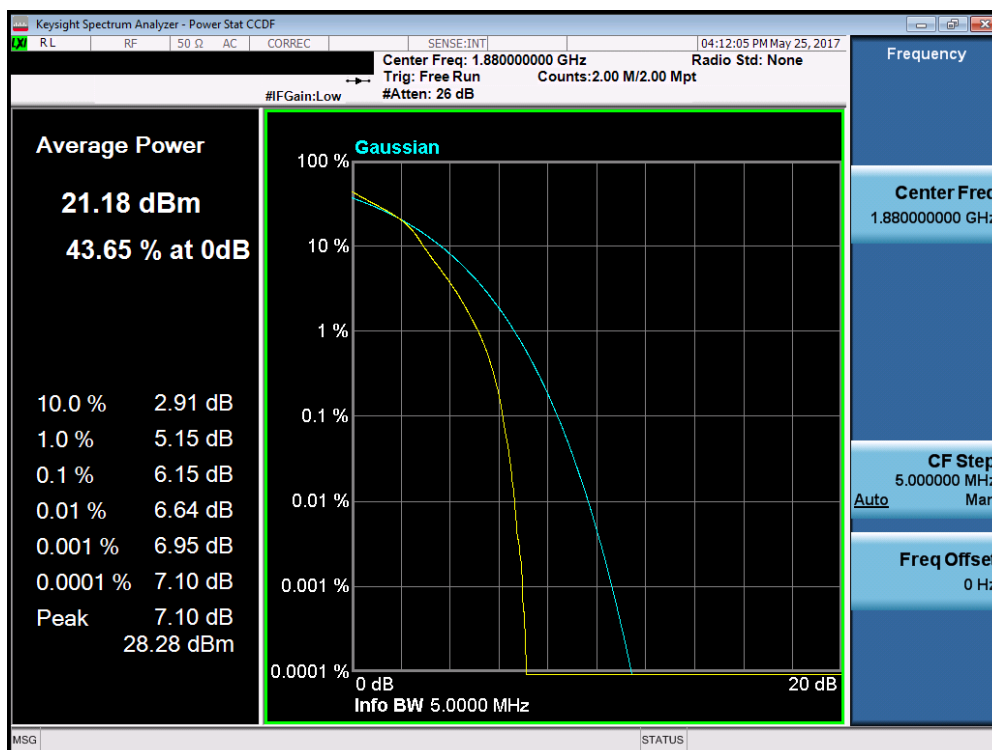
Plot 7-196. PAR Plot (Band 2 – 5.0MHz 16-QAM – RB Size 25)
