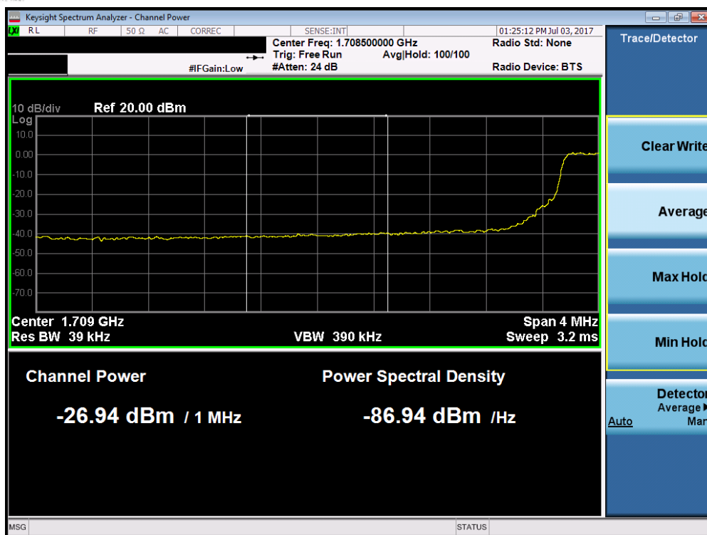
Plot 7-144. Lower Extended Band Edge Plot (Band 66 – 5.0MHz QPSK – RB Size 25)
