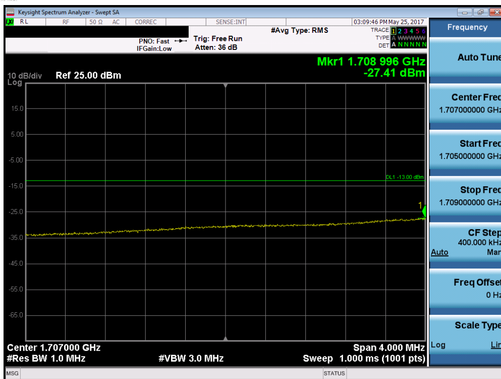
Plot 7-128. Lower Extended Band Edge Plot (Band 4 – 15.0MHz QPSK – RB Size 75)
