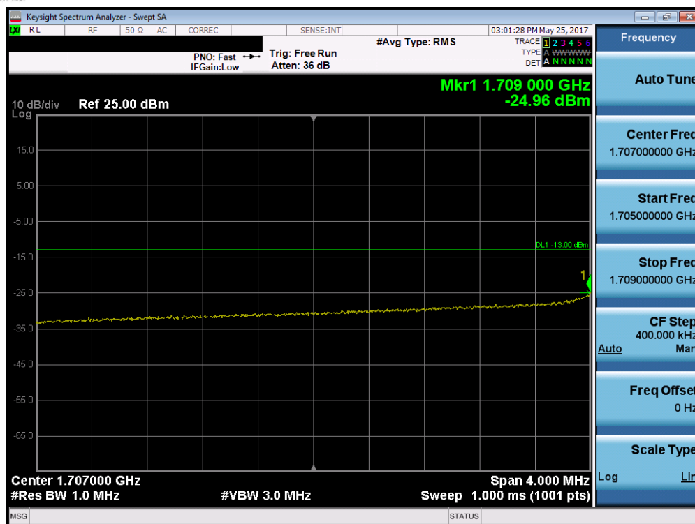
Plot 7-124. Lower Extended Band Edge Plot (Band 4 – 10.0MHz QPSK – RB Size 50)
