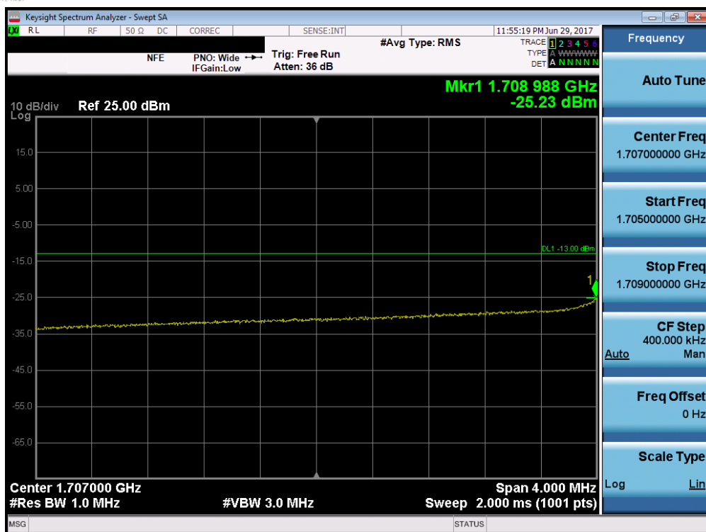
Plot 7-148. Lower Extended Band Edge Plot (Band 66 – 10.0MHz QPSK – RB Size 50)
