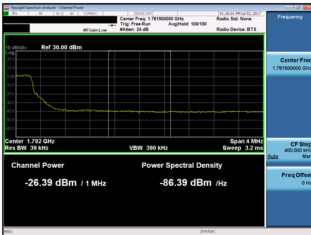
Plot 7-146. Upper Extended Band Edge Plot (Band 66 – 5.0MHz QPSK – RB Size 25)
