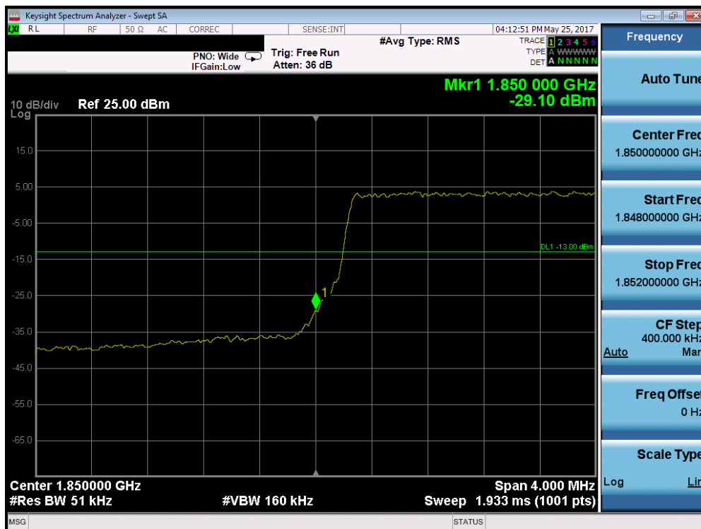
Plot 7-167. Lower Band Edge Plot (Band 2 – 5.0MHz QPSK – RB Size 25)
