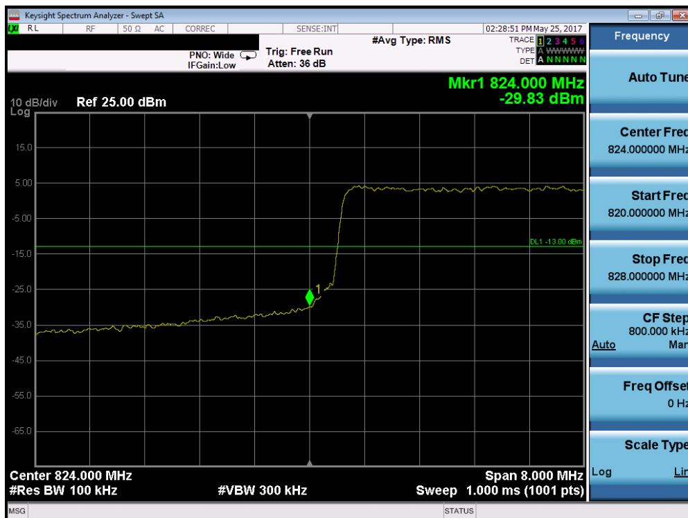
Plot 7-109. Lower Band Edge Plot (Band 5 - 10.0MHz QPSK - RB Size 50)
