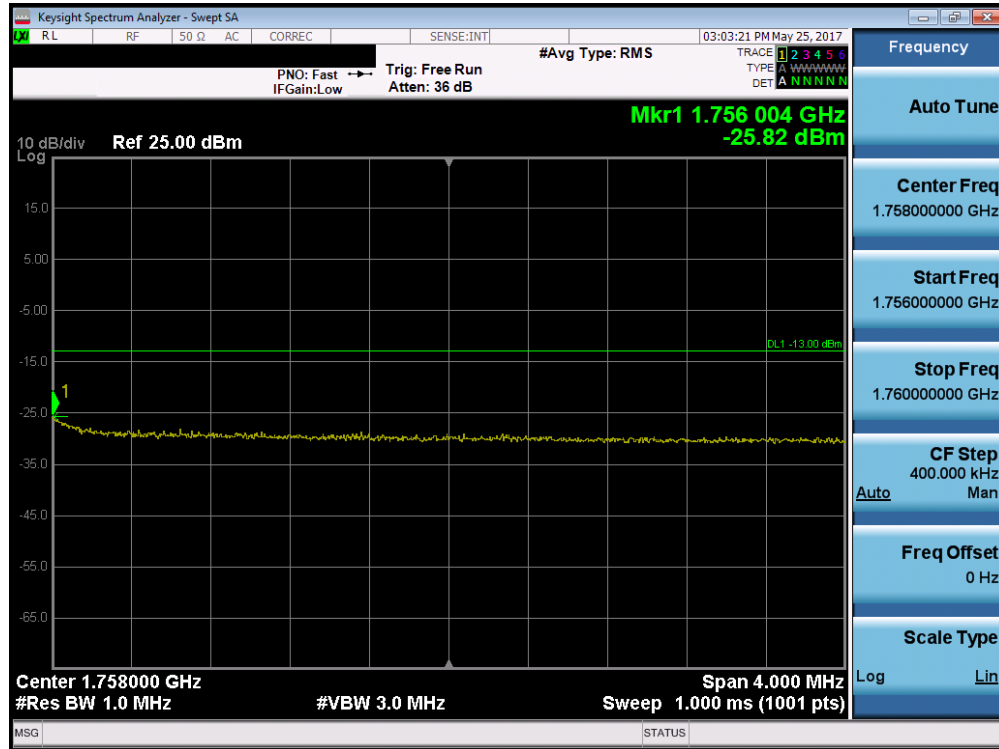
Plot 7-126. Upper Extended Band Edge Plot (Band 4 – 10.0MHz QPSK – RB Size 50)
