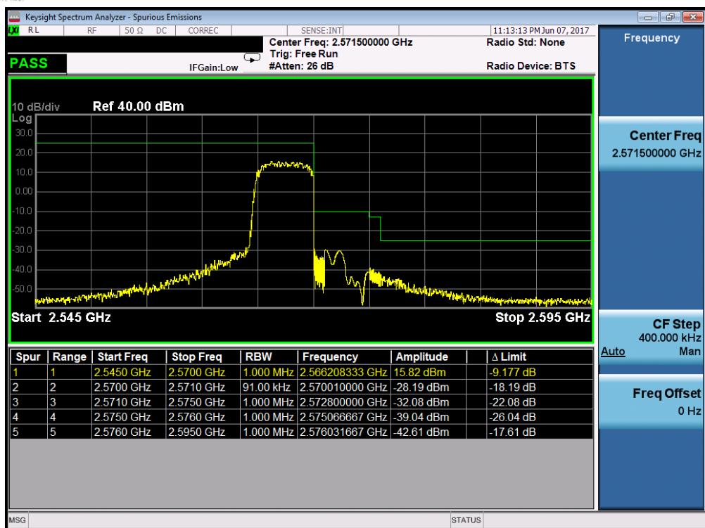
Plot 7-184. Upper ACP Plot (Band 7 – 5.0MHz QPSK – RB Size 25)
