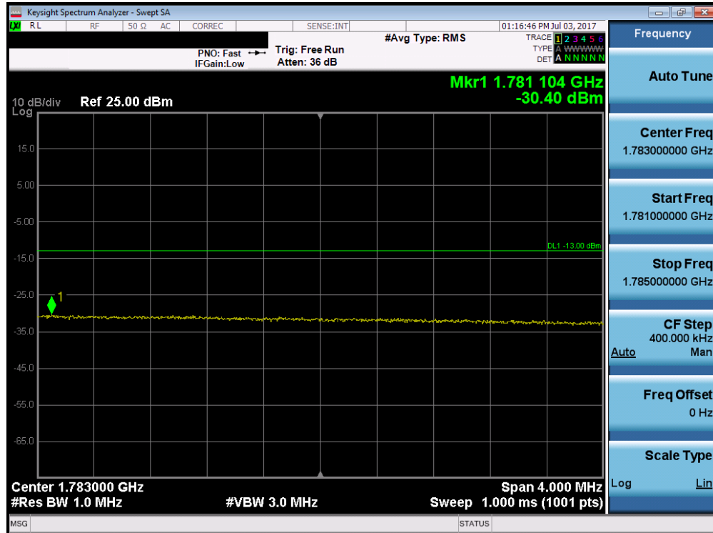
Plot 7-158. Upper Extended Band Edge Plot (Band 66 – 20.0MHz QPSK – RB Size 100)
