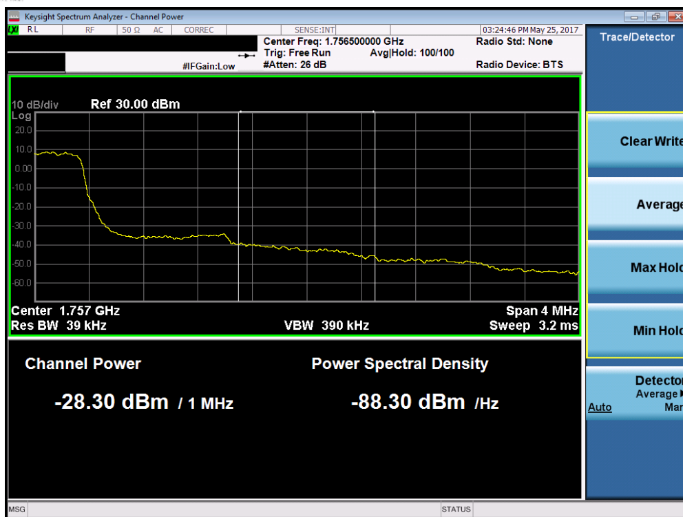
Plot 7-114. Upper Extended Band Edge Plot (Band 4 – 1.4MHz QPSK – RB Size 6)
