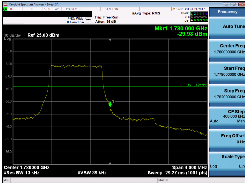
Plot 7-137. Upper Band Edge Plot (Band 66 – 1.4MHz QPSK – RB Size 6)
