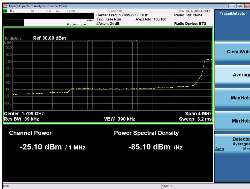
Plot 7-140. Lower Extended Band Edge Plot (Band 66 – 3.0MHz QPSK – RB Size 15)
