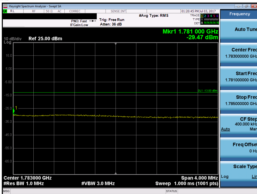
Plot 7-154. Upper Extended Band Edge Plot (Band 66 – 15.0MHz QPSK – RB Size 75)
