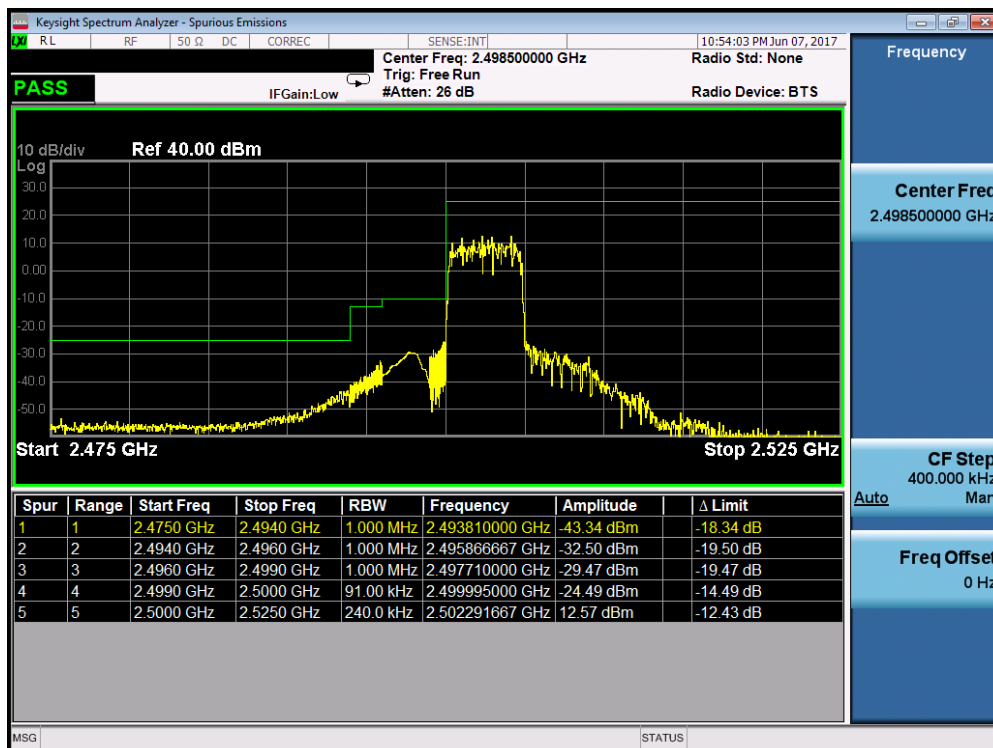
Plot 7-183. Lower ACP Plot (Band 7 – 5.0MHz QPSK – RB Size 25)
