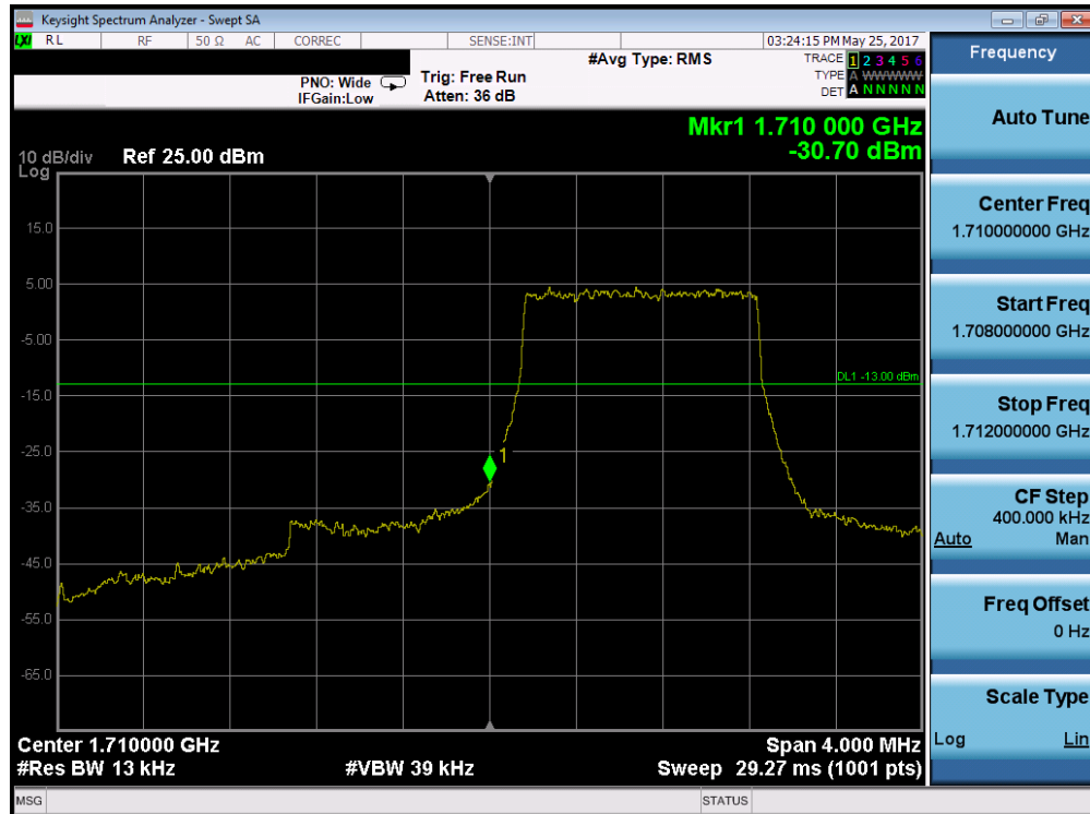
Plot 7-111. Lower Band Edge Plot (Band 4 – 1.4MHz QPSK – RB Size 6)
