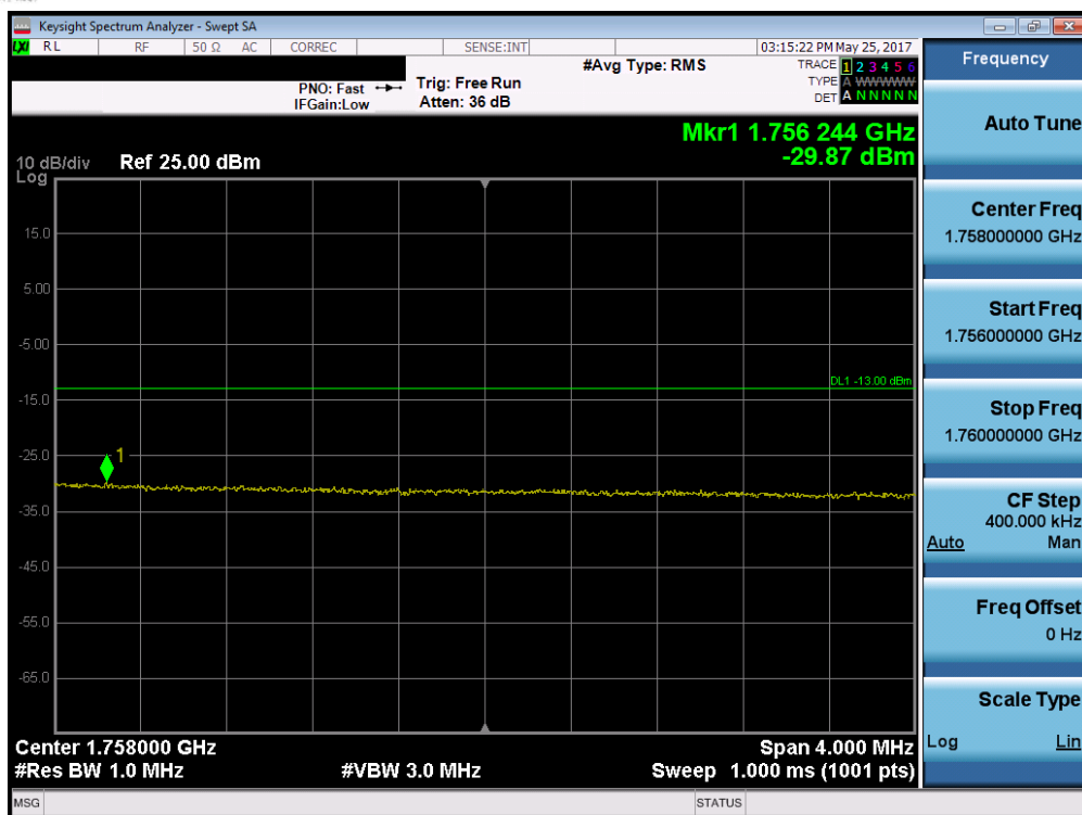
Plot 7-134. Upper Extended Band Edge Plot (Band 4 – 20.0MHz QPSK – RB Size 100)
