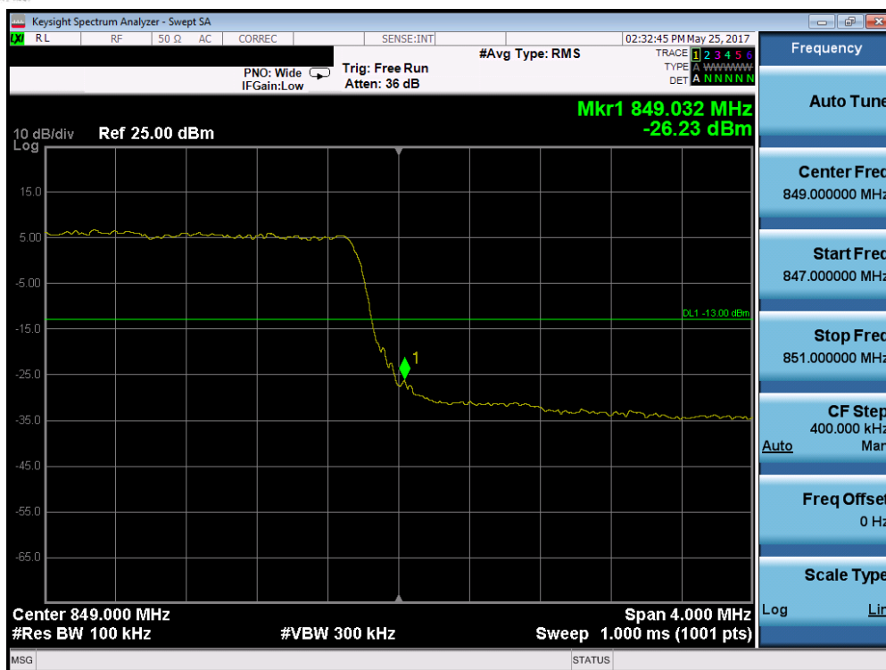
Plot 7-108. Upper Band Edge Plot (Band 5 - 5.0MHz QPSK - RB Size 25)
