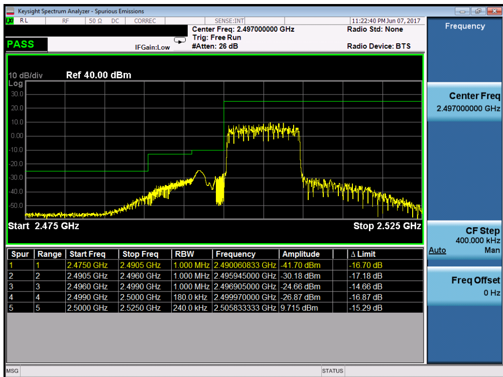
Plot 7-185. Lower ACP Plot (Band 7 – 10.0MHz QPSK – RB Size 50)
