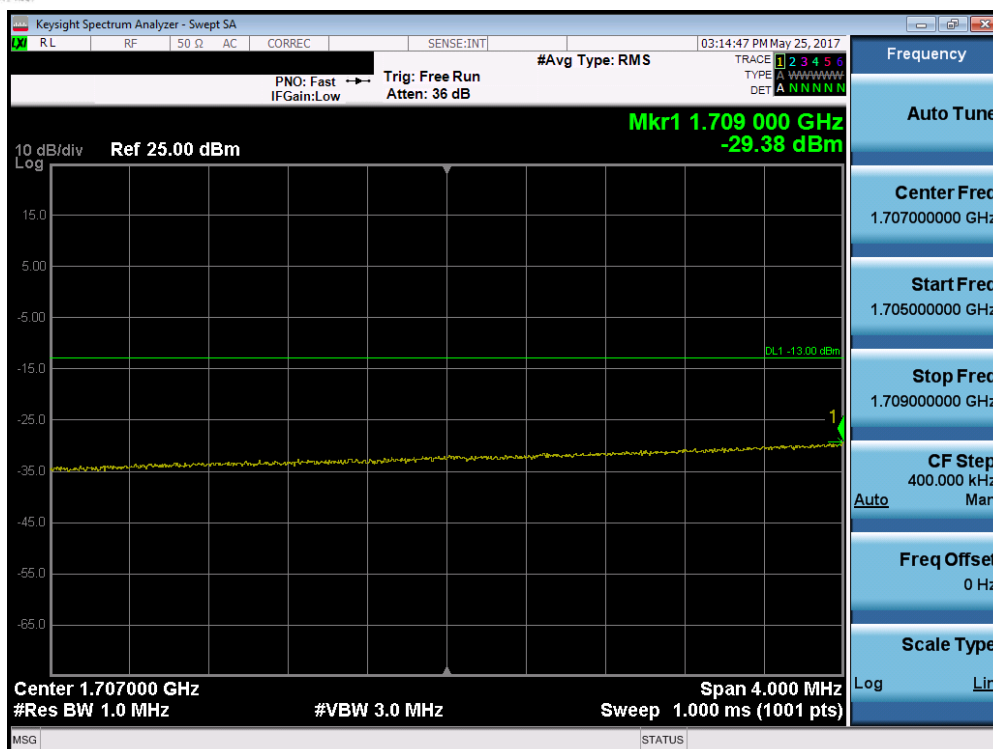
Plot 7-132. Lower Extended Band Edge Plot (Band 4 - 20.0MHz QPSK - RB Size 100)
