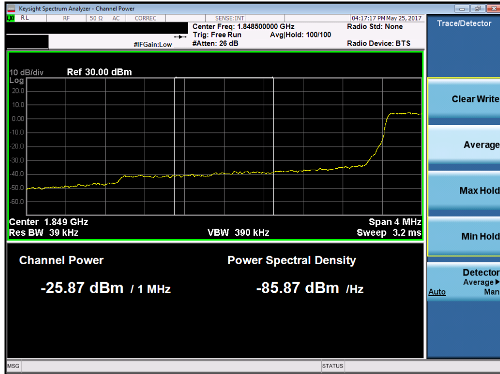
Plot 7-164. Lower Extended Band Edge Plot (Band 2 – 3.0MHz QPSK – RB Size 15)
