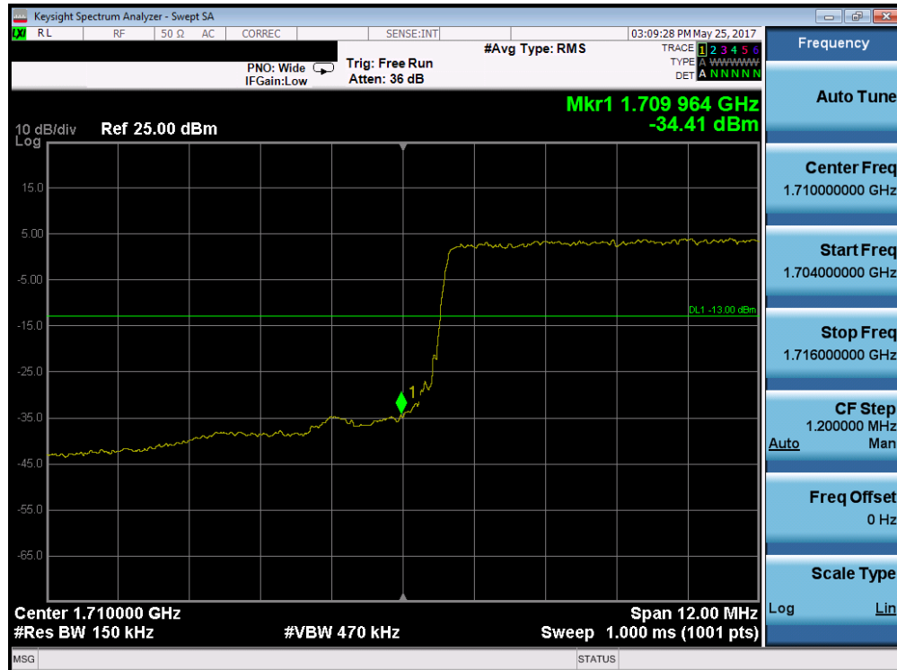
Plot 7-127. Lower Band Edge Plot (Band 4 – 15.0MHz QPSK – RB Size 75)
