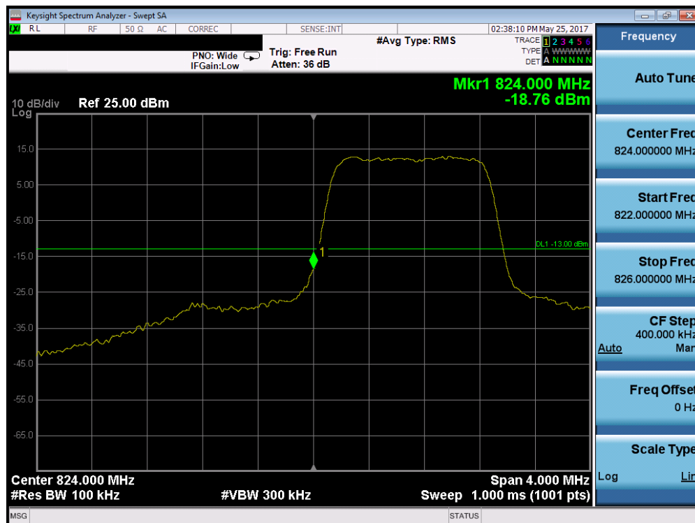
Plot 7-103. Lower Band Edge Plot (Band 5 – 1.4MHz QPSK – RB Size 6)
