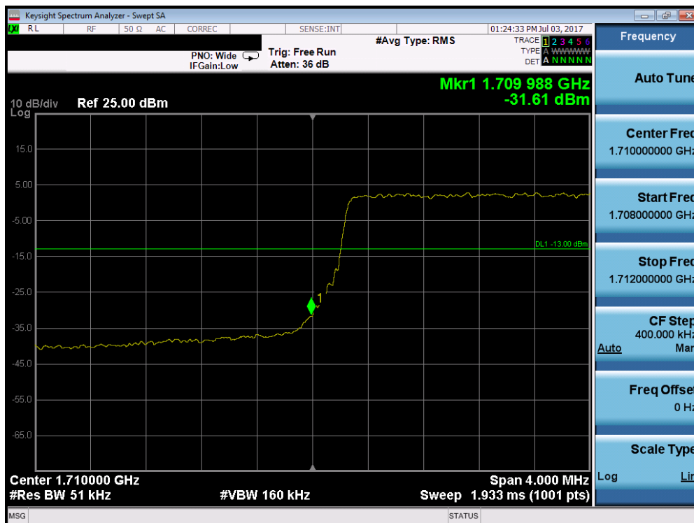
Plot 7-143. Lower Band Edge Plot (Band 66 – 5.0MHz QPSK – RB Size 25)
