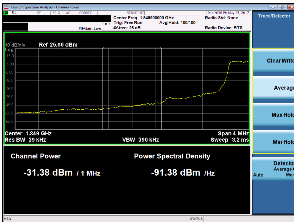
Plot 7-160. Lower Extended Band Edge Plot (Band 2 – 1.4MHz QPSK – RB Size 6)
