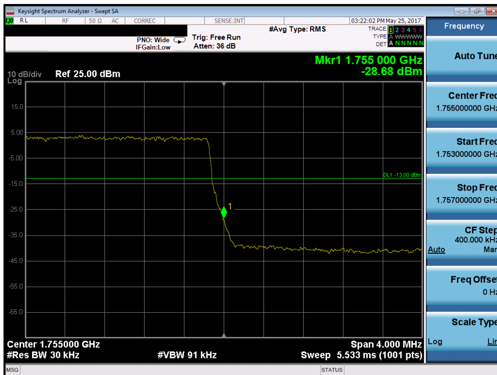
Plot 7-117. Upper Band Edge Plot (Band 4 – 3.0MHz QPSK – RB Size 15)
