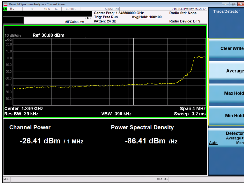
Plot 7-168. Lower Extended Band Edge Plot (Band 2 – 5.0MHz QPSK – RB Size 25)
