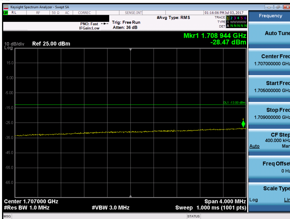
Plot 7-156. Lower Extended Band Edge Plot (Band 66 – 20.0MHz QPSK – RB Size 100)
