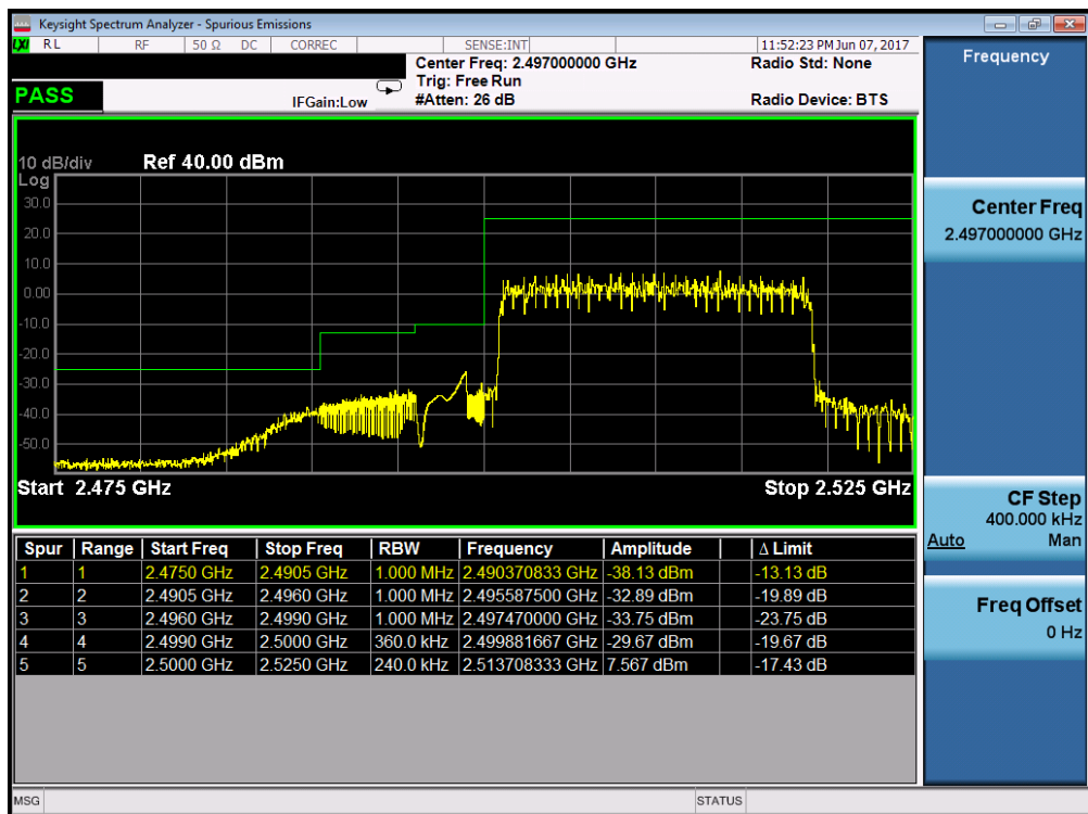
Plot 7-189. Lower ACP Plot (Band 7 – 20.0MHz QPSK – RB Size 100)
