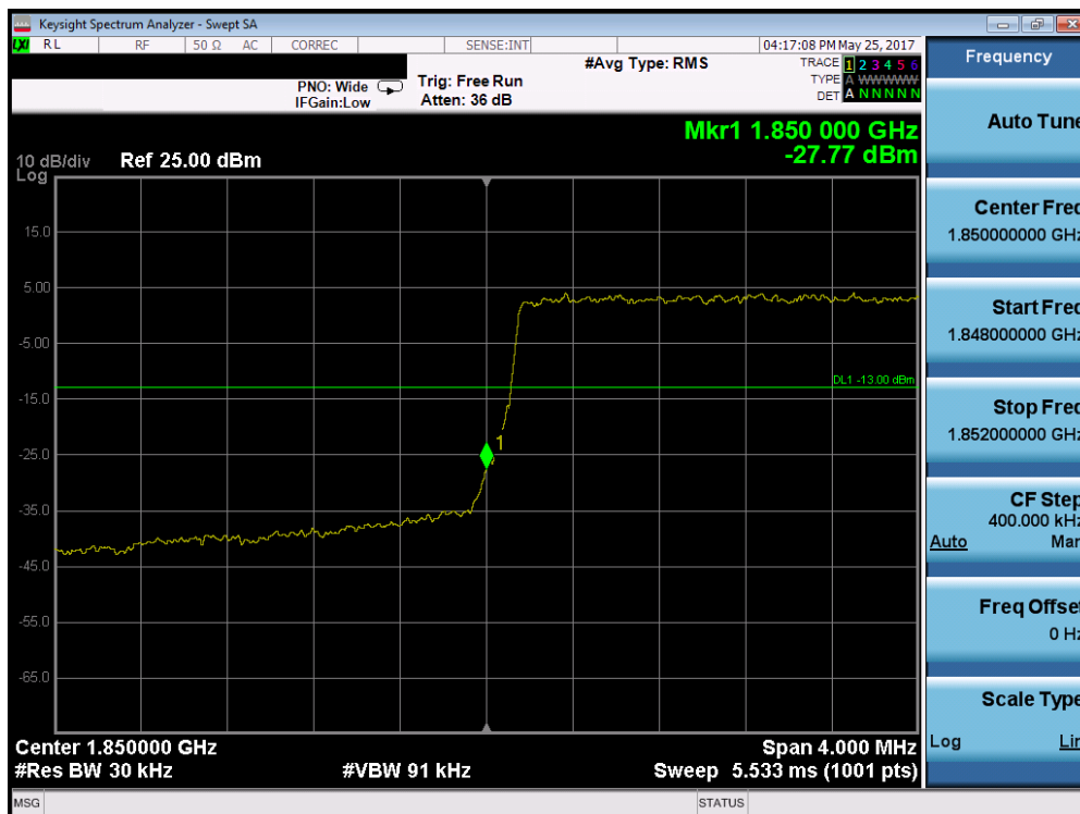
Plot 7-163. Lower Band Edge Plot (Band 2 – 3.0MHz QPSK – RB Size 15)
