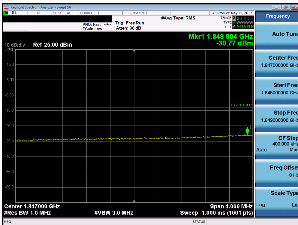
Plot 7-180. Lower Extended Band Edge Plot (Band 2 – 20.0MHz QPSK – RB Size 100)
