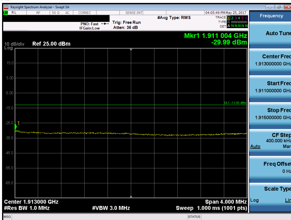
Plot 7-178. Upper Extended Band Edge Plot (Band 2 – 15.0MHz QPSK – RB Size 75)
