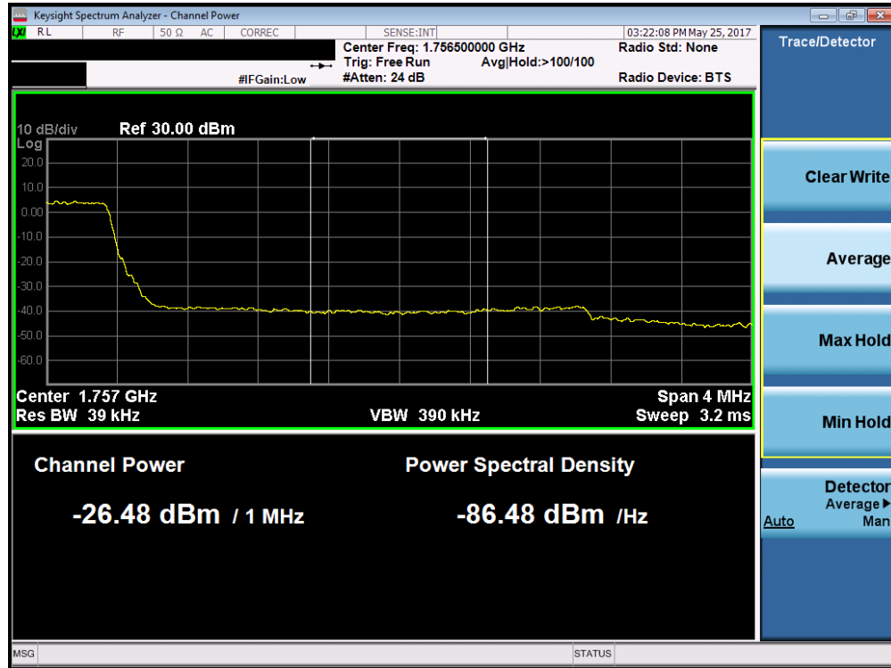
Plot 7-118. Upper Extended Band Edge Plot (Band 4 – 3.0MHz QPSK – RB Size 15)
