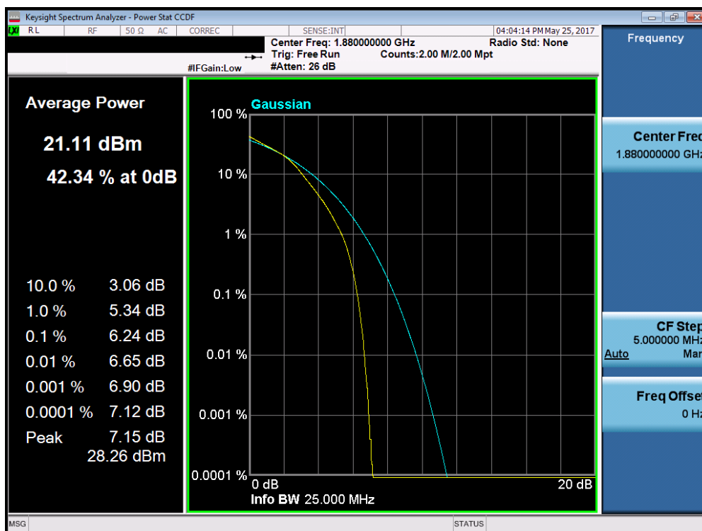
Plot 7-200. PAR Plot (Band 2 – 15.0MHz 16-QAM – RB Size 75)
