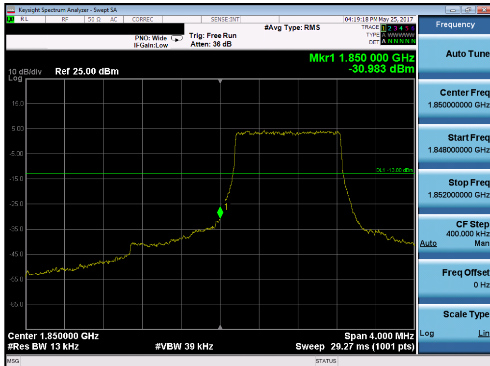
Plot 7-159. Lower Band Edge Plot (Band 2 – 1.4MHz QPSK – RB Size 6)
