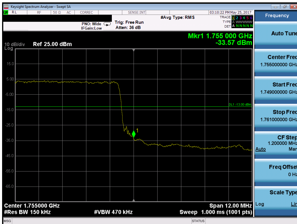
Plot 7-129. Upper Band Edge Plot (Band 4 – 15.0MHz QPSK – RB Size 75)
