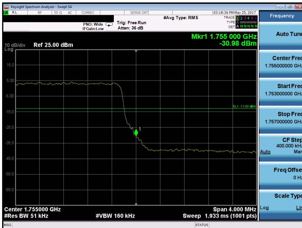
Plot 7-121. Upper Band Edge Plot (Band 4 – 5.0MHz QPSK – RB Size 25)
