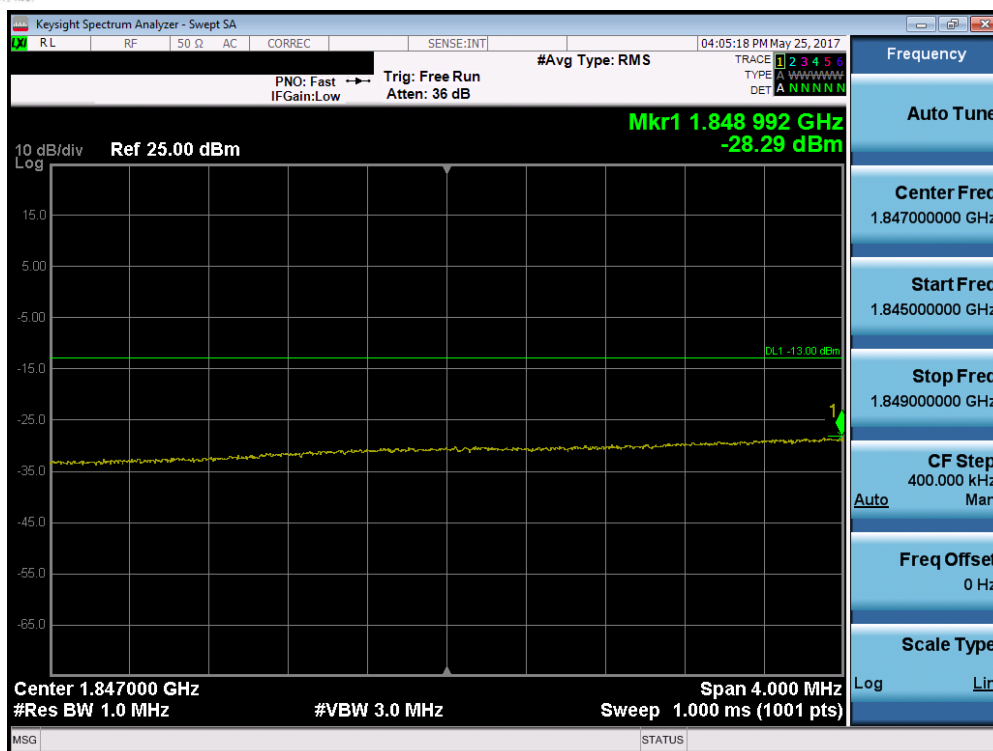
Plot 7-176. Lower Extended Band Edge Plot (Band 2 – 15.0MHz QPSK – RB Size 75)
