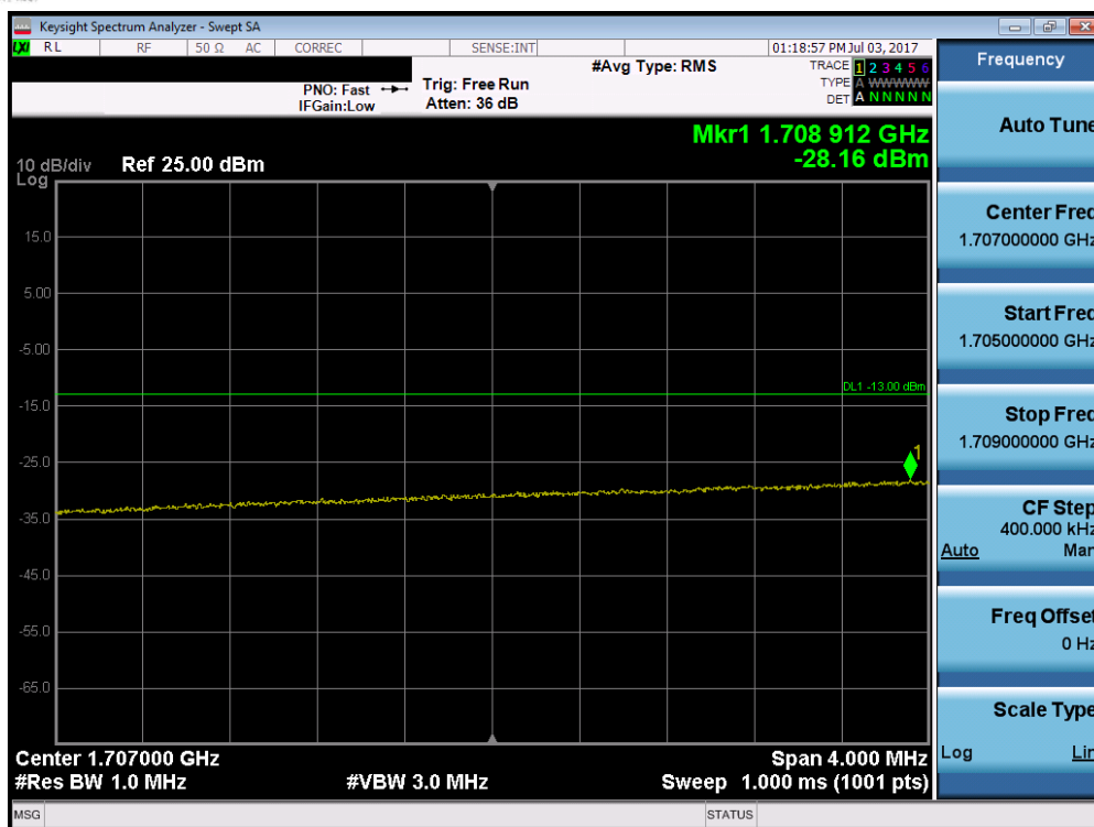
Plot 7-152. Lower Extended Band Edge Plot (Band 66 – 15.0MHz QPSK – RB Size 75)
