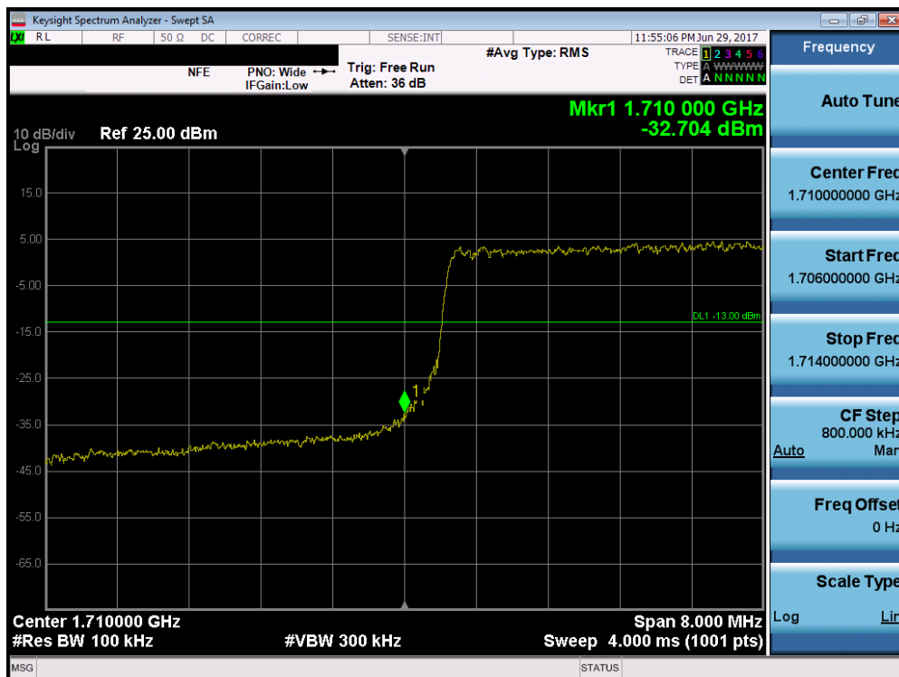
Plot 7-147. Lower Band Edge Plot (Band 66 – 10.0MHz QPSK – RB Size 50)
