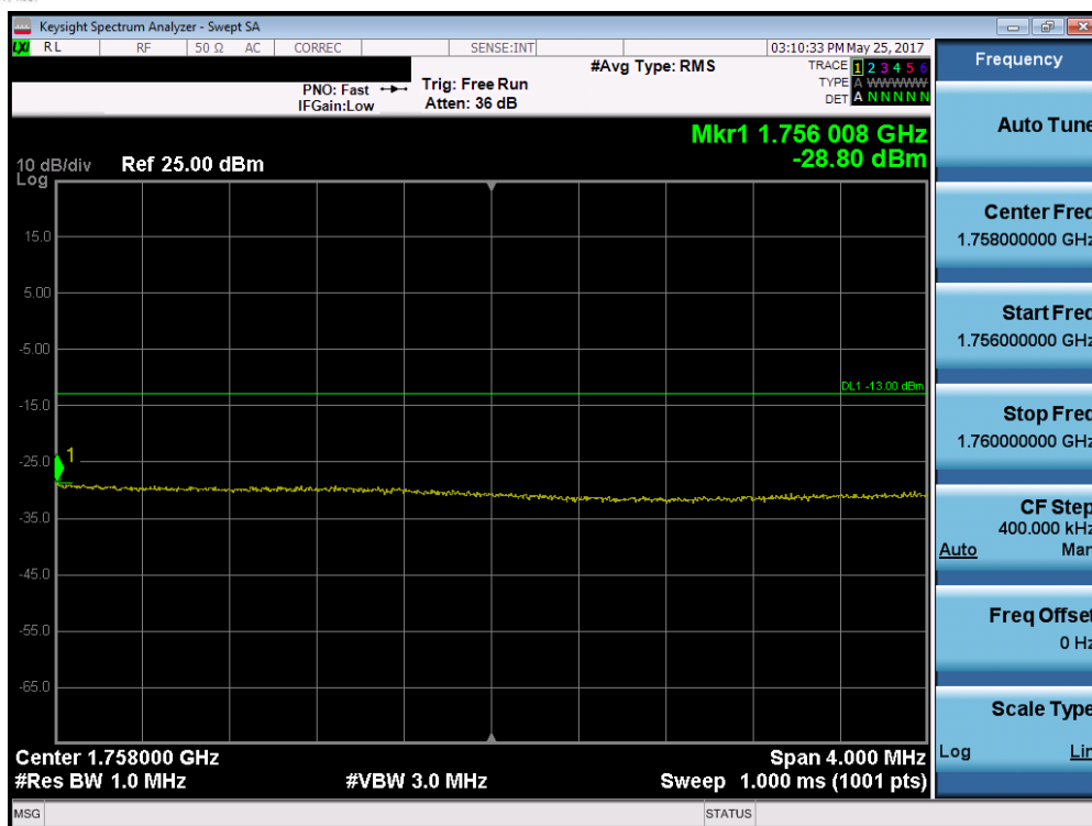
Plot 7-130. Upper Extended Band Edge Plot (Band 4 - 15.0MHz QPSK - RB Size 75)
