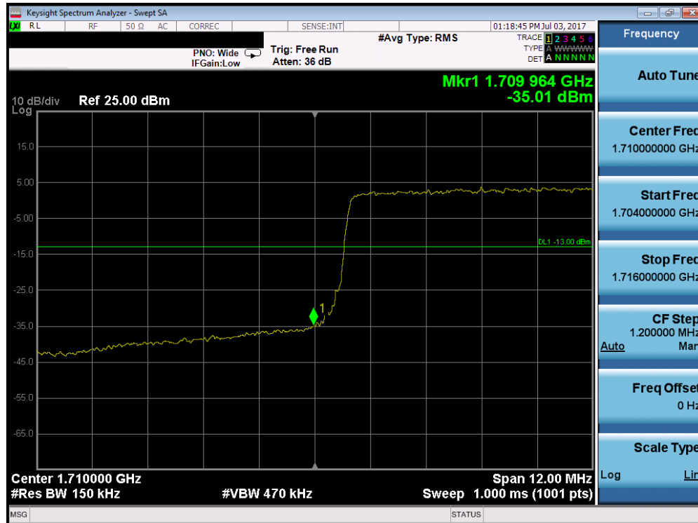
Plot 7-151. Lower Band Edge Plot (Band 66 – 15.0MHz QPSK – RB Size 75)
