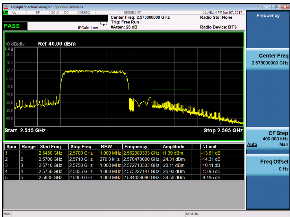
Plot 7-188. Upper ACP Plot (Band 7 – 15.0MHz QPSK – RB Size 75)
