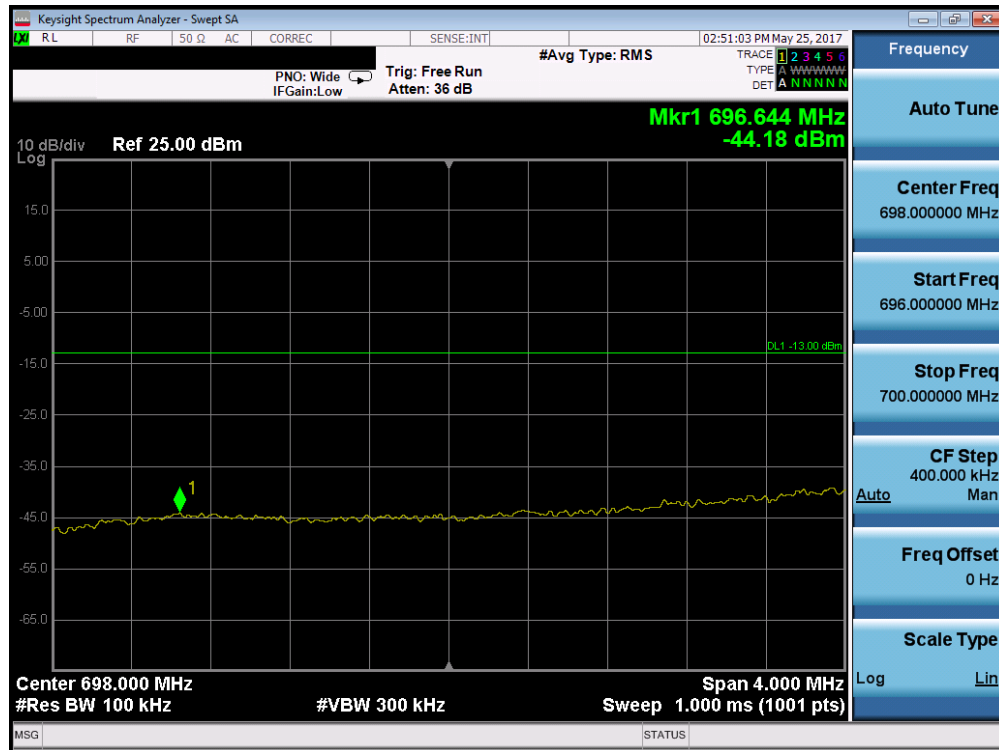
Plot 7-99. Lower Band Edge Plot (Band 17 – 5.0MHz QPSK – RB Size 25)
