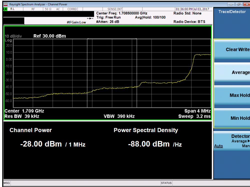
Plot 7-136. Lower Extended Band Edge Plot (Band 66 – 1.4MHz QPSK – RB Size 6)
