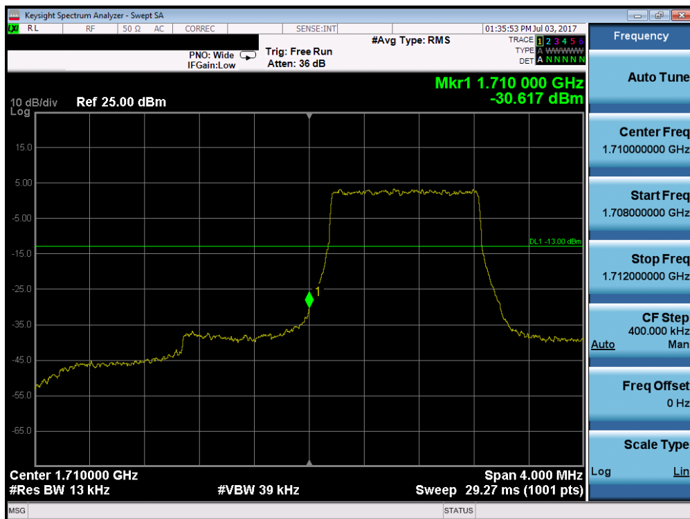
Plot 7-135. Lower Band Edge Plot (Band 66 – 1.4MHz QPSK – RB Size 6)
