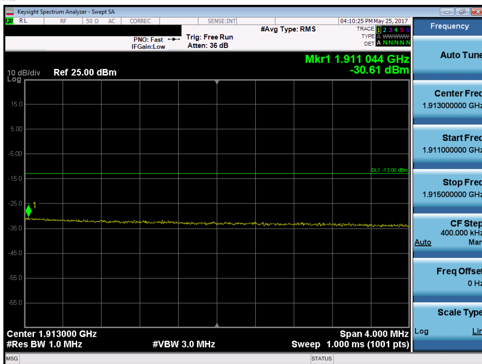
Plot 7-182. Upper Extended Band Edge Plot (Band 2 – 20.0MHz QPSK – RB Size 100)
