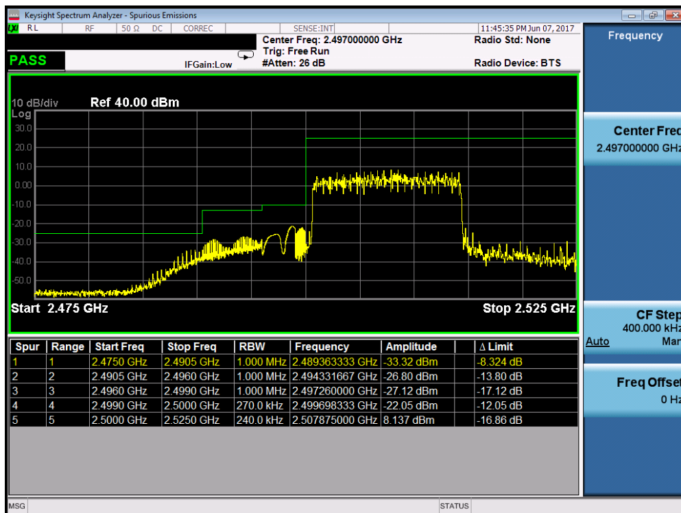
Plot 7-187. Lower ACP Plot (Band 7 – 15.0MHz QPSK – RB Size 75)
