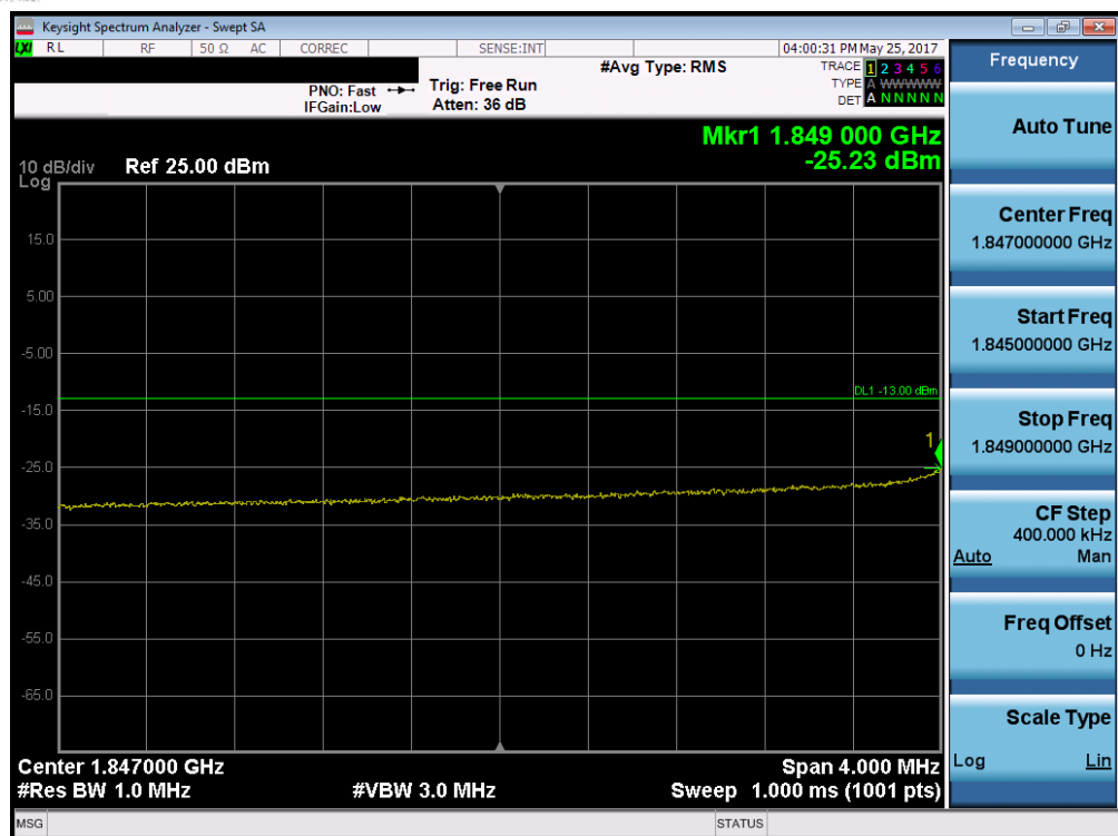
Plot 7-172. Lower Extended Band Edge Plot (Band 2 – 10.0MHz QPSK – RB Size 50)
