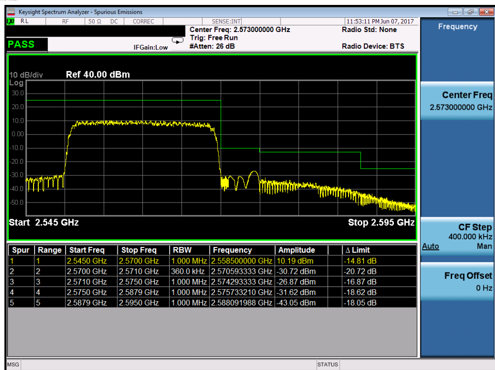
Plot 7-190. Upper ACP Plot (Band 7 – 20.0MHz QPSK – RB Size 100)
