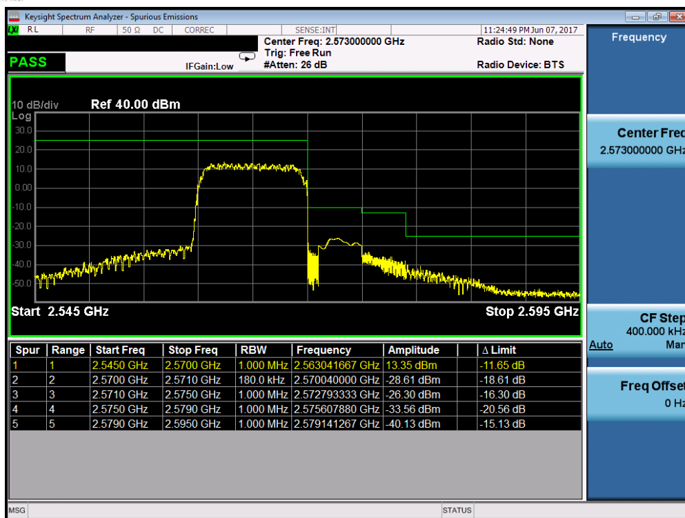
Plot 7-186. Upper ACP Plot (Band 7 – 10.0MHz QPSK – RB Size 50)
