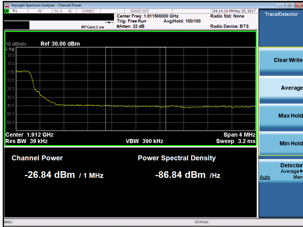
Plot 7-170. Upper Extended Band Edge Plot (Band 2 – 5.0MHz QPSK – RB Size 25)
