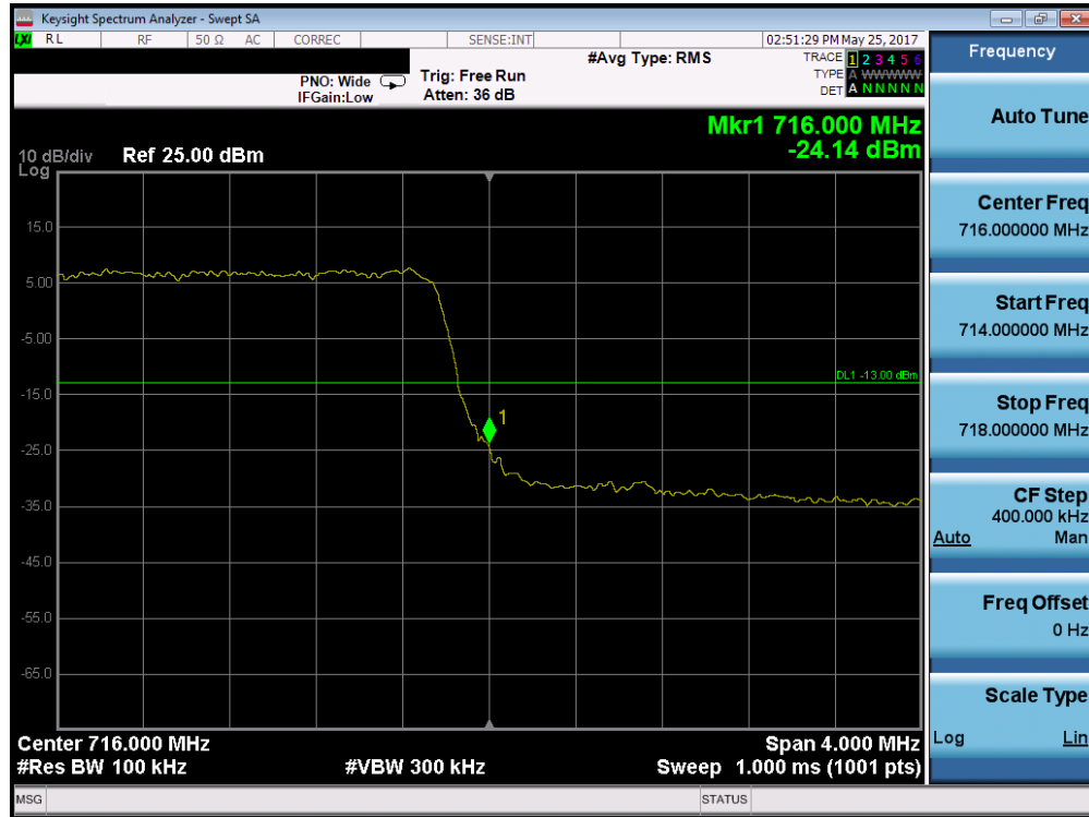
Plot 7-100. Upper Band Edge Plot (Band 17 – 5.0MHz QPSK – RB Size 25)
