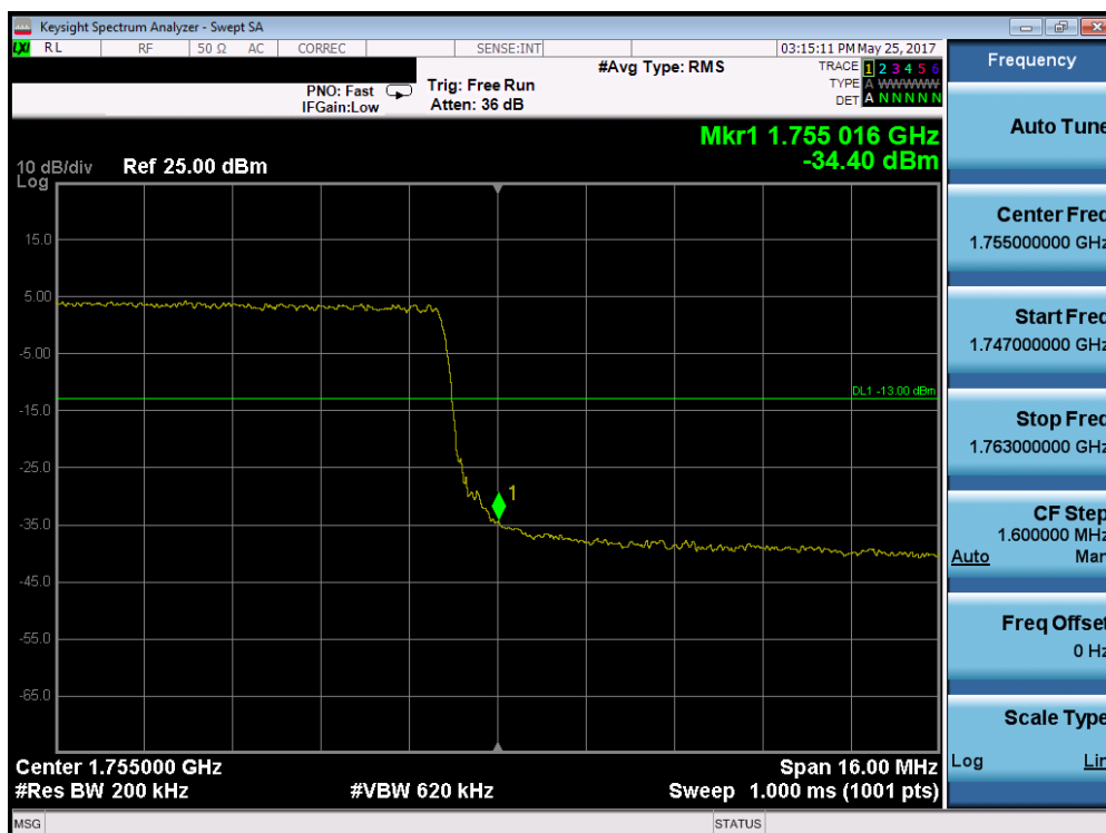
Plot 7-133. Upper Band Edge Plot (Band 4 - 20.0MHz QPSK - RB Size 100)
