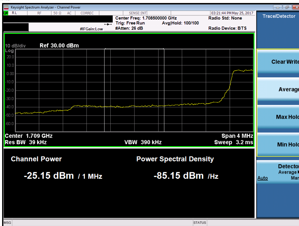
Plot 7-116. Lower Extended Band Edge Plot (Band 4 – 3.0MHz QPSK – RB Size 15)
