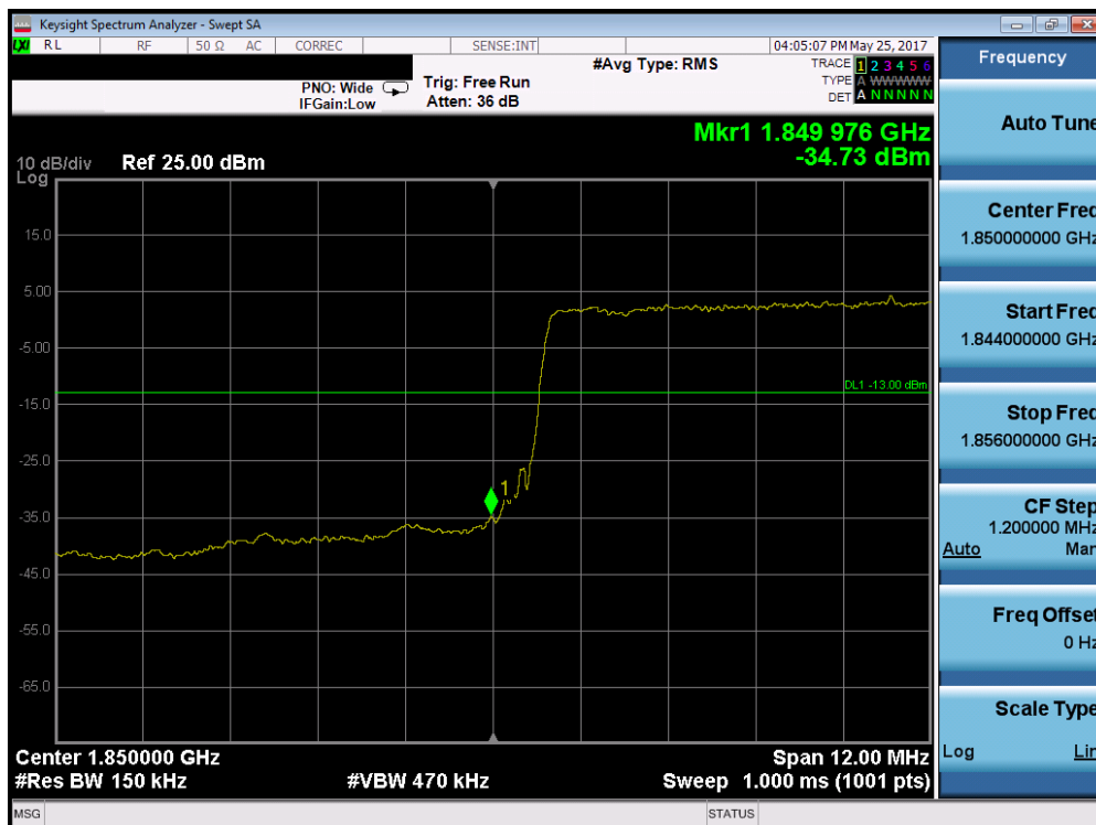
Plot 7-175. Lower Band Edge Plot (Band 2 - 15.0MHz QPSK - RB Size 75)
