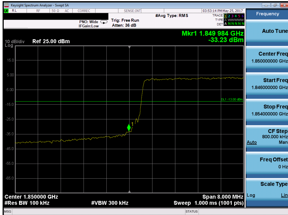
Plot 7-171. Lower Band Edge Plot (Band 2 – 10.0MHz QPSK – RB Size 50)
