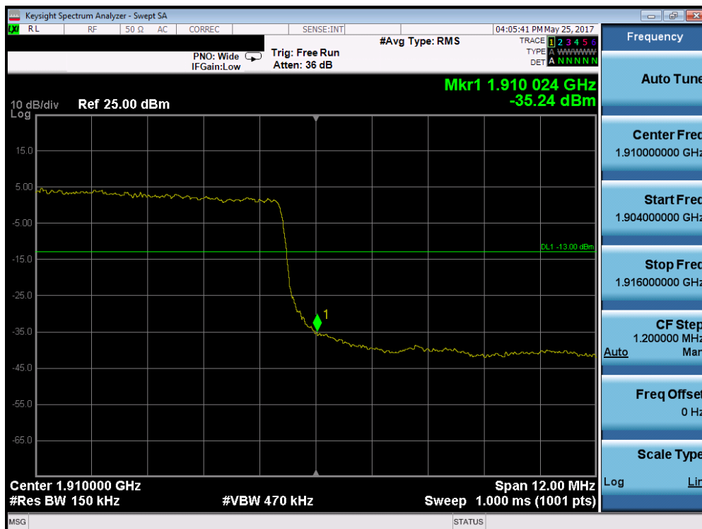
Plot 7-177. Upper Band Edge Plot (Band 2 – 15.0MHz QPSK – RB Size 75)
