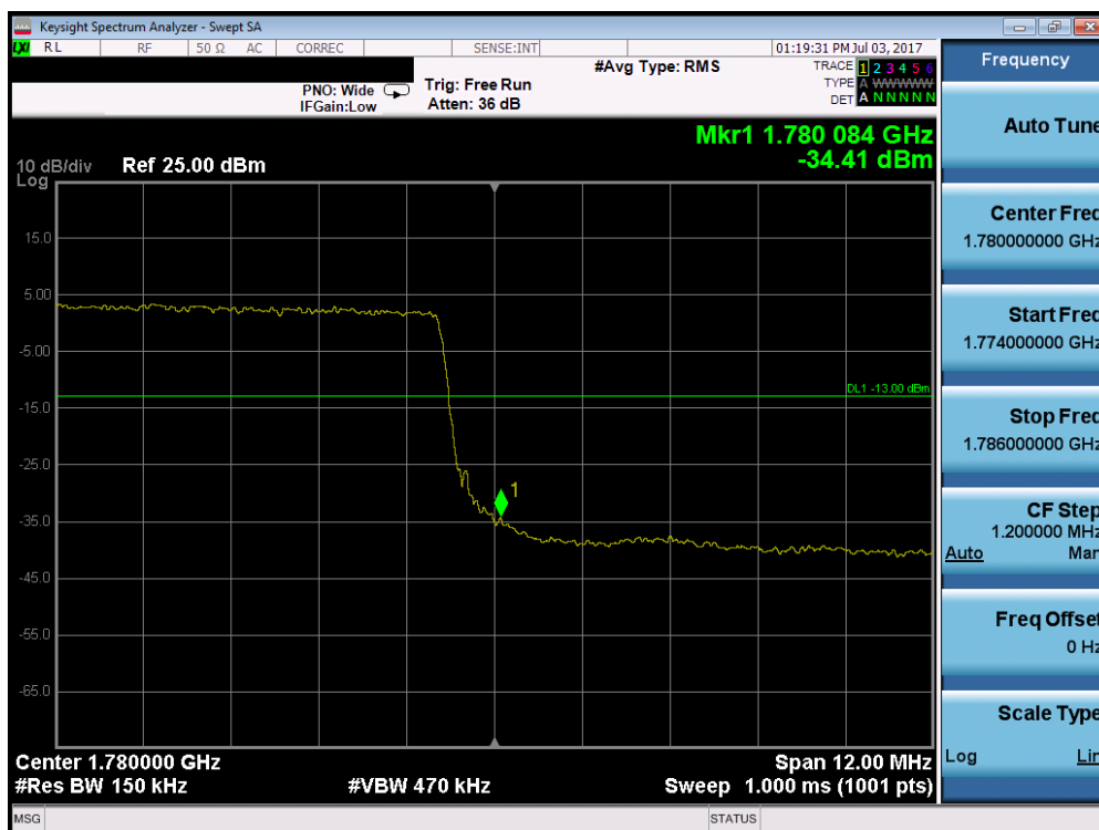
Plot 7-153. Upper Band Edge Plot (Band 66 – 15.0MHz QPSK – RB Size 75)
