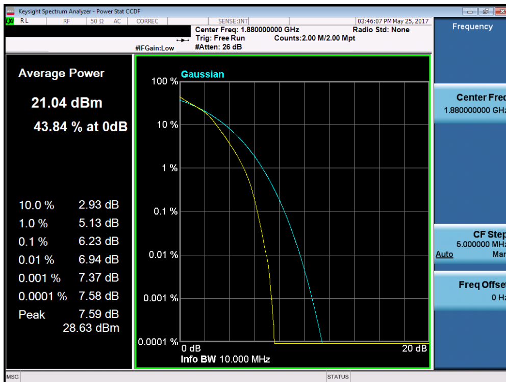
Plot 7-198. PAR Plot (Band 2 – 10.0MHz 16-QAM – RB Size 50)
