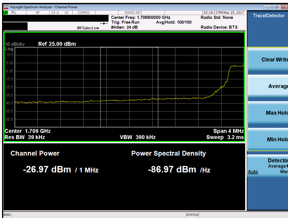
Plot 7-120. Lower Extended Band Edge Plot (Band 4 – 5.0MHz QPSK – RB Size 25)
