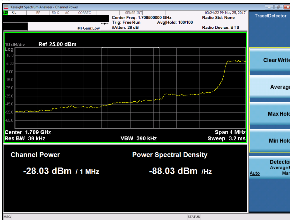
Plot 7-112. Lower Extended Band Edge Plot (Band 4 – 1.4MHz QPSK – RB Size 6)
