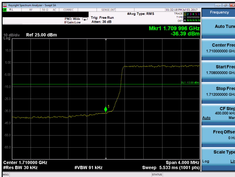
Plot 7-139. Lower Band Edge Plot (Band 66 – 3.0MHz QPSK – RB Size 15)
