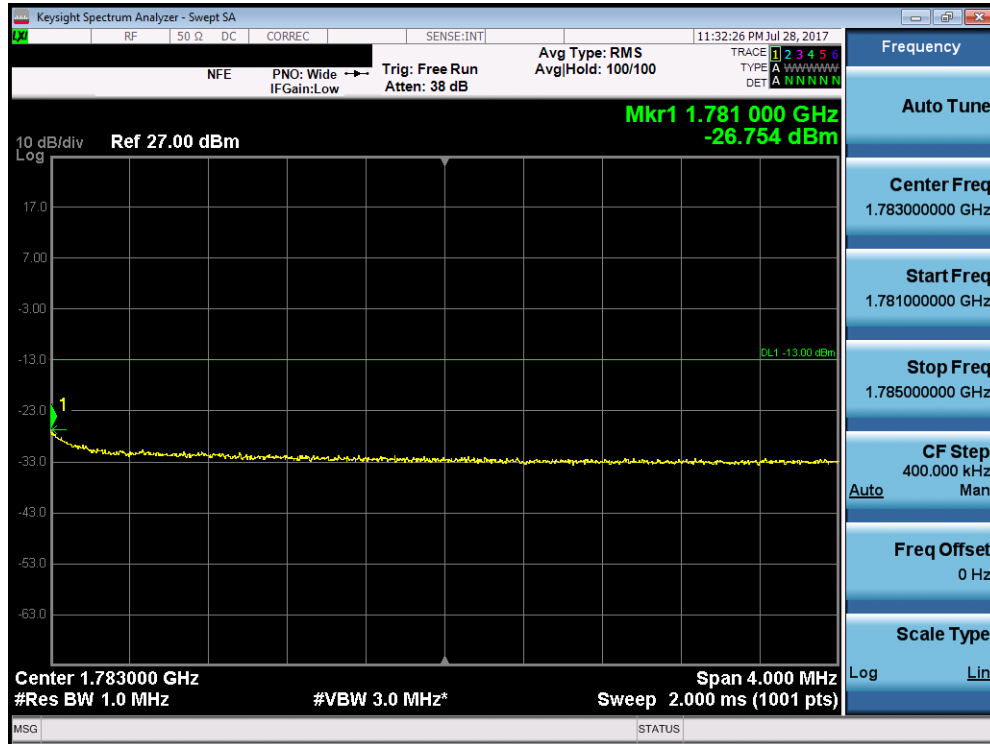
Plot 7-150. Upper Extended Band Edge Plot (Band 66 – 10.0MHz QPSK – RB Size 50)
