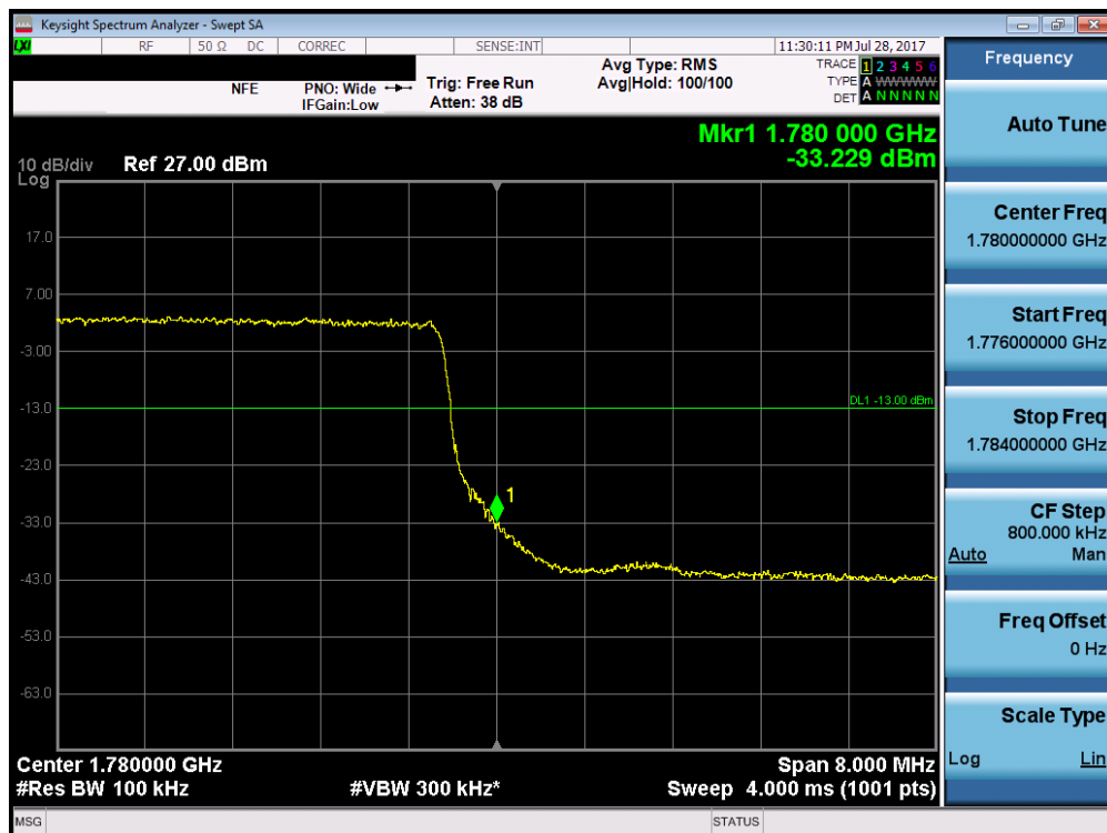
Plot 7-149. Upper Band Edge Plot (Band 66 – 10.0MHz QPSK – RB Size 50)
