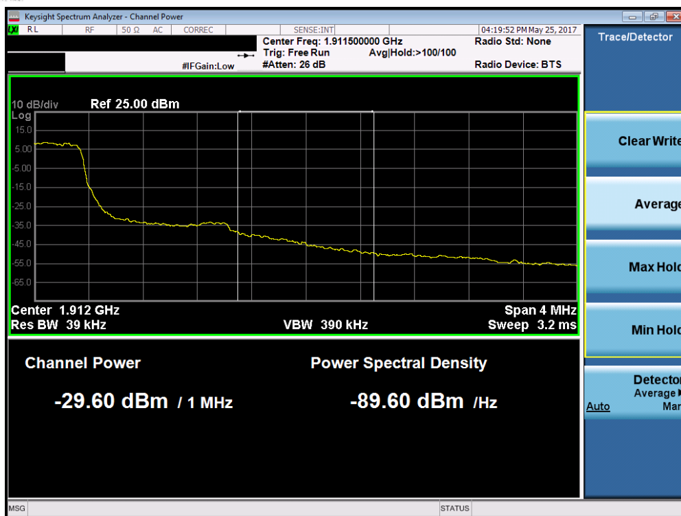
Plot 7-162. Upper Extended Band Edge Plot (Band 2 – 1.4MHz QPSK – RB Size 6)
