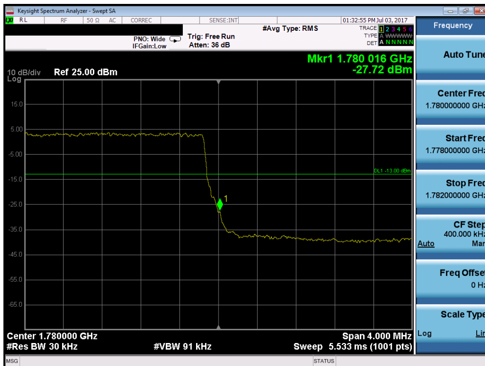
Plot 7-141. Upper Band Edge Plot (Band 66 – 3.0MHz QPSK – RB Size 15)
