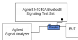
Figure 7-2. Test Instrument & Measurement Setup
