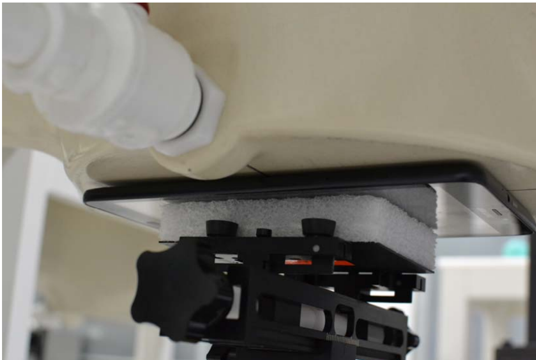
SAR Test Setup Photo 8: Back 0 mm
