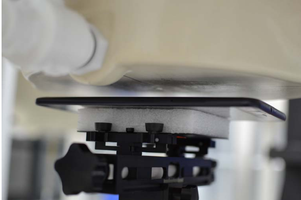
SAR Test Setup Photo 5: Back 14mm
