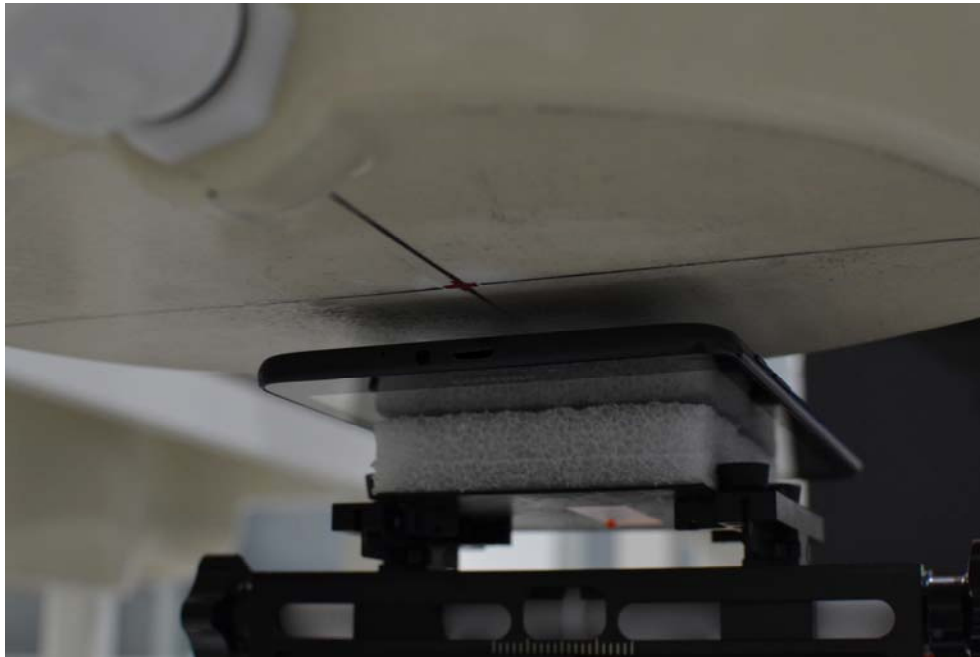
SAR Test Setup Photo 7: Back 11mm (5 GHz WLAN testing)
