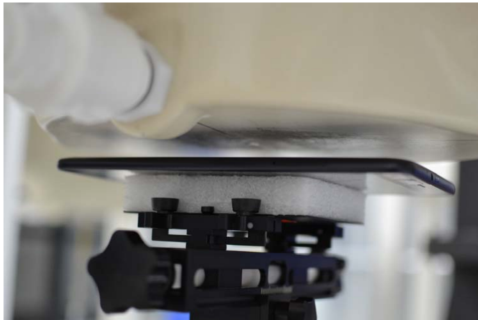
SAR Test Setup Photo 6: Back 11mm
