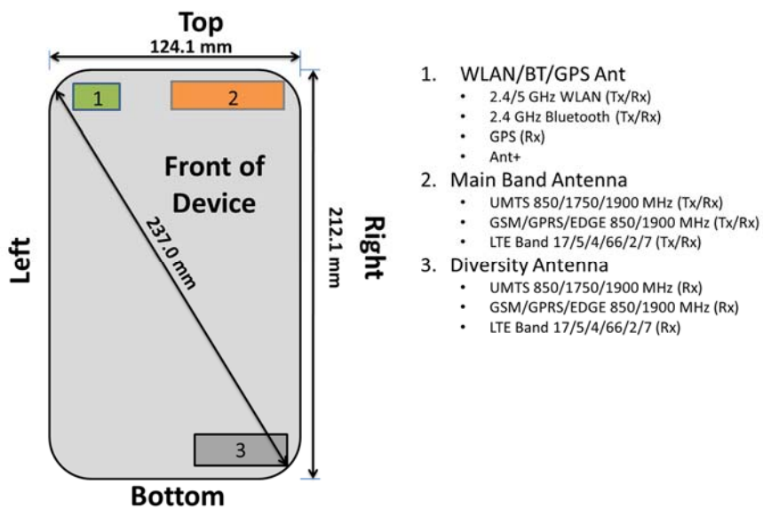
Figure F-1 DUT Antenna Locations
