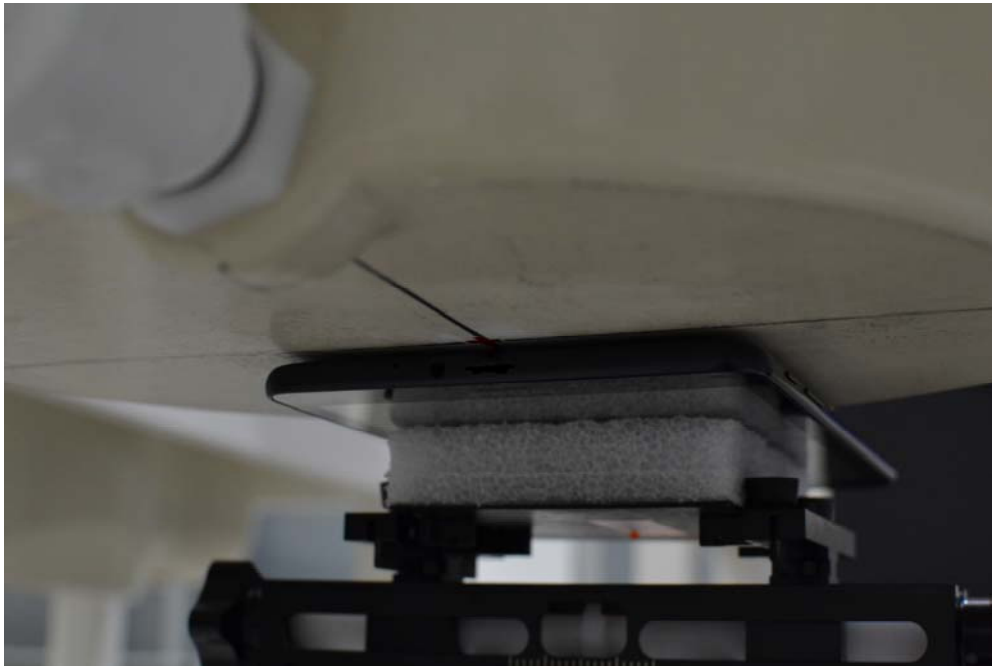
SAR Test Setup Photo 9: Back 0 mm (5 GHz WLAN testing)
