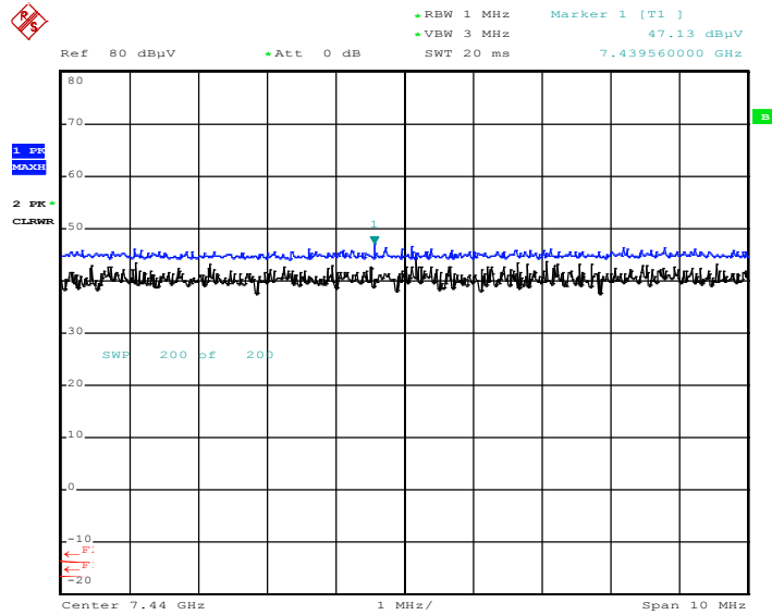
Radiated Spurious Emissions plot – Average Reading (Ch.78 3rd Harmonic)
