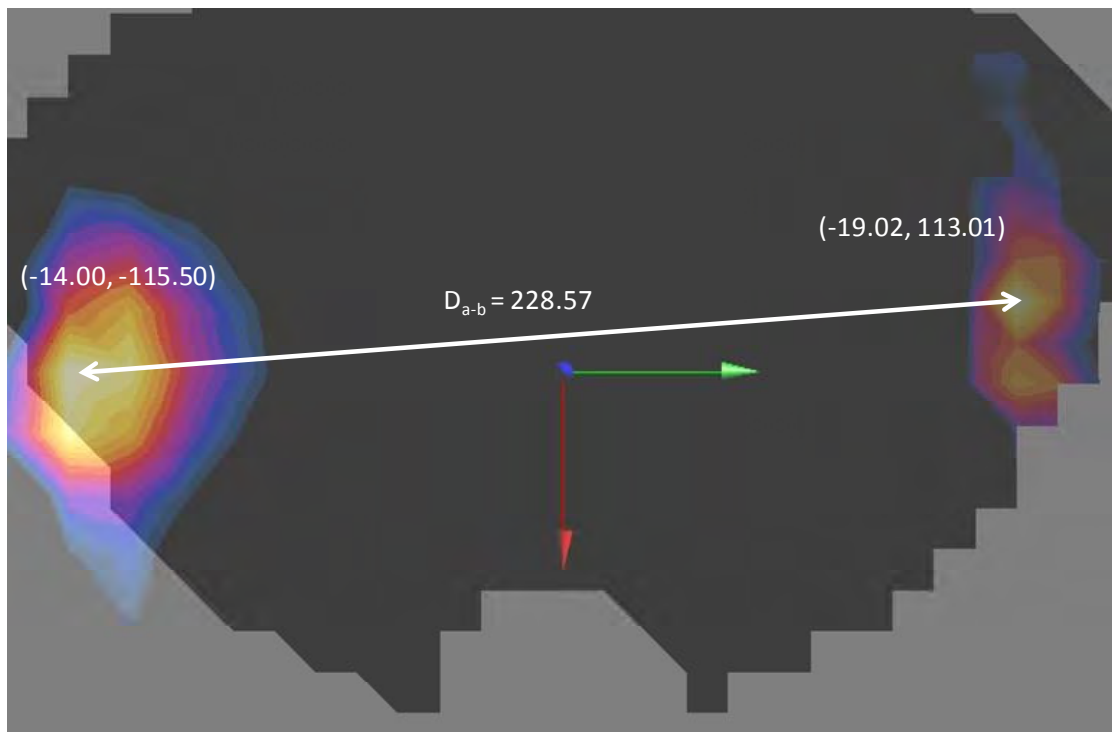
Figure 11-3 Peak SAR Location of 5 GHz WLAN and UMTS 1900 MHz
