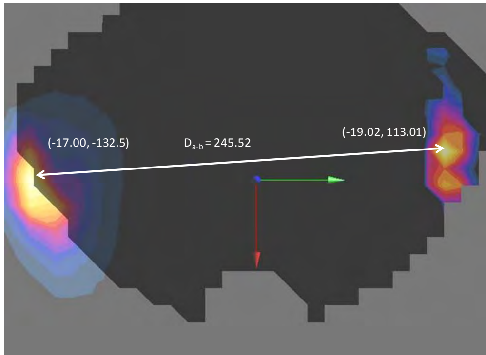
Figure 11-1 Peak SAR Location of 5 GHz WLAN and GRPS 850 MHz
