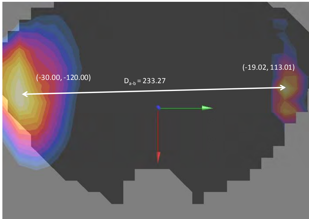
Figure 11-2 Peak SAR Location of 5 GHz WLAN and UMTS 850 MHz
