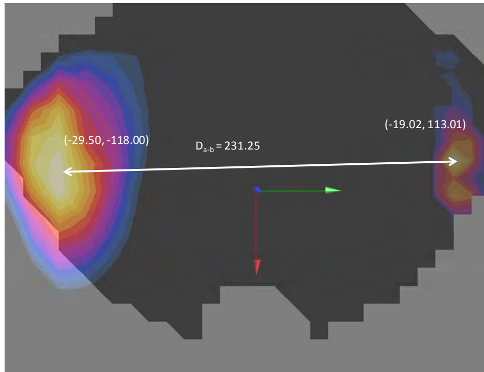
Figure 11-4 Peak SAR Location of 5 GHz WLAN and LTE Band 5 MHz
