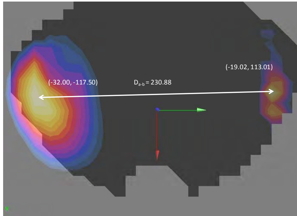
Figure 11-5 Peak SAR Location of 5 GHz WLAN and GPRS 850 MHz
