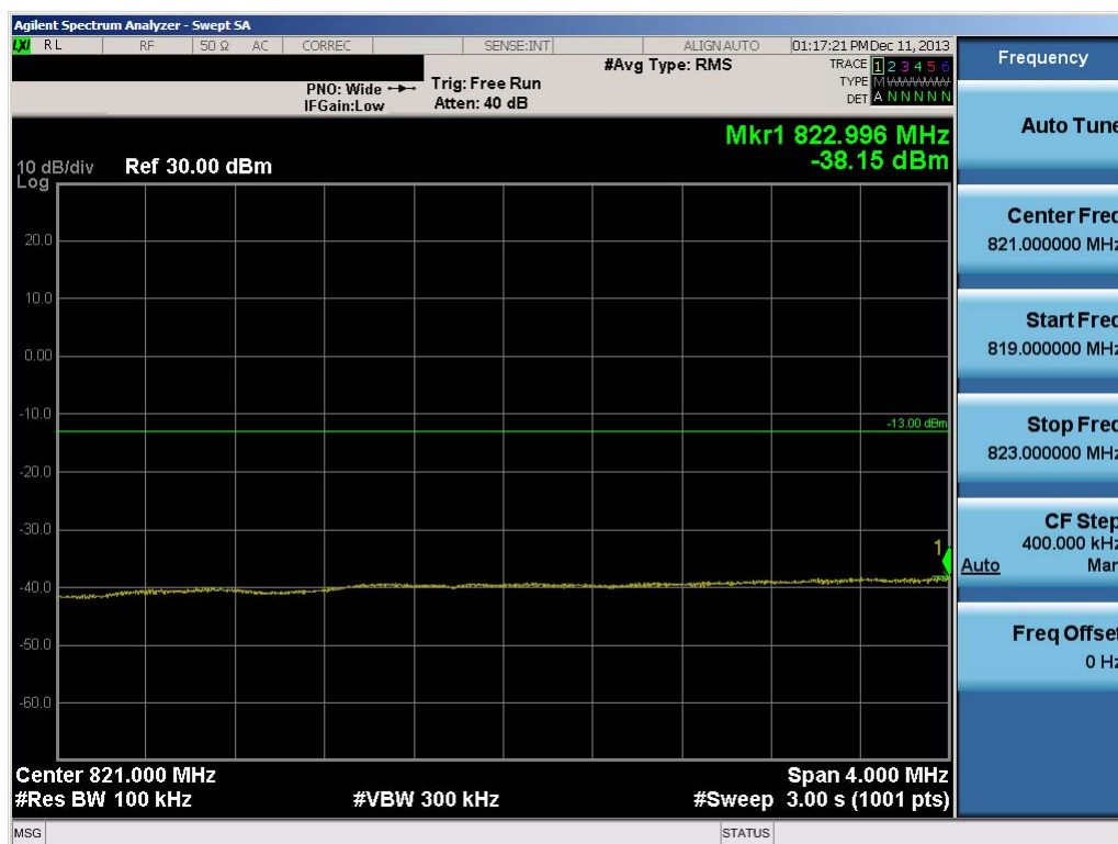
Plot 7-38. Lower Extended Band Edge Plot (10.0MHz QPSK – RB Size 50)
