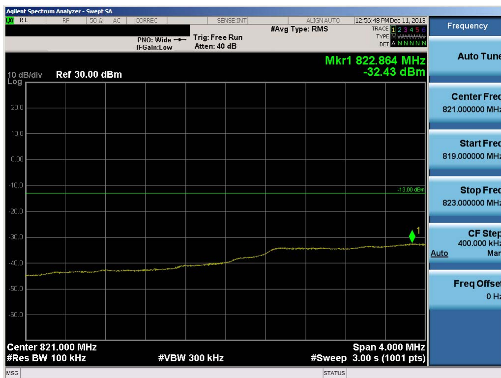
Plot 7-14. Lower Extended Band Edge Plot (3.0MHz QPSK – RB Size 15)
