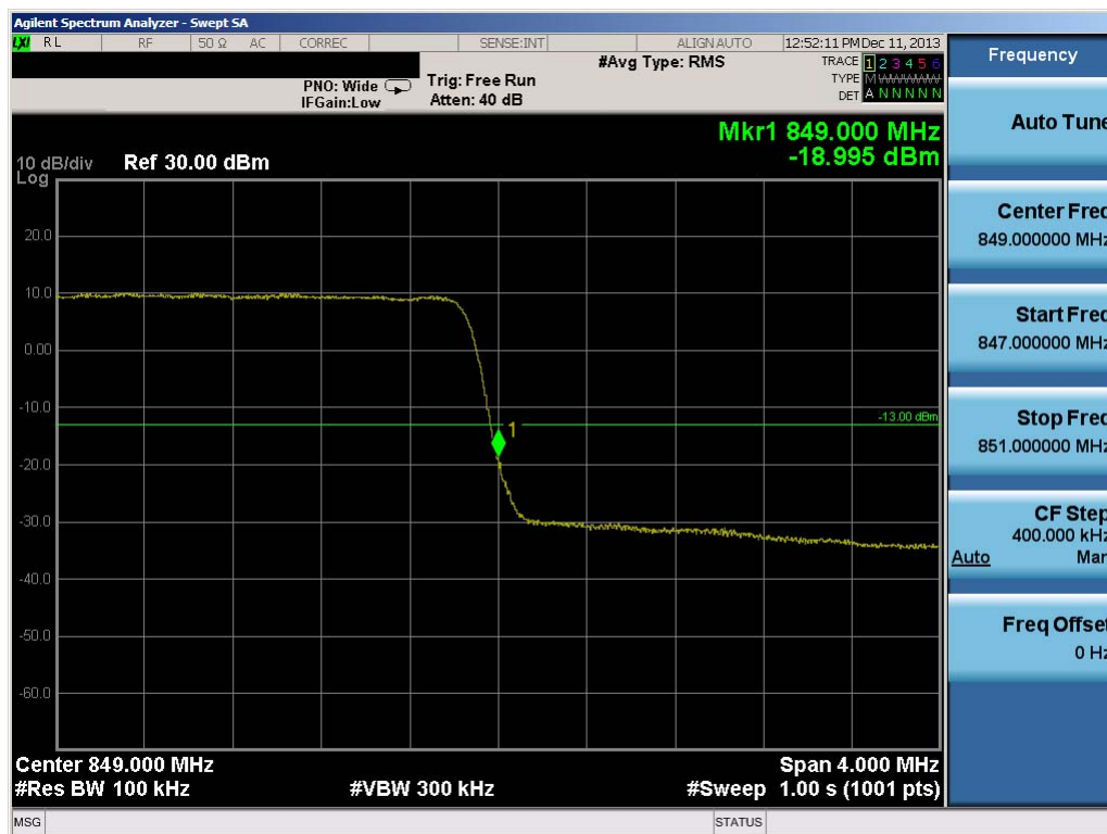
Plot 7-11. Upper Band Edge Plot (1.4MHz QPSK – RB Size 6)
