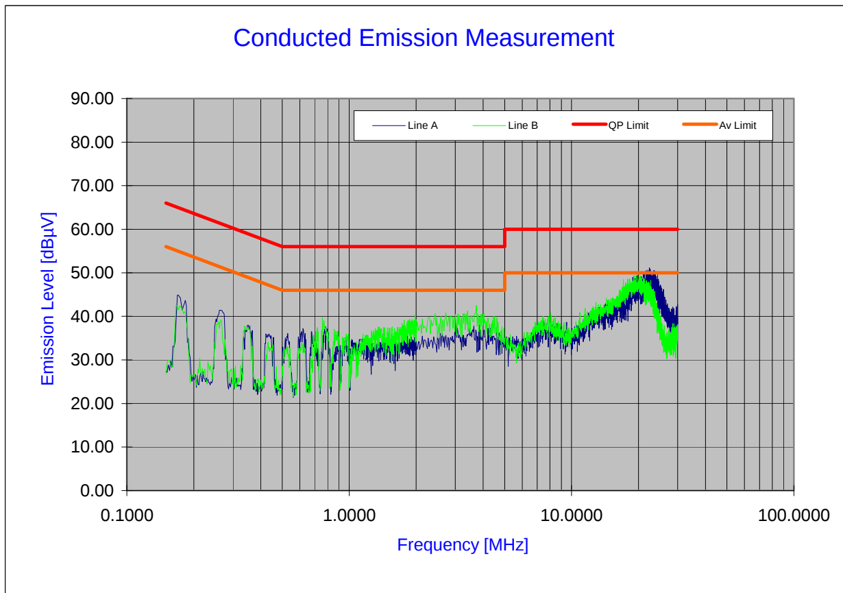
Plot 6-65. Line Conducted Plot with 802.11b
