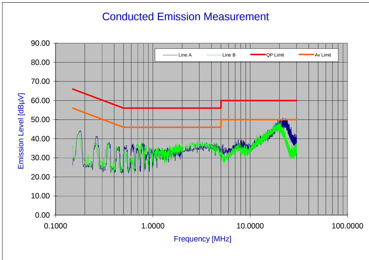
Plot 6-66. Line Conducted Plot with 802.11a
