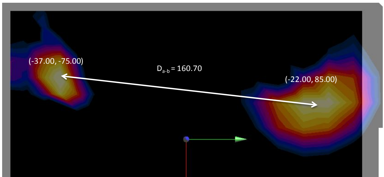
Figure 10-4 Peak SAR Location of 5 GHz WLAN and GPRS 1900 MHz
