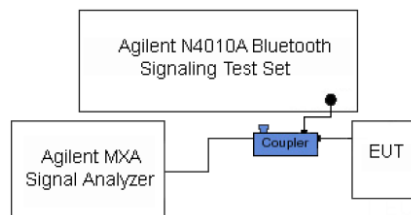
Figure 7-4 Power Measurement Setup
