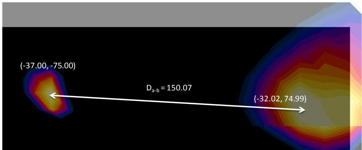
Figure 10-2 Peak SAR Location of 5 GHz WLAN and GPRS 850 MHz
