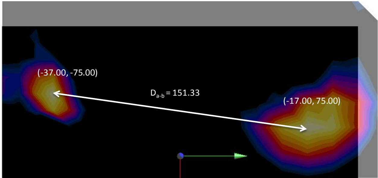
Figure 10-5 Peak SAR Location of 5 GHz WLAN and UMTS 1900 MHz
