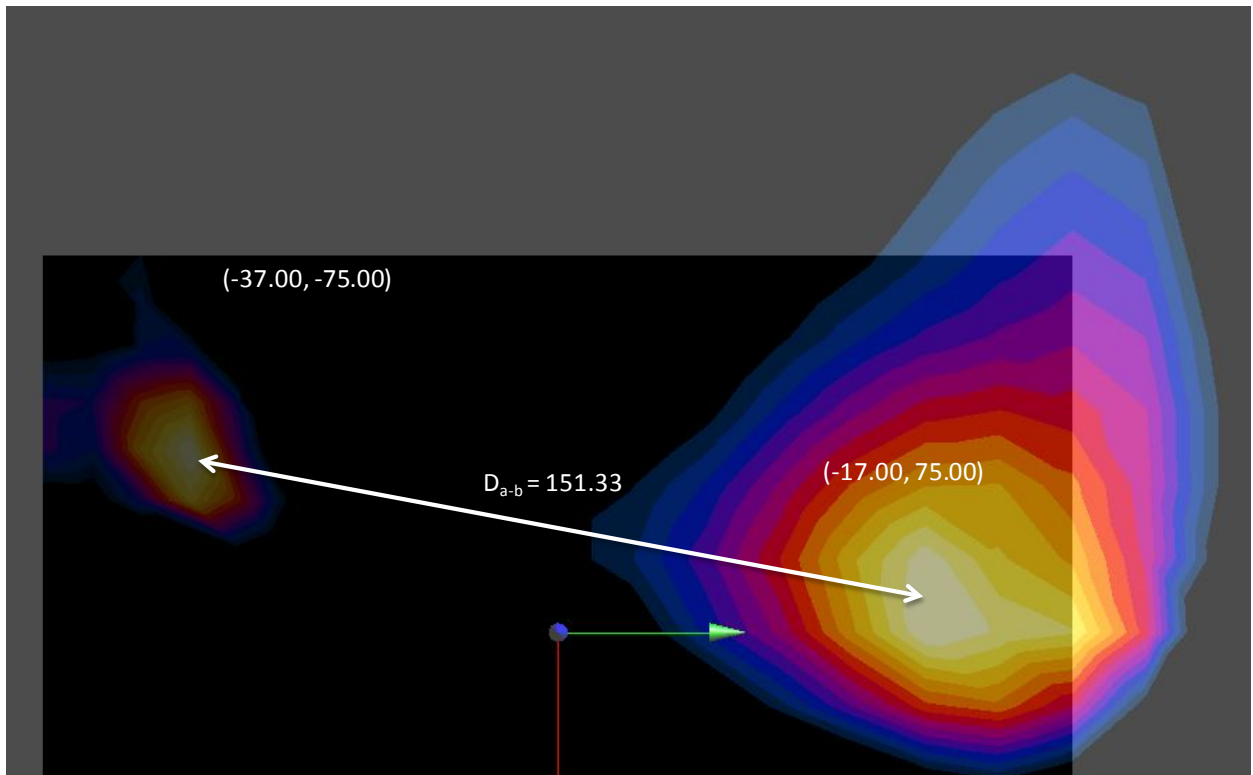
Figure 10-3 Peak SAR Location of 5 GHz WLAN and UMTS 850 MHz
