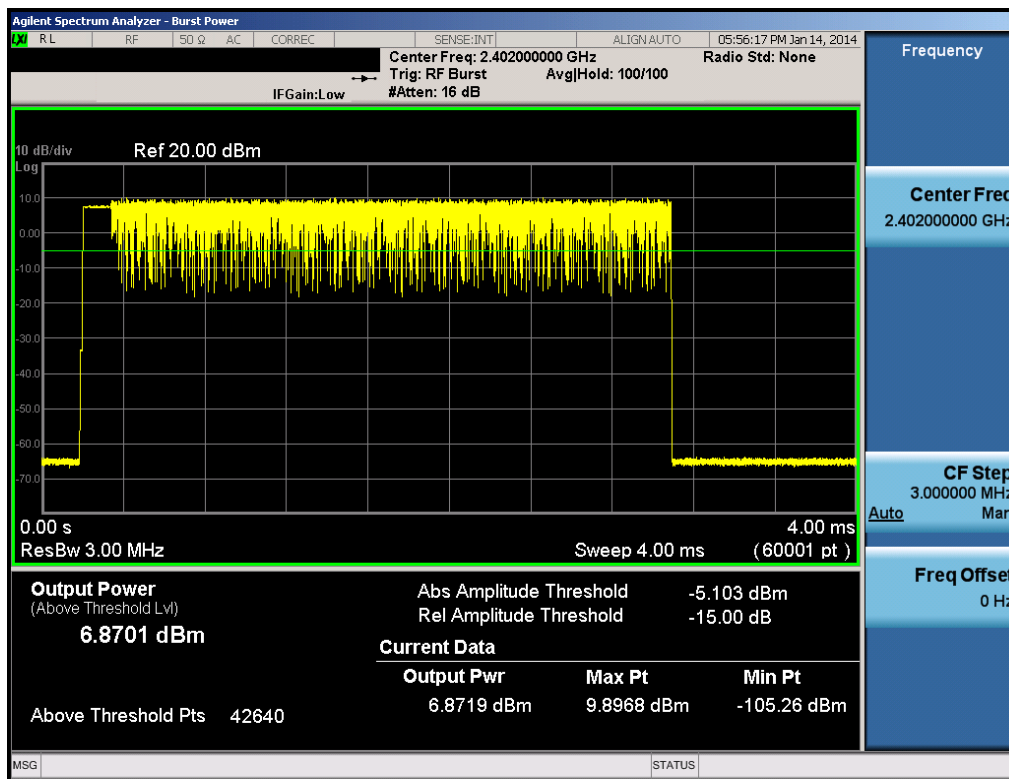
Plot 6-25. Average Conducted Power (3Mbps – Ch. 0)
