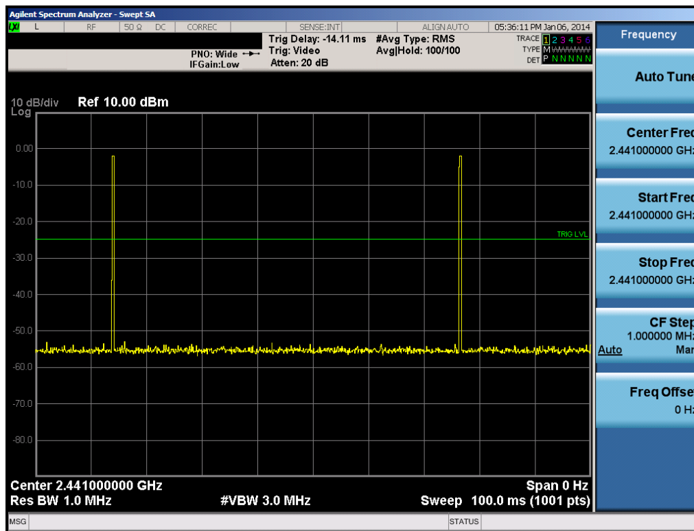
Plot 6-2. Worst Case 100ms Operation
