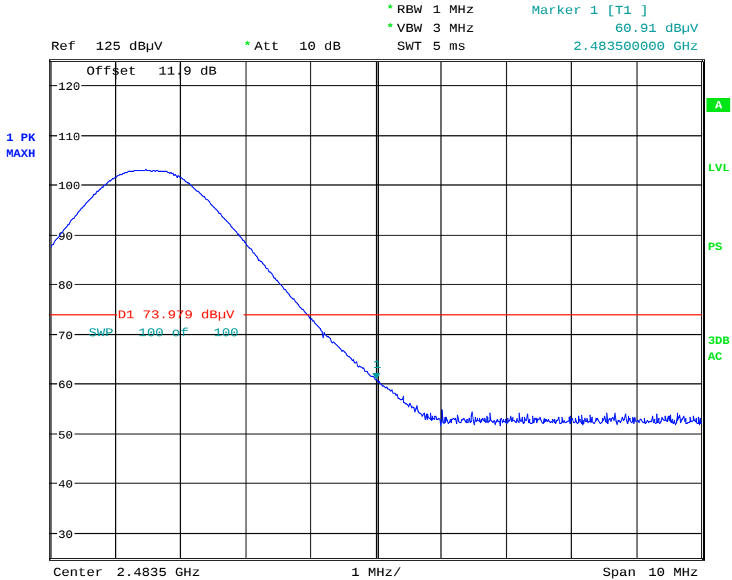
Plot 6-4. Radiated Restricted Upper Band Edge Measurement (Peak)
