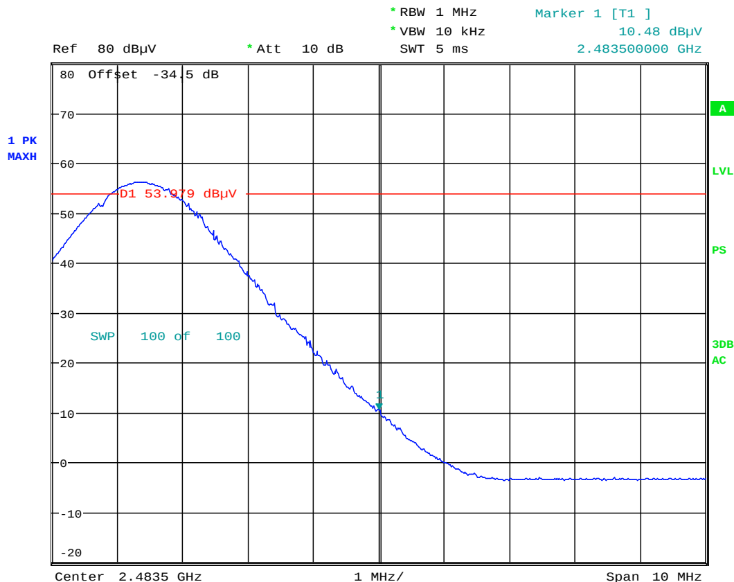
Plot 6-3. Radiated Restricted Upper Band Edge Measurement (Average)
