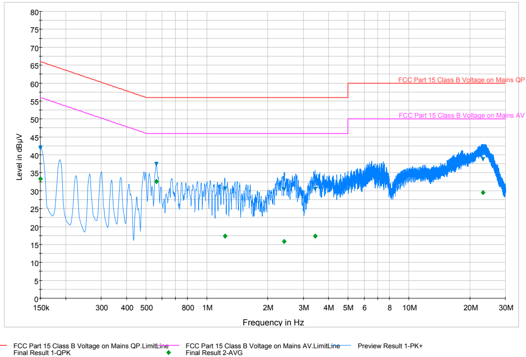
Plot 6-5. Line Conducted Plot with ANT+ (L1)
