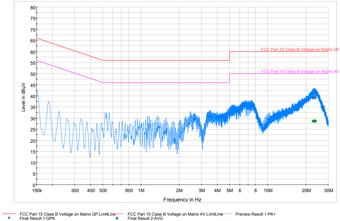
Plot 6-6. Line Conducted Plot with ANT+ (N)
