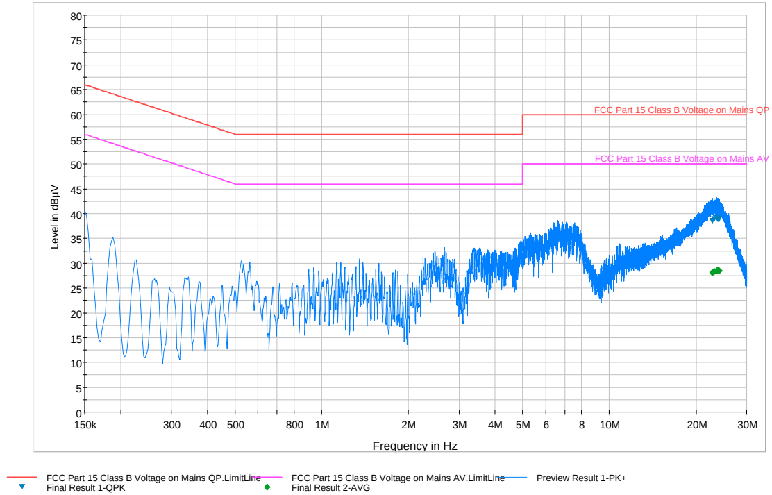
Plot 6-76. Line Conducted Plot with 802.11a UNII Band 2A (N)
