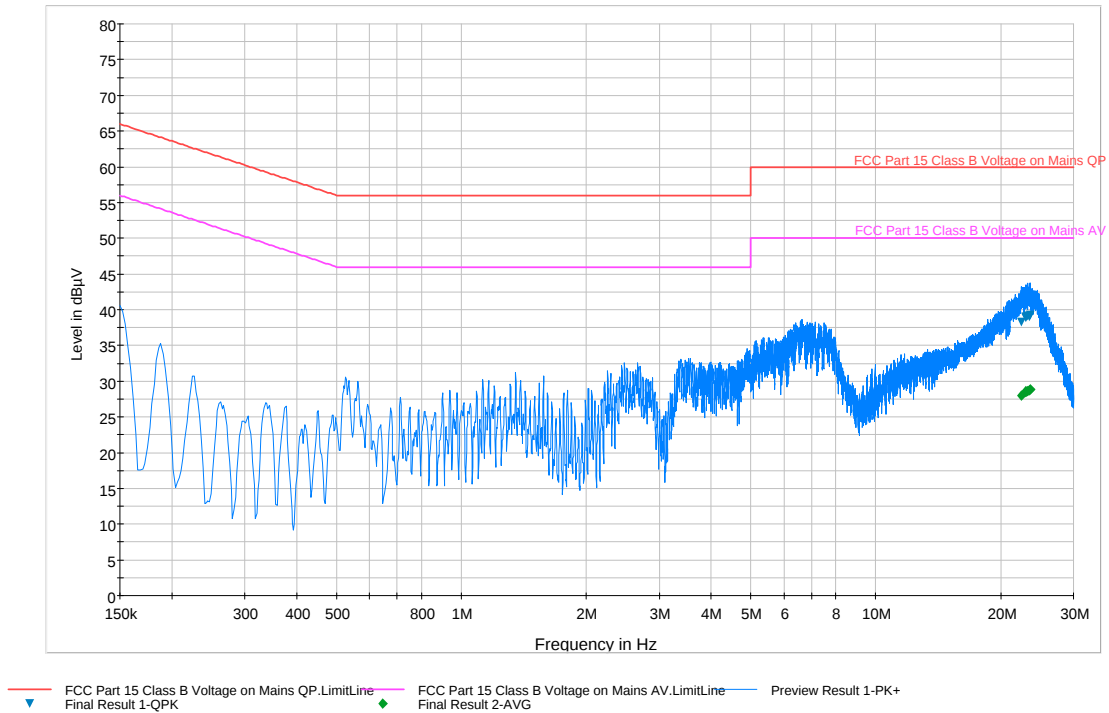
Plot 6-74. Line Conducted Plot with 802.11a UNII Band 1 (N)
