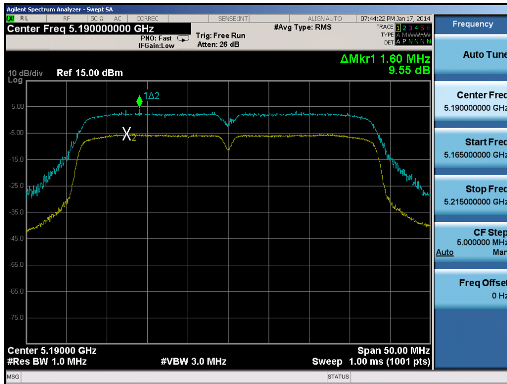
Plot 6-58. Peak Excursion Ratio Plot (40MHz BW 802.11n)
