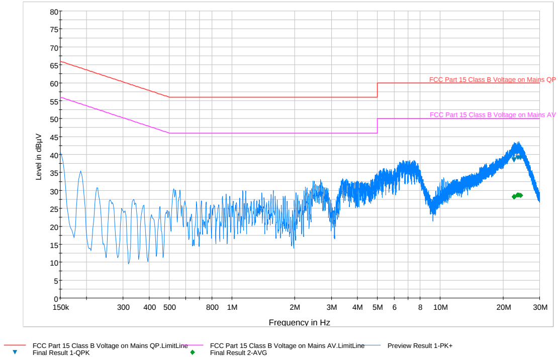
Plot 6-78. Line Conducted Plot with 802.11a UNII Band 2C (N)
