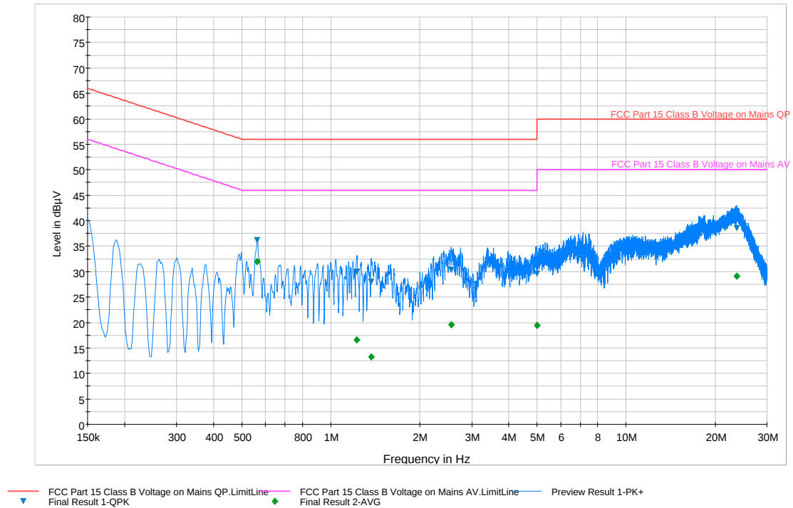
Plot 6-75. Line Conducted Plot with 802.11a UNII Band 2A (L1)
