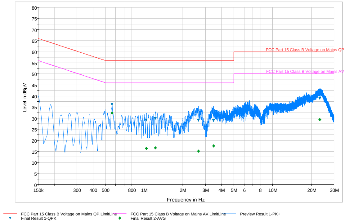
Plot 6-77. Line Conducted Plot with 802.11a UNII Band 2C (L1)
