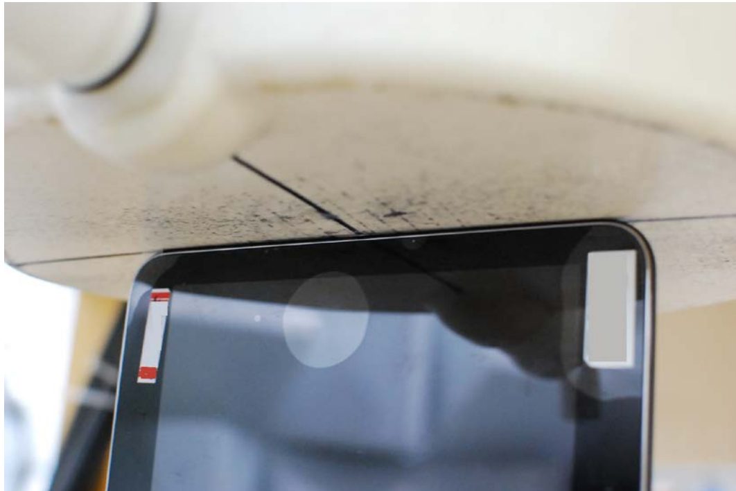
SAR Test Setup Photo 4: Right at 0.0 mm
