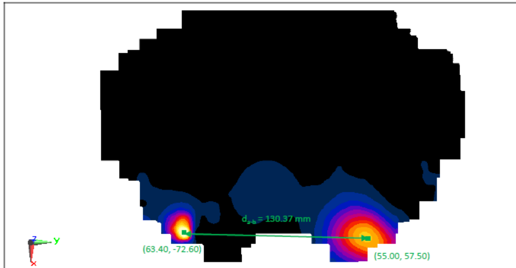
Figure 11-4 Peak SAR Locations for Body Back Side at 20 mm LTE Band 2 and 2.4 GHz WLAN Antenna
