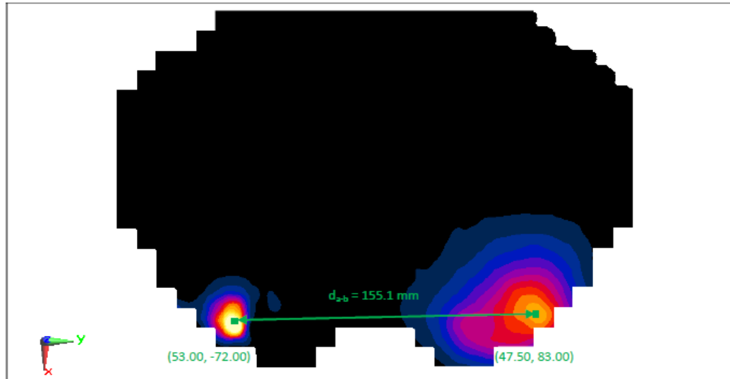
Figure 11-1 Peak SAR Locations for Body Back Side at 0 mm LTE Band 17 and 5 GHz WLAN Antenna
