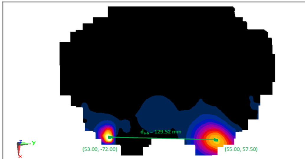
Figure 11-6 Peak SAR Locations for Body Back Side at 20 mm LTE Band 2 and 5 GHz WLAN Antenna
