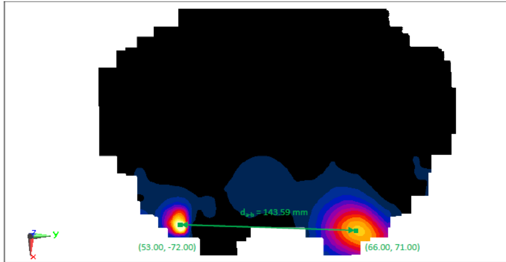
Figure 11-2 Peak SAR Locations for Body Back Side at 0 mm LTE Band 2 and 5 GHz WLAN Antenna
