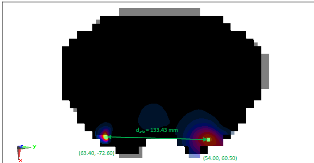
Figure 11-3 Peak SAR Locations for Body Back Side at 20 mm UMTS 1900 and 2.4 GHz WLAN Antenna
