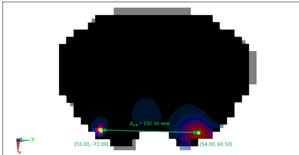
Figure 11-5 Peak SAR Locations for Body Back Side at 20 mm UMTS 1900 and 5 GHz WLAN Antenna
