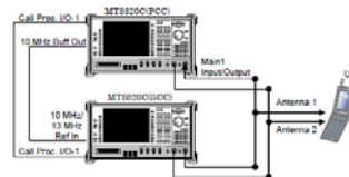
Figure 8-2 Power Measurement Setup
