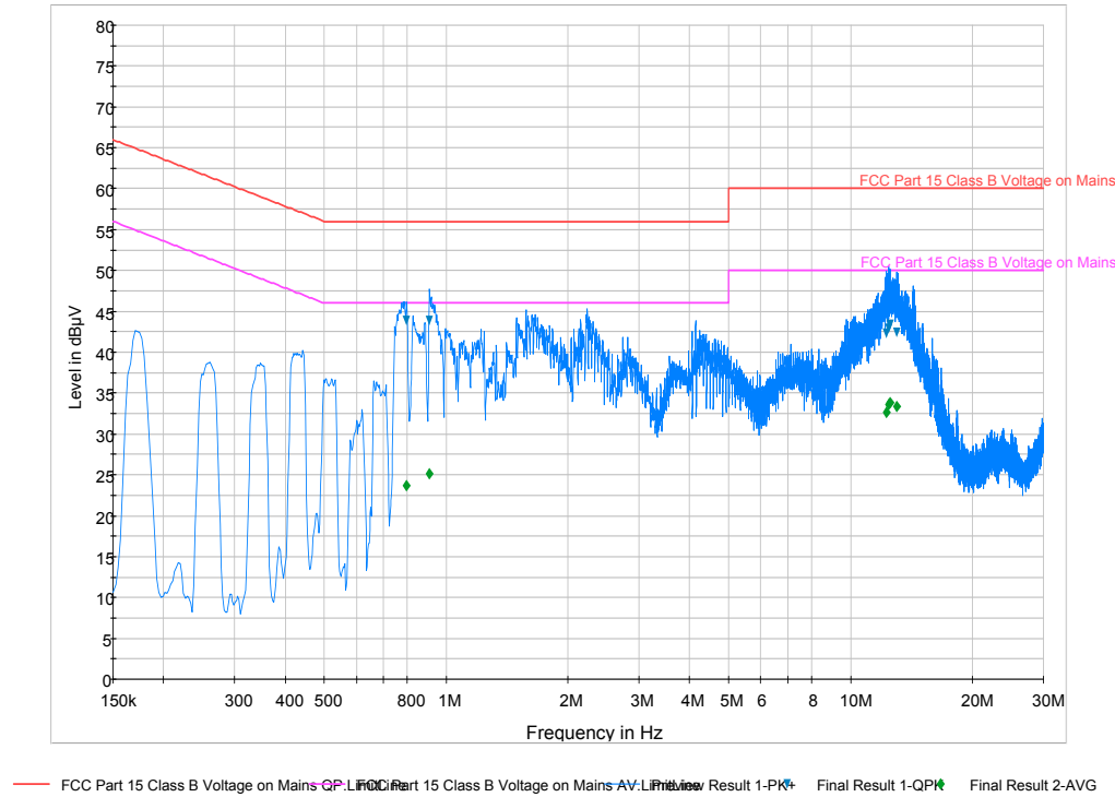
Plot 6-45. Line-Conducted Test Plot (N)
