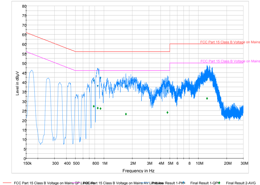
Plot 6-44. Line-Conducted Test Plot (L1)
