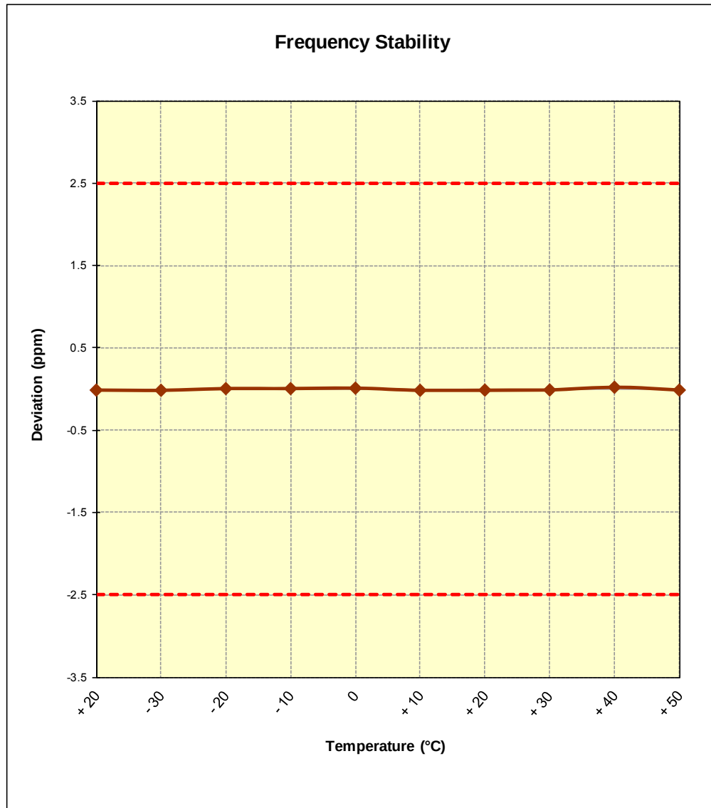
Figure 6-7. Frequency Stability Graph (Cellular WCDMA Mode – Ch. 4183)
