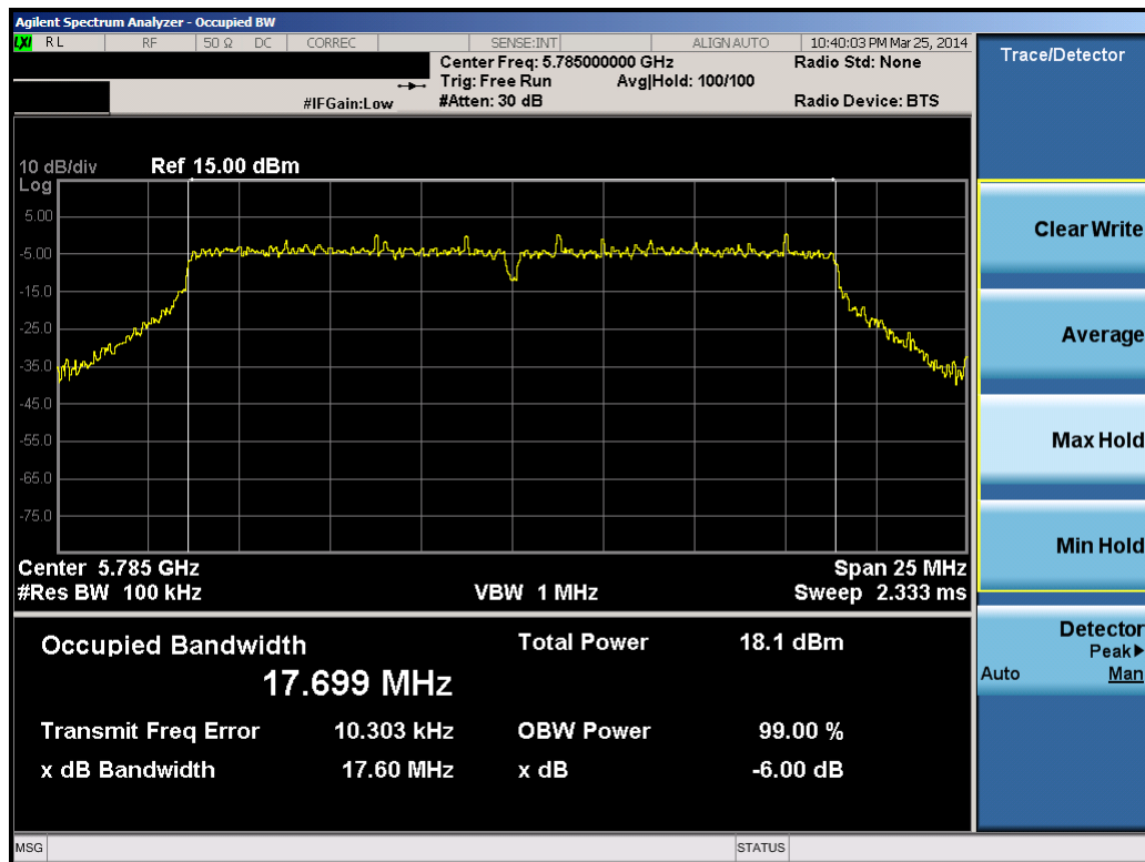
Plot 6-14. 6dB Bandwidth Plot (20MHz BW 802.11a/b/g/n (5.8GHz) – Ch. 157)
