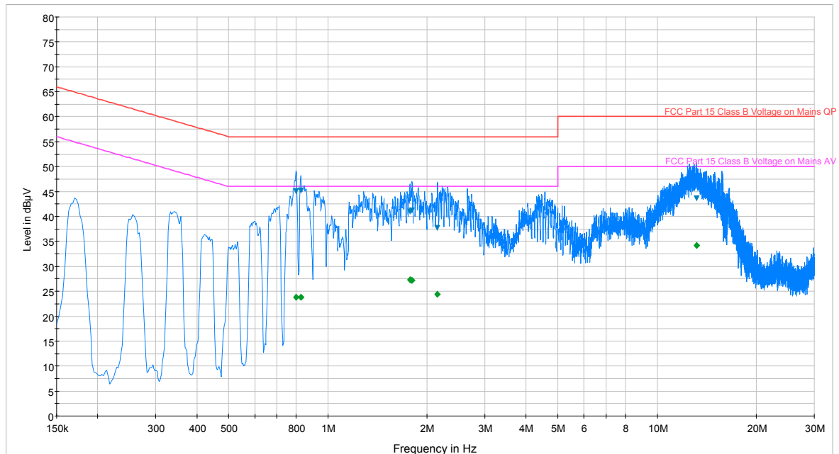
Plot 6-66. Line Conducted Plot with 802.11a (N)
