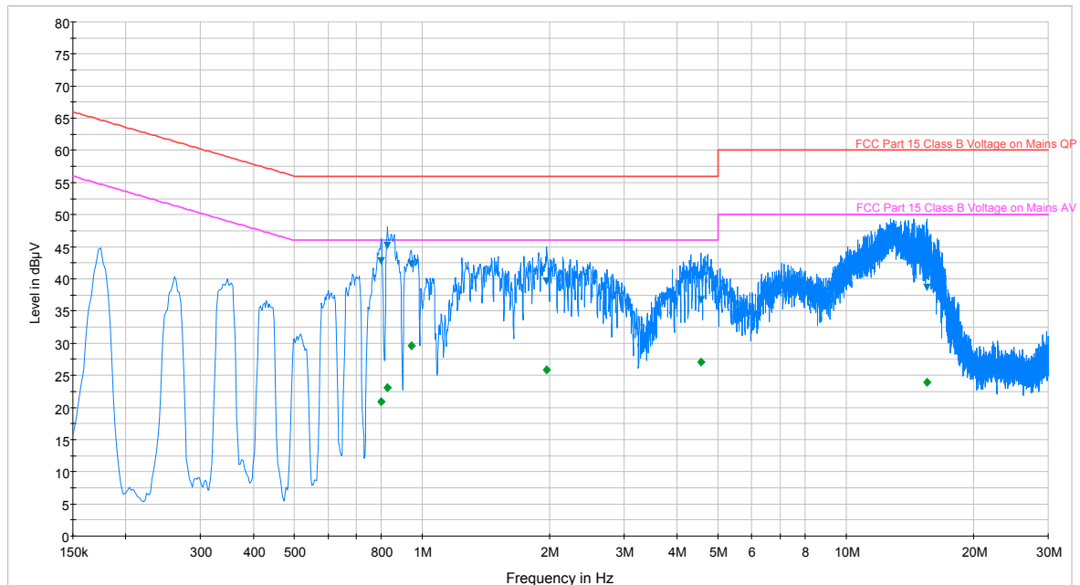
Plot 6-65. Line Conducted Plot with 802.11a (L1)
