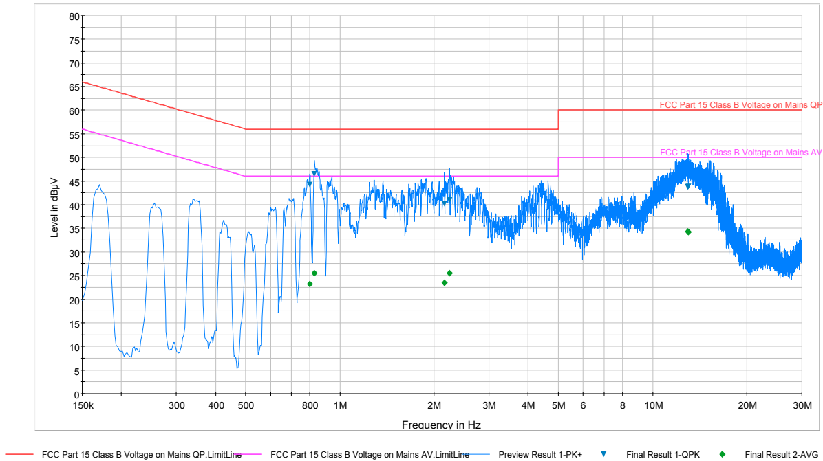
Plot 6-64. Line Conducted Plot with 802.11b (N)
