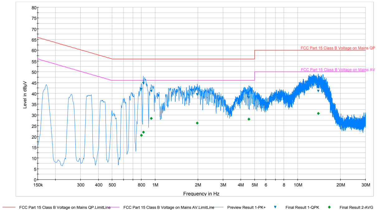
Plot 6-63. Line Conducted Plot with 802.11b (L1)
