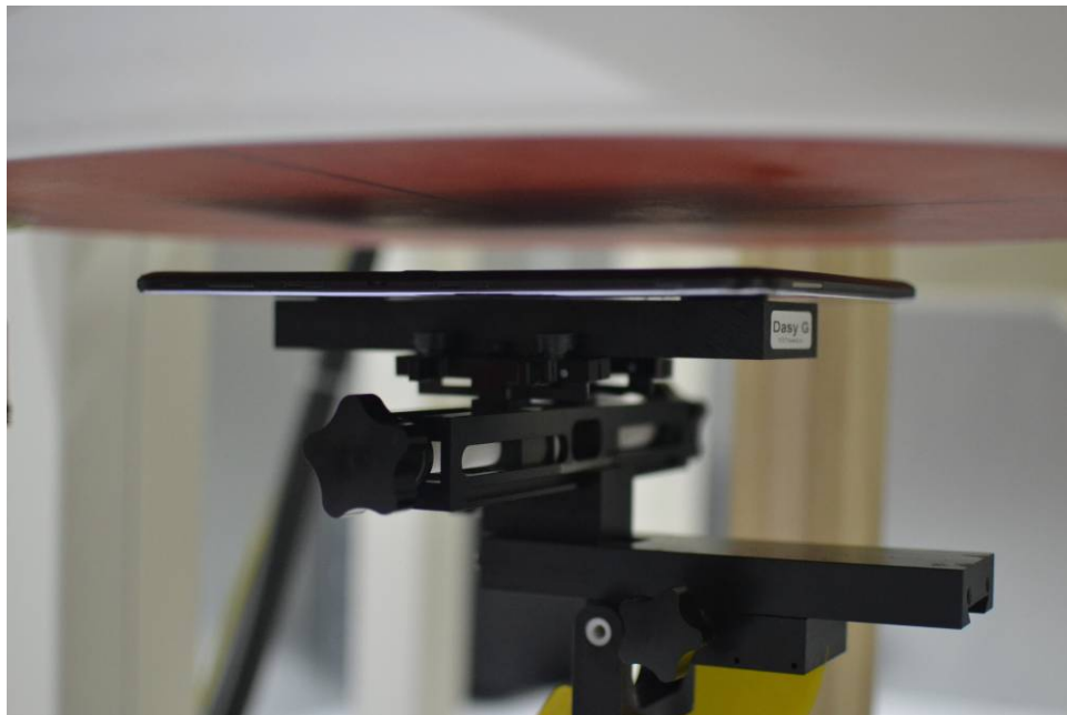
SAR Test Setup Photo 2- Back Side at 22 mm
