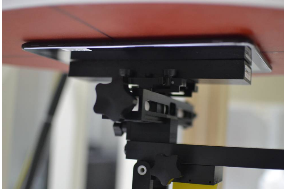
SAR Test Setup Photo 1- Back Side at 0.0 mm
