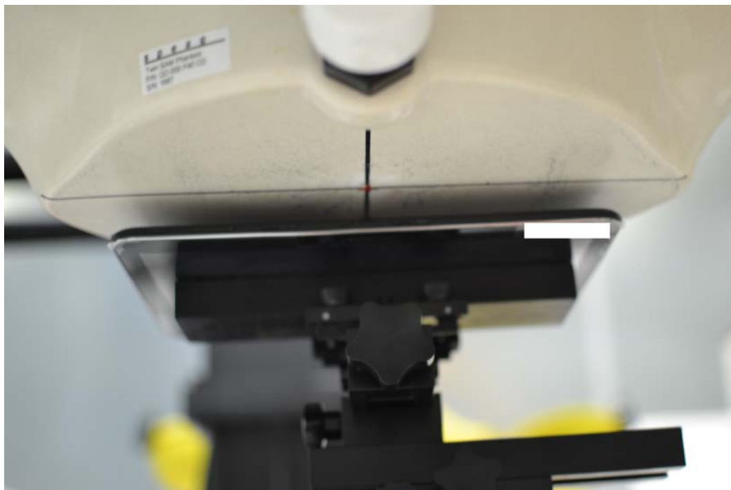
SAR Test Setup Photo 2: Back at 19.0 mm
