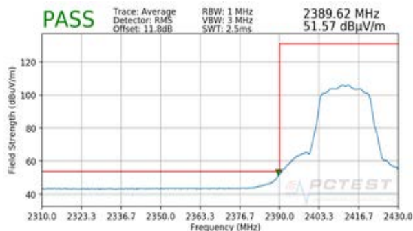
Plot 7-45. Radiated Restricted Lower Band Edge Measurement (Average)
