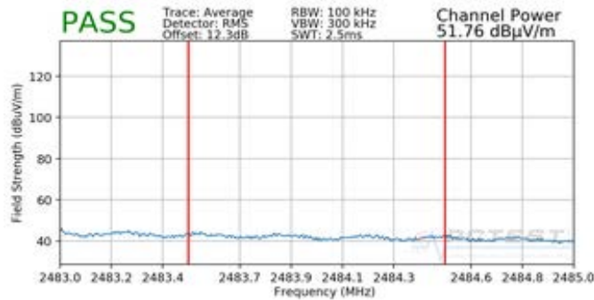
Plot 7-49. Radiated Restricted Upper Band Edge Measurement (Average)
