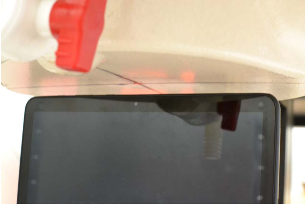
SAR Test Setup Photo 3 – Top Edge at 0.6 cm
