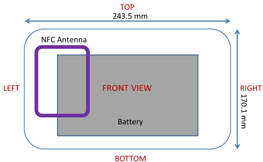
Figure F-2 NFC Antenna Location
