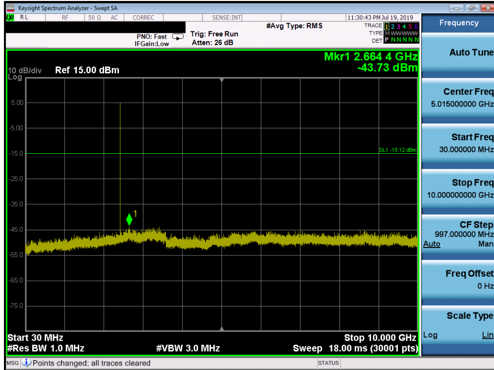
Plot 7-25. Conducted Spurious Plot (Bluetooth (LE), 2Mbps – Ch. 19)
