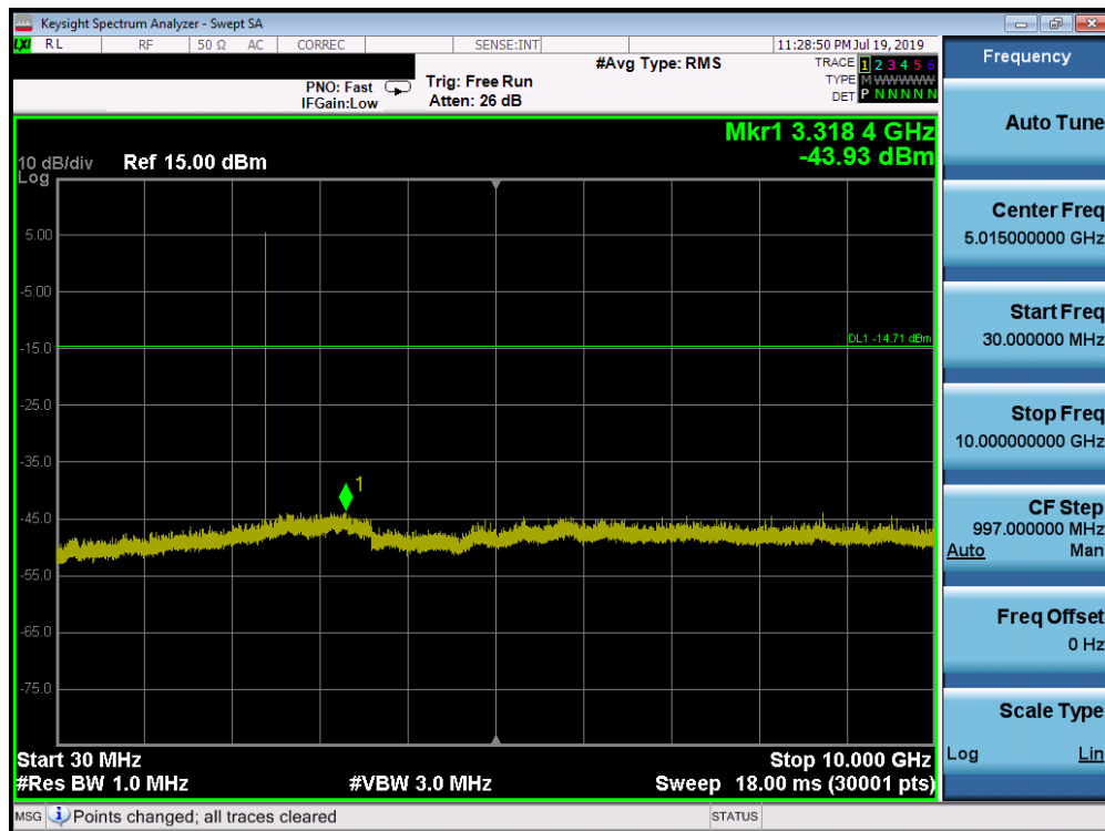
Plot 7-23. Conducted Spurious Plot (Bluetooth (LE), 2Mbps - Ch. 0)
