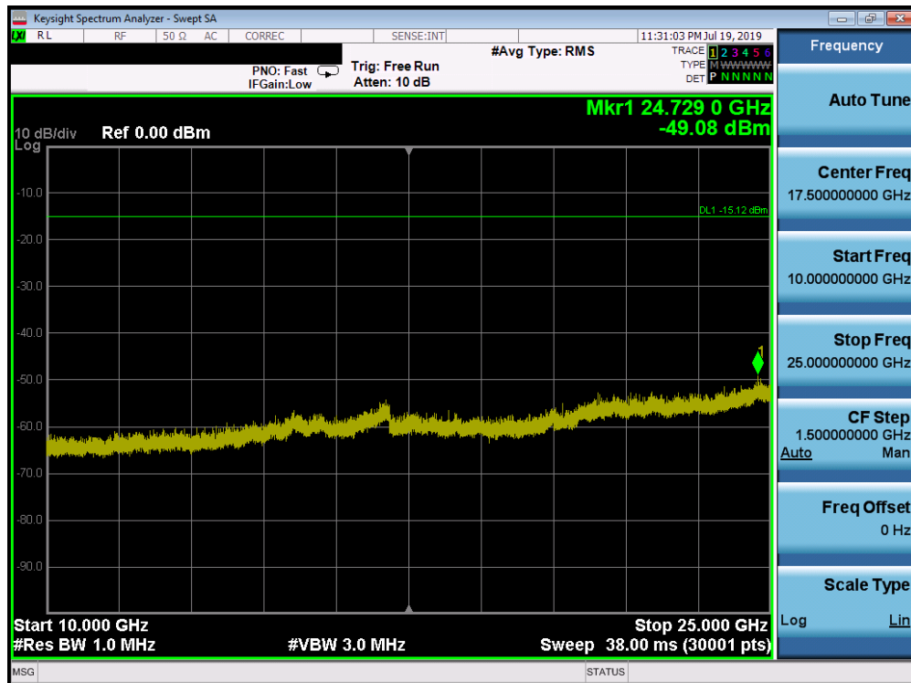
Plot 7-26. Conducted Spurious Plot (Bluetooth (LE), 2Mbps – Ch. 19)
