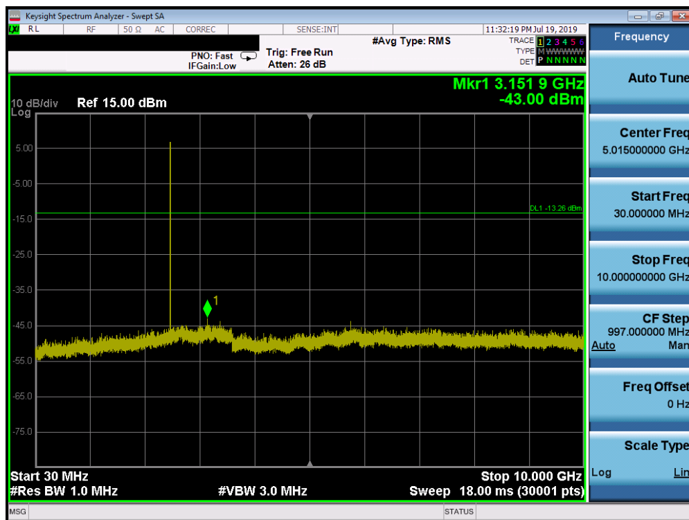
Plot 7-27. Conducted Spurious Plot (Bluetooth (LE), 2Mbps - Ch. 39)
