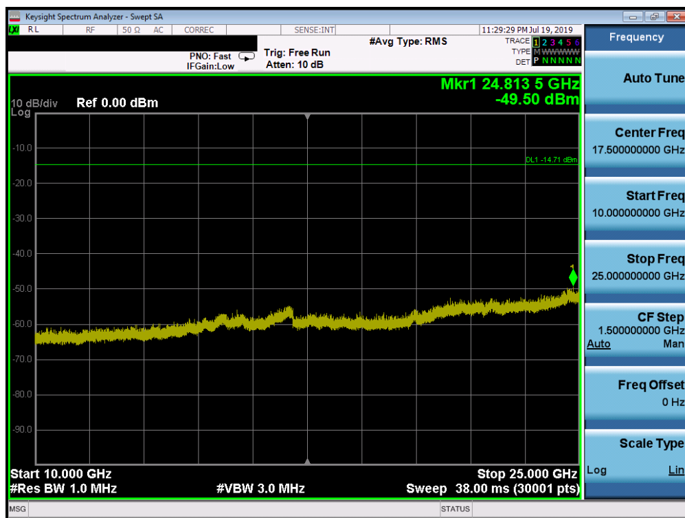
Plot 7-24. Conducted Spurious Plot (Bluetooth (LE), 2Mbps - Ch. 0)
