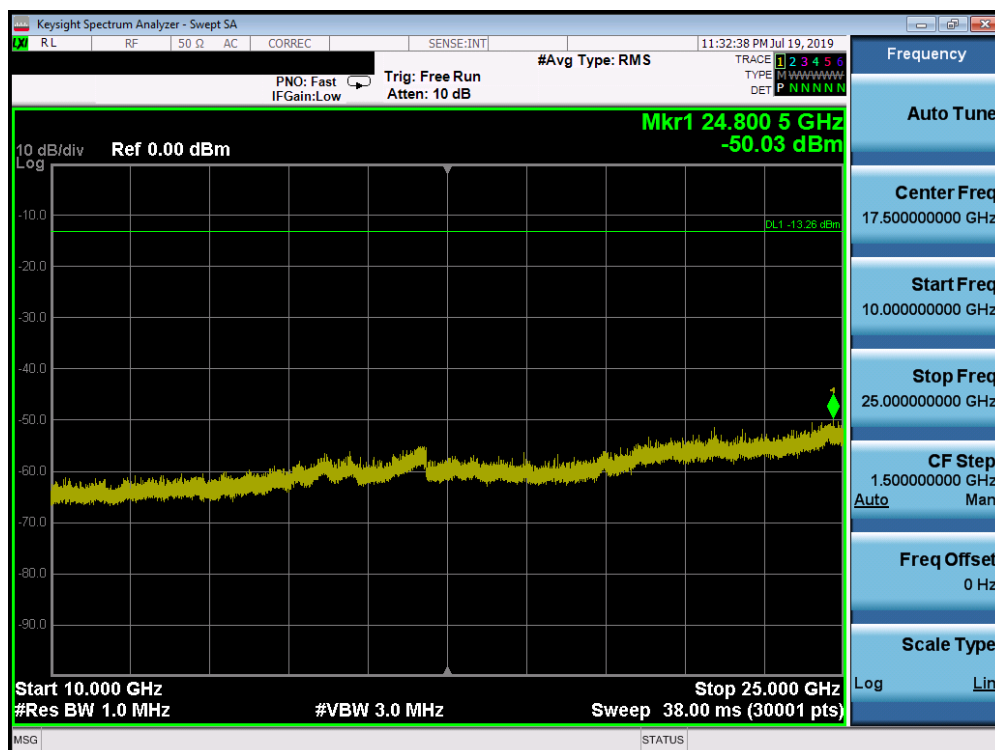
Plot 7-28. Conducted Spurious Plot (Bluetooth (LE), 2Mbps - Ch. 39)
