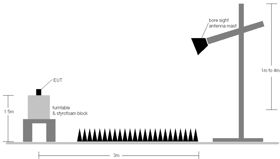
Figure 7-8. Test Instrument & Measurement Setup >1 GHz
