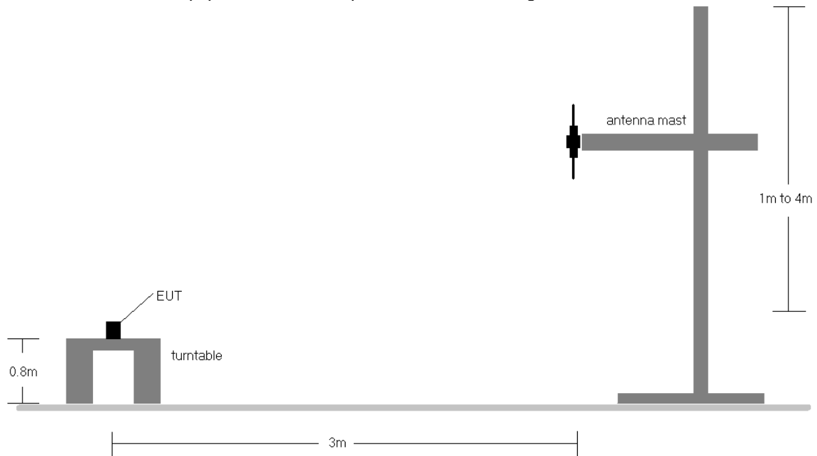
Figure 7-5. Radiated Test Setup <1GHz
