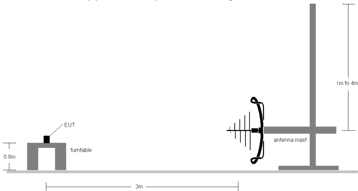
Figure 7-7. Test Instrument & Measurement Setup < 1GHz
