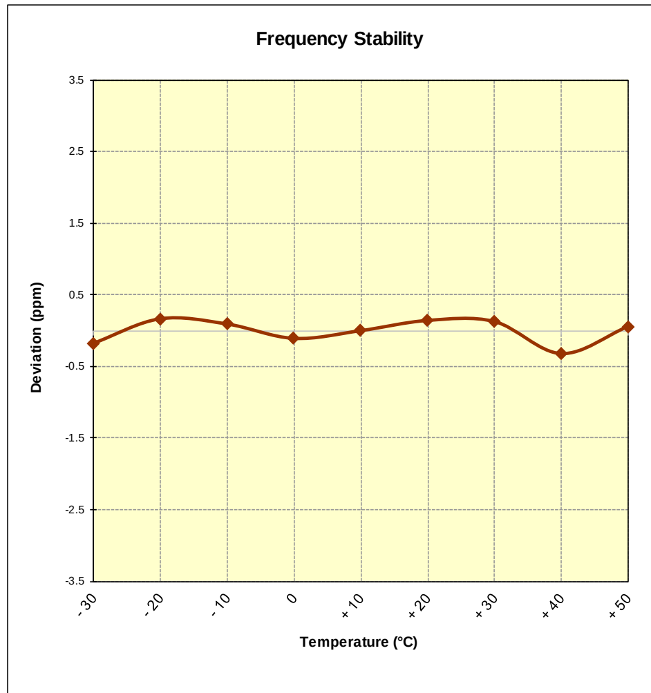
Figure 7-10. Frequency Stability Graph (Cellular WCDMA Mode – Ch. 4183)
