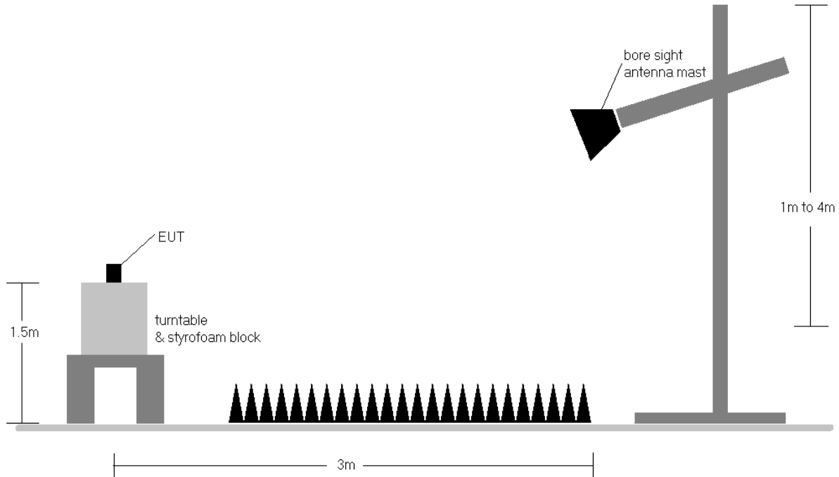
Figure 7-6. Radiated Test Setup >1GHz
